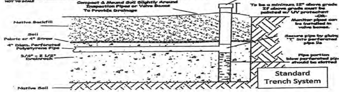
Monitor Pipe Detail ( To be installed at all trench ends) NOT TO SCALE
