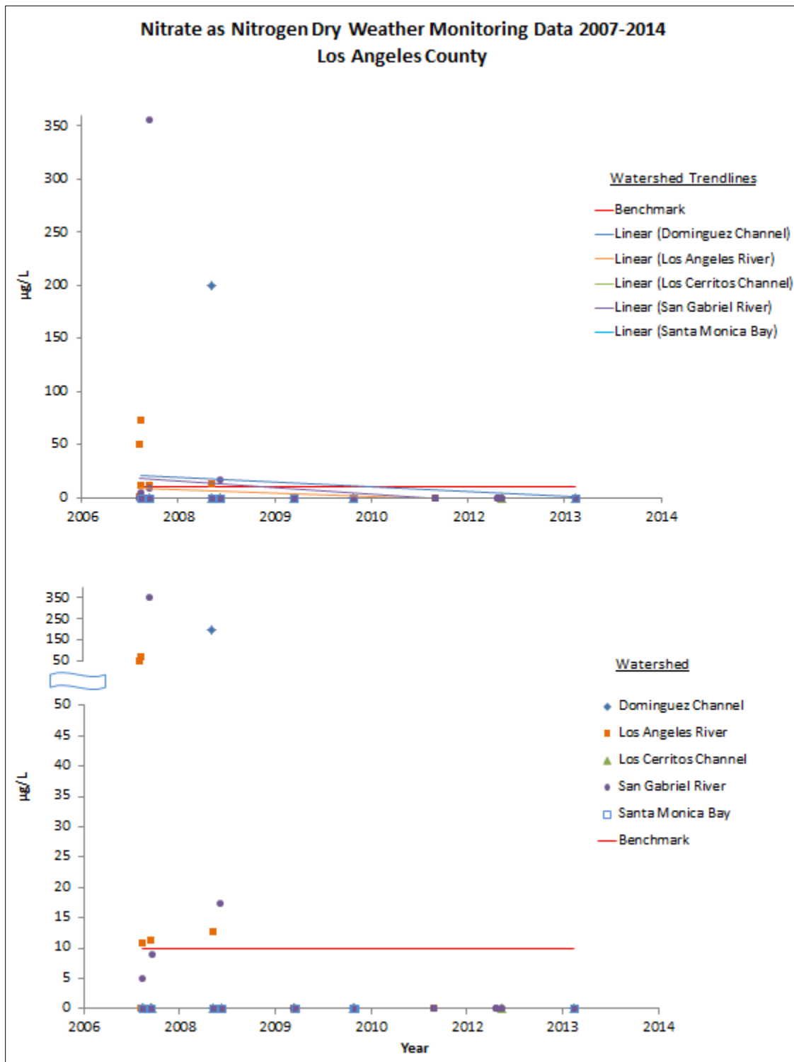
Figure 24 Nitrate as Nitrogen dry weather monitoring data 2007-2014, Los Angeles County (Y-axis on bottom graph is split to show detail.)
