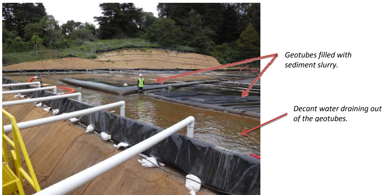
Figure 2. Sediment dewatering in geotubes with the decant water being pumped to the water treatment system.
