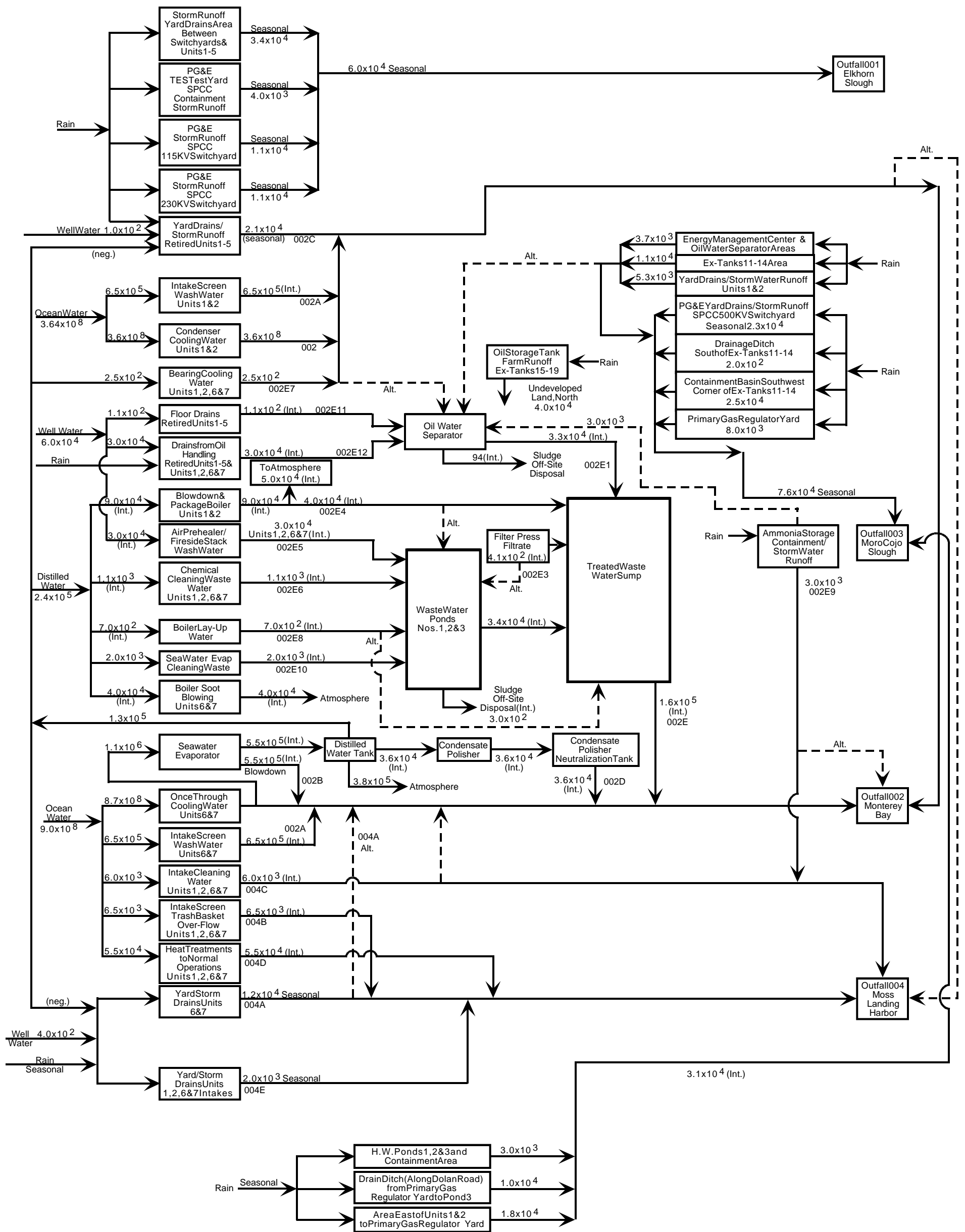
FIGURE 4 PROPOSED DUKE ENERGY MOSS LANDING POWER PLANT WATER FLOW SCHEMATIC FOR UNITS 1, 2, 6 AND 7
