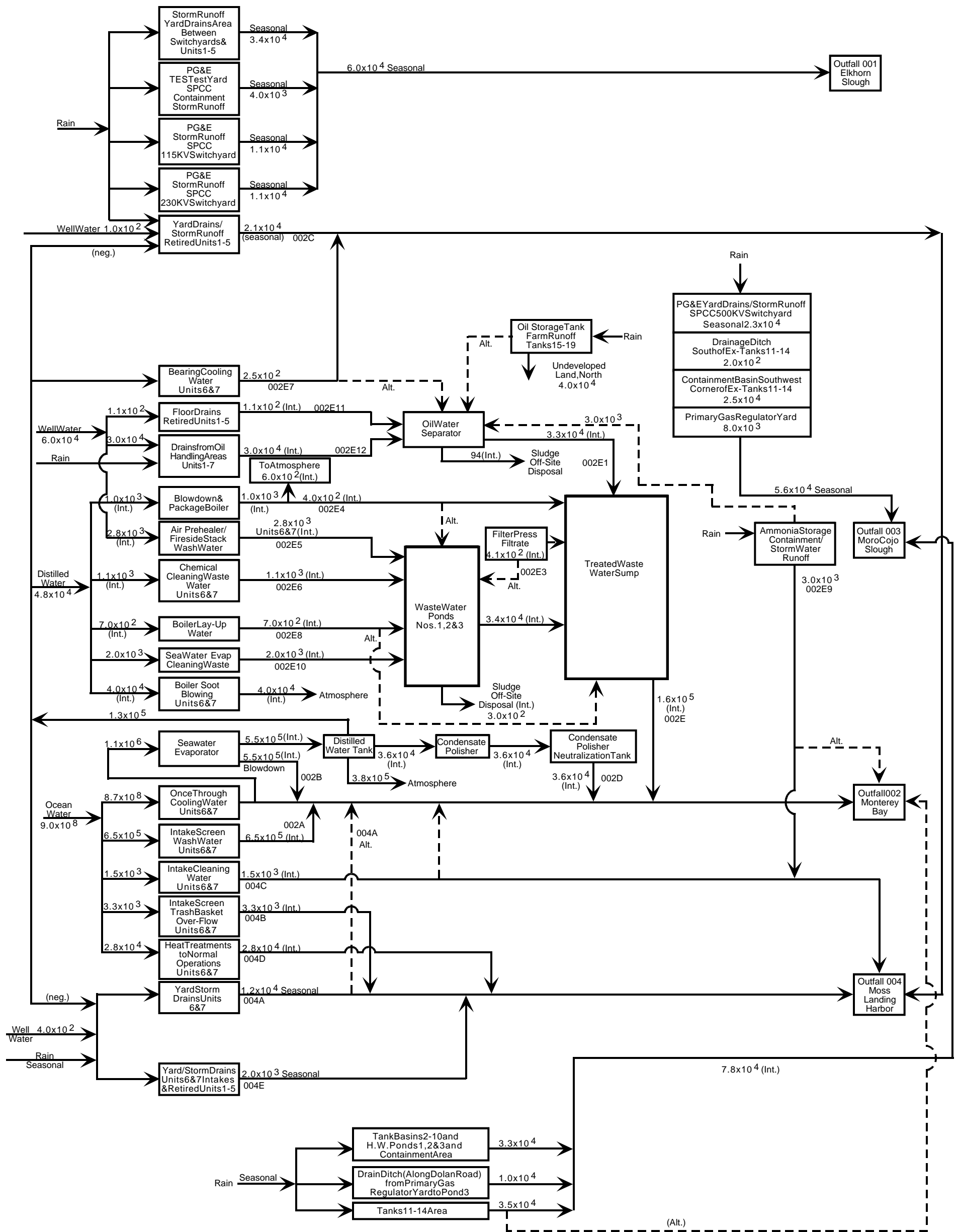
FIGURE 3 EXISTING DUKE ENERGY MOSS LANDING POWER PLANT WATER FLOW SCHEMATIC FOR UNITS 6 AND 7
