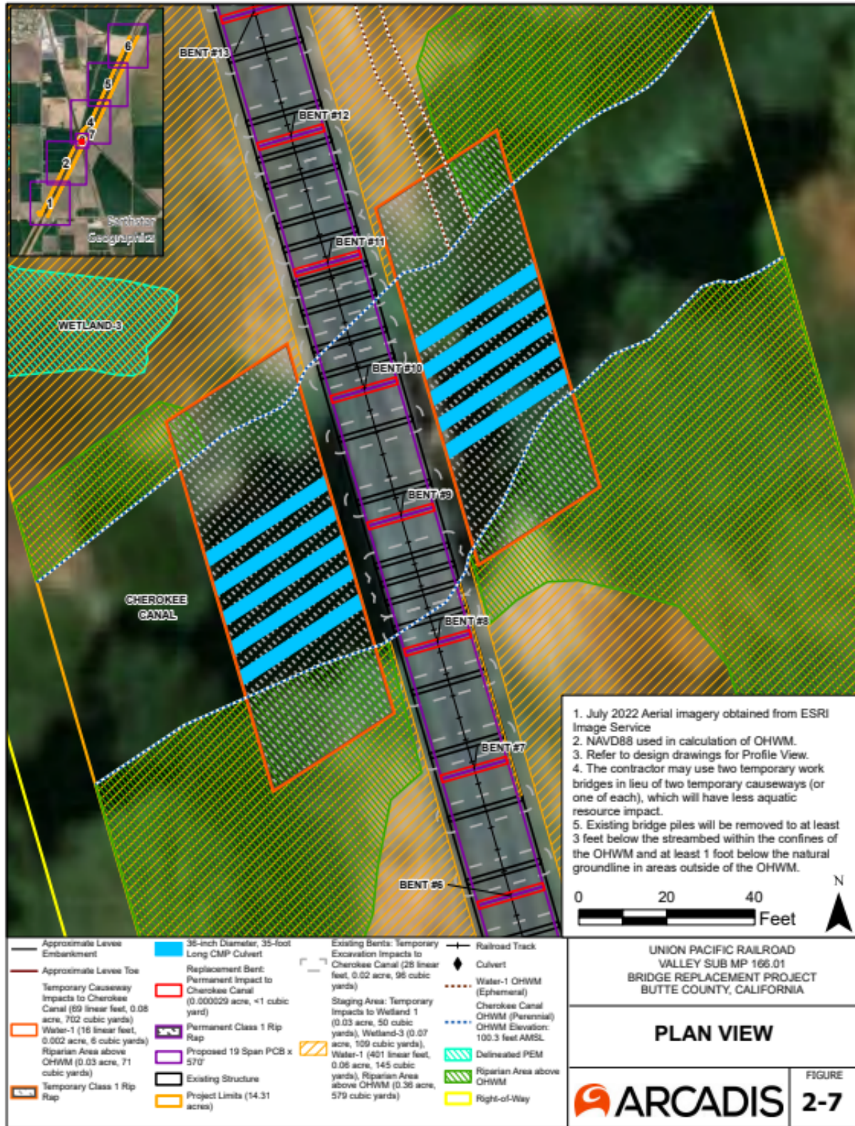
Figure 8: Project Area Impacts - Bridge
