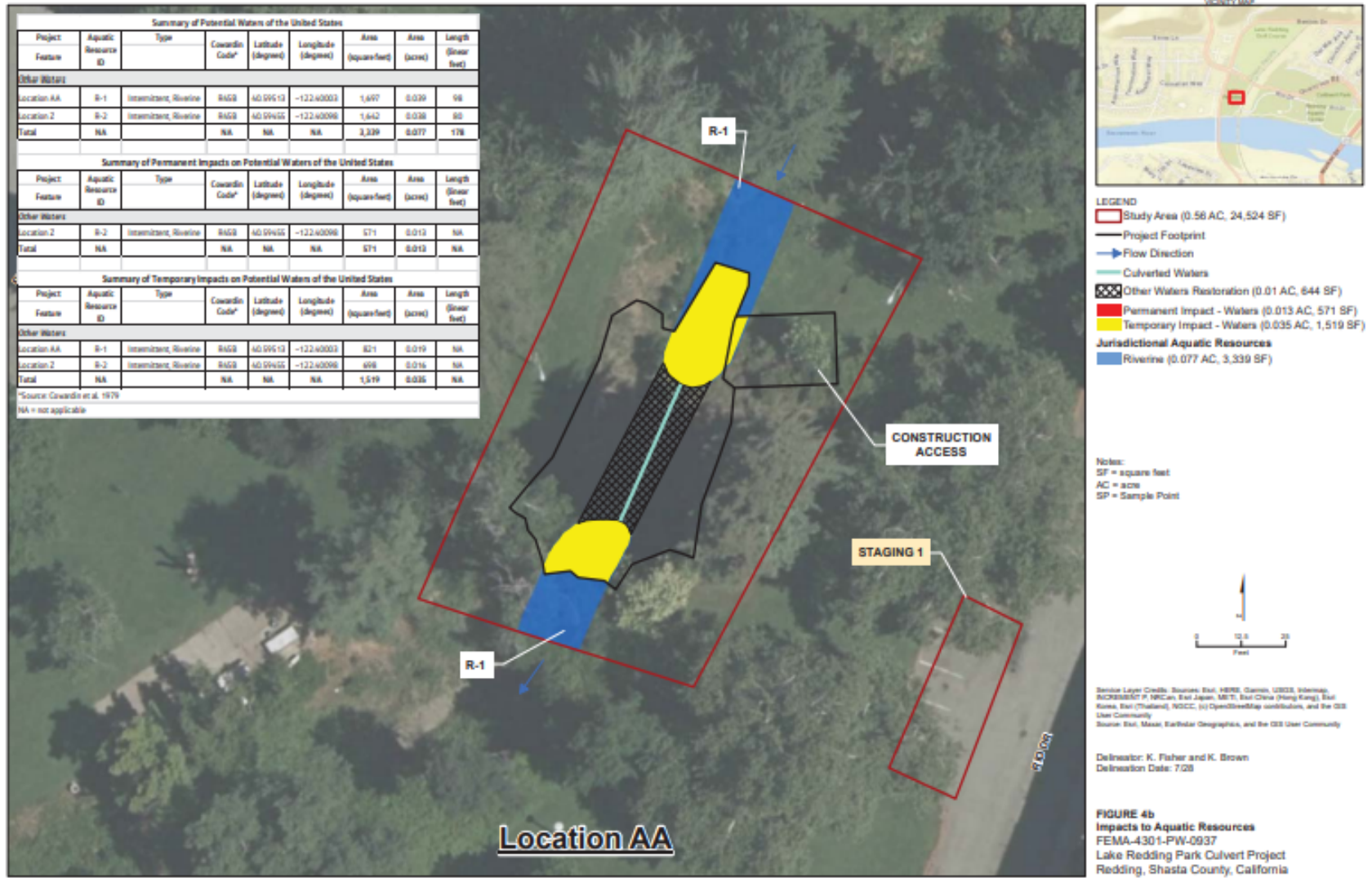
Figure 2. Project Impacts – Location AA
