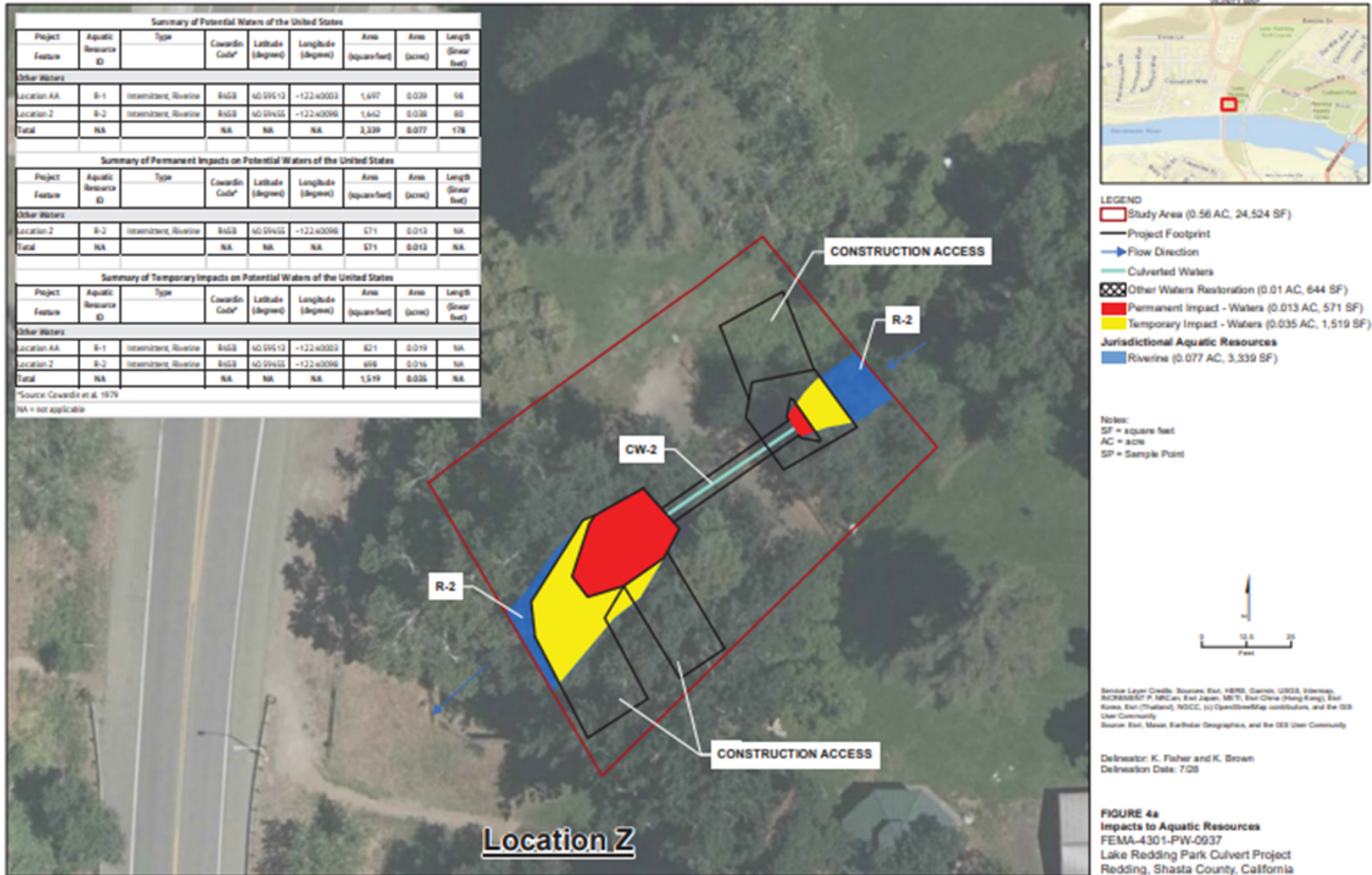
Figure 3. Project Impacts – Location Z
