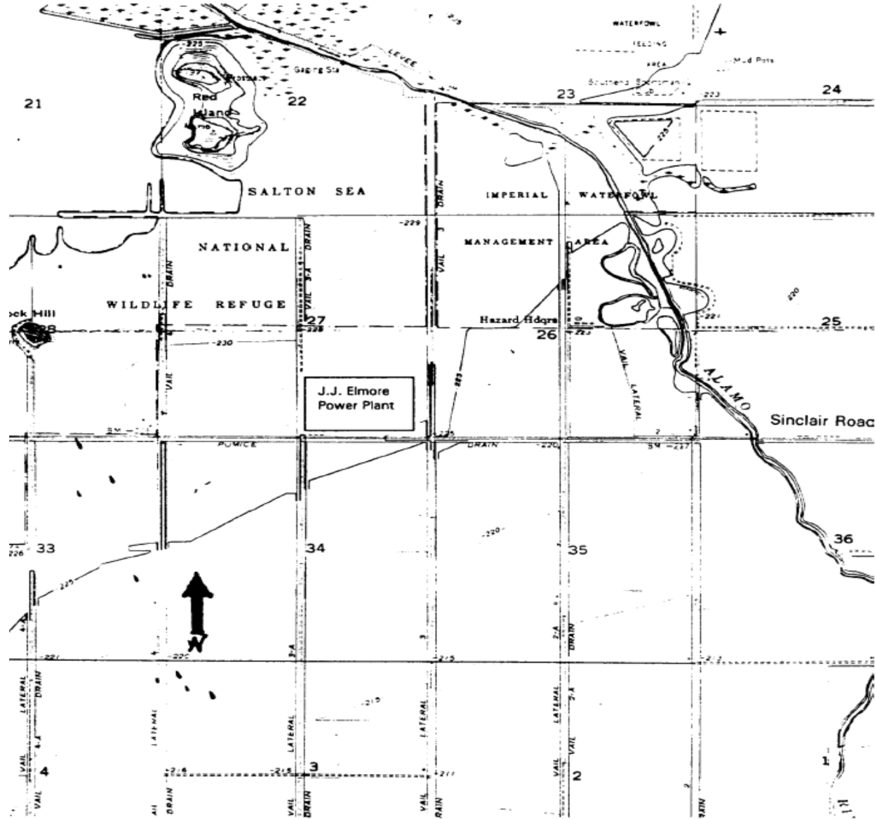
VICINITY MAP MAGMA POWER COMPANY, OWNER CAENERGY OPERATING CORPORATION, OPERATOR J.J. ELMORE POWER PLANT HOLDING POND AND WELFIELD BASIN (MUD SUMPS) Salton Sea Known Geothermal Resource Area - Imperial County Board Order R7-2015-0015
