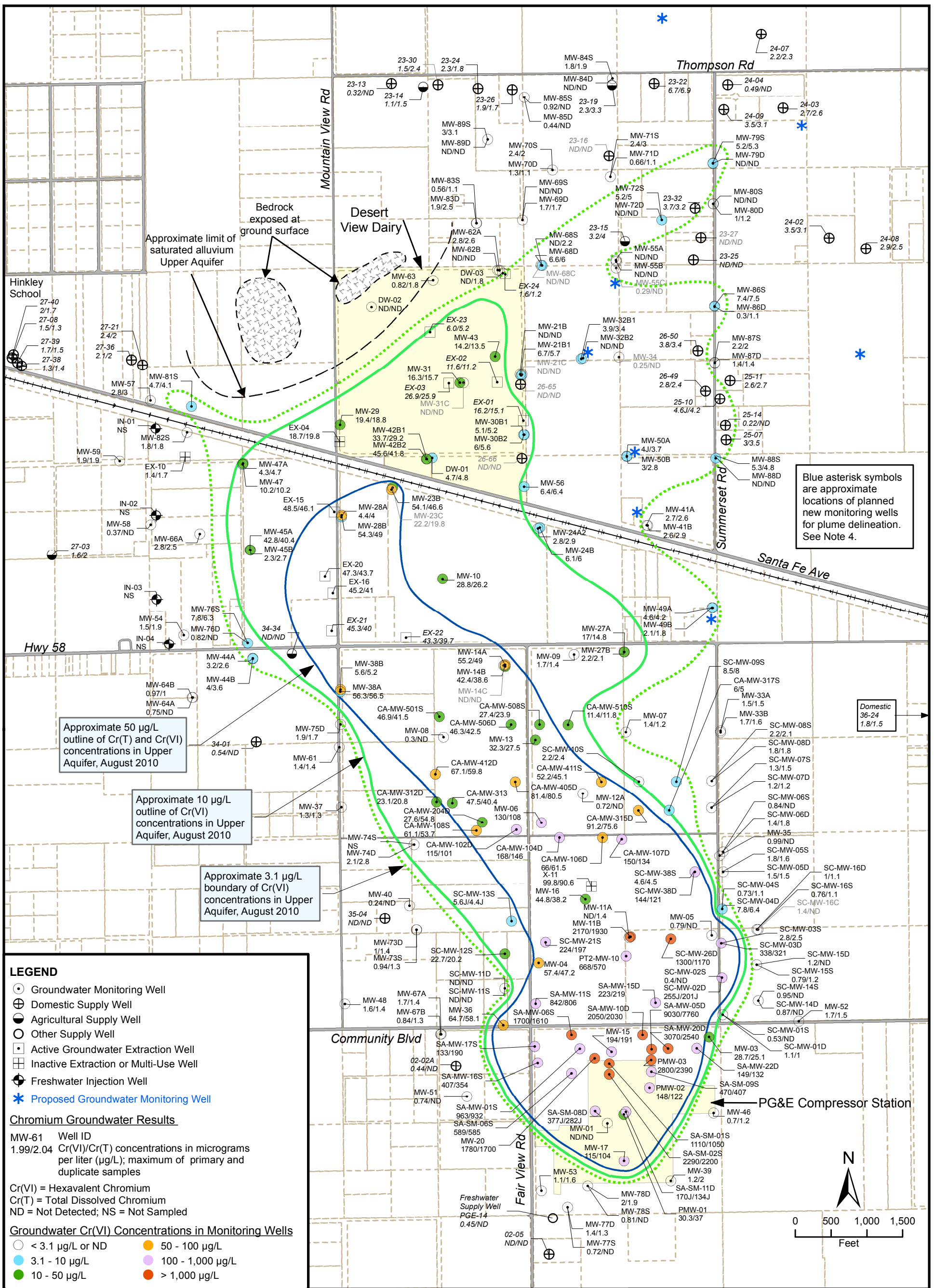
FIGURE 5 HEXAVALENT AND TOTAL CHROMIUM CONCENTRATIONS, AUGUST 2010 AND INTERPRETED MAXIMUM PLUME OUTLINE IN UPPER AQUIFER
