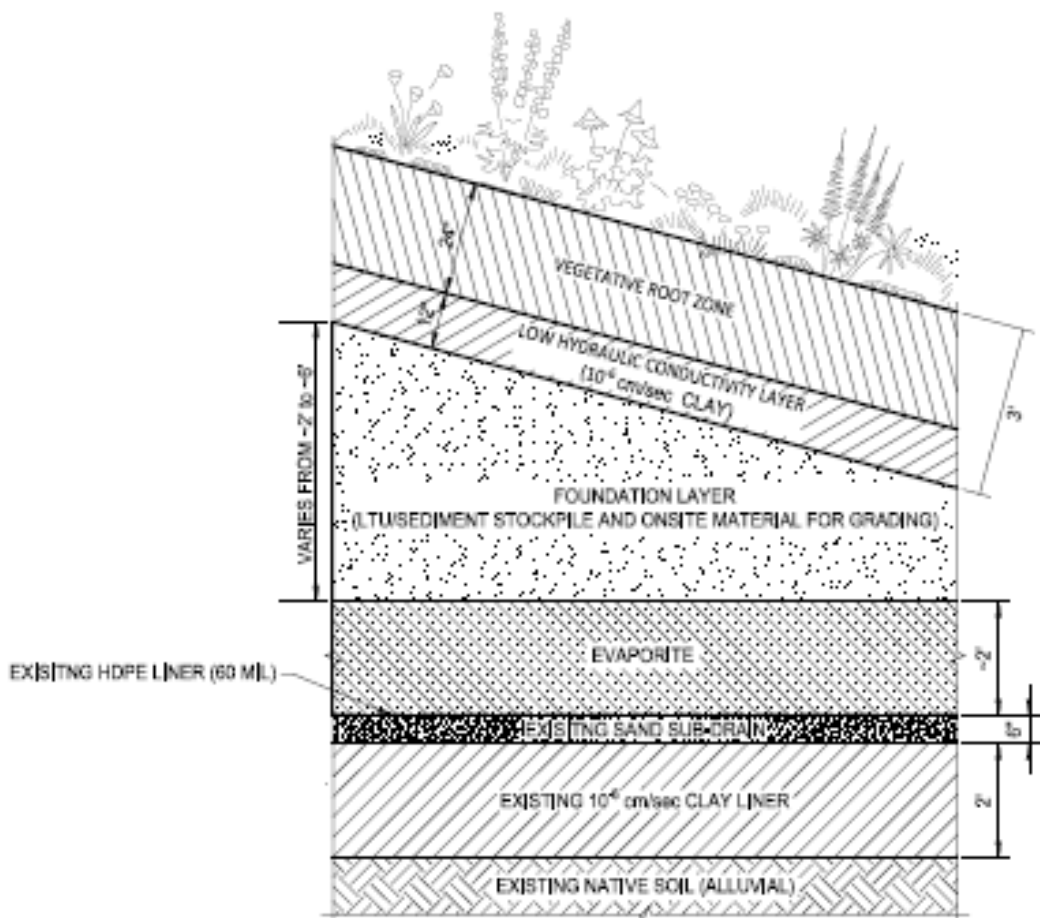
3 5 DETAIL • WEST POND CLOSURE SYSTEM SCALE: 1/2"=1'
