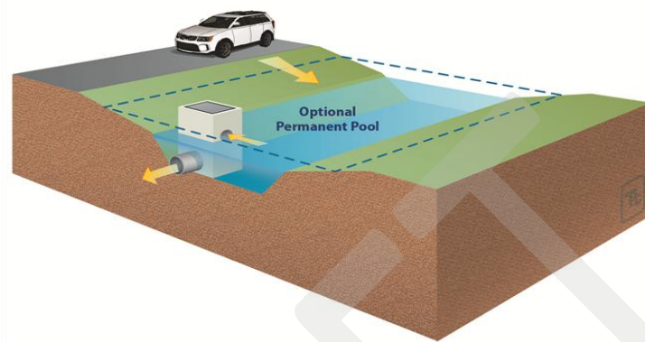
Figure 3-10: Wet detention basin schematic
