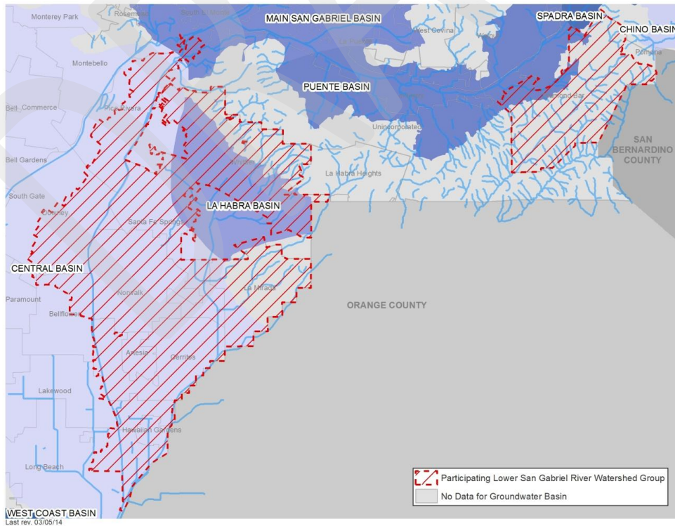
Figure 1-8: Groundwater basins
