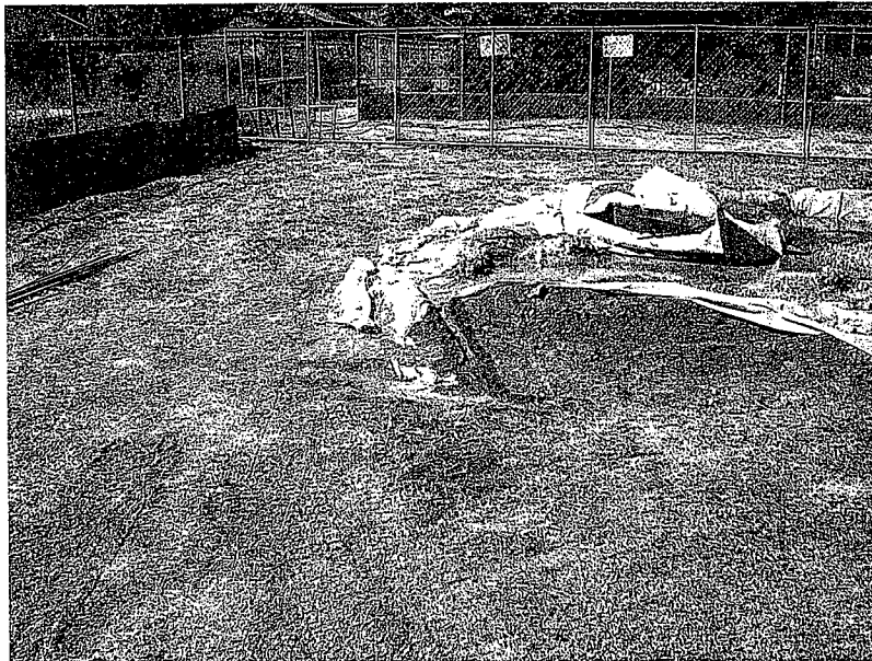
5. Concrete washout area has inadequate construction and capacity to contain washwater. Washwater is spilling onto the ground.
