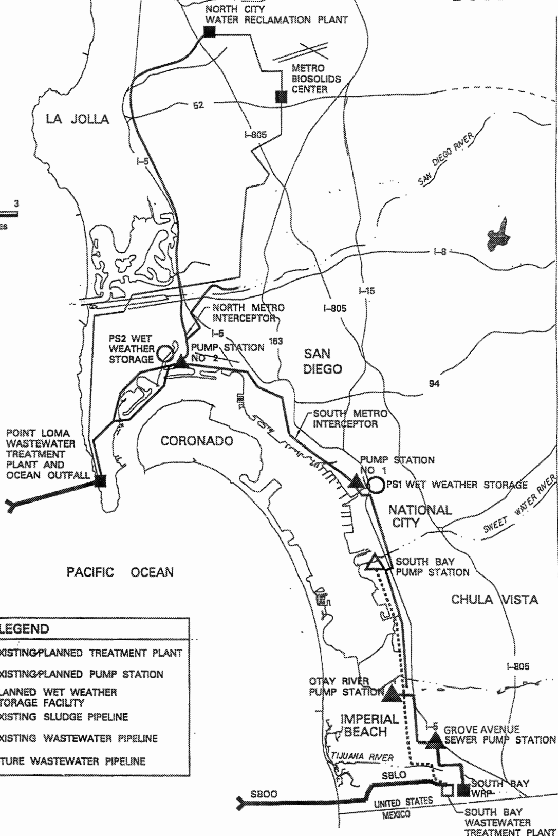
EXISTING AND PLANNED METRO SYSTEM FACILITIES
