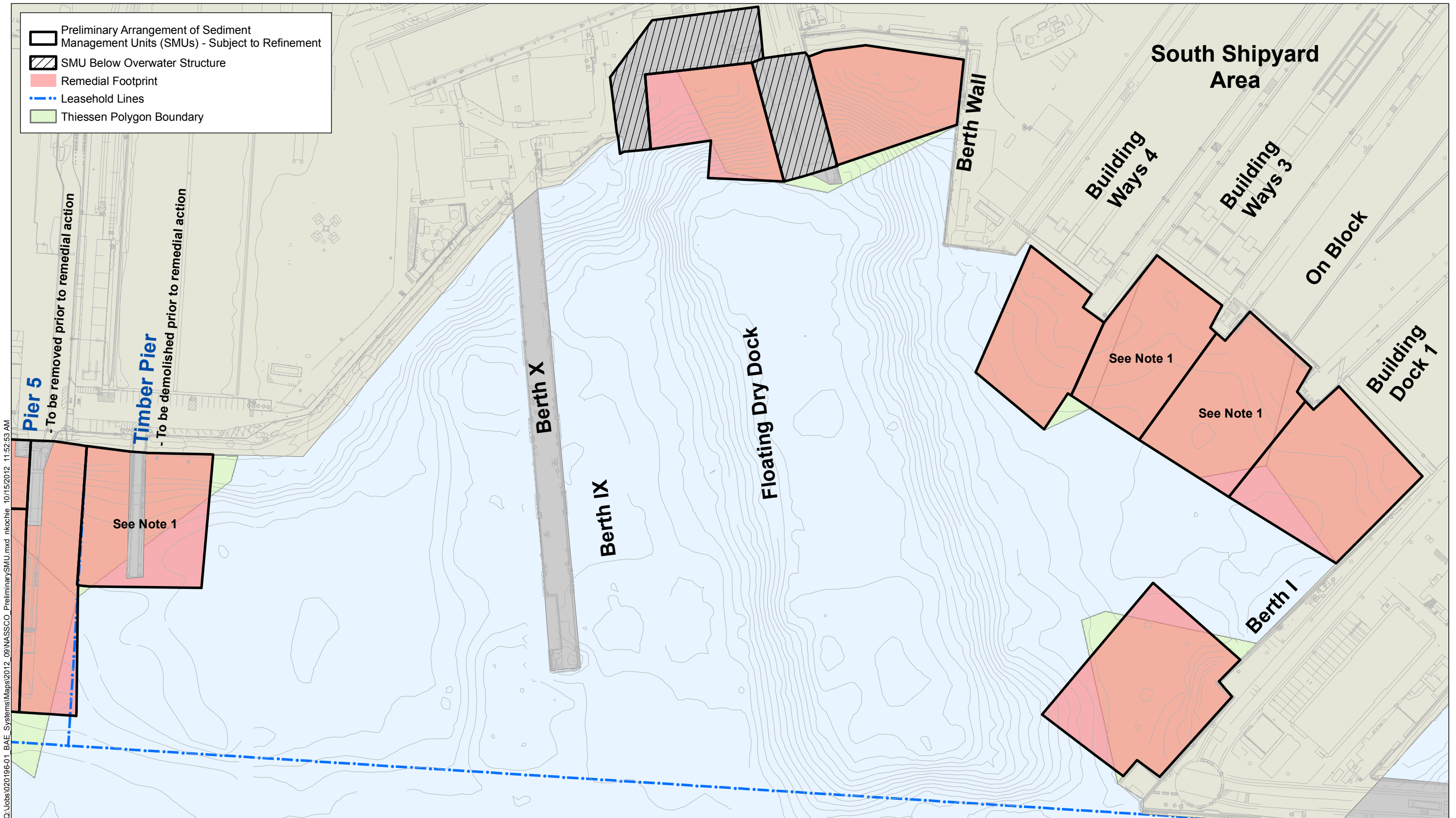
Figure 4 South Shipyard Area Remedial Footprint and SMUs San Diego Shipyard Sediment Site
