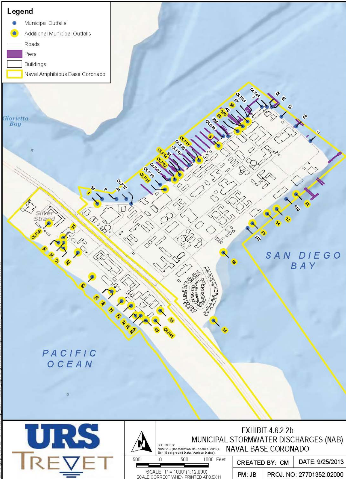
Figure B-1314. NBC Small Military Base MS4 Discharge Locations at NAB
