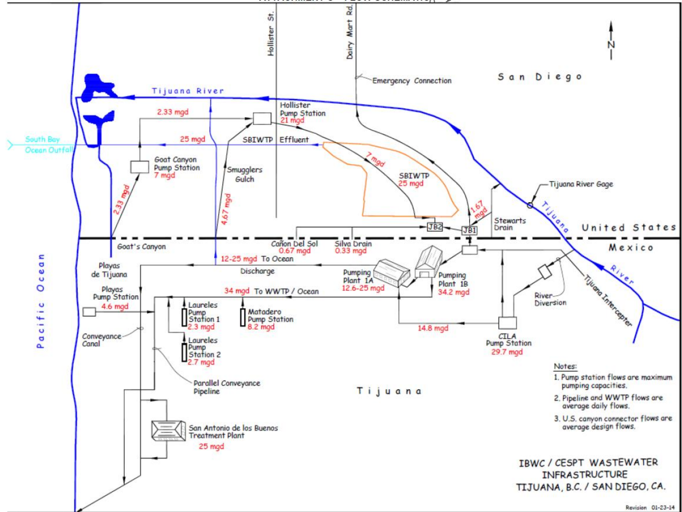
Figure 3. Collection System Flow Schematic in the United States and Mexico.
