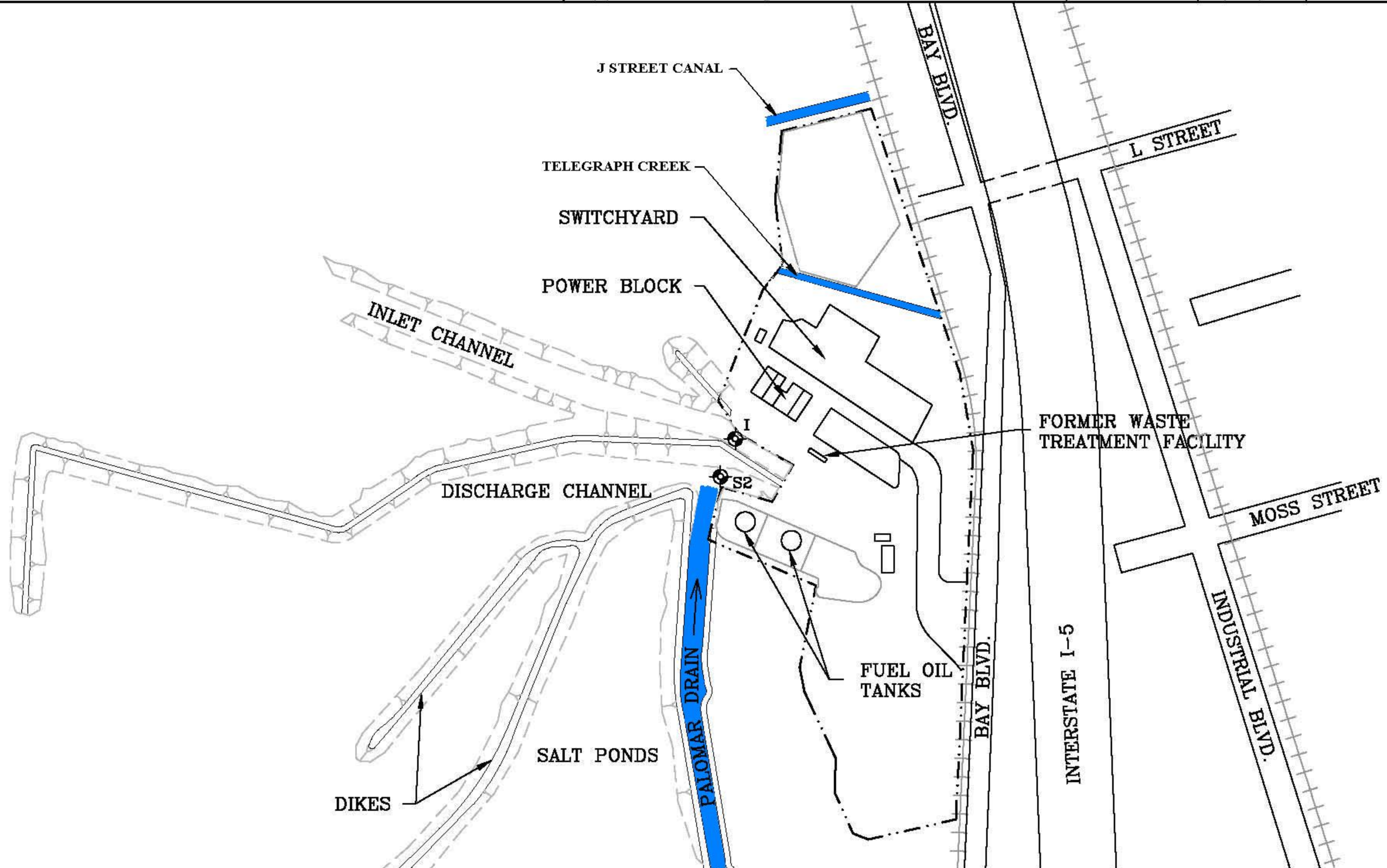
Figure 3 Facility Map Dynegy South Bay, LLC South Bay Power Plant Chula Vista, California
