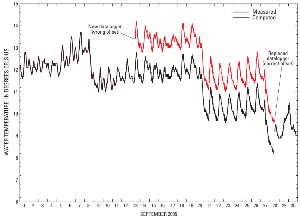
Figure 9. Example of a constant data correction of -1.4 degrees Celsius applied in September 2005 to correct for programming error that produced an incorrect offset at South Fork Tolt River (12148000) near Carnation, Washington.
