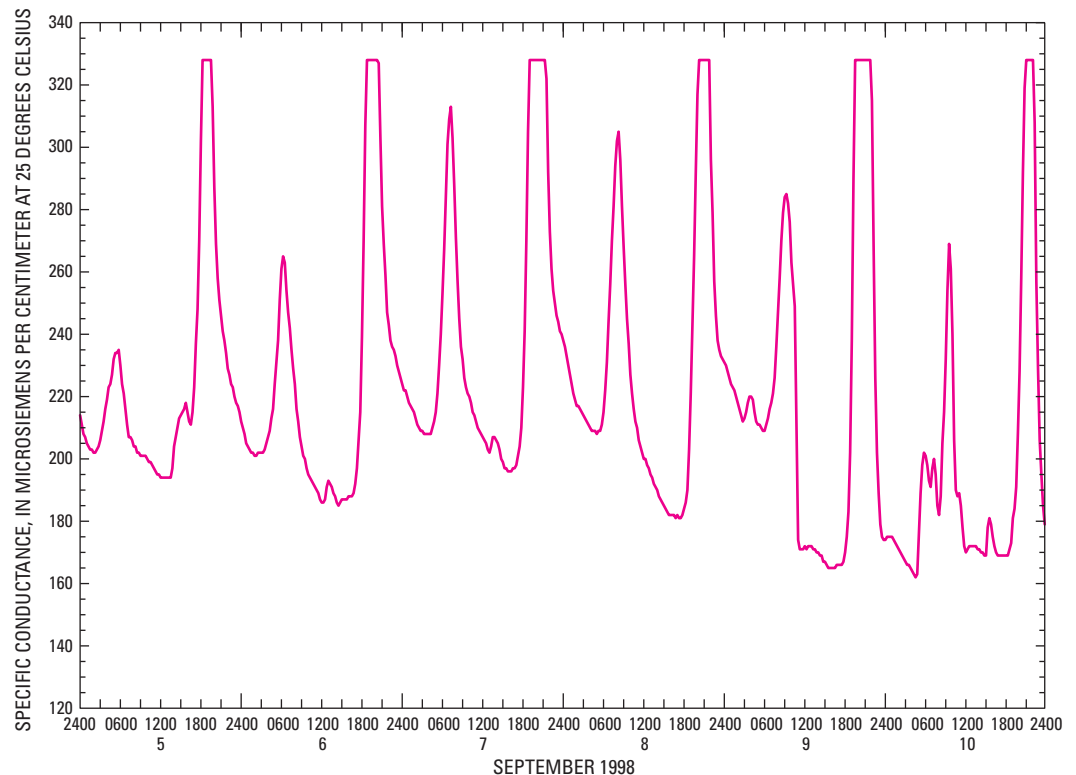
Figure 5. Specific conductance record at Duwamish River at Tukwila, Washington, September 5–10, 1998, was truncated at 330 microsiemens per centimeter, which was the default maximum setting for the data logger.
