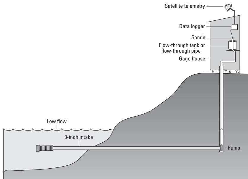
Figure 2. Ramapo River at Pompton Lakes, New Jersey, and schematic of flow-through water-quality monitoring station.
