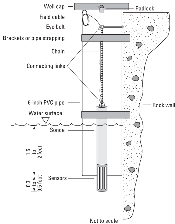
Figure 3. Delaware River and Araitan Canal feeder at Raven Rock, New Jersey, and schematic of internal-logging water-quality monitoring sensor and recording system.
