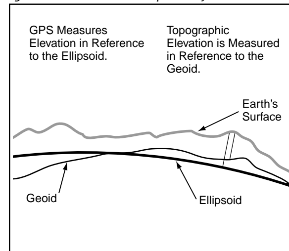
Figure GPS-P-3: Geoid and Ellipsoid Surfaces
