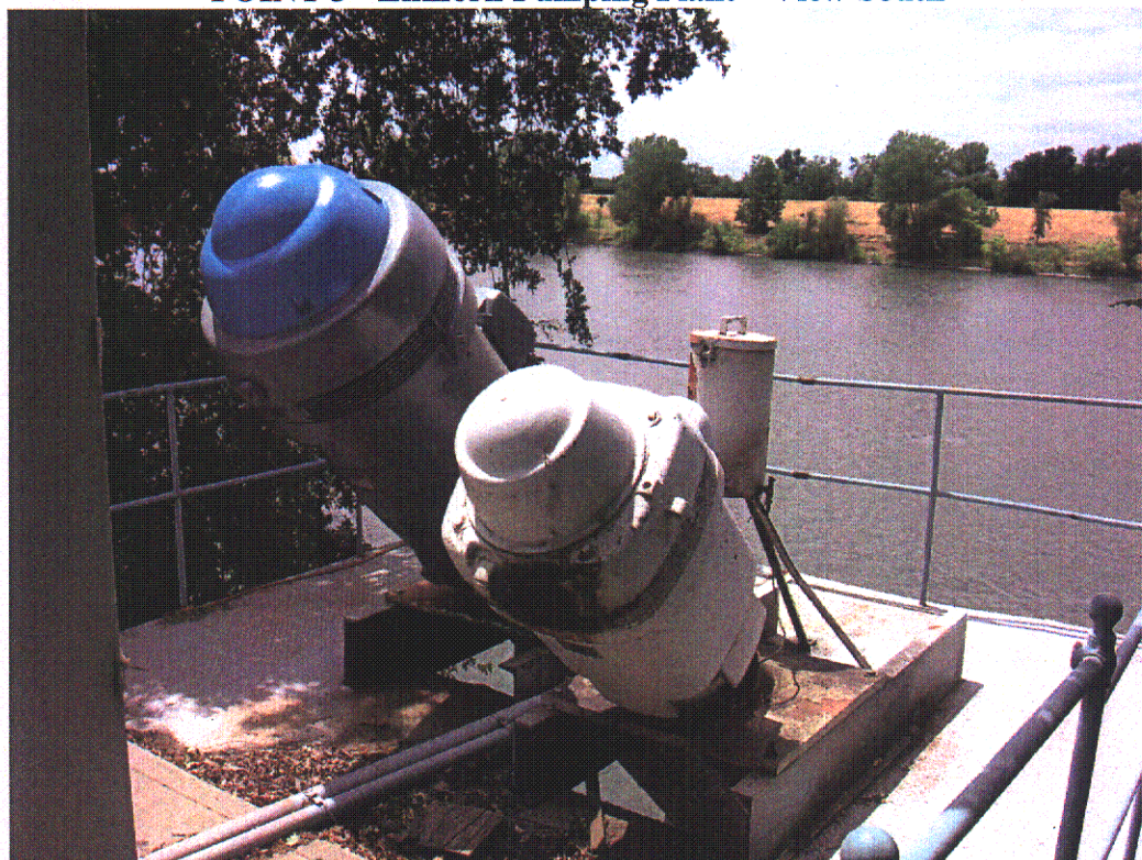
POINT 6 - Riverside Pumping Plant (Sacramento River)
