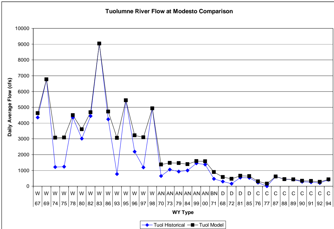
Figure 60. Tuolumne Flow—Model Scenario 11 Additional Water vs Historical.
