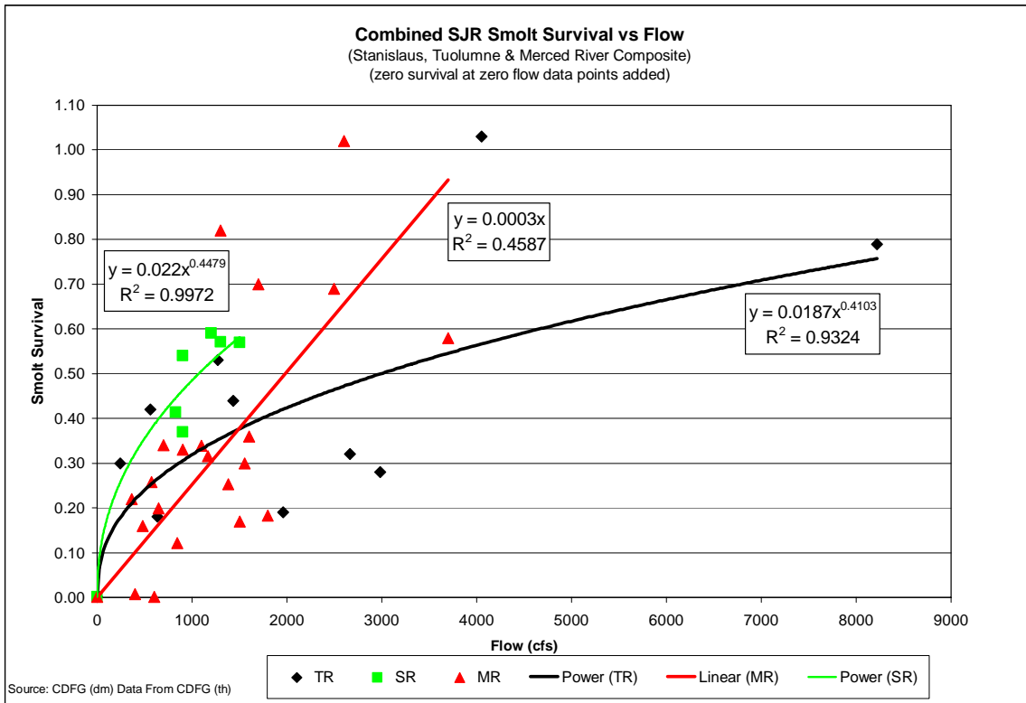
Figure 40. SJR East-side Tributary Smolt Survival Versus Flow.
