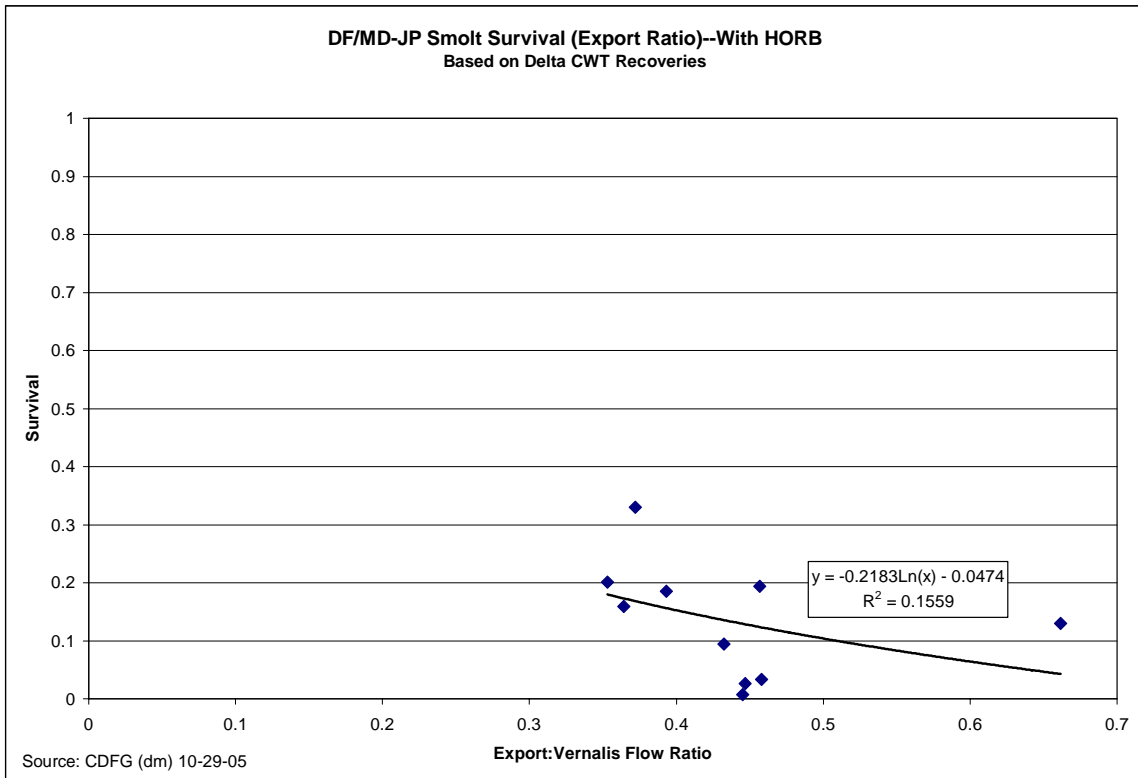
Figure 20. Smolt Survival and Export Ratio.
