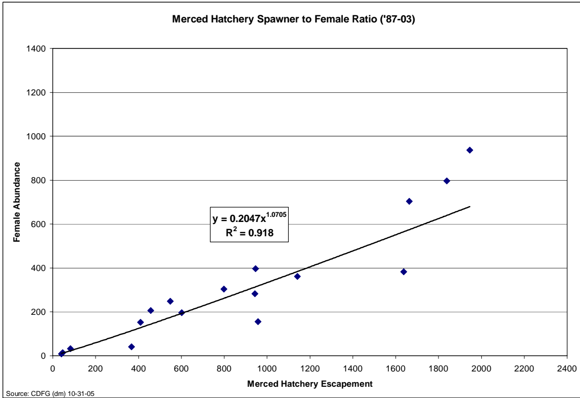
Figure 39. Merced Hatchery Escapement to Female Escapement.
