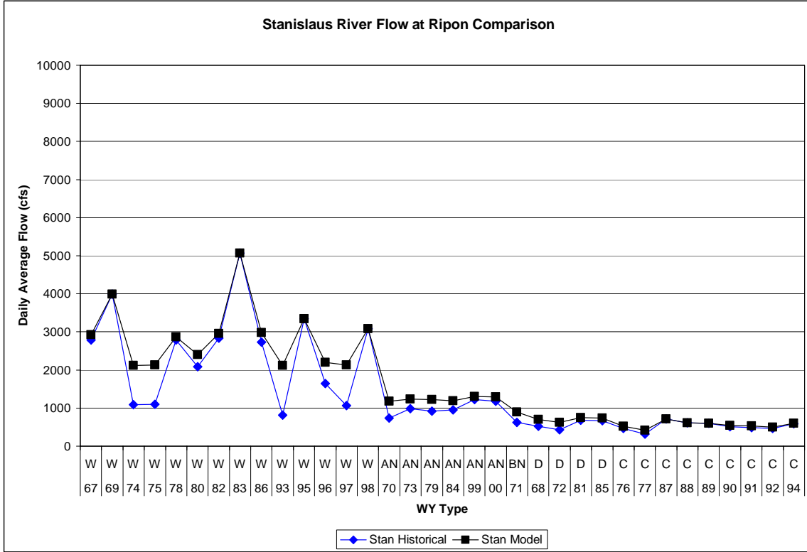
Figure 59. Stanislaus Flow—Model Scenario 11 Additional Water vs Historical.
