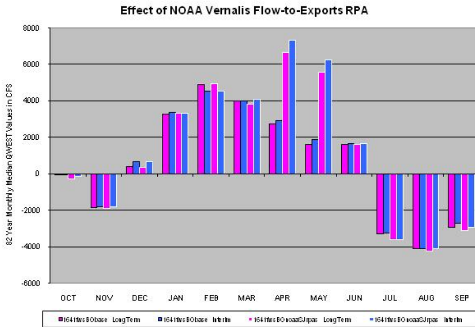
Figure 44: Response of QWEST to the implementation of the Vernalis RPA.
