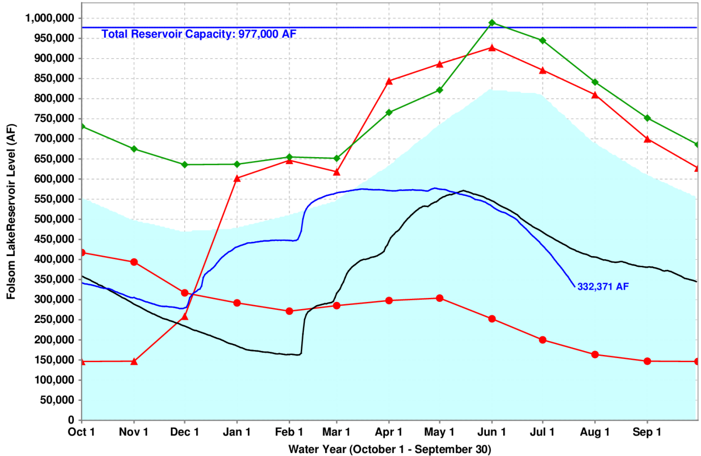
Folsom Lake Levels: Various Past Water Years and Current Water Year, Ending At Midnight July 20, 2015
