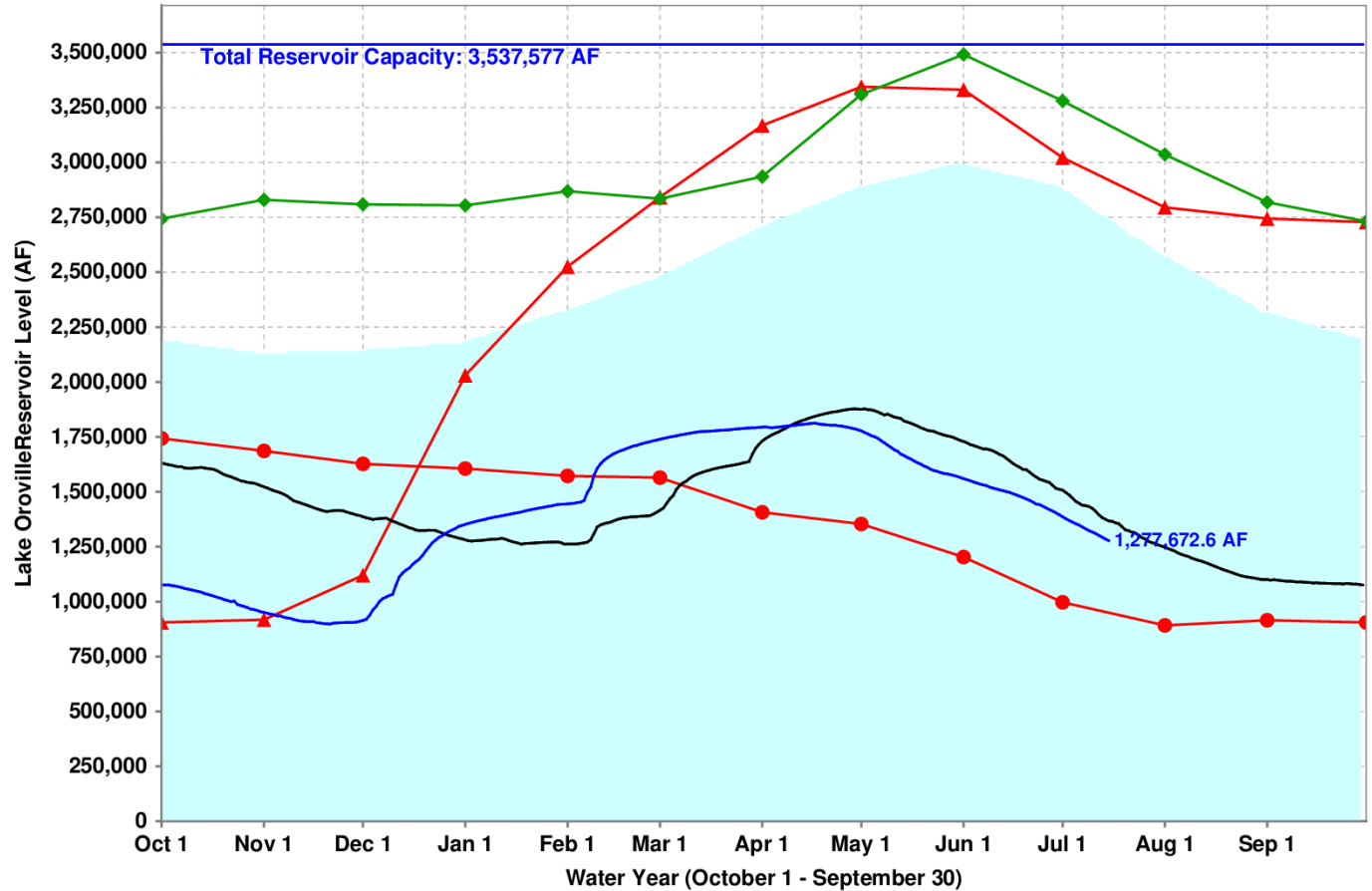
Lake Oroville Levels: Various Past Water Years and Current Water Year, Ending At Midnight July 15, 2015
