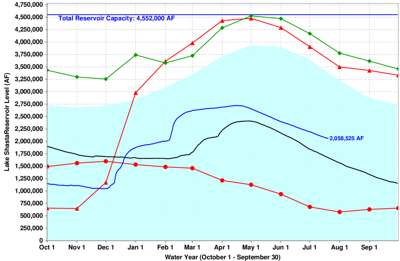
Lake Shasta Levels: Various Past Water Years and Current Water Year, Ending At Midnight July 20, 2015
