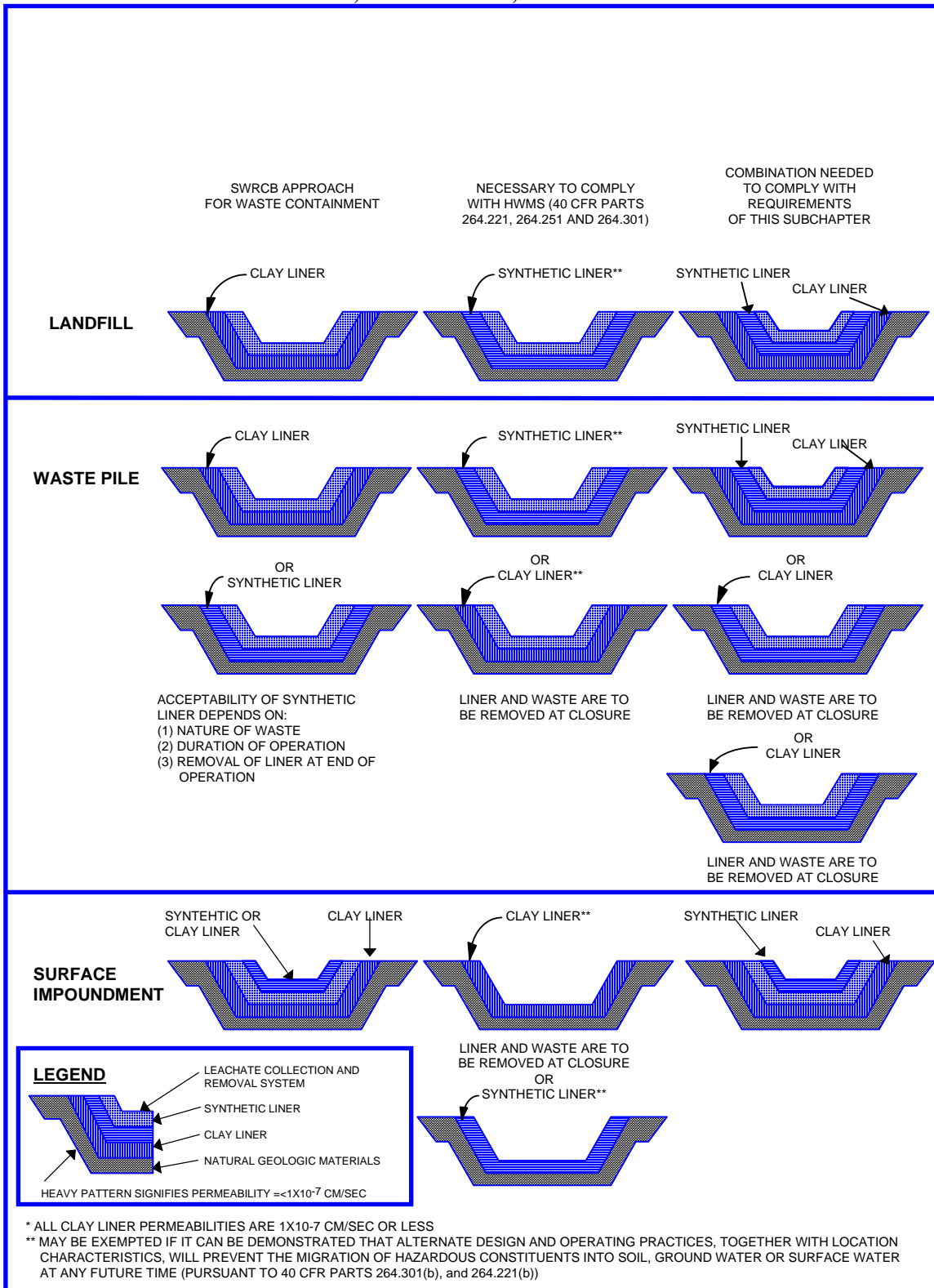
FIGURE 4.1 CLAY & SYNTHETIC LINER REQUIREMENTS FOR CLASS I LANDFILLS, WASTE PILES, & SURFACE IMPOUNDMENTS
