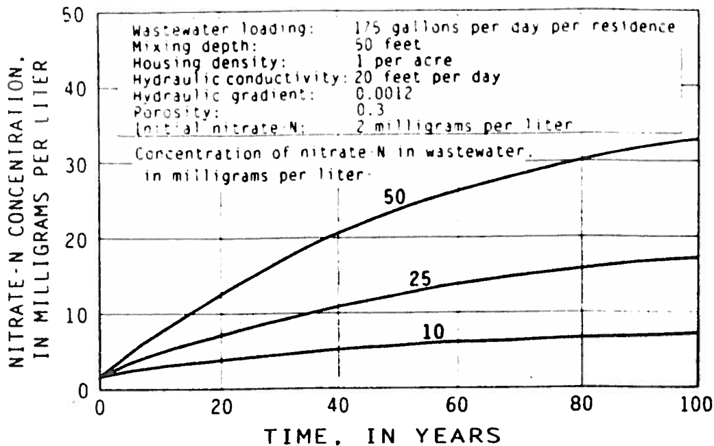
Figure 2. Model-computed nitrate concentrations in ground water in the study area for selected nitrate-N concentrations in wastewater.
