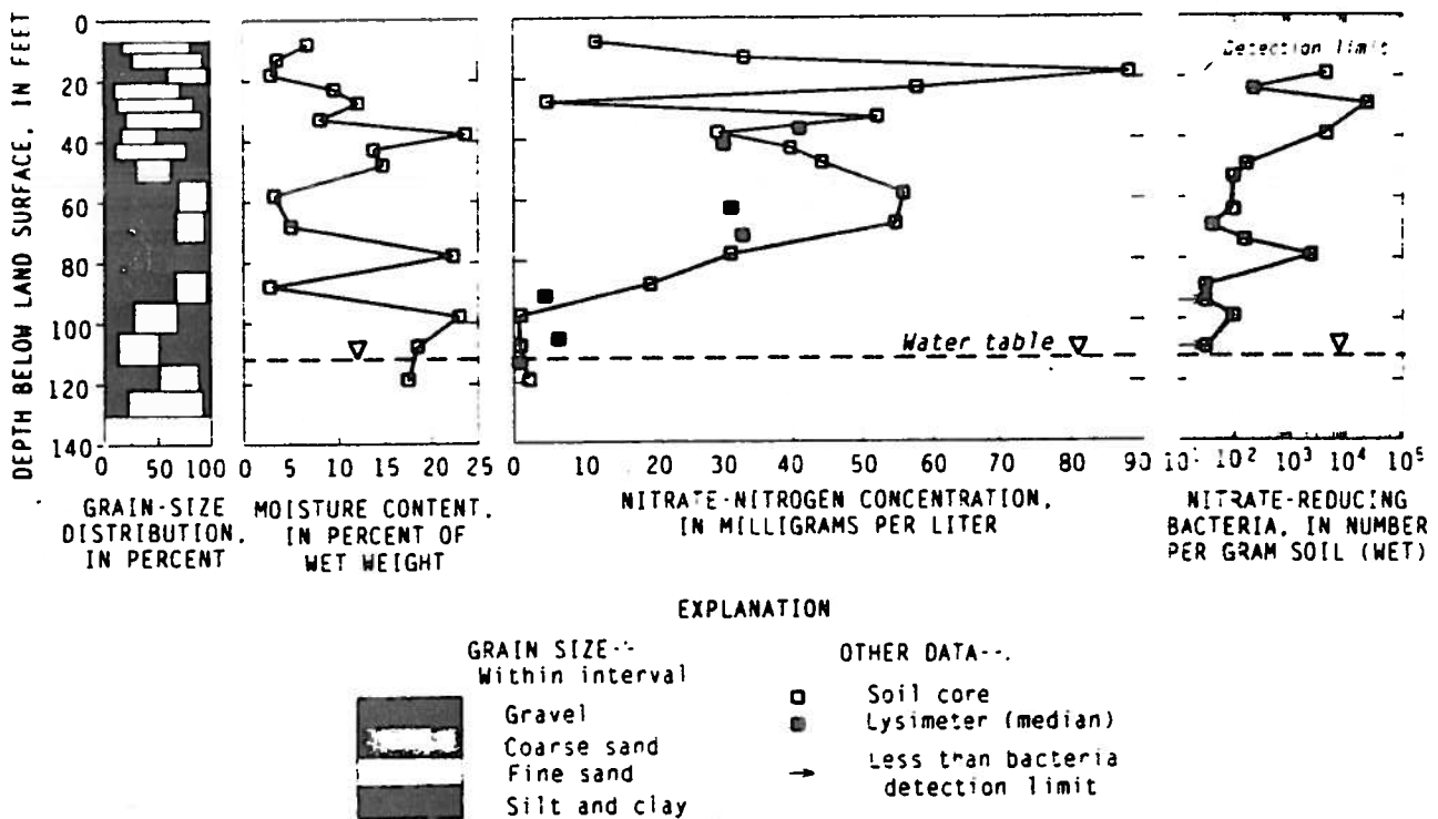
Figure 4. Grain-size distribution, moisture content, nitrate concentration, and nitrate-reducing bacteria counts at the Cheyenne-I site.
