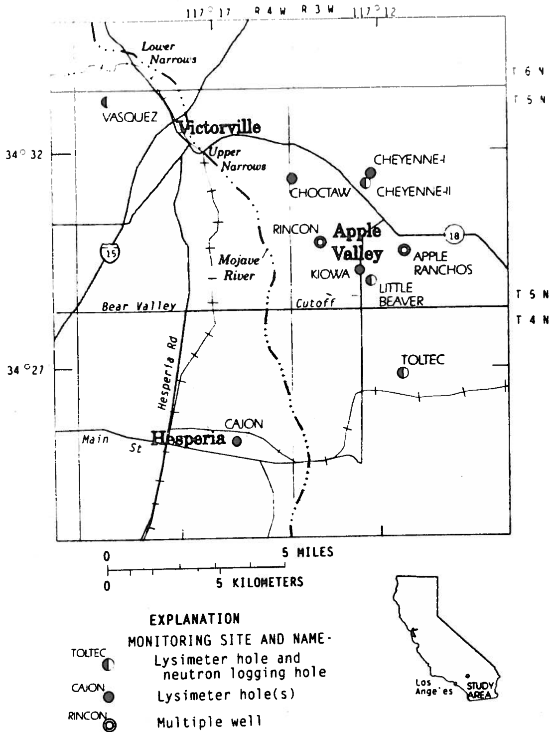
Figure 1. Location of study area and monitoring sites in the upper Mojave River Basin.
