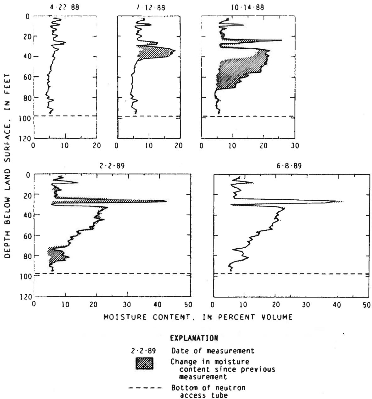
Figure 3. Temporal variation in soil-moisture content in the unsaturated zone at the Tollec site. Shaded areas indicate moisture additions in succeeding time intervals and record the downward movement of the wastewater wetting front.
