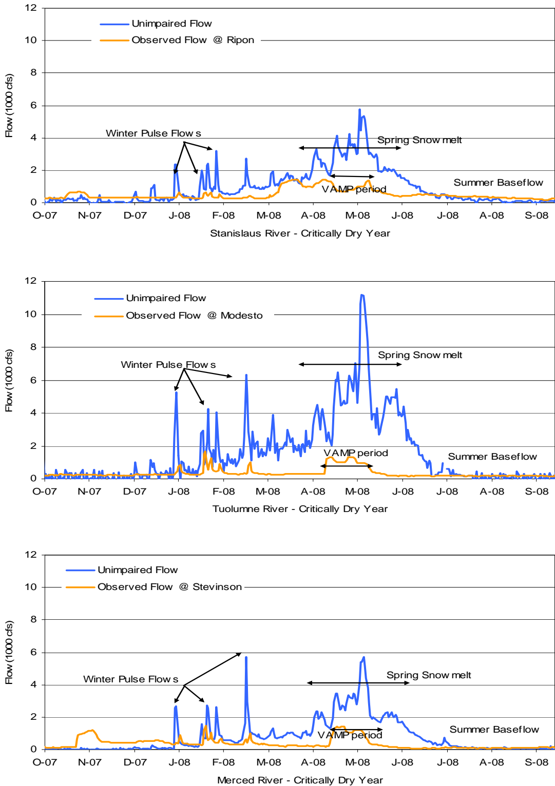
Figure 2.7. Daily Unimpaired Flow and Observed Flow for a Critically Dry Water Year (WY 2008) in the Stanislaus At Ripon (Top), Tuolumne at Modesto (Middle), and Merced at Stevenson (Bottom)
