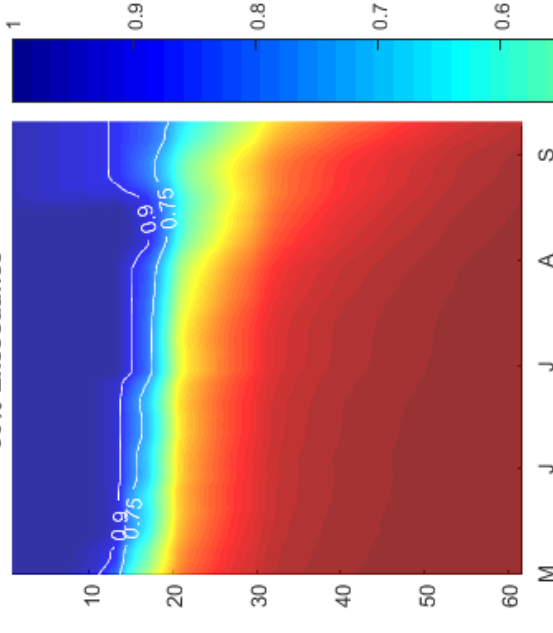
Survival using 90% CI of Survival Parameters, 90% Exceedance
