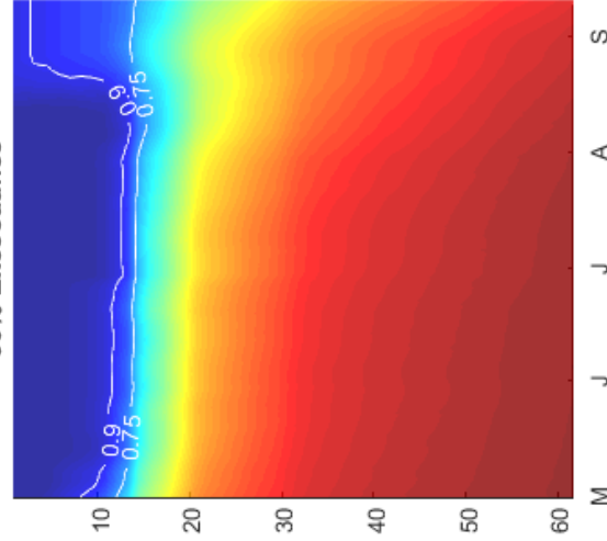
Survival using Median Survival Parameters, 90% Exceedance
