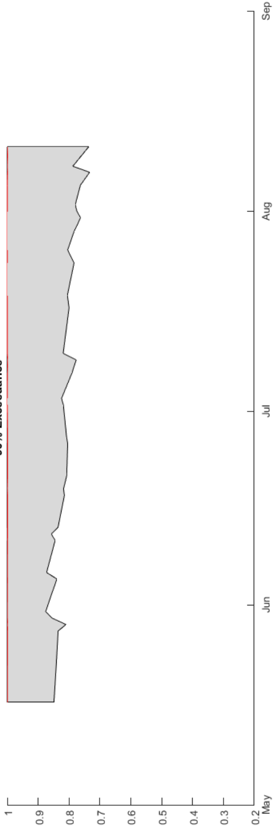
Temperature-dependent Survival, 2012-2015 Redd Data 90% Exceedance
