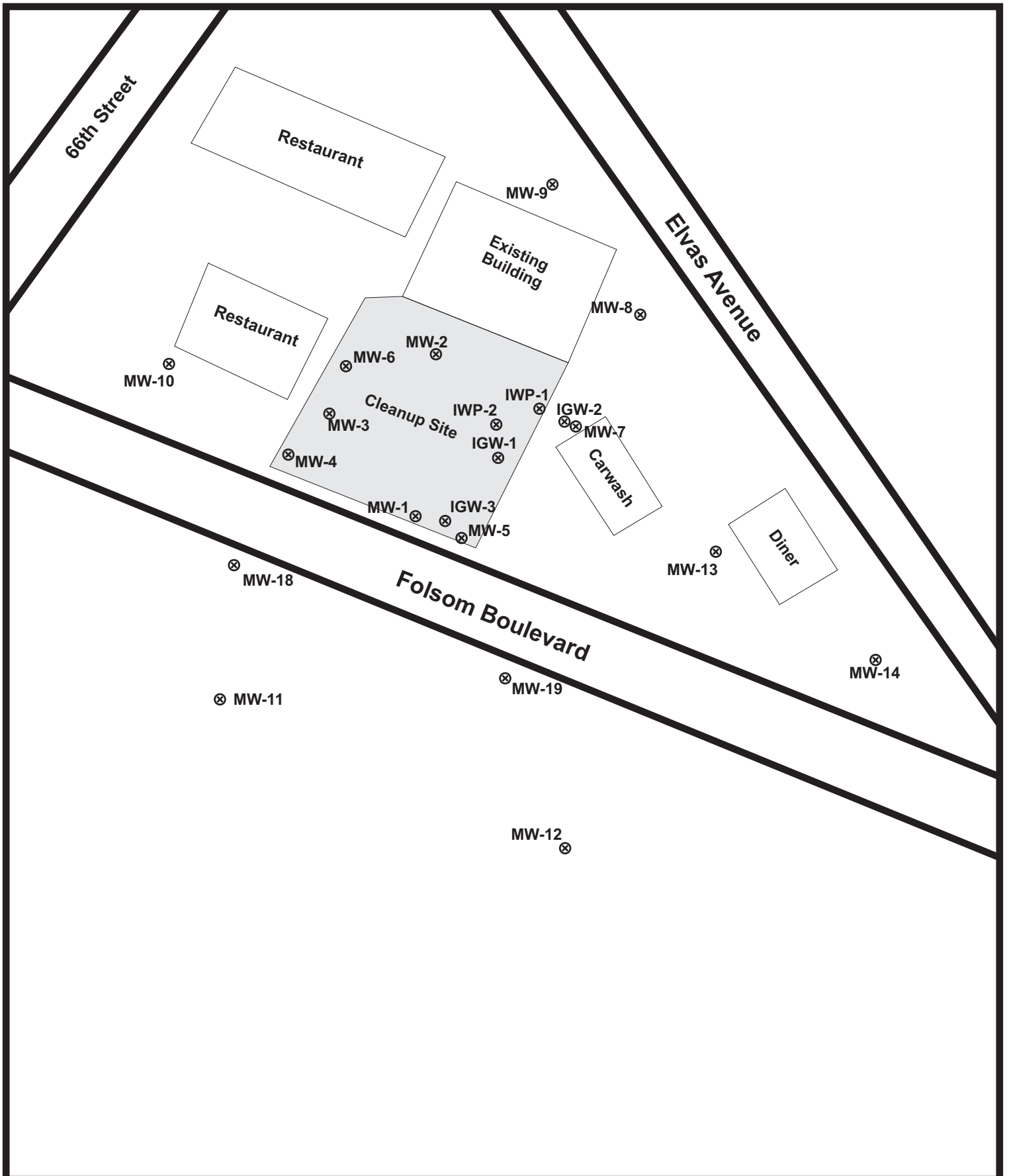
Former Eagle Service Station 6661 Folsom Blvd, Sacramento Site and Well Locations
