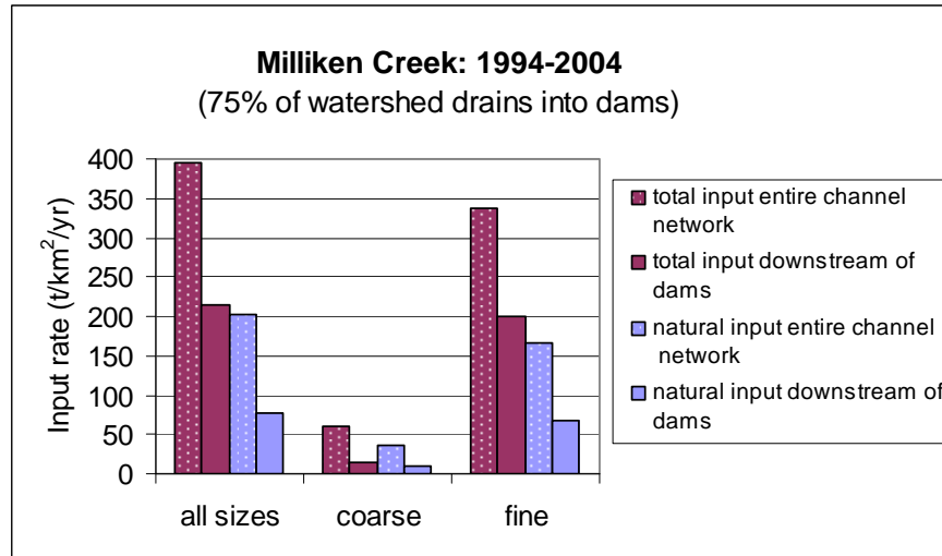
Figure 15: Sediment Input to Channels in Milliken Creek Watershed (1994-2004). Coarse corresponds to boulders, cobbles, and coarse gravels (e.g., 11.2-to-64 mm). Fine corresponds to fine gravel, sand, silt, and clay. Between 1994 and 2004, half of sediment input to channels was associated with land use activities. Dams captured about ¾ of coarse sediment input to channels and about ½ of the fine sediment input to channels. As such, total sediment delivery to channels located downstream of dams (all sizes) was approximately equal to natural background rate of sediment supply (e.g., absent dams and human caused erosion), albeit with a much smaller proportion of supply in the coarse size range.
