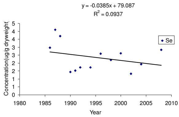
Trend of Se concentration at Santa Cruz Island
