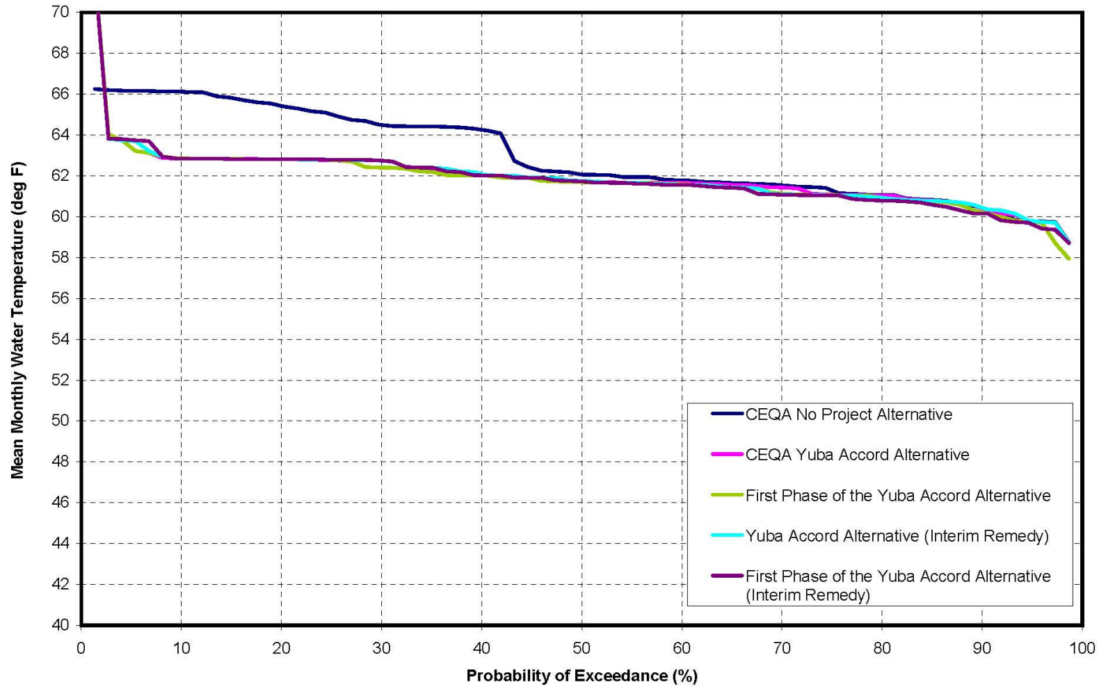
Simulated Mean Monthly Lower Yuba River Water Temperature at Marysville during September
