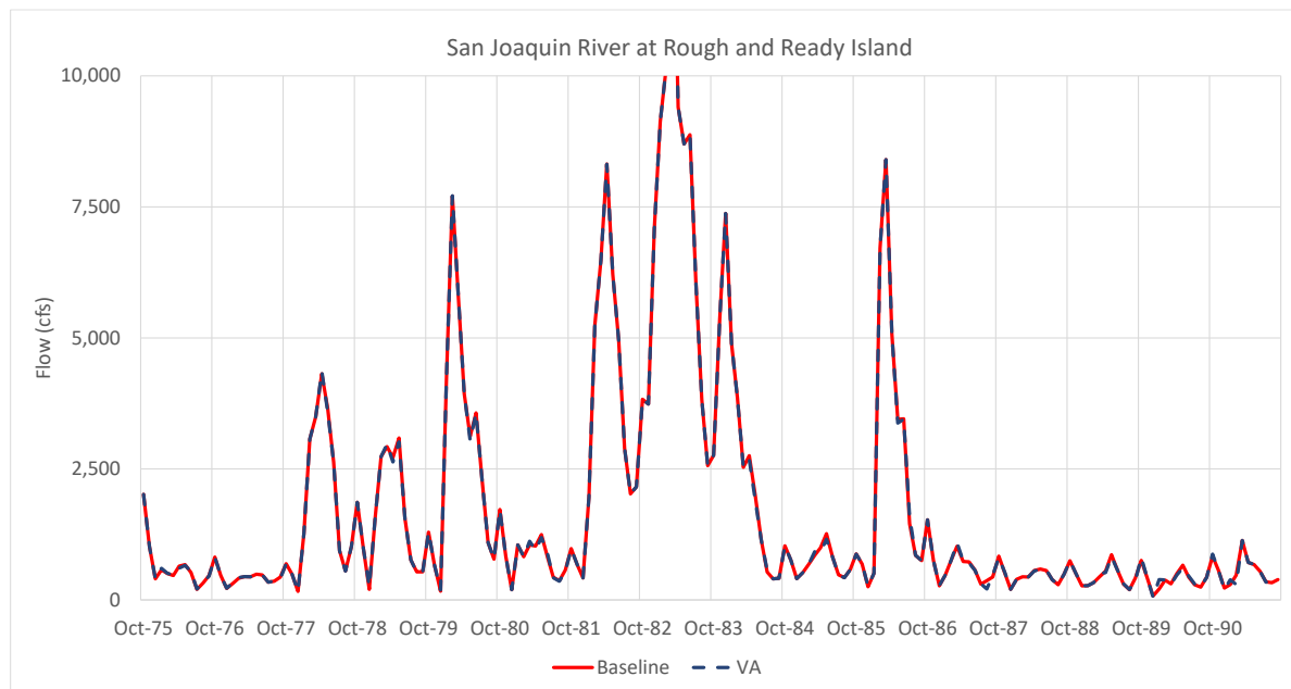
Figure G3b-6. DSM2 Flow in the San Joaquin River near Stockton – Baseline and the Proposed VAs for Water Years 1976–1991
