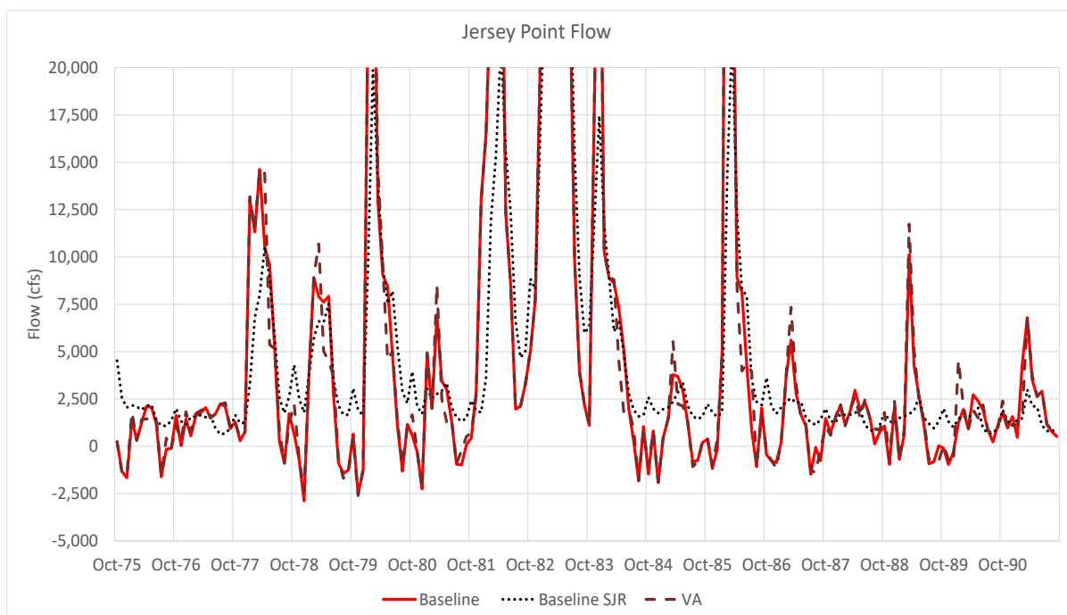
Figure G3b-4. San Joaquin River Flow at Jersey Point – Baseline and the Proposed VAs for Water Years 1976–1991
