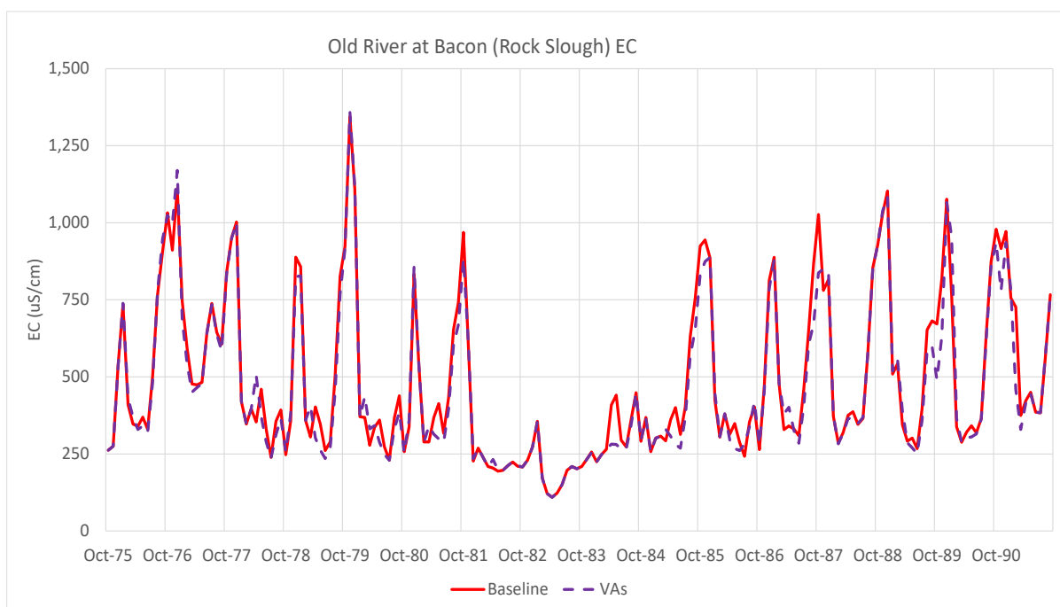
Figure G3b-16. Time Series of DSM2 EC Values for Old River at Bacon Island (CCWD Rock Slough Intake) – Baseline and the Proposed VAs for Water Years 1976–1991
