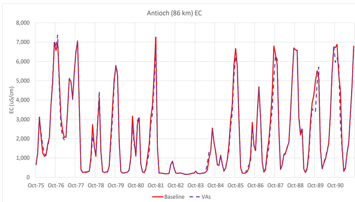
Figure G3b-15. Time Series of DSM2 EC Values for Antioch EC – Baseline and the Proposed VAs for Water Years 1976–1991
