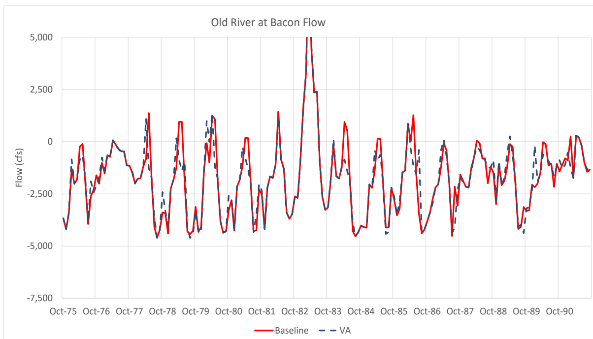
Figure G3b-5. DSM2 Flow in Old River at Bacon Island – Baseline and the Proposed VAs for Water Years 1976–1991
