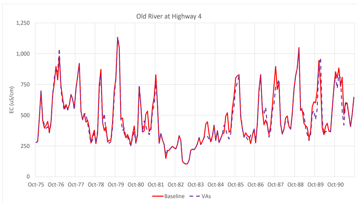
Figure G3b-17. Time Series of DSM2 EC Values for Old River at Highway 4 (CCWD Old River Intake) – Baseline Compared with the Proposed VAs for Water Years 1976–1991
