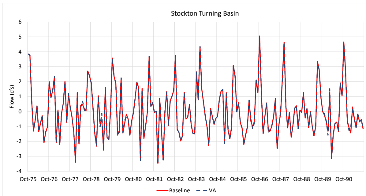
Figure G3b-7. DSM2 Flow in the Port of Stockton Turning Basin – Baseline and the Proposed VAs for Water Years 1976–1991
