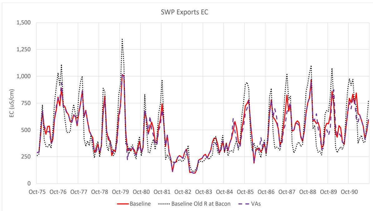
Figure G3b-19. Time Series of DSM2 EC Values for SWP Exports – Baseline and the Proposed VAs for Water Years 1976–1991 with Baseline Old River at Bacon Island EC for Reference
