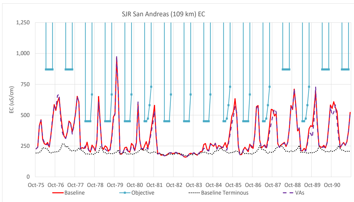
Figure G3b-14. Time Series of DSM2 EC Values for San Andreas Landing – Baseline and the Proposed VAs for Water Years 1976–1991 with EC Objectives for Reference
