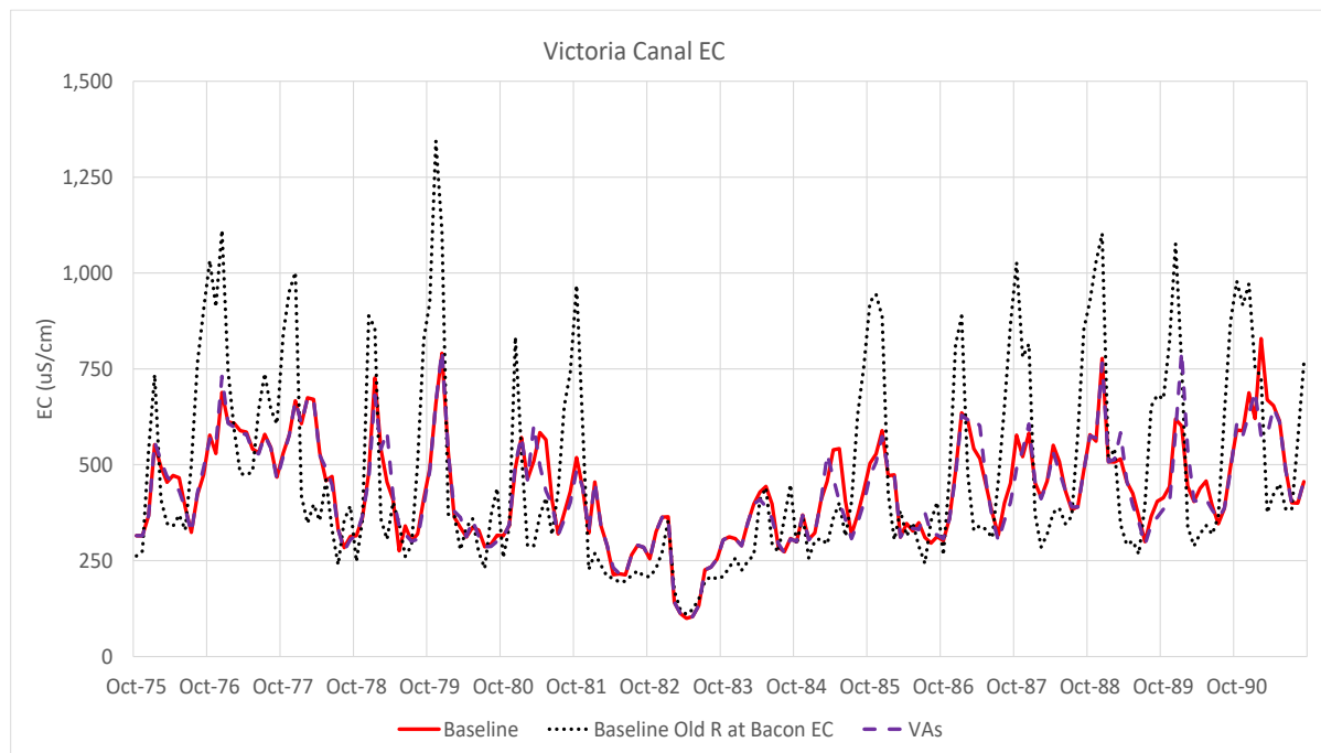
Figure G3b-18. Time Series of DSM2 EC Values for Victoria Canal EC (CCWD Middle River Intake) for Baseline and for the Proposed VAs for Water Years 1976–1991
