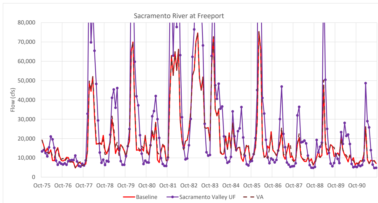
Figure G3b-1. SacWAM Sacramento River Flow at Freeport – Baseline and Proposed VAs for Water Years 1976–1991
