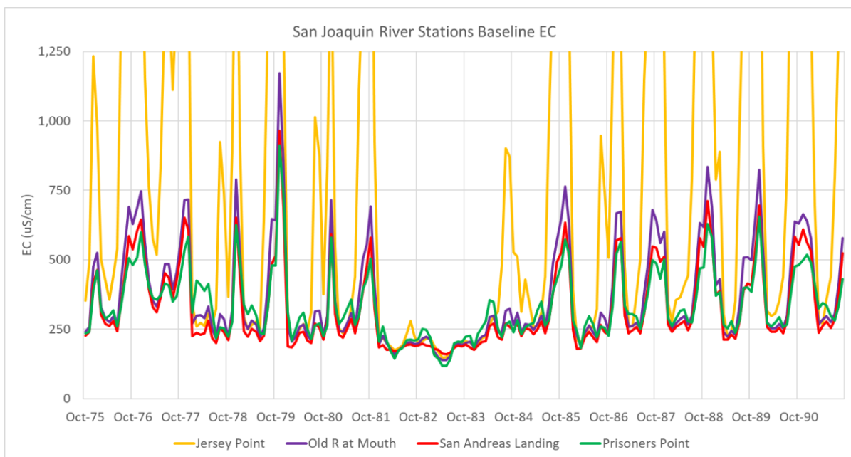
Figure G3b-22. Time Series of DSM2 Baseline EC Values for San Joaquin River Stations for Water Years 1976–1991
