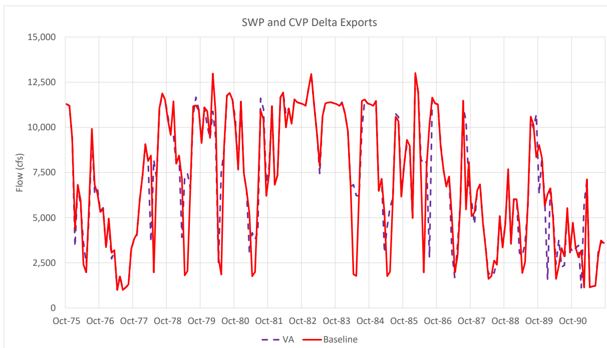
Figure G3b-3. SacWAM CVP and SWP Delta Exports – Baseline and the Proposed VAs for Water Years 1976–1991
