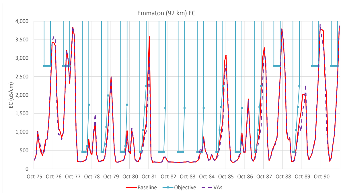
Figure G3b-13. Time Series of DSM2 EC Values for Emmatton – Baseline and the Proposed VAs for Water Years 1976–1991 with EC Objectives for Reference
