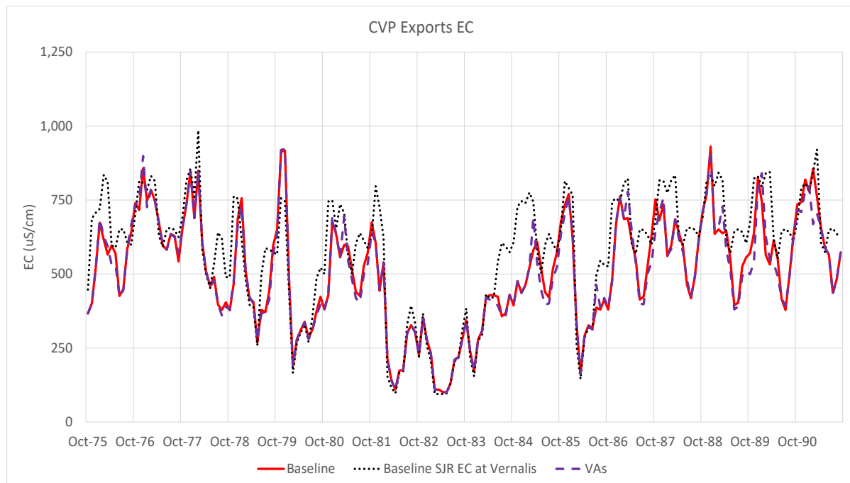
Figure G3b-20. Time Series of DSM2 EC Values for CVP Exports – Baseline and the Proposed VAs for Water Years 1976–1991 with Baseline San Joaquin River EC for Reference
