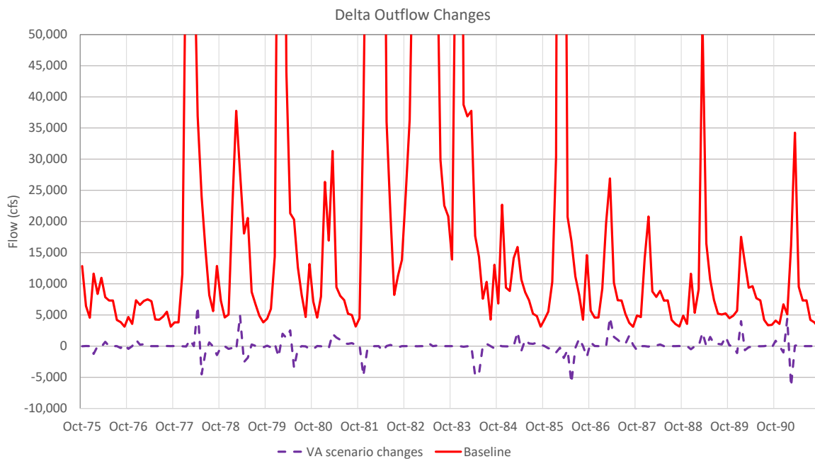
Figure G3b-2. Delta Outflow – Baseline and Changes from Baseline for the Proposed VAs for Water Years 1976–1991
