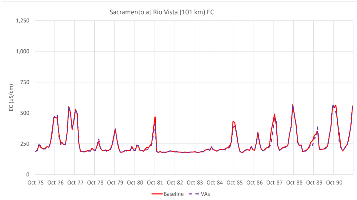
Figure G3b-21. Time Series of DSM2 EC Values for the Sacramento River at Rio Vista – Baseline and the Proposed VAs for Water Years 1976–1991
