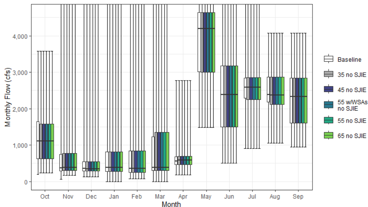
Figure H1a5-38. Trinity River Streamflow below Lewiston Reservoir Monthly Boxplot (cfs)
