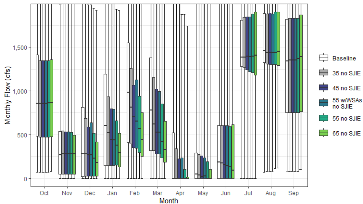
Figure H1a5-64. Spring Creek Conduit Monthly Boxplot (cfs)
