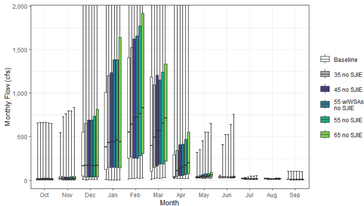
Figure H1a5-10. Cache Creek Streamflow above Yolo Bypass Monthly Boxplot (cfs)
