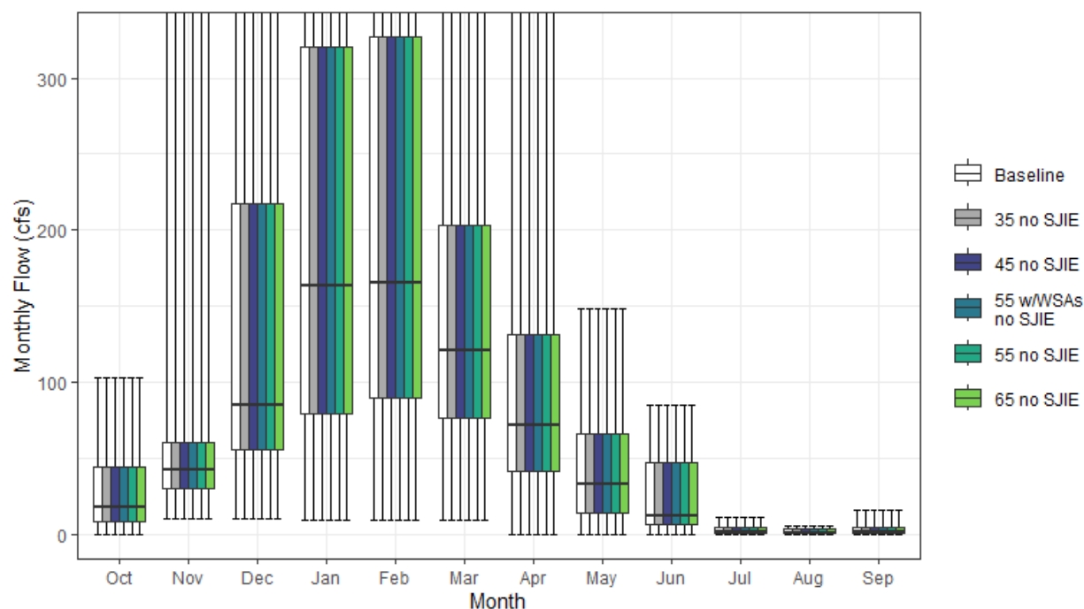
Figure H1a5-25. Paynes Creek Streamflow above Confluence with Sacramento River Monthly Boxplot (cfs)
