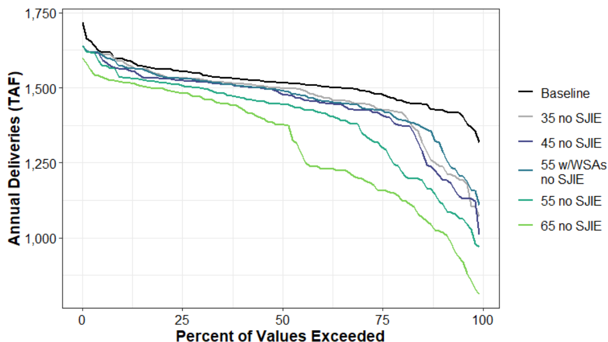
Figure H1a5-168. Total Water Supplied to Water Budget Area 8 (Agricultural) Annual Percent Exceedance Plot.
