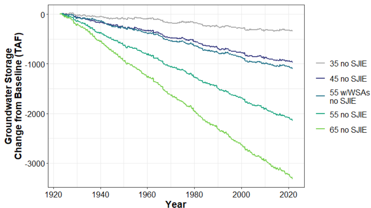
Figure H1a5-242. American River Groundwater Basin End of Year Storage—Change from Baseline (TAF)
