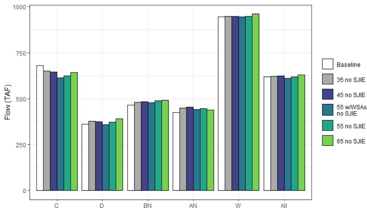
Figure H1a5-238. Total Average Annual Stream-Groundwater Flux (Net Groundwater Gain) by WYT and Scenario (TAF/yr).
