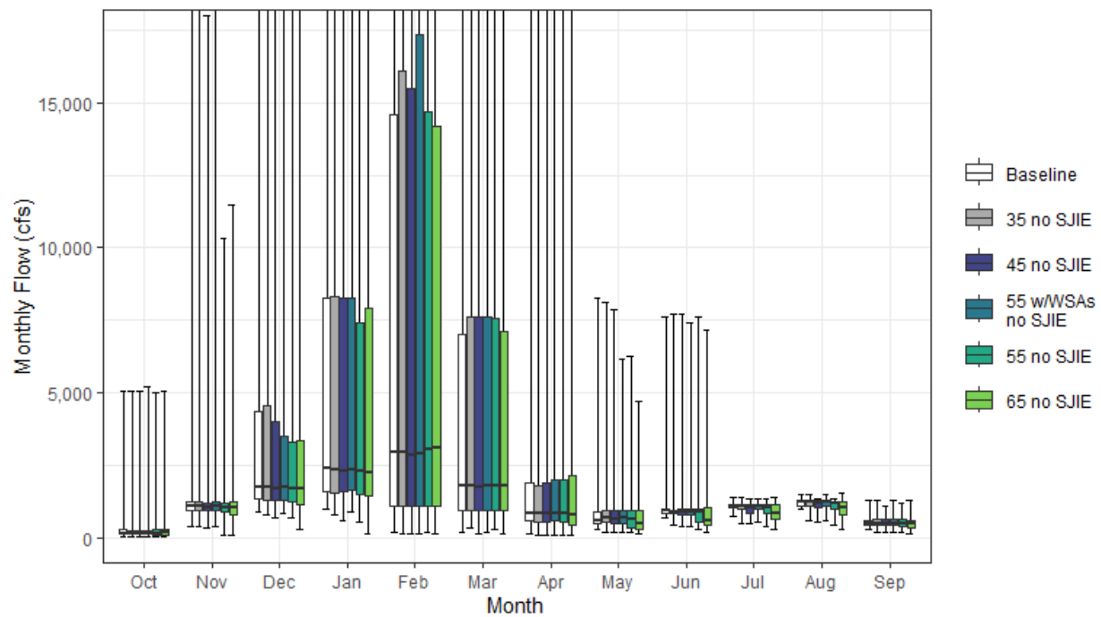
Figure H1a5-36. Sutter Bypass Streamflow near Karnak Monthly Boxplot (cfs)
