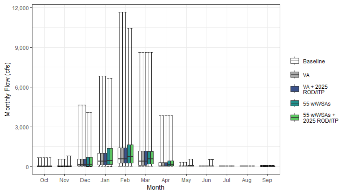
Figure H1a6-10. Monthly Streamflow for Cache Creek above the Yolo Bypass under Baseline, Voluntary Agreement Pathway, and Regulatory Pathway Agreement Pathway
