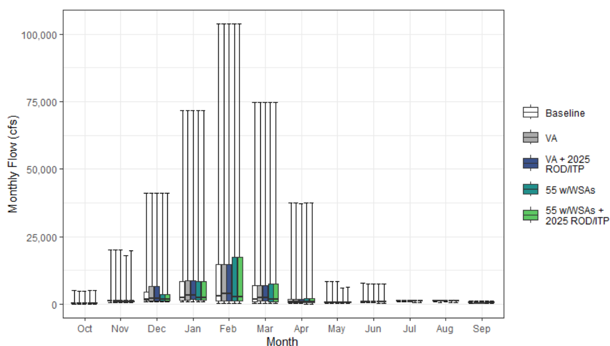
Figure H1a6-17. Monthly Streamflow at Sacramento Slough (downstream end of Sutter Bypass) under Baseline, Voluntary Agreement Pathway, and Regulatory Pathway Agreement Pathway
