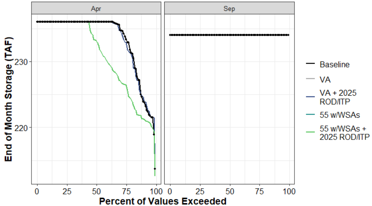
Figure H1a6-36. Whiskeytown Reservoir End-of-April and End-of-September Storage under Baseline, Regulatory Pathway, and Voluntary Agreement Pathway
