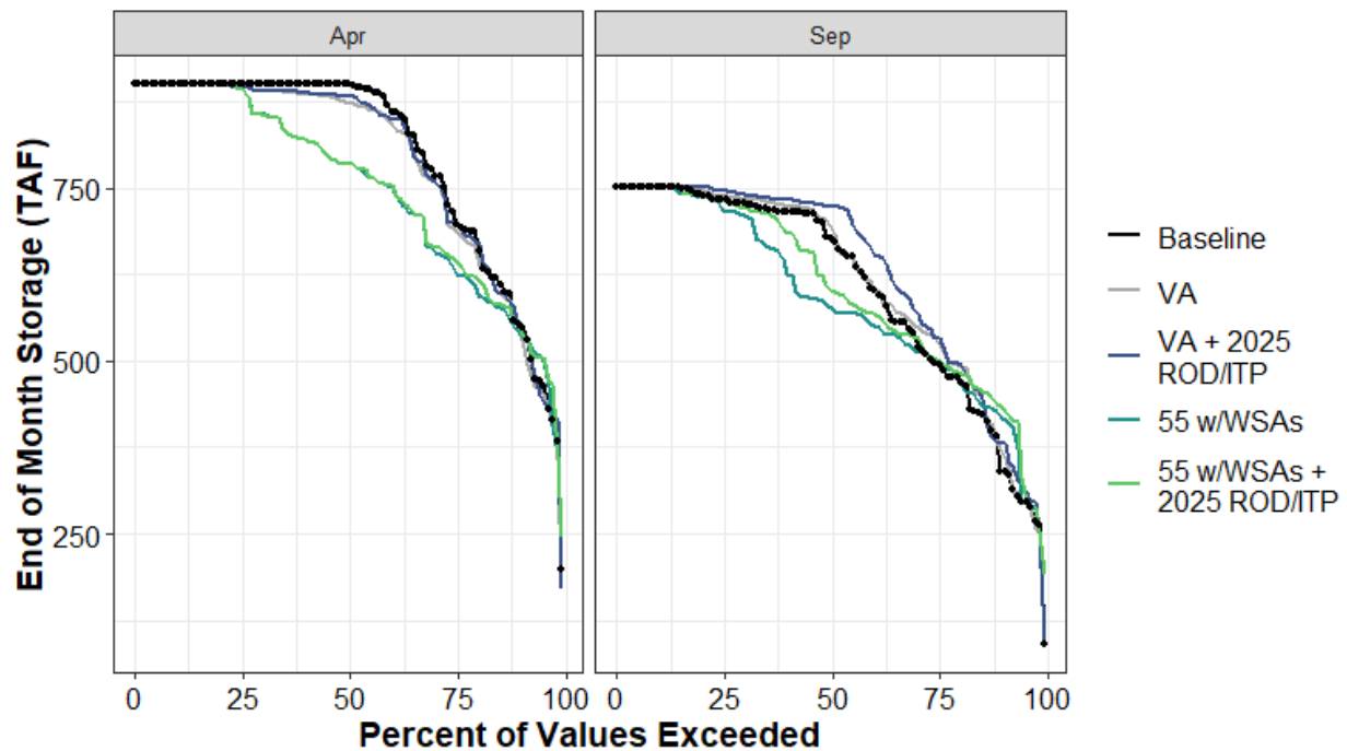
Figure H1a6-29. Folsom Lake End-of-April and End-of-September Storage under Baseline, Regulatory Pathway, and Voluntary Agreement Pathway
