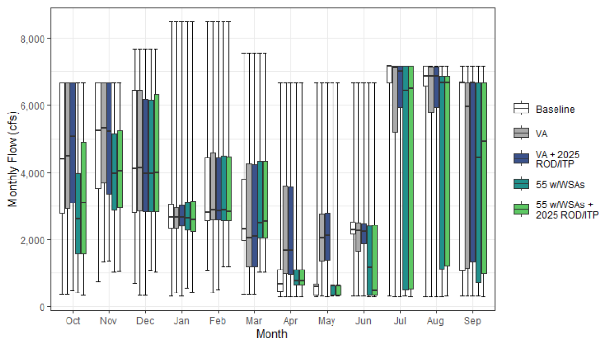
Figure H1a6-20. Monthly SWP Exports for Baseline, Regulatory Pathway, and Voluntary Agreement Pathway
