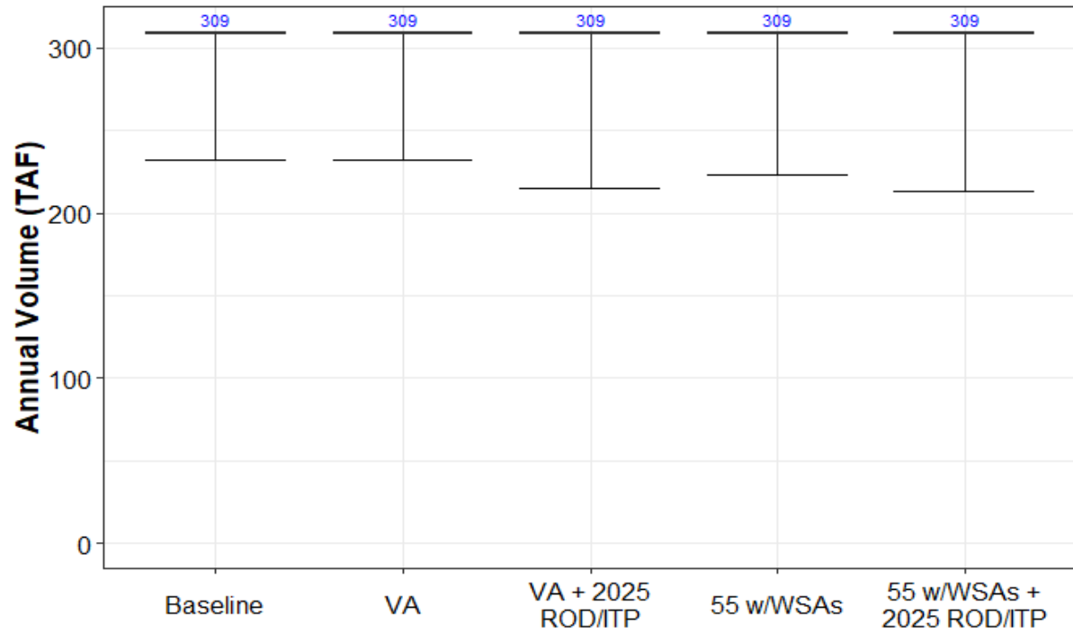
Figure H1a6-49. Annual Sacramento/Delta Supply to Wildlife Refuges in the San Joaquin Valley Region for Baseline, VA Pathway, and Regulatory Pathway Scenarios
