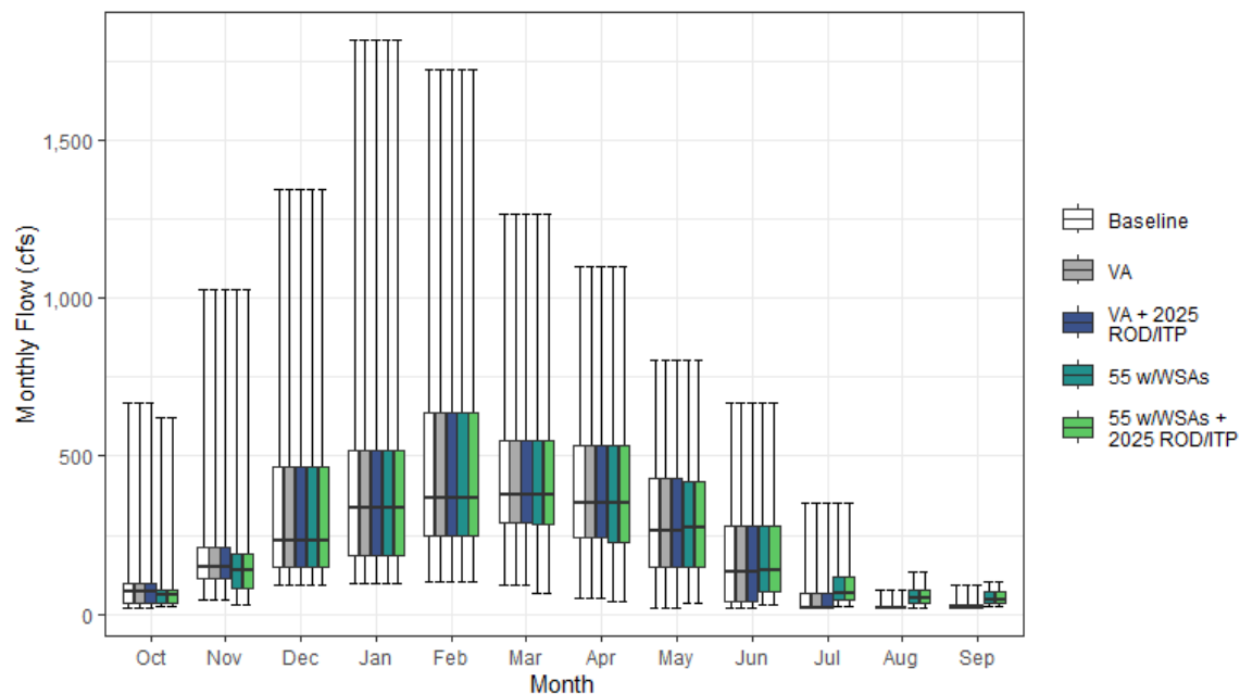
Figure H1a6-12. Monthly Streamflow for Mill Creek under Baseline, Voluntary Agreement Pathway, and Regulatory Pathway Agreement Pathway
