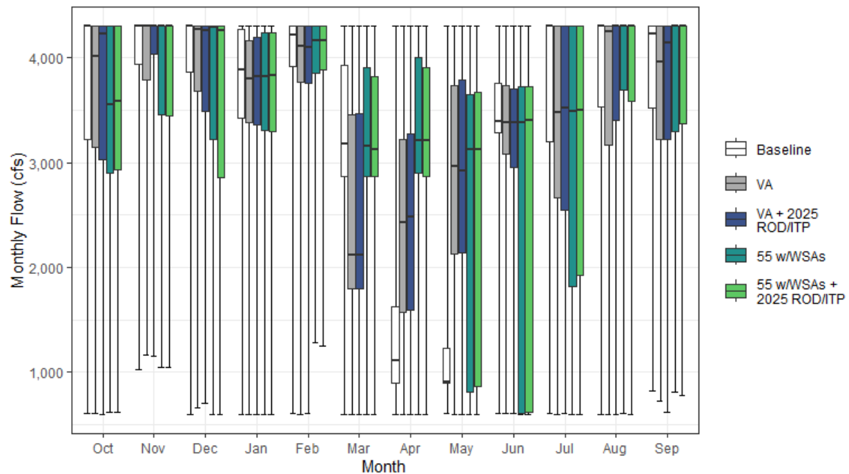
Figure H1a6-21. Monthly CVP Exports for Baseline, Regulatory Pathway, and Voluntary Agreement Pathway
