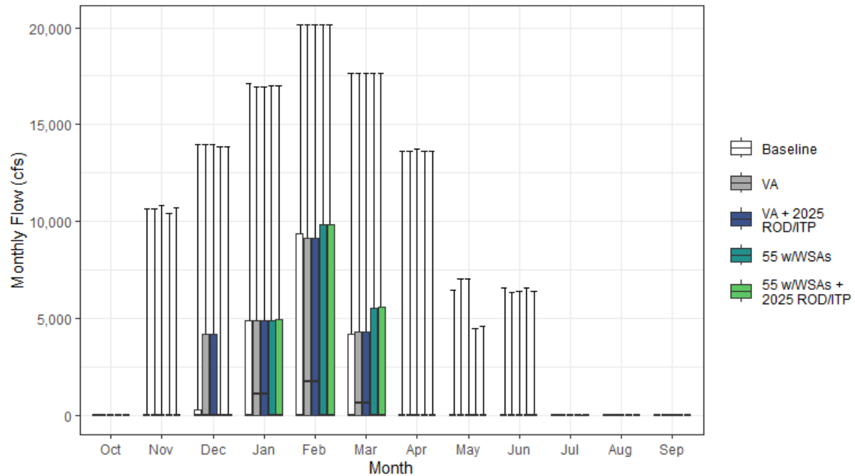
Figure H1a6-16. Monthly Streamflow over the Tisdale Weir into the Sutter Bypass under Baseline, Voluntary Agreement Pathway, and Regulatory Pathway Agreement Pathway
