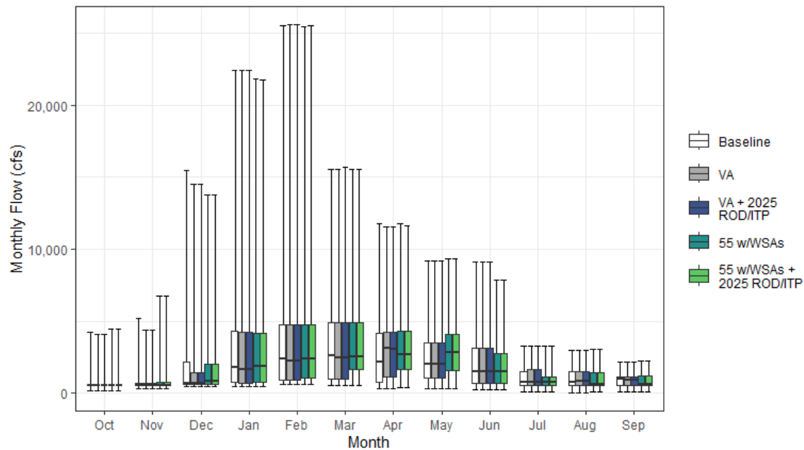
Figure H1a6-5. Monthly Streamflow for the Yuba River above the Feather River under Baseline, Voluntary Agreement Pathway, and Regulatory Pathway Agreement Pathway
