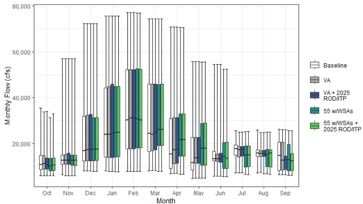
Figure H1a6-4. Monthly Streamflow for the Sacramento River at Freeport under Baseline, Voluntary Agreement Pathway, and Regulatory Pathway Agreement Pathway
