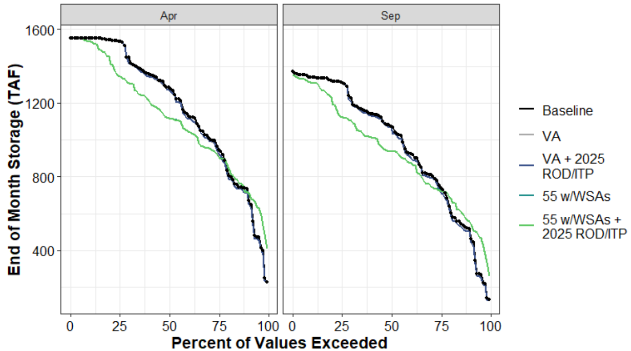
Figure H1a6-30. Lake Berryessa End-of-April and End-of-September Storage under Baseline, Regulatory Pathway, and Voluntary Agreement Pathway
