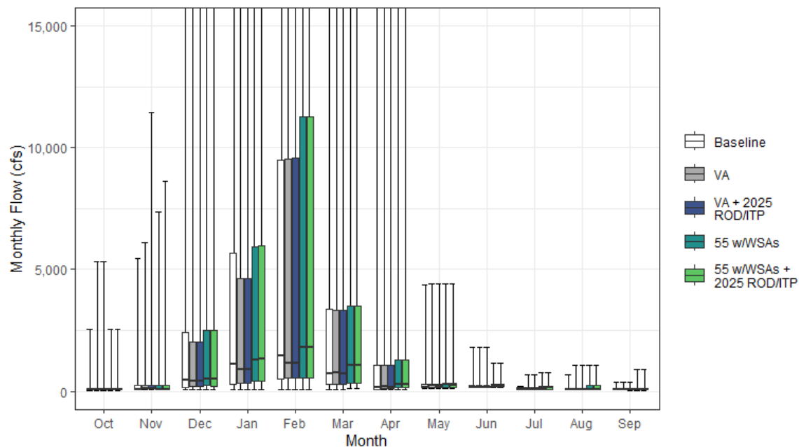
Figure H1a6-15. Monthly Streamflow for the Yolo Bypass below Putah Creek Inflow under Baseline, Voluntary Agreement Pathway, and Regulatory Pathway Agreement Pathway
