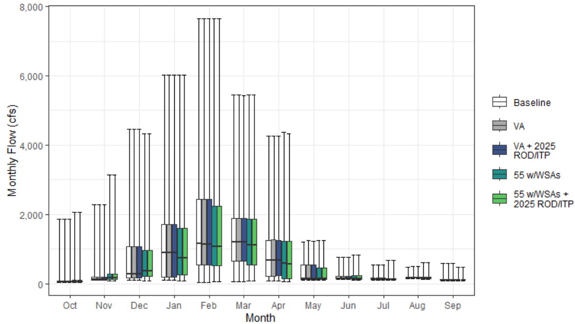
Figure H1a6-6. Monthly Streamflow for the Bear River above the Feather River under Baseline, Voluntary Agreement Pathway, and Regulatory Pathway Agreement Pathway
