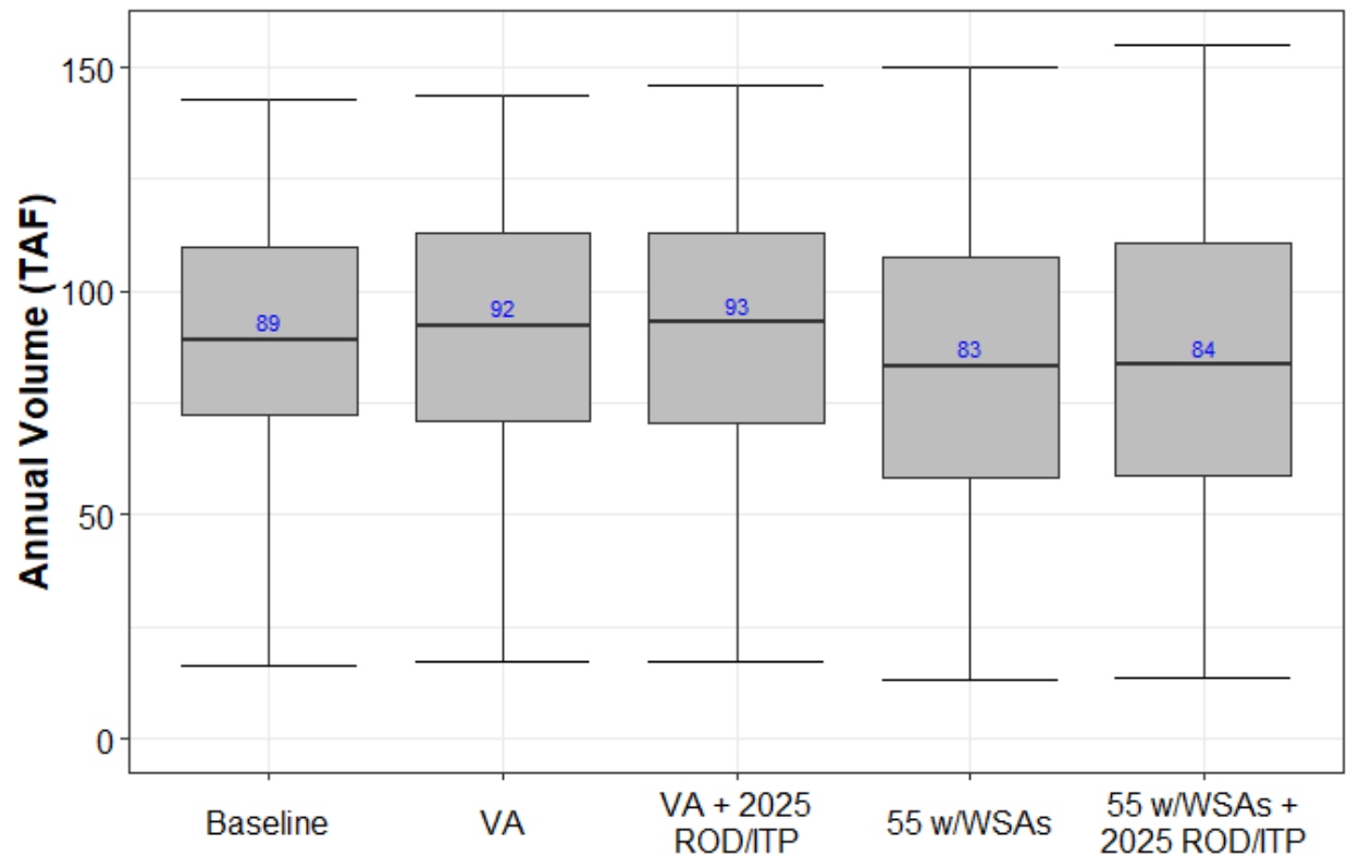
Figure H1a6-51. Annual Total Sacramento/Delta Supply to the Central Coast Region for Baseline, VA Pathway, and Regulatory Pathway Scenarios
