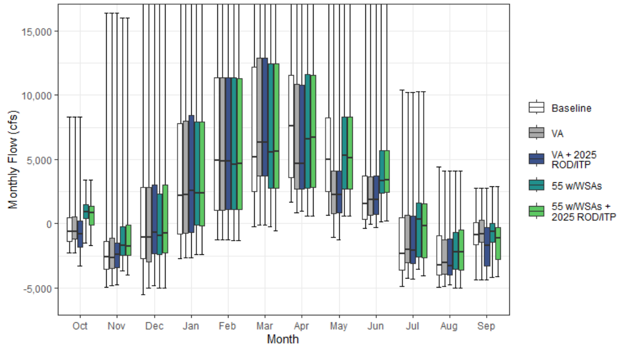
Figure H1a6-23. Monthly Distributions of QWEST under Baseline, Regulatory Pathway, and Voluntary Agreement Pathway
