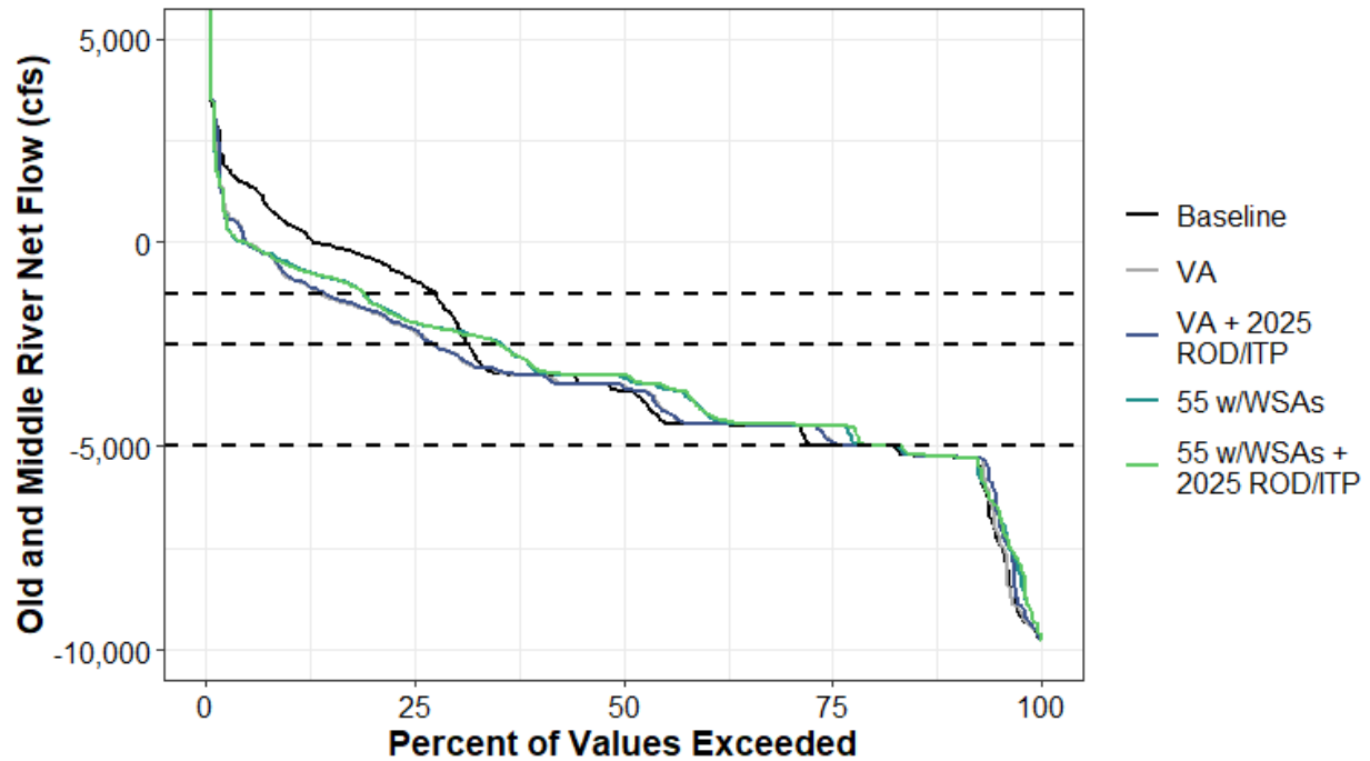
Figure H1a6-22. Monthly Exceedance Frequency Distribution of Old and Middle River Net Flow for December–June under Baseline, Regulatory Pathway, and Voluntary Agreement Pathway
