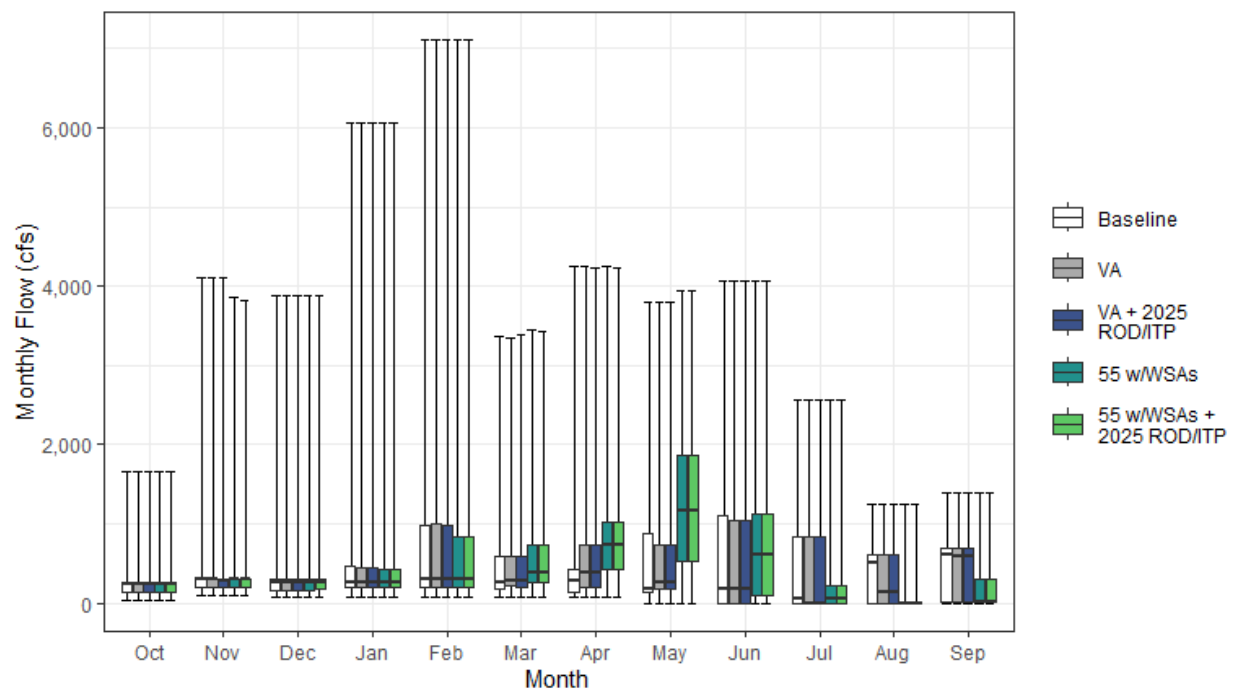
Figure H1a6-7. Monthly Streamflow for the Mokelumne River above the Confluence with the Cosumnes River under Baseline, Voluntary Agreement Pathway, and Regulatory Pathway Agreement Pathway
