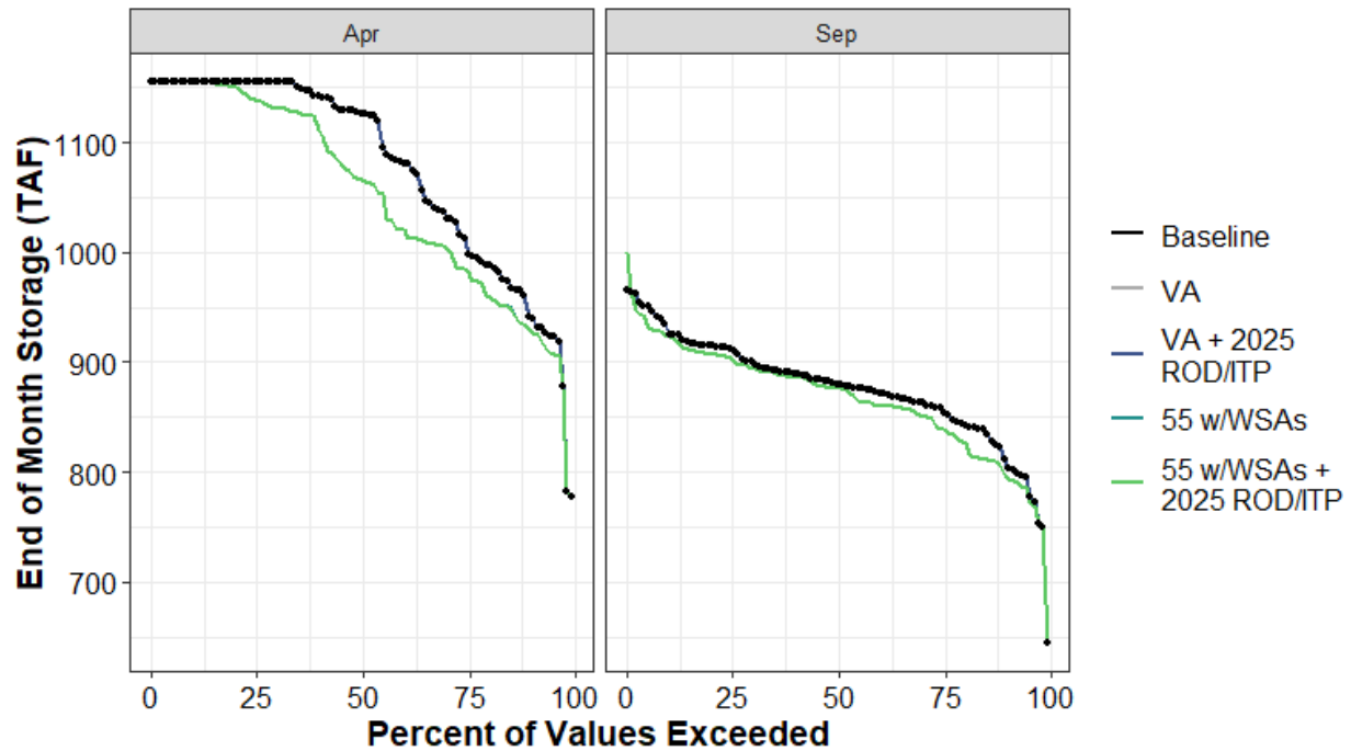
Figure H1a6-28. Clear Lake End-of-April and End-of-September Storage under Baseline, Regulatory Pathway, and Voluntary Agreement Pathway
