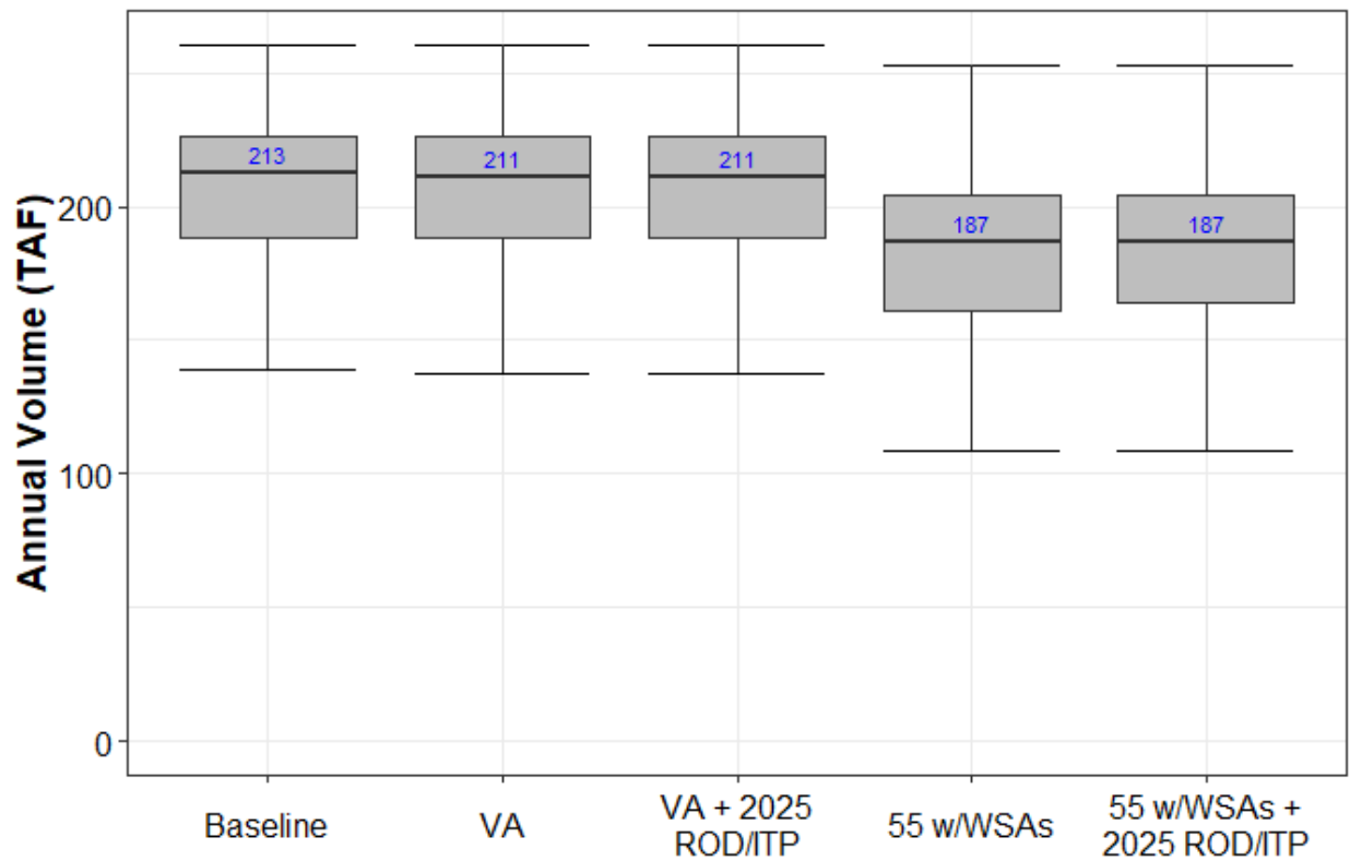
Figure H1a6-42. Annual Total Sacramento/Delta Supply to the Delta Eastside Tributaries Region for Baseline, VA Pathway, and Regulatory Pathway Scenarios
