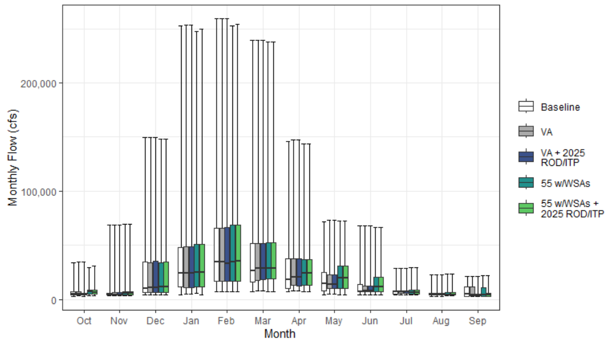
Figure H1a6-24. Monthly Delta Outflow for Baseline, Regulatory Pathway, and Voluntary Agreement Pathway
