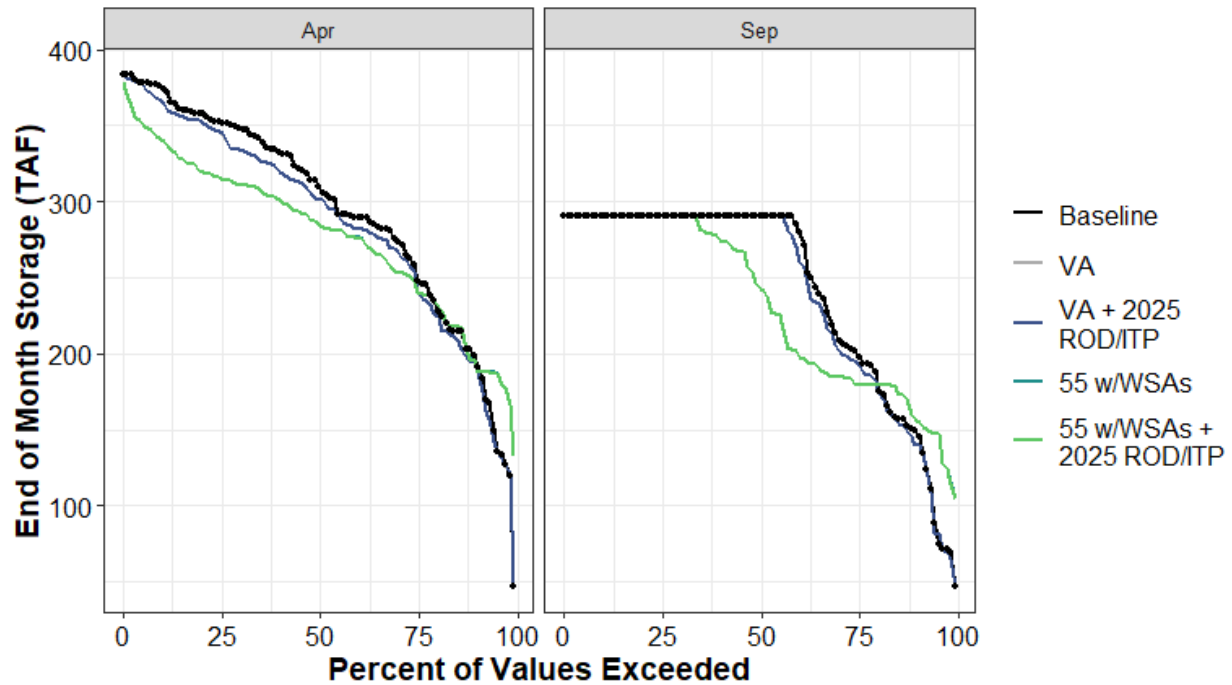
Figure H1a6-26. Camanche Reservoir End-of-April and End-of-September Storage under Baseline, Regulatory Pathway, and Voluntary Agreement Pathway
