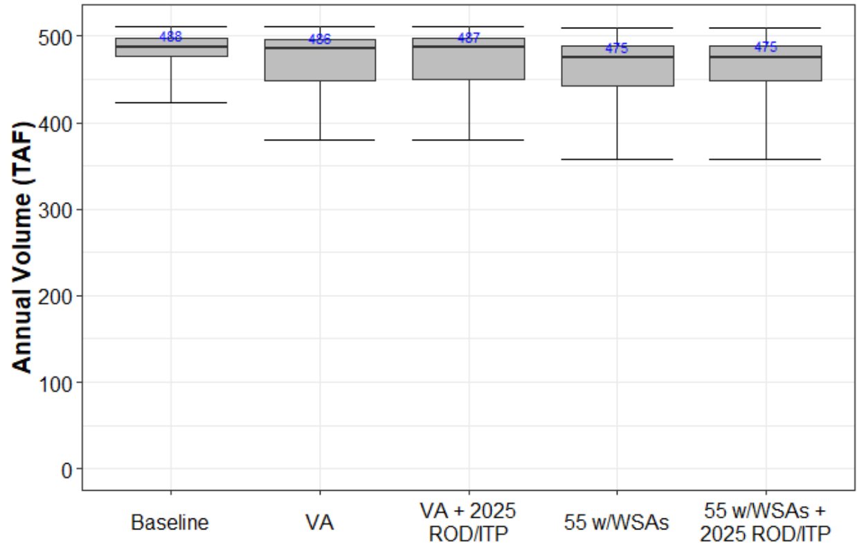
Figure H1a6-40. Annual Sacramento/Delta Supply to Municipal and Industrial Use in the Sacramento River Watershed for Baseline, VA Pathway, Regulatory Pathway Scenarios
