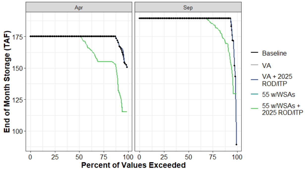
Figure H1a6-34. Pardee Reservoir End-of-April and End-of-September Storage under Baseline, Regulatory Pathway, and Voluntary Agreement Pathway
