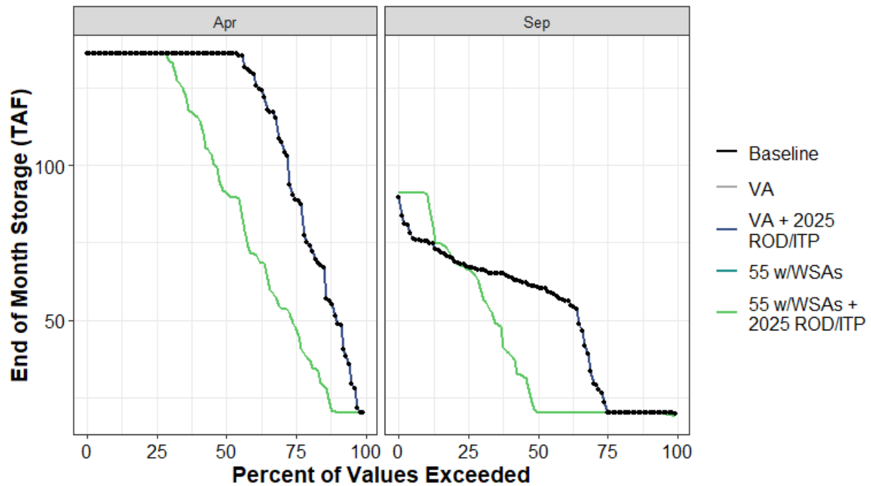
Figure H1a6-25. Black Butte Reservoir End-of-April and End-of-September Storage under Baseline, Regulatory Pathway, and Voluntary Agreement Pathway
