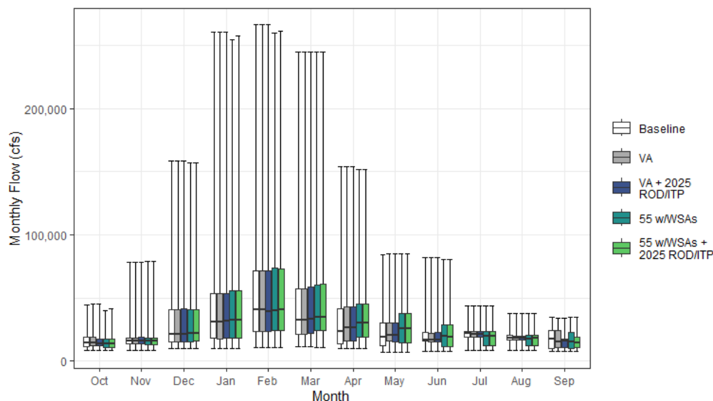
Figure H1a6-18. Monthly Delta Inflow for Baseline, Regulatory Pathway, and Voluntary Agreement Pathway
