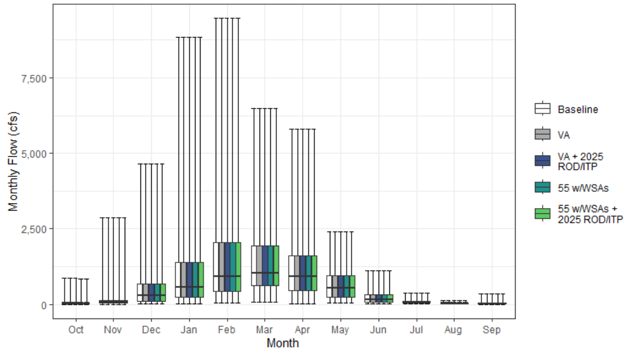
Figure H1a6-11. Monthly Streamflow for the Cosumnes River above the Confluence with the Mokelumne River under Baseline, Voluntary Agreement Pathway, and Regulatory Pathway Agreement Pathway
