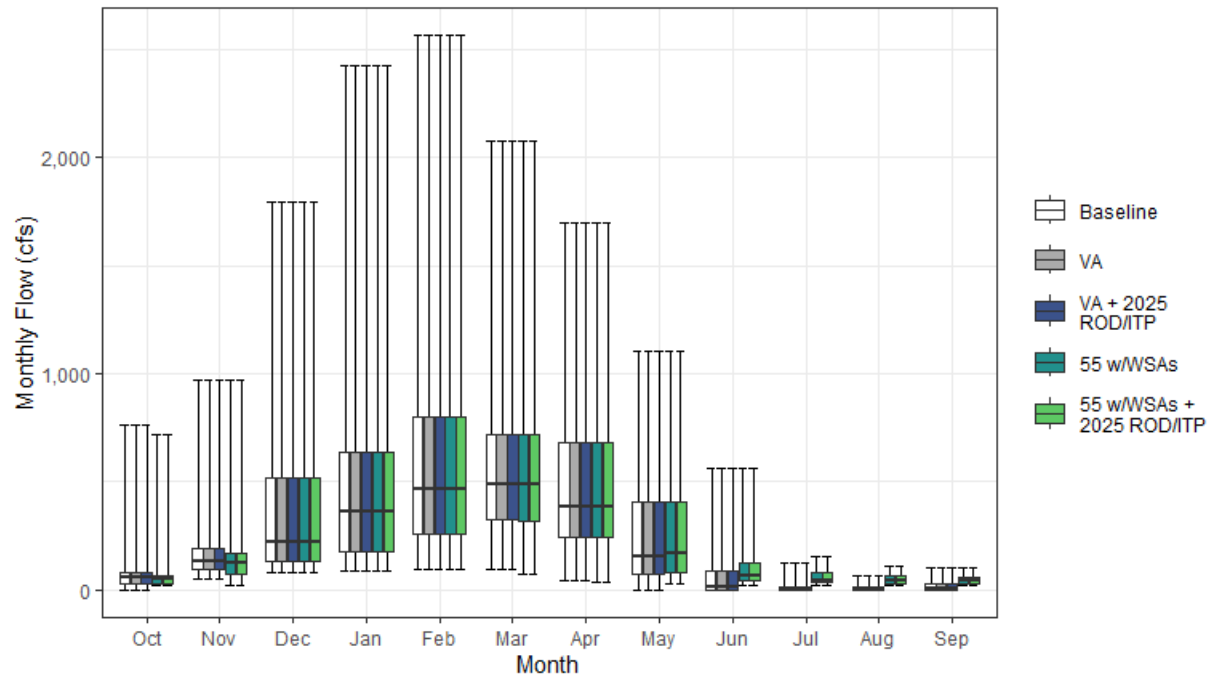
Figure H1a6-13. Monthly Streamflow for Deer Creek under Baseline, Voluntary Agreement Pathway, and Regulatory Pathway Agreement Pathway
