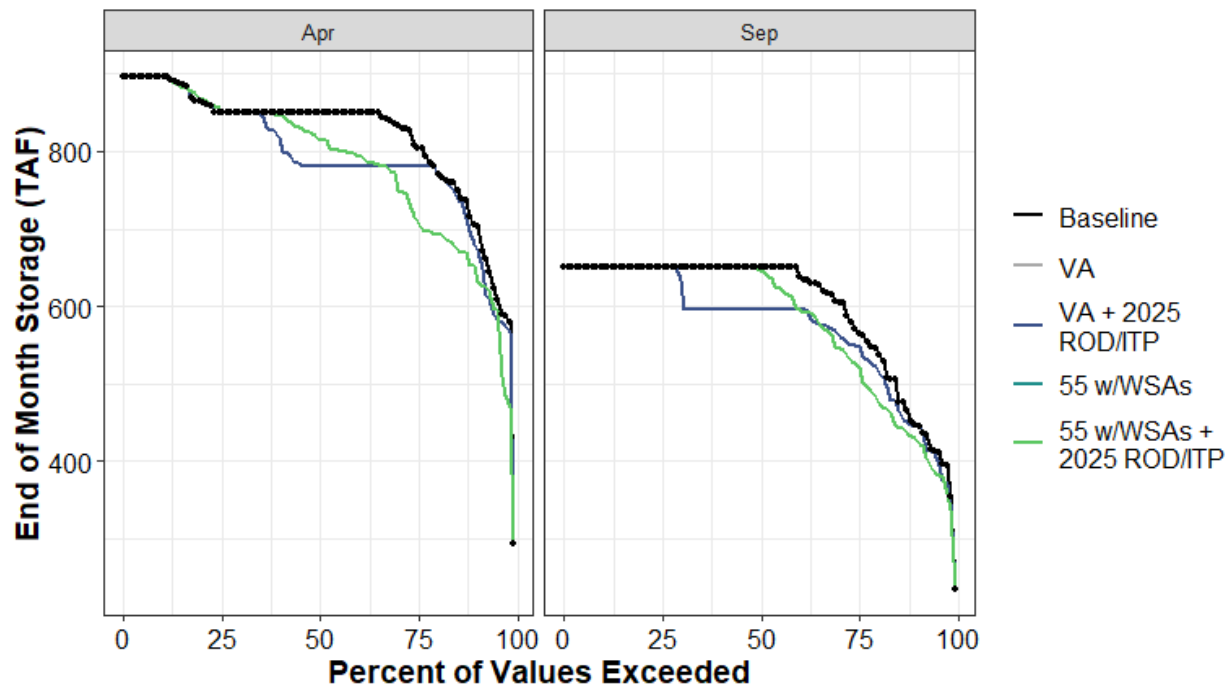
Figure H1a6-31. New Bullards Bar Reservoir End-of-April and End-of-September Storage under Baseline, Regulatory Pathway, and Voluntary Agreement Pathway
