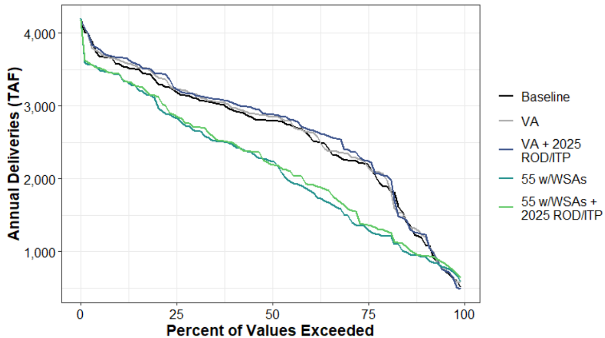
Figure H1a7-219. Surface Water Supplied to Total SWP Table A Annual Percent Exceedance Plot.
