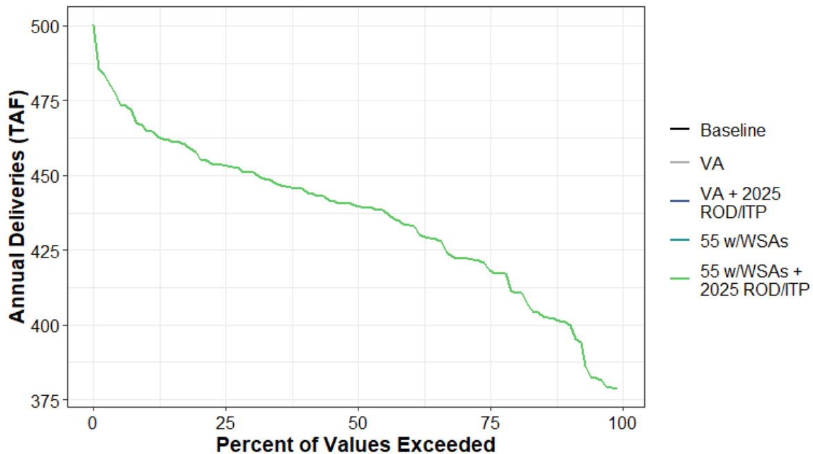
Figure H1a7-201. Total Water Supplied to Water Budget Area 61N (Agricultural) Annual Percent Exceedance Plot.
