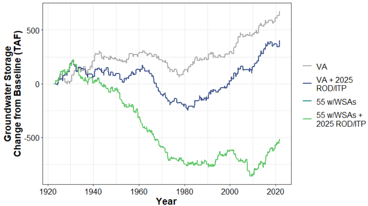
Figure H1a7-245. Eastern San Joaquin Groundwater Basin End of Year Storage—Change from Baseline (TAF)
