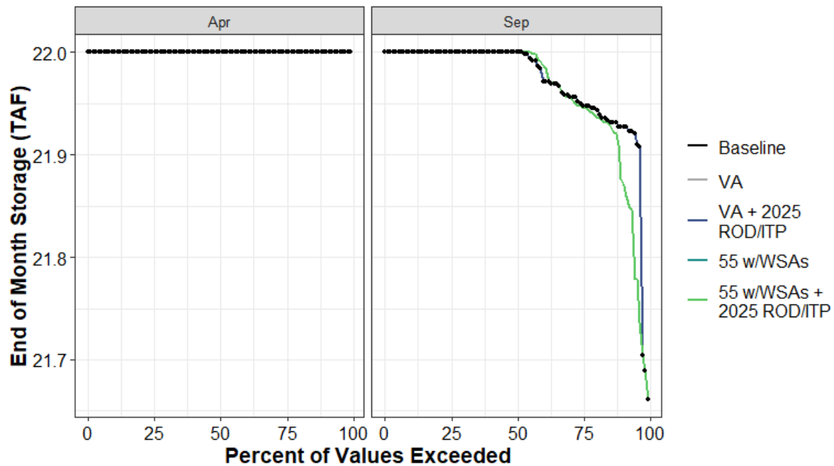
Figure H1a7-107. Lake Amador End of April and End of September Storage (TAF) Percent Exceedance Plot
