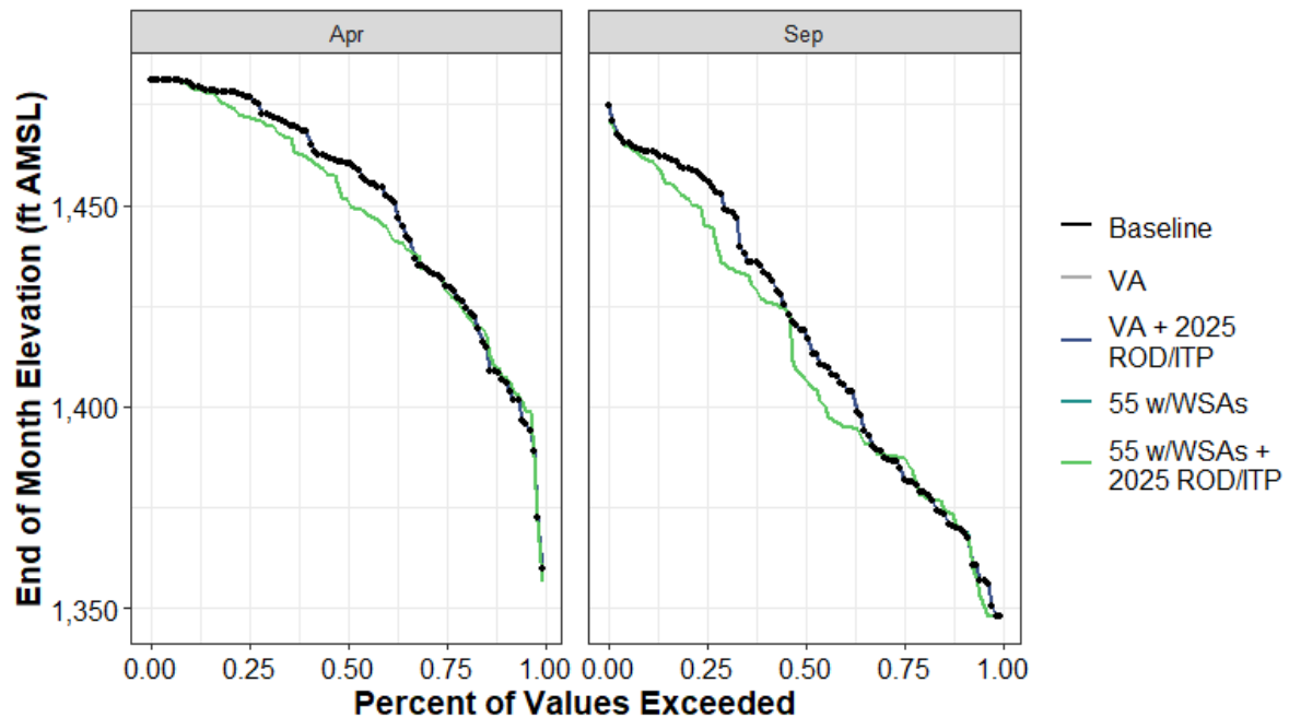
Figure H1a7-100. Indian Valley Reservoir End-of-April and End-of-September Elevation (ft AMSL) Percent Exceedance Plot
