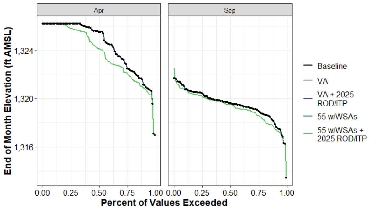
Figure H1a7-84. Clear Lake Reservoir End-of-April and End-of-September Elevation (ft AMSL) Percent Exceedance Plot
