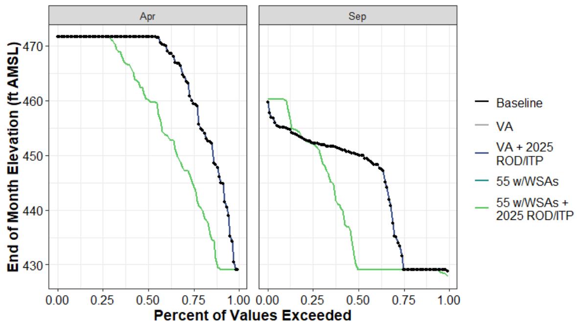
Figure H1a7-70. Black Butte Reservoir End-of-April and End-of-September Elevation (ft AMSL) Percent Exceedance Plot
