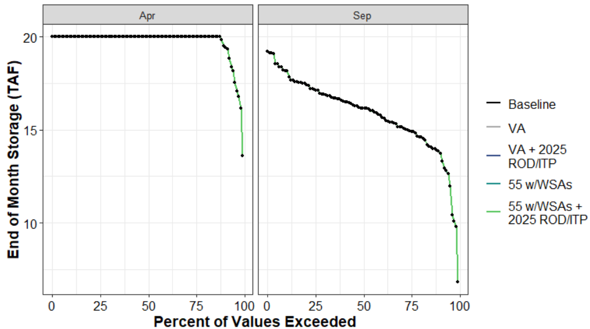
Figure H1a7-151. Stumpy Meadows End of April and End of September Storage (TAF) Percent Exceedance Plot
