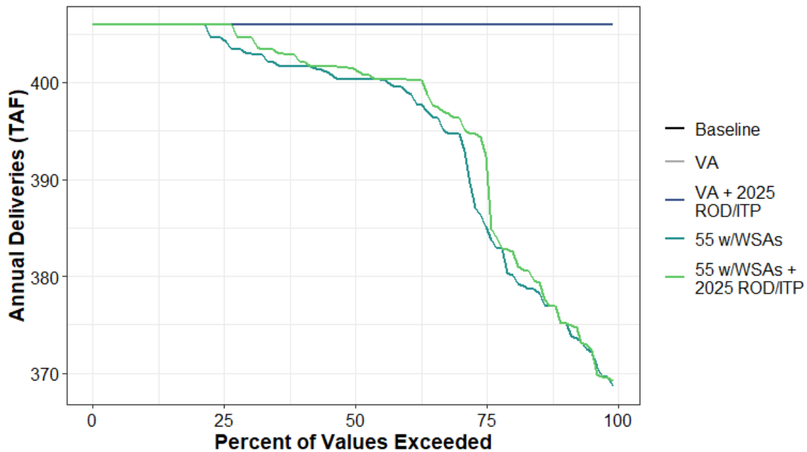
Figure H1a7-194. Total Water Supplied to Water Budget Area 26 (Urban) Annual Percent Exceedance Plot.
