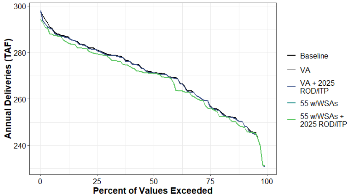
Figure H1a7-177. Total Water Supplied to Water Budget Areas 14 and 15N (Agricultural) Annual Percent Exceedance Plot.
