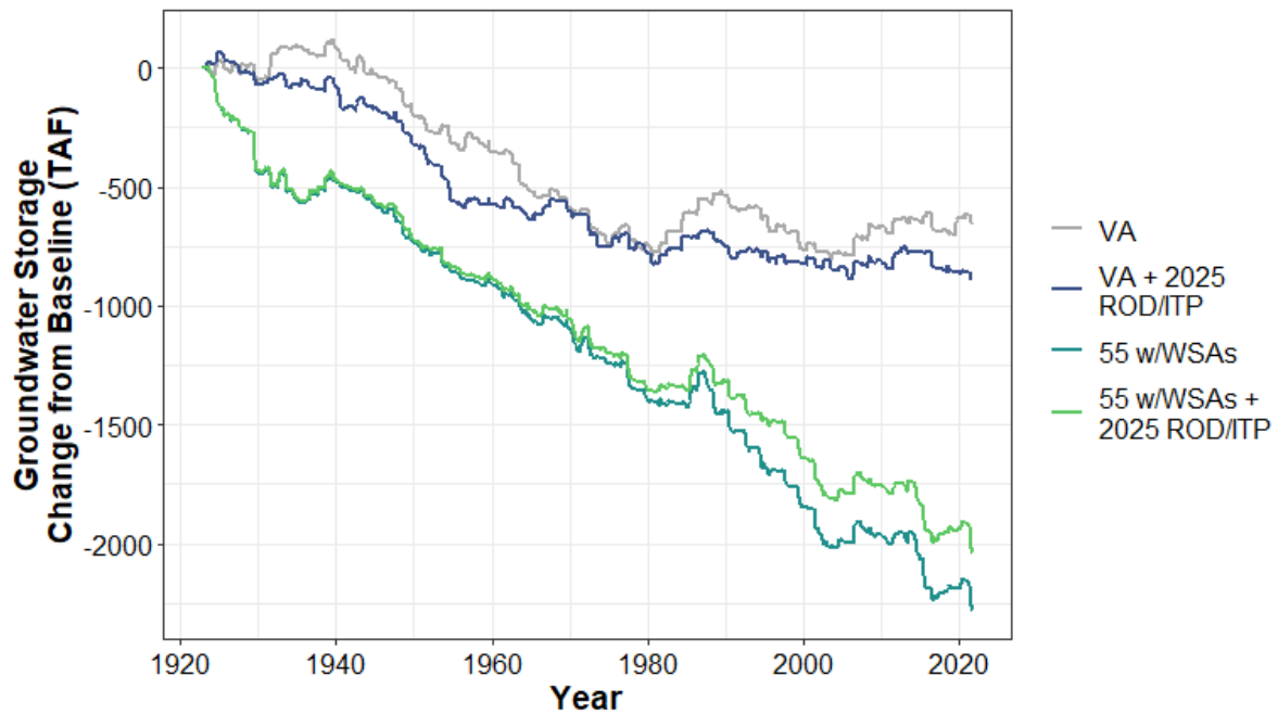
Figure H1a7-243. Colusa Groundwater Basin End of Year Storage—Change from Baseline (TAF)
