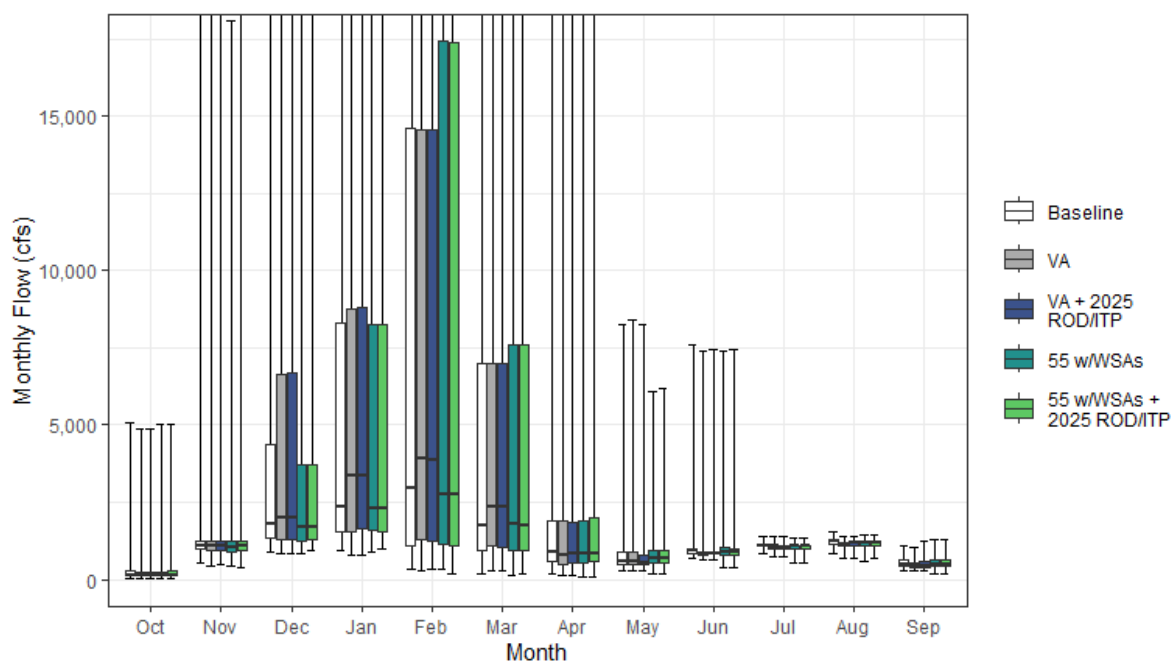
Figure H1a7-36. Sutter Bypass Streamflow near Karnak Monthly Boxplot (cfs)
