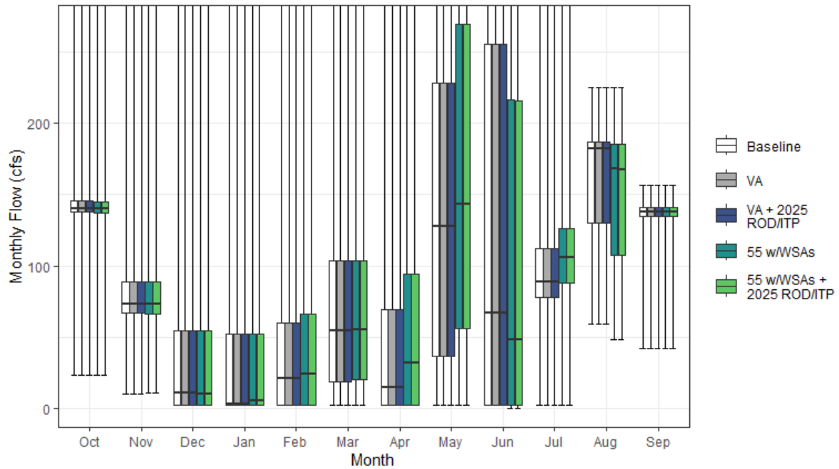
Figure H1a7-57. Milton-Bowman Tunnel Monthly Boxplot (cfs)
