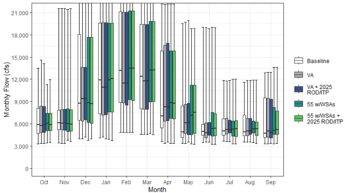
Figure H1a7-30. Sacramento River Streamflow below Wilkins Slough Monthly Boxplot (cfs)
