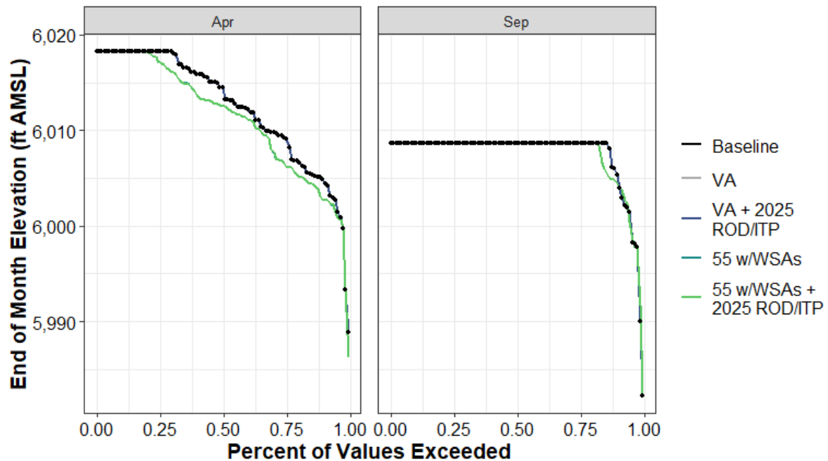
Figure H1a7-102. Jackson Meadows Reservoir End-of-April and End-of-September Elevation (ft AMSL) Percent Exceedance Plot
