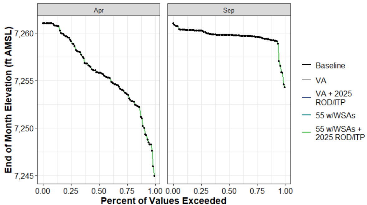
Figure H1a7-146. Silver Lake Reservoir End-of-April and End-of-September Elevation (ft AMSL) Percent Exceedance Plot
