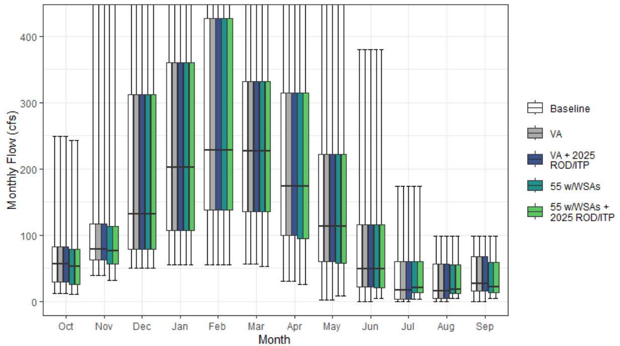
Figure H1a7-3. Antelope Creek Streamflow above Confluence with Sacramento River Monthly Boxplot (cfs)
