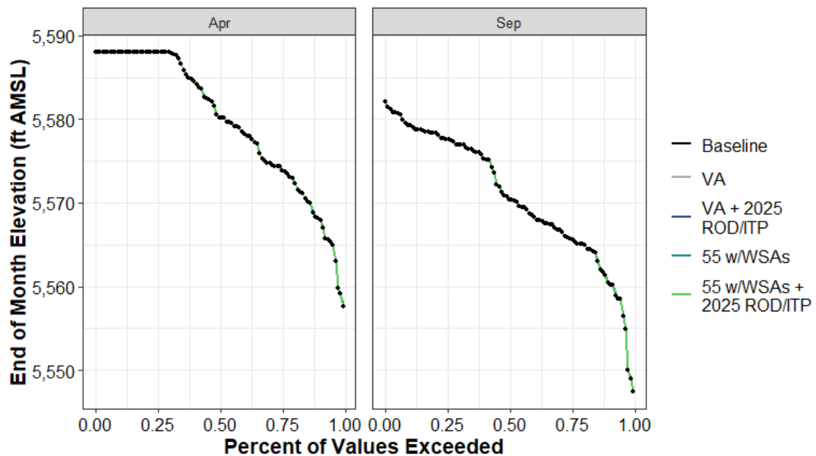
Figure H1a7-94. Frenchman Lake Reservoir End-of-April and End-of-September Elevation (ft AMSL) Percent Exceedance Plot
