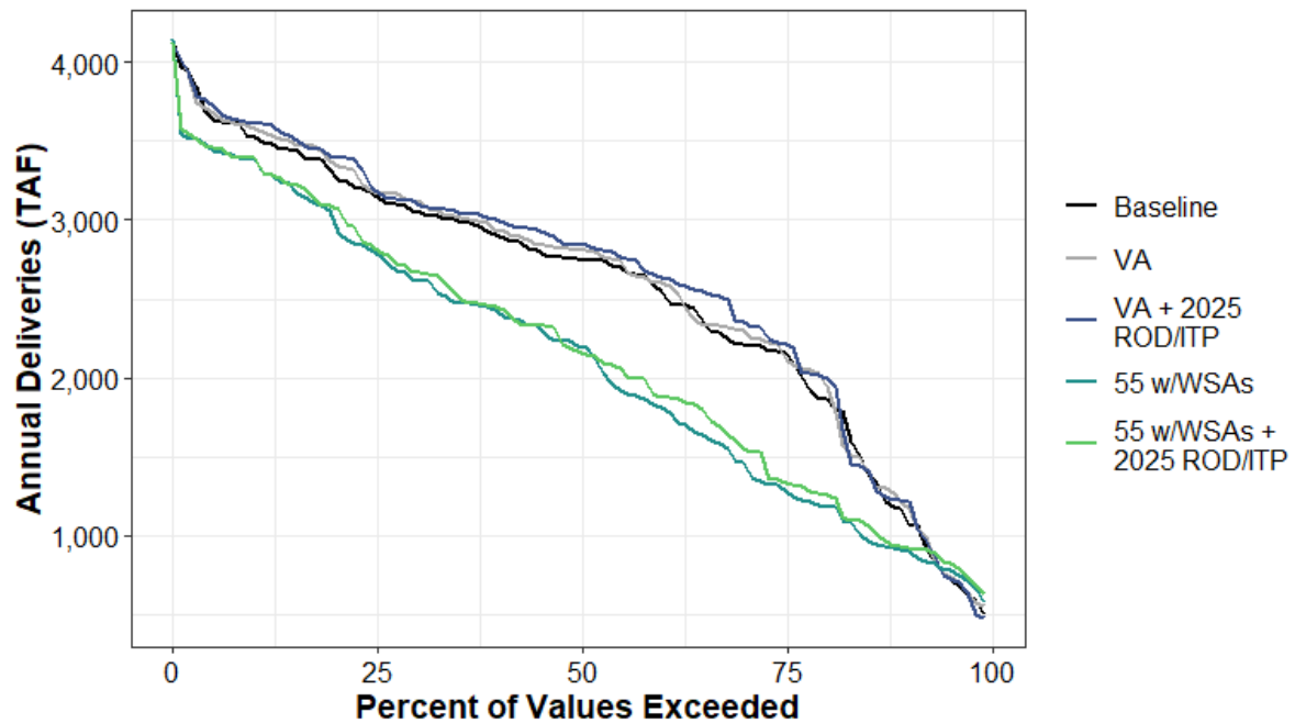
Figure H1a7-221. Surface Water Supplied to SWP Table A South of Delta Annual Percent Exceedance Plot.
