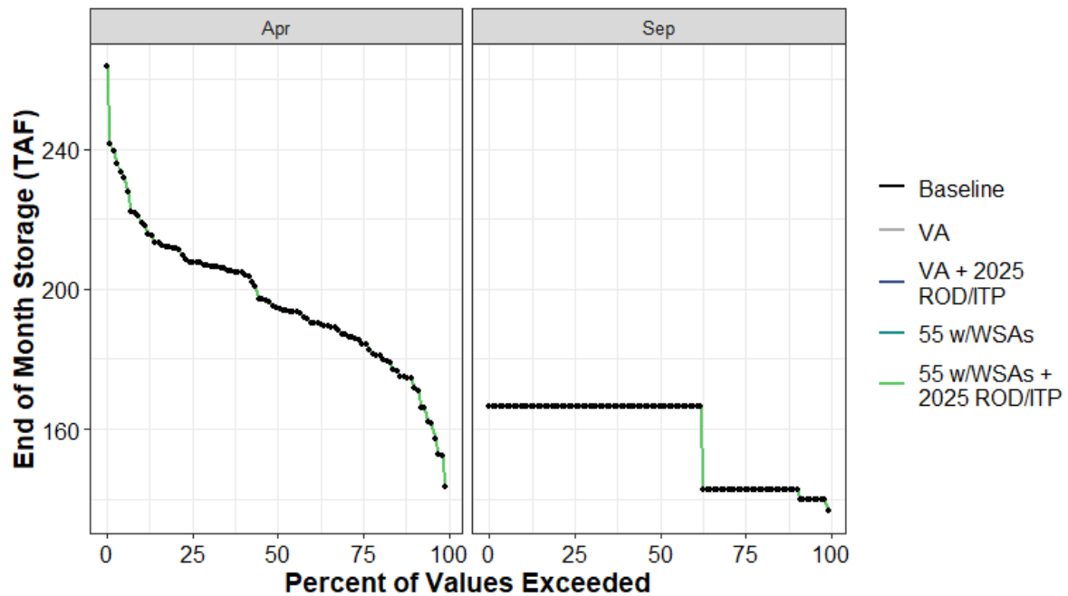
Figure H1a7-157. Union Valley Reservoir End of April and End of September Storage (TAF) Percent Exceedance Plot
