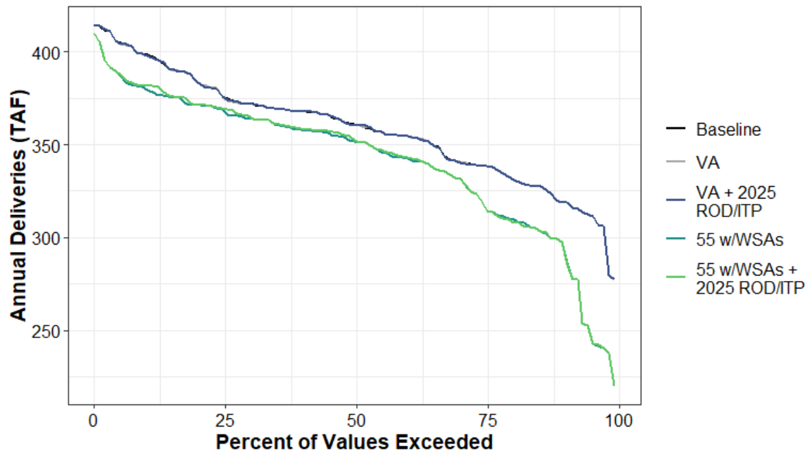
Figure H1a7-165. Total Water Supplied to Water Budget Areas 4 and 6 (Agricultural) Annual Percent Exceedance Plot.
