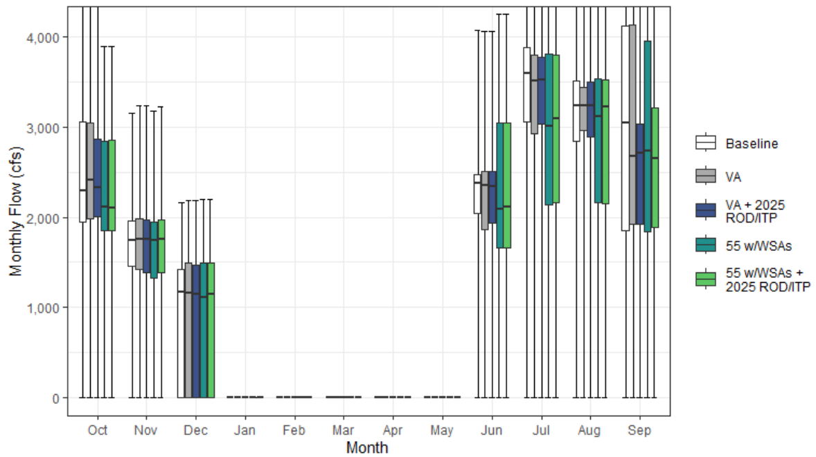
Figure H1a7-47. Delta Cross Channel Monthly Boxplot (cfs)
