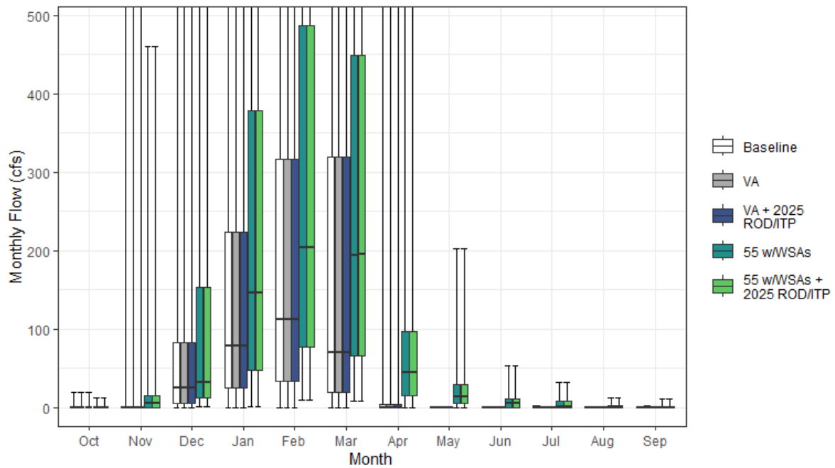
Figure H1a7-12. Calaveras River Streamflow above Delta Monthly Boxplot (cfs)
