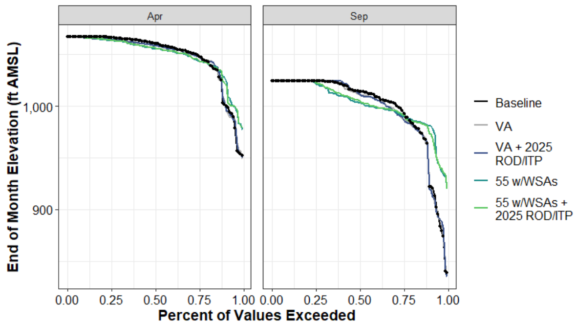
Figure H1a7-144. Shasta Lake Reservoir End-of-April and End-of-September Elevation (ft AMSL) Percent Exceedance Plot
