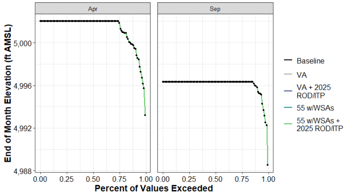
Figure H1a7-68. Antelope Reservoir End-of-April and End-of-September Elevation (ft AMSL) Percent Exceedance Plot
