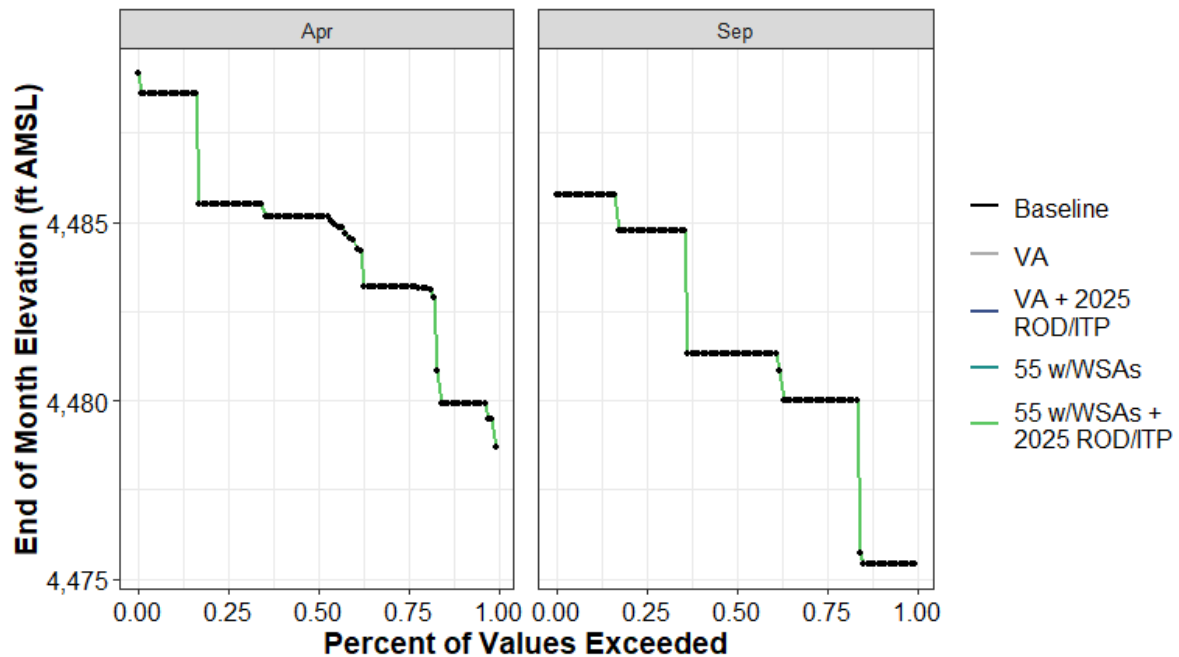
Figure H1a7-105. Lake Almanor Reservoir End-of-April and End-of-September Elevation (ft AMSL) Percent Exceedance Plot
