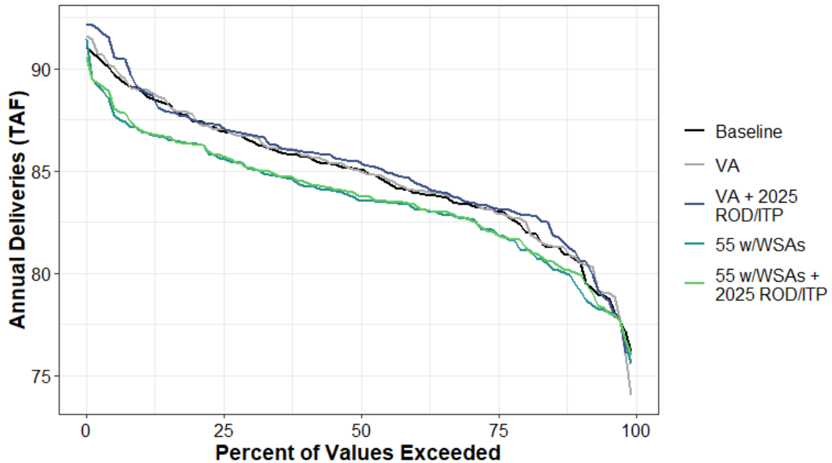
Figure H1a7-183. Total Water Supplied to Water Budget Area 17 (Refuge) Annual Percent Exceedance Plot.
