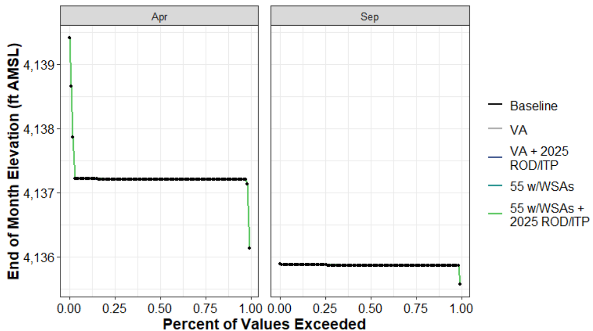
Figure H1a7-76. Butt Valley Reservoir End-of-April and End-of-September Elevation (ft AMSL) Percent Exceedance Plot
