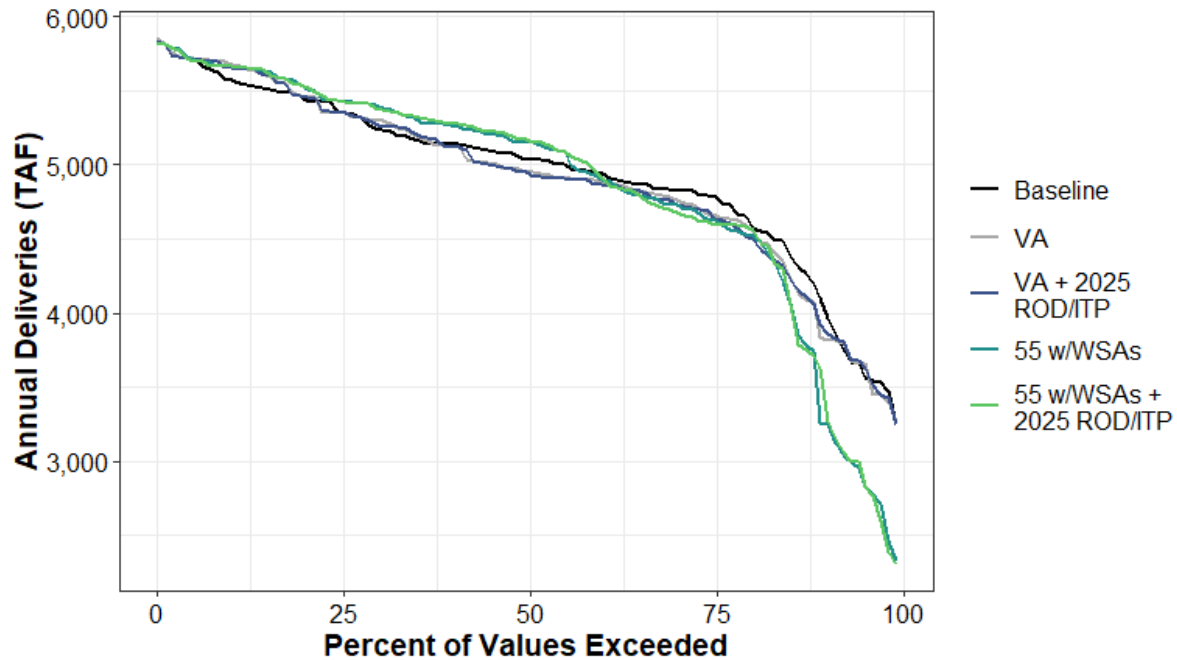
Figure H1a7-206. Surface Water Supplied to Total CVP Deliveries Annual Percent Exceedance Plot.
