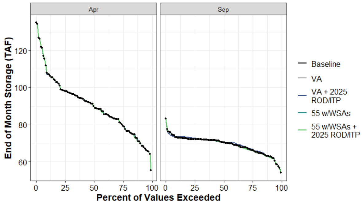
Figure H1a7-91. French Meadows End of April and End of September Storage (TAF) Percent Exceedance Plot
