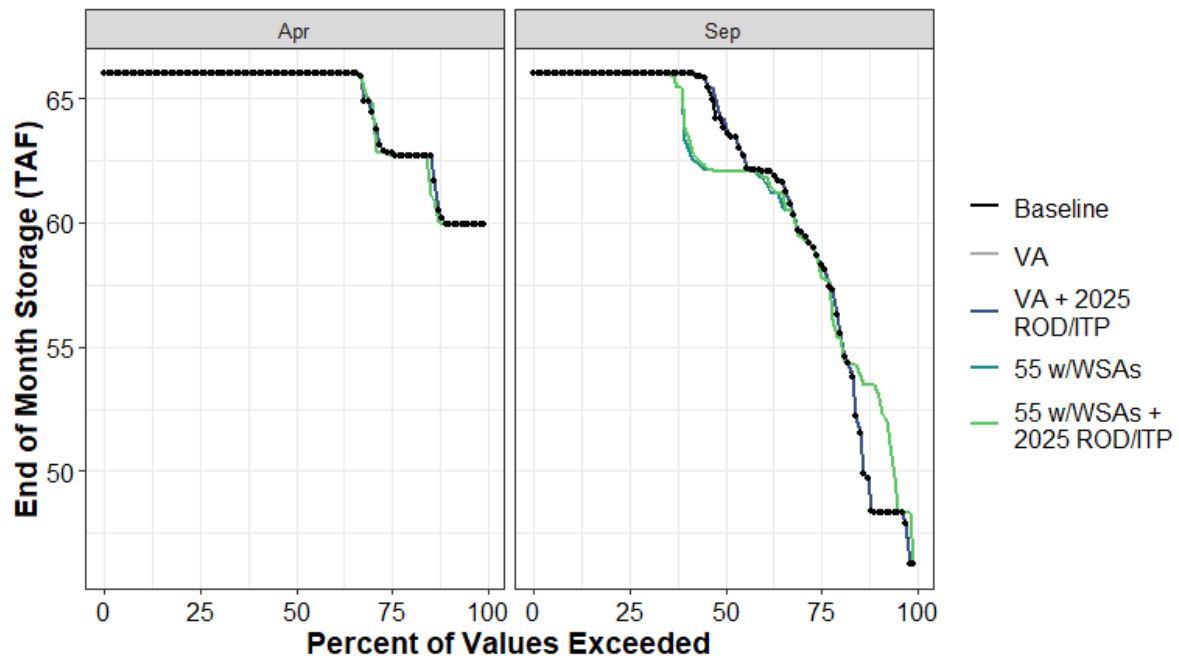
Figure H1a7-137. Rollins Reservoir End of April and End of September Storage (TAF) Percent Exceedance Plot
