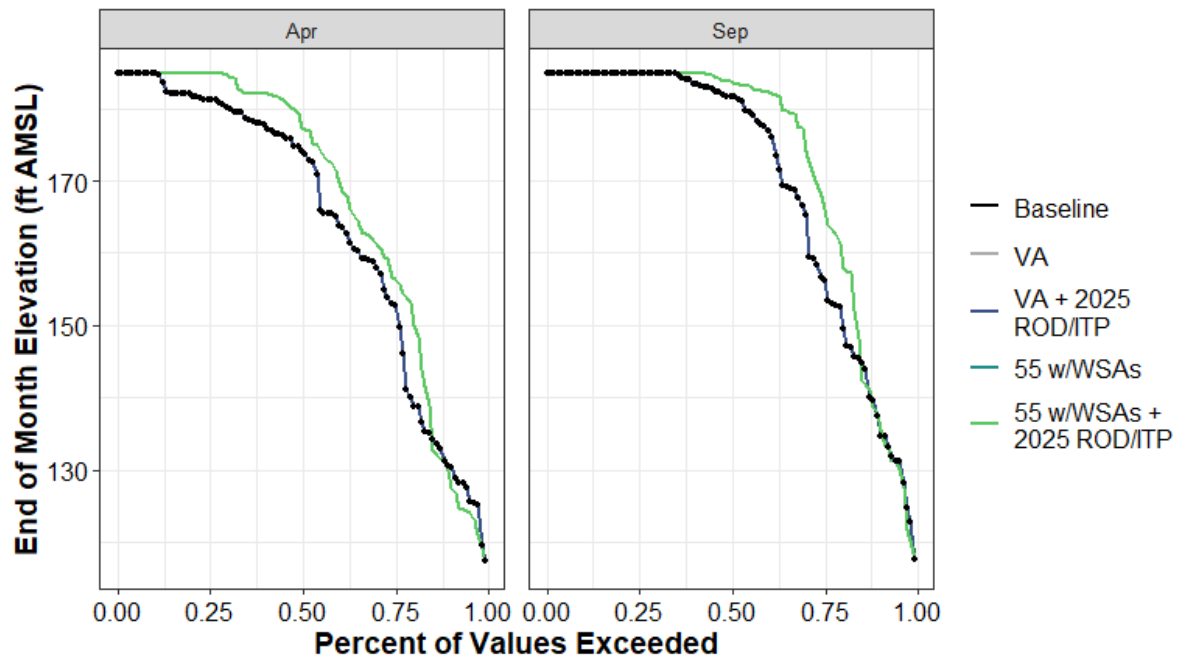
Figure H1a7-122. Los Vaqueros Reservoir End-of-April and End-of-September Elevation (ft AMSL) Percent Exceedance Plot
