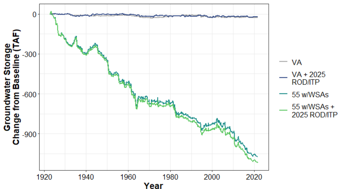
Figure H1a7-250. Yolo-Solano Groundwater Basin End of Year Storage—Change from Baseline
