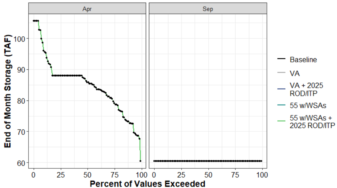
Figure H1a7-73. Bucks Lake End of April and End of September Storage (TAF) Percent Exceedance Plot
