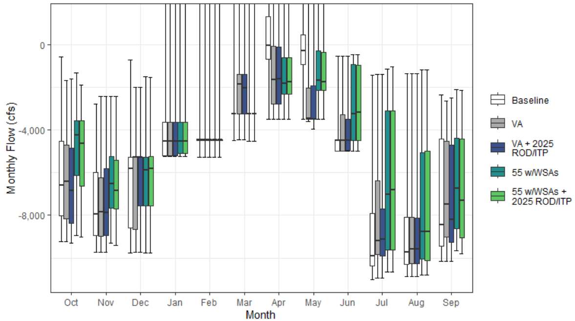
Figure H1a7-50. Old and Middle Rivers Net Flow Monthly Boxplot (cfs)
