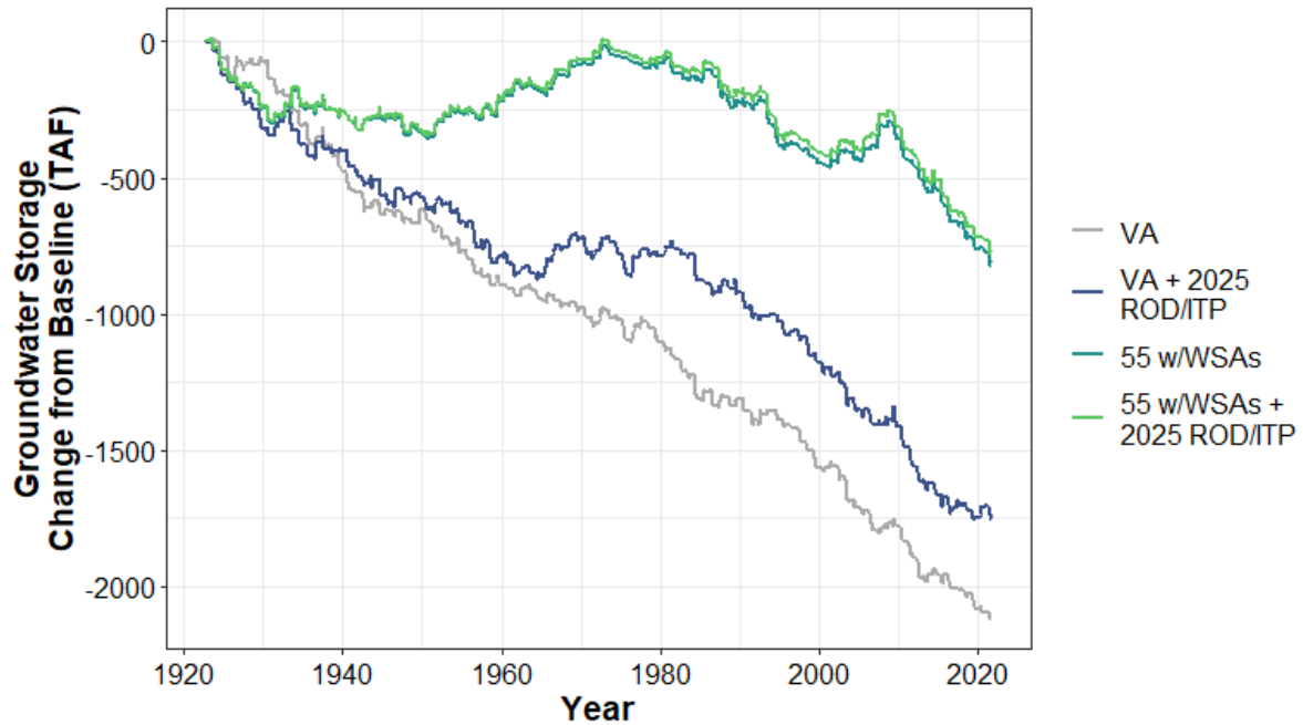
Figure H1a7-244. Cosumnes Groundwater Basin End of Year Storage—Change from Baseline (TAF)
