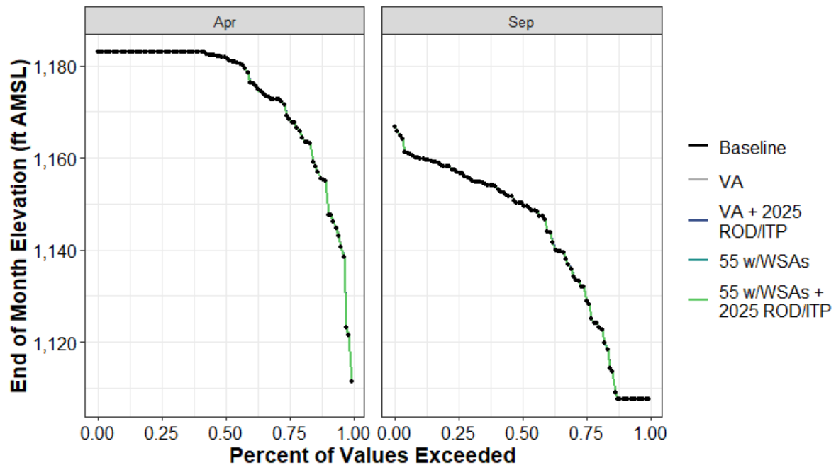
Figure H1a7-126. Merle Collins Reservoir End-of-April and End-of-September Elevation (ft AMSL) Percent Exceedance Plot
