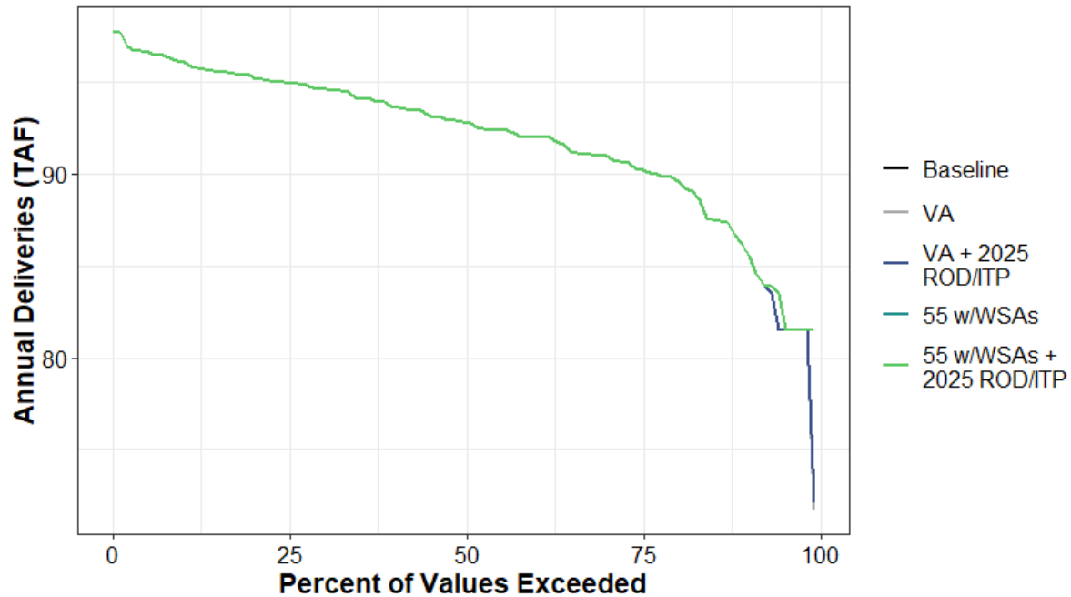
Figure H1a7-169. Total Water Supplied to Water Budget Area 8 (Refuge) Annual Percent Exceedance Plot.
