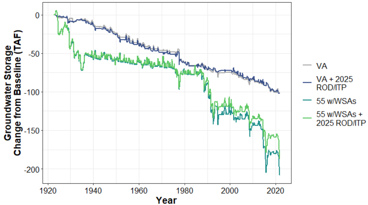
Figure H1a7-248. Redding Groundwater Basin End of Year Storage—Change from Baseline
