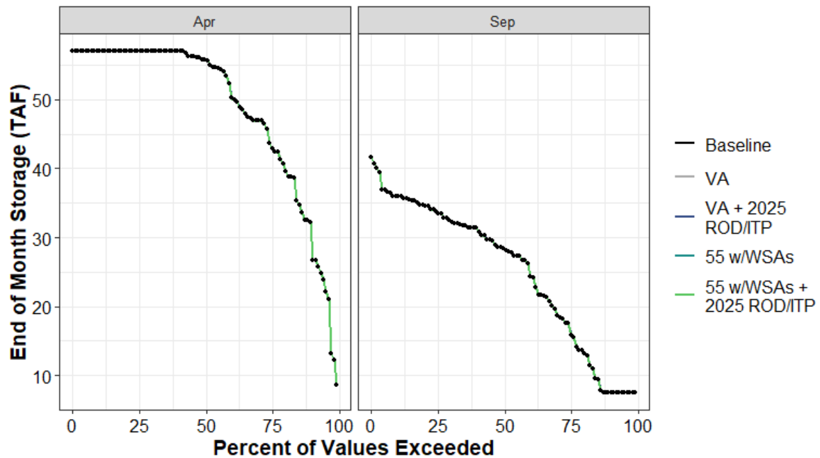
Figure H1a7-125. Merle Collins Reservoir End of April and End of September Storage (TAF) Percent Exceedance Plot
