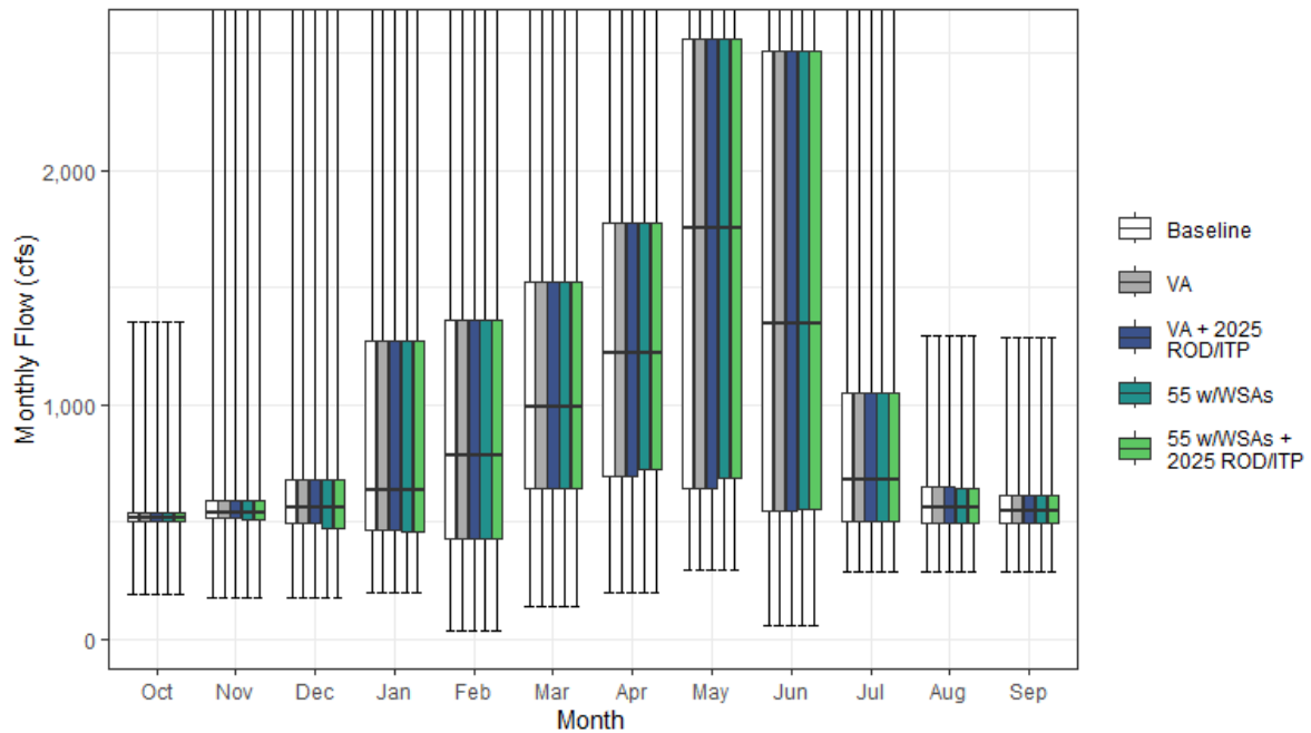
Figure H1a7-22. Mokelumne River Streamflow above Pardee Reservoir Monthly Boxplot (cfs)
