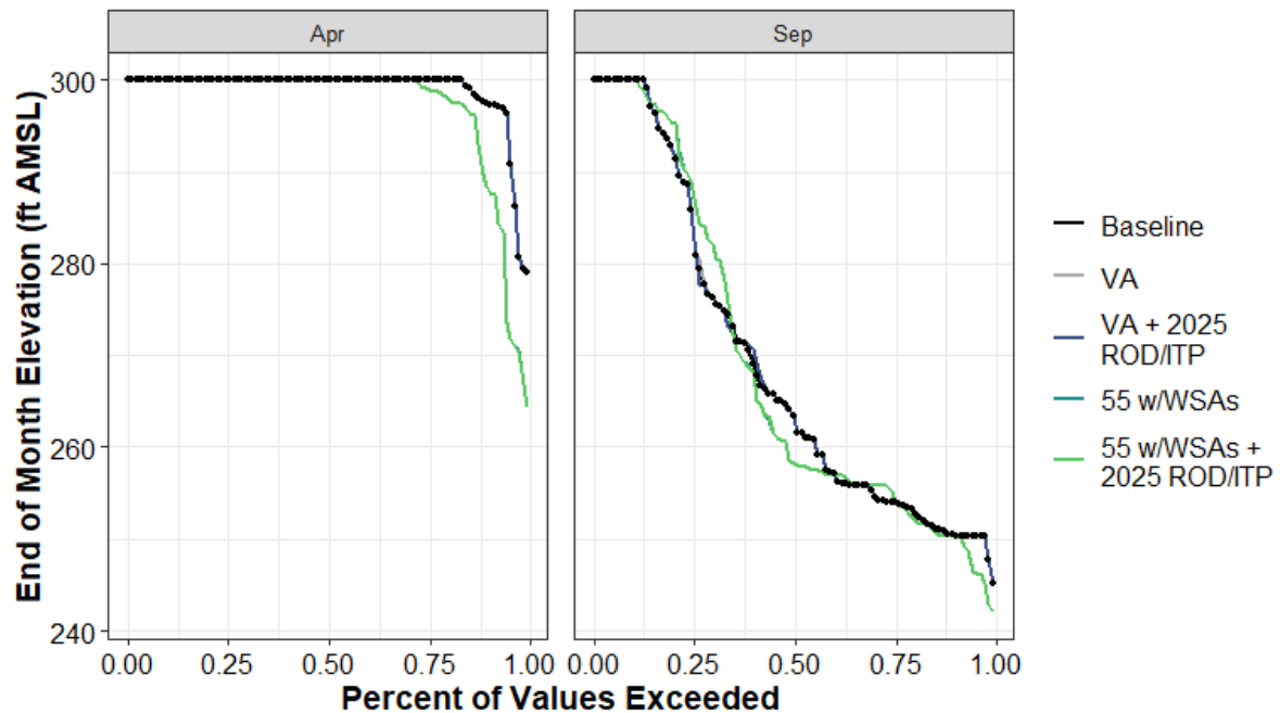
Figure H1a7-80. Camp Far West Reservoir End-of-April and End-of-September Elevation (ft AMSL) Percent Exceedance Plot
