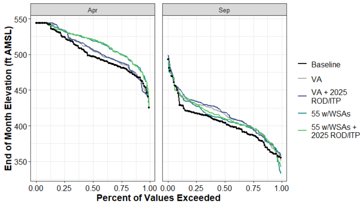
Figure H1a7-154. Total San Luis Reservoir End-of-April and End-of-September Elevation (ft AMSL) Percent Exceedance Plot
