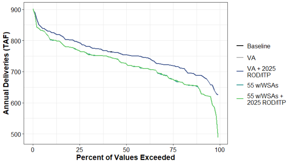
Figure H1a7-185. Total Water Supplied to Water Budget Areas 20 and 25 (Agricultural) Annual Percent Exceedance Plot.
