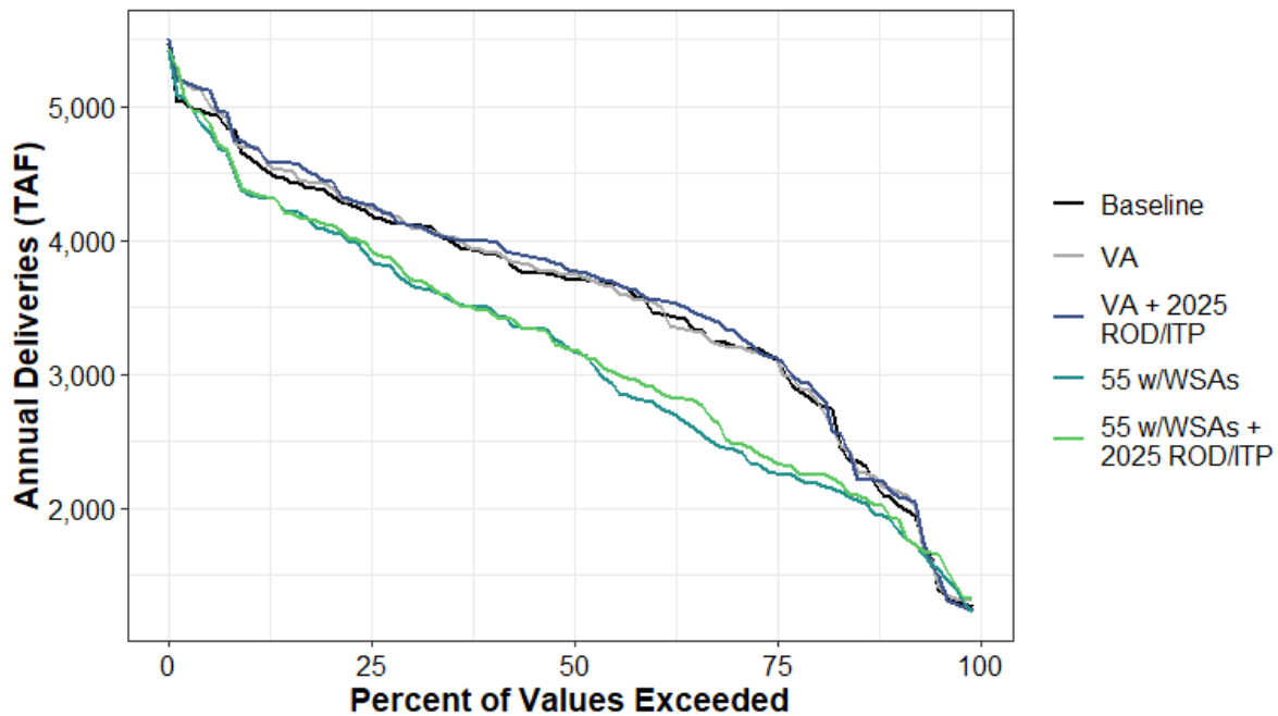
Figure H1a7-218. Surface Water Supplied to Total SWP Deliveries Annual Percent Exceedance Plot.
