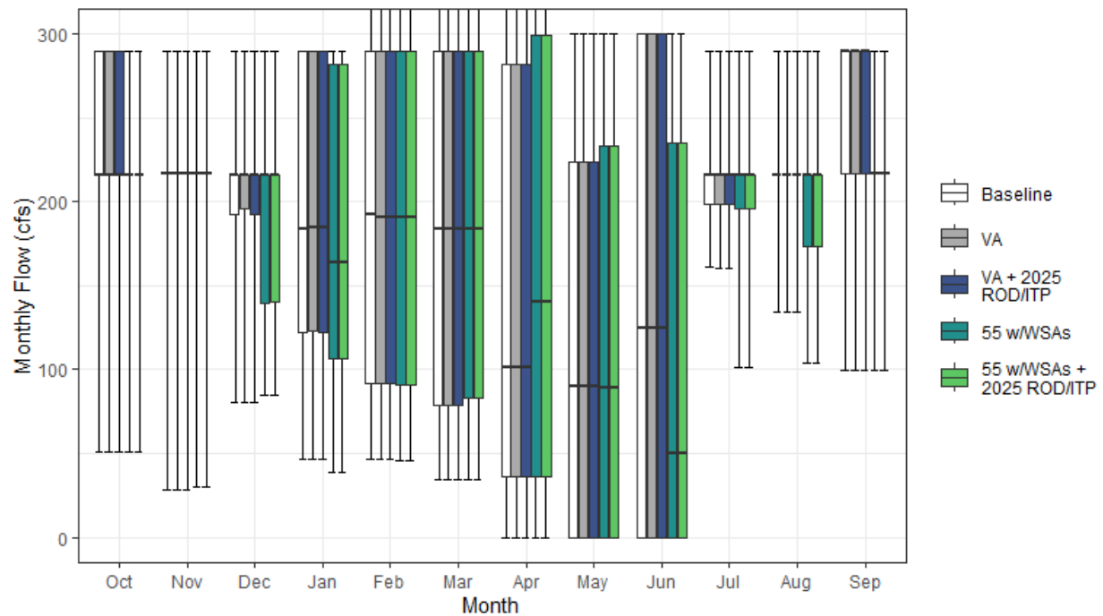
Figure H1a7-53. Bowman-Spaulding Conduit Monthly Boxplot (cfs)
