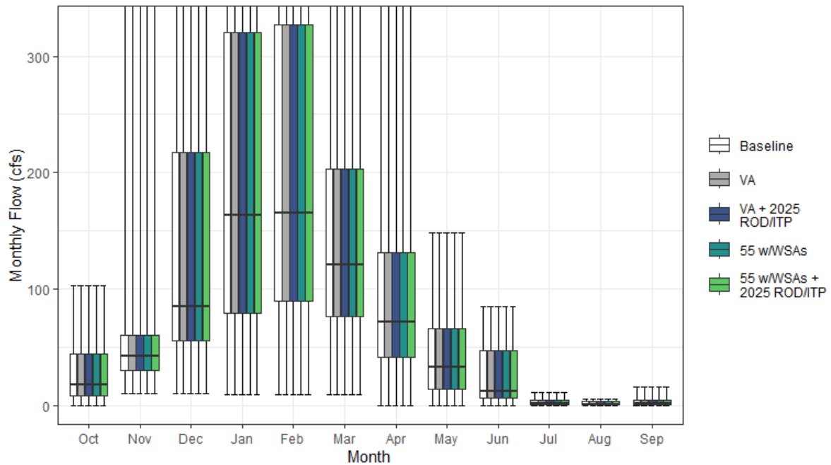
Figure H1a7-25. Paynes Creek Streamflow above Confluence with Sacramento River Monthly Boxplot (cfs)
