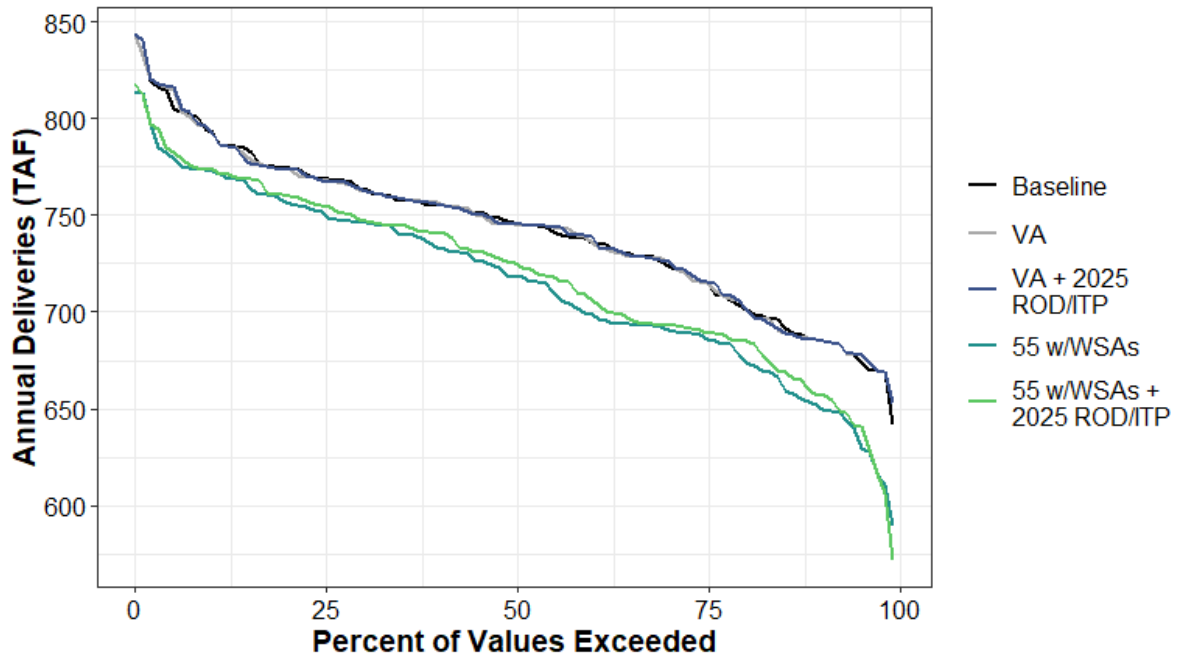
Figure H1a7-167. Total Water Supplied to Water Budget Area 7 (Agricultural) Annual Percent Exceedance Plot.
