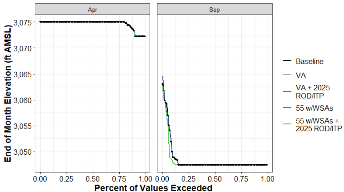
Figure H1a7-142. Scotts Flat Reservoir End-of-April and End-of-September Elevation (ft AMSL) Percent Exceedance Plot
