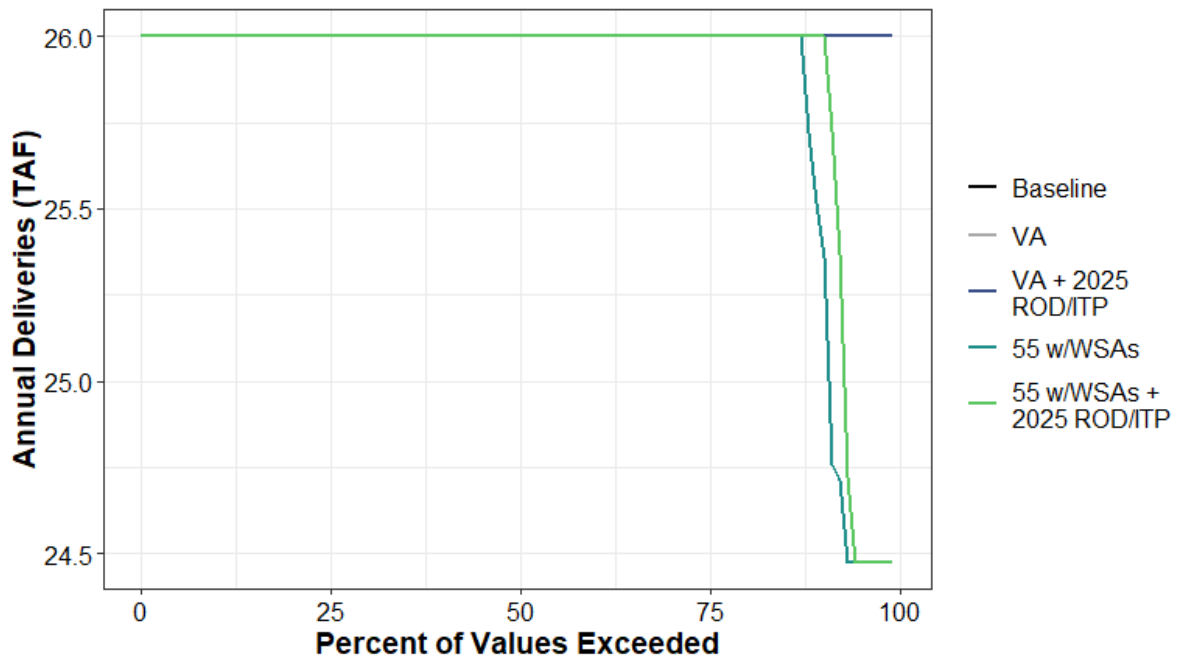
Figure H1a7-181. Total Water Supplied to Water Budget Area 16 (Urban) Annual Percent Exceedance Plot.
