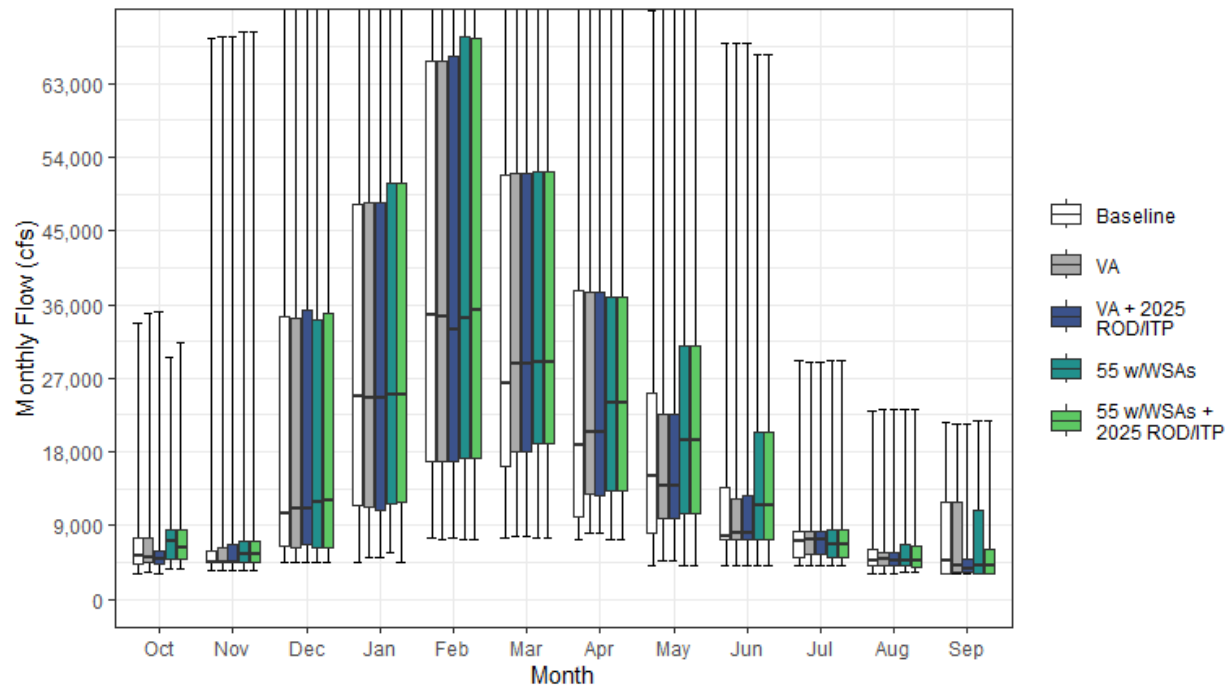
Figure H1a7-46. Delta Outflow, including Postprocessed VA Flows Monthly Boxplot (cfs)
