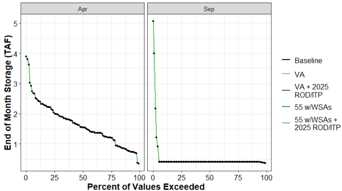
Figure H1a7-106. Lake Aloha End of April and End of September Storage (TAF) Percent Exceedance Plot
