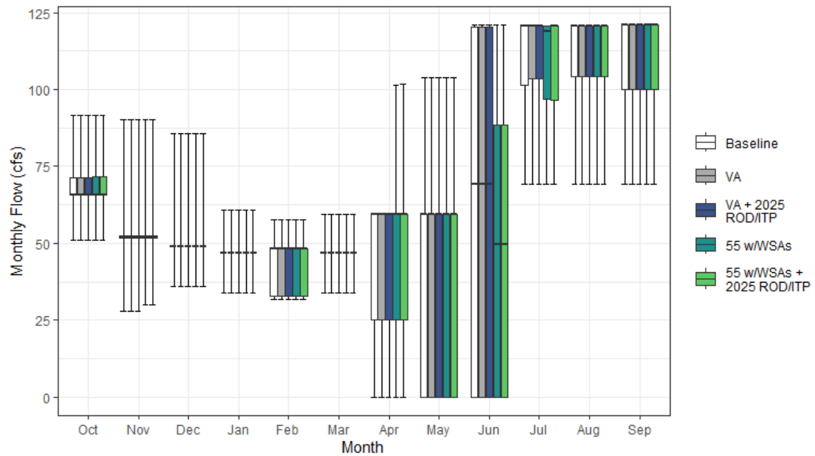
Figure H1a7-62. Chalk Bluff Canal Monthly Boxplot (cfs)
