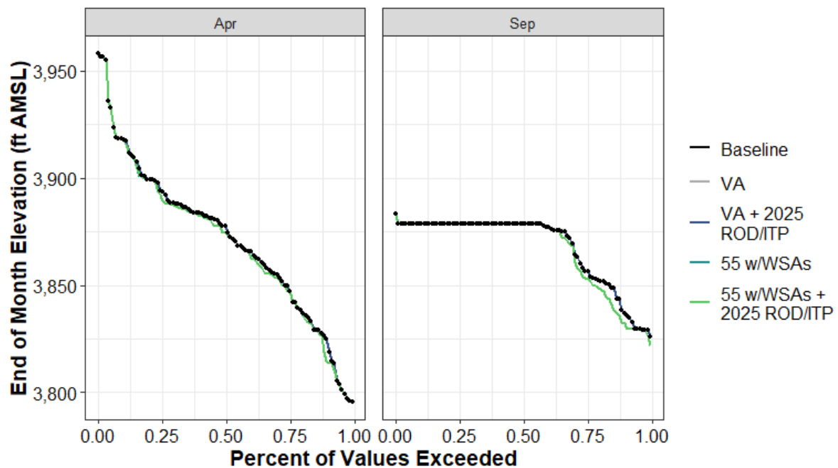
Figure H1a7-140. Salt Springs Reservoir End-of-April and End-of-September Elevation (ft AMSL) Percent Exceedance Plot
