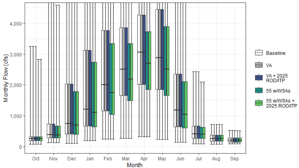
Figure H1a7-40. Yuba River, North Fork Streamflow above New Bullards Bar Reservoir Monthly Boxplot (cfs)
