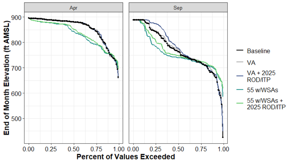
Figure H1a7-133. Oroville Reservoir End-of-April and End-of-September Elevation (ft AMSL) Percent Exceedance Plot
