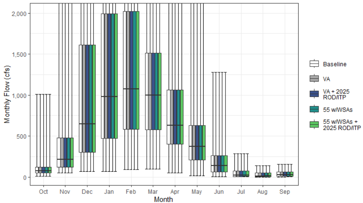
Figure H1a7-16. Cow Creek Streamflow above Confluence with Sacramento River Monthly Boxplot (cfs)
