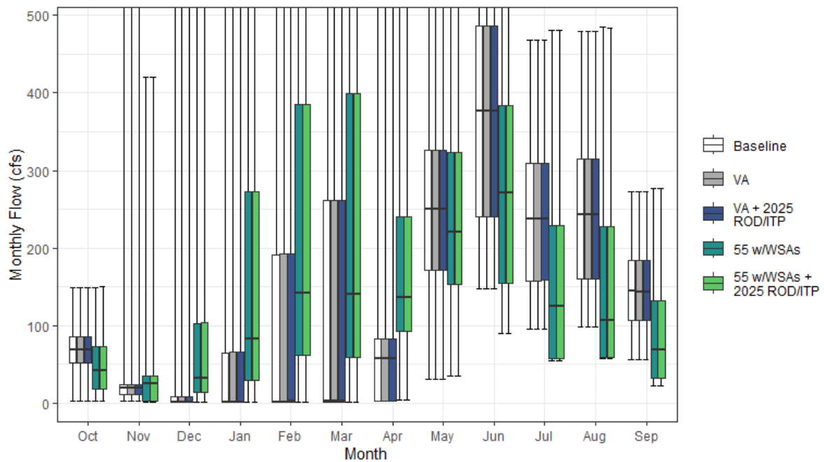
Figure H1a7-11. Calaveras River Streamflow below New Hogan Reservoir Monthly Boxplot (cfs)
