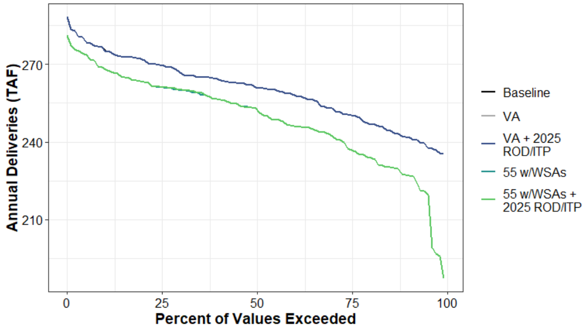
Figure H1a7-190. Total Water Supplied to Water Budget Area 23 (Agricultural) Annual Percent Exceedance Plot.
