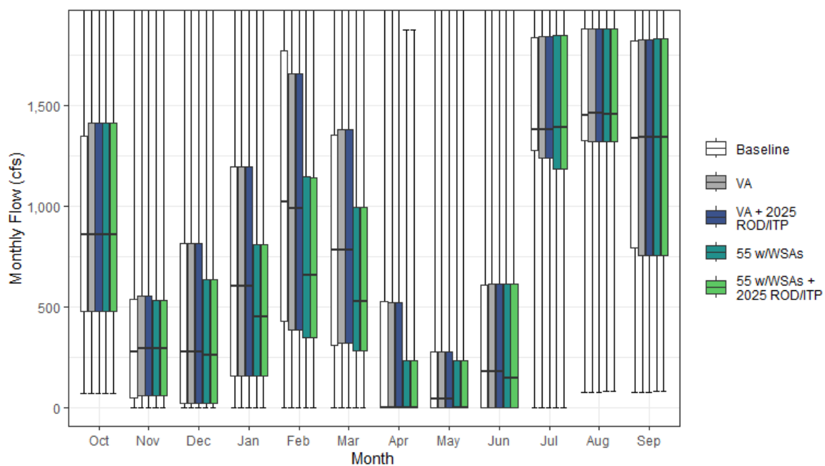
Figure H1a7-64. Spring Creek Conduit Monthly Boxplot (cfs)
