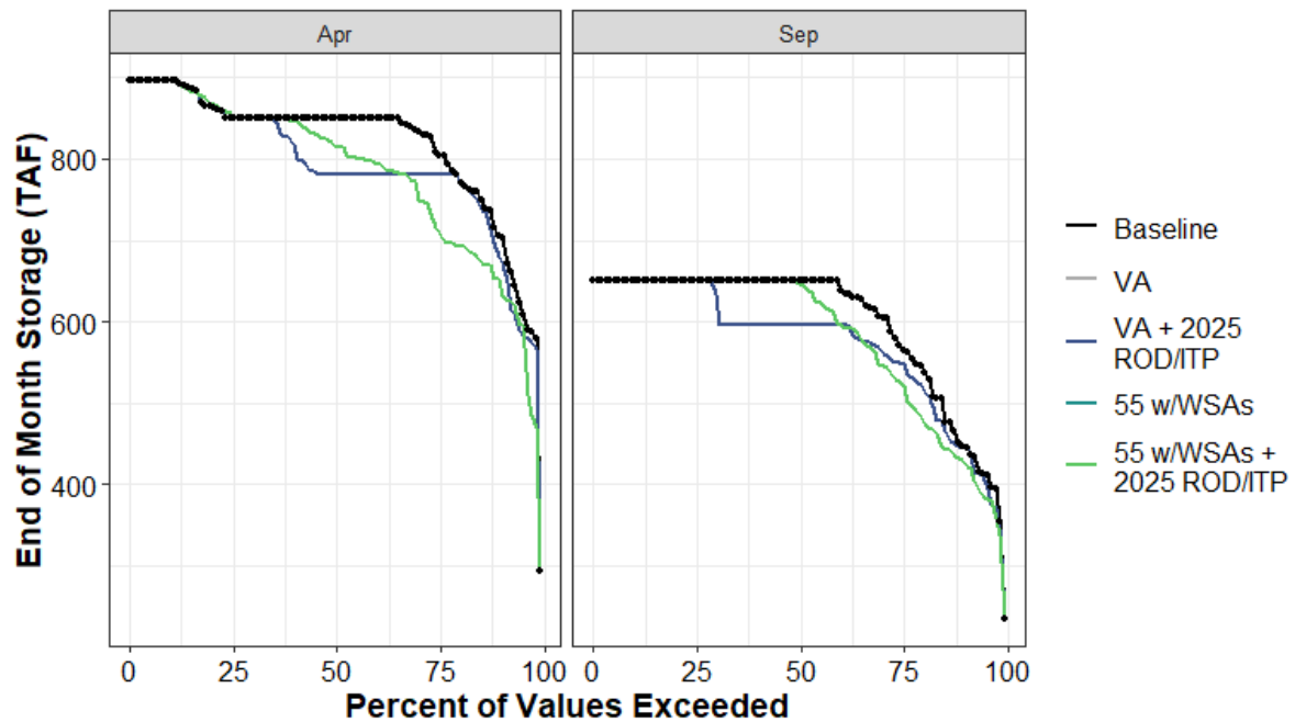
Figure H1a7-128. New Bullards Bar Reservoir End of April and End of September Storage (TAF) Percent Exceedance Plot
