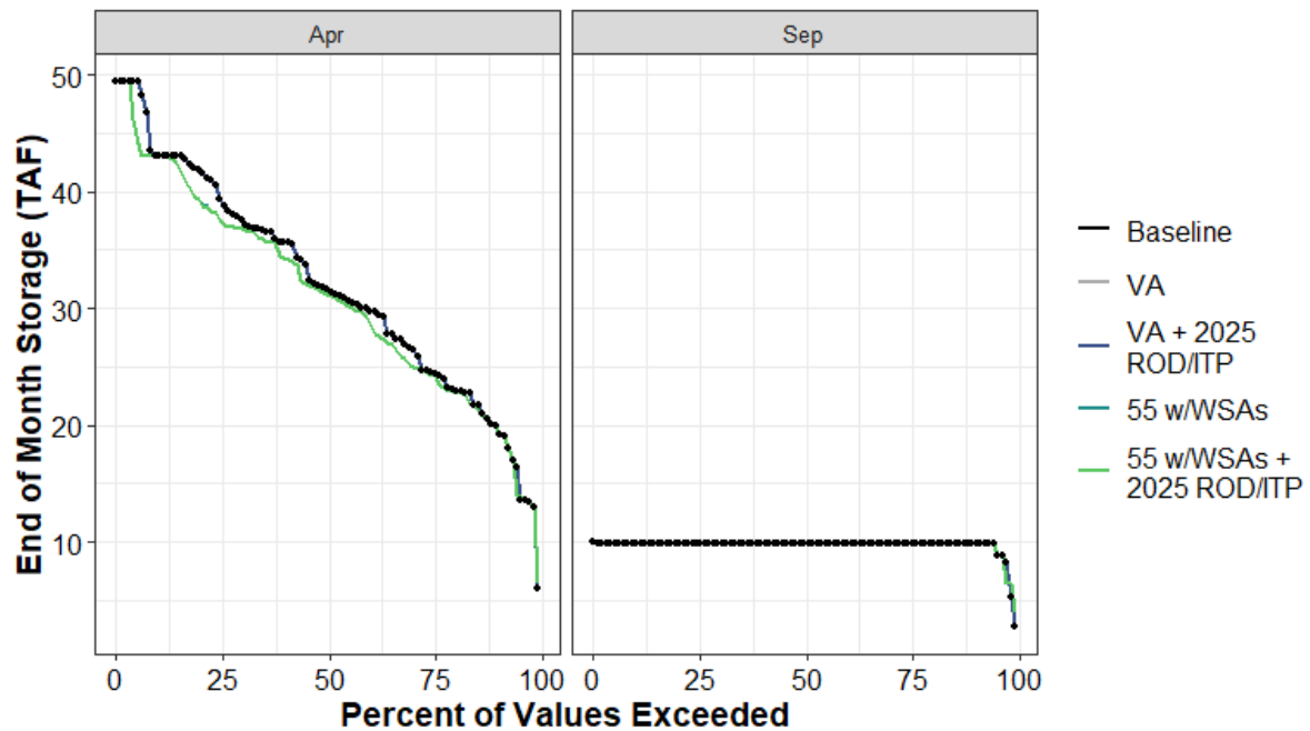
Figure H1a7-112. Lake Fordyce End of April and End of September Storage (TAF) Percent Exceedance Plot
