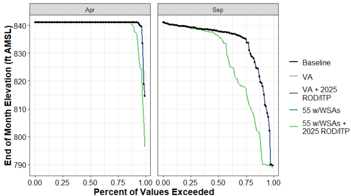
Figure H1a7-150. Stony Gorge Reservoir End-of-April and End-of-September Elevation (ft AMSL) Percent Exceedance Plot
