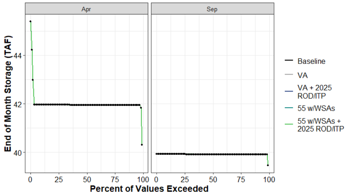
Figure H1a7-75. Butt Valley End of April and End of September Storage (TAF) Percent Exceedance Plot
