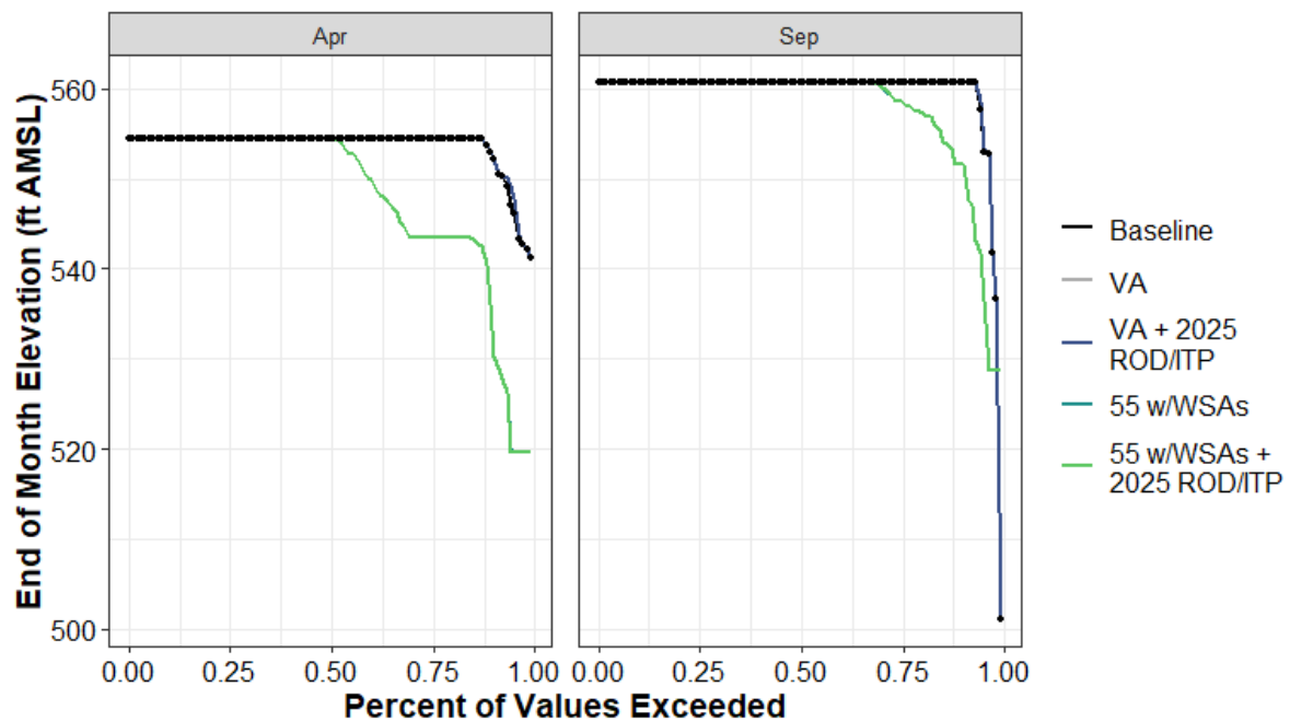
Figure H1a7-135. Pardee Reservoir End-of-April and End-of-September Elevation (ft AMSL) Percent Exceedance Plot
