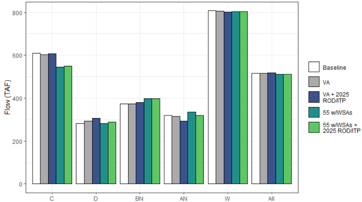
Figure H1a7-239. Total Average Annual Stream-Groundwater Flux (Net Groundwater Gain) for Sacramento River Watershed by WYT and Scenario (TAF/yr).
