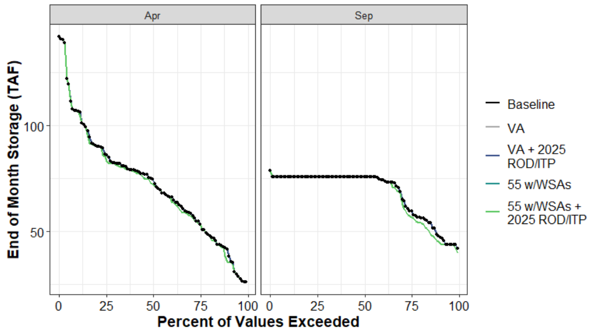
Figure H1a7-139. Salt Springs End of April and End of September Storage (TAF) Percent Exceedance Plot
