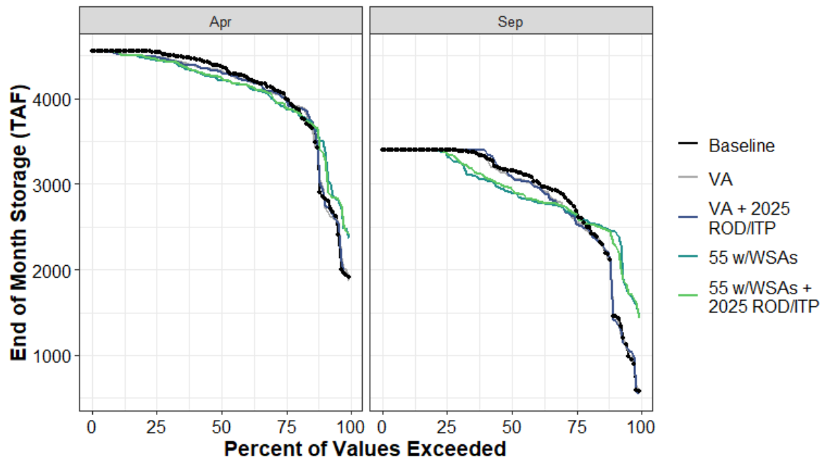
Figure H1a7-143. Shasta Lake End of April and End of September Storage (TAF) Percent Exceedance Plot
