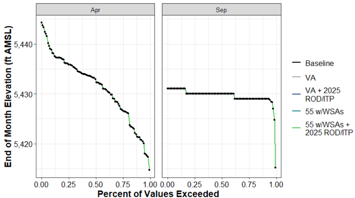
Figure H1a7-98. Ice House Reservoir End-of-April and End-of-September Elevation (ft AMSL) Percent Exceedance Plot
