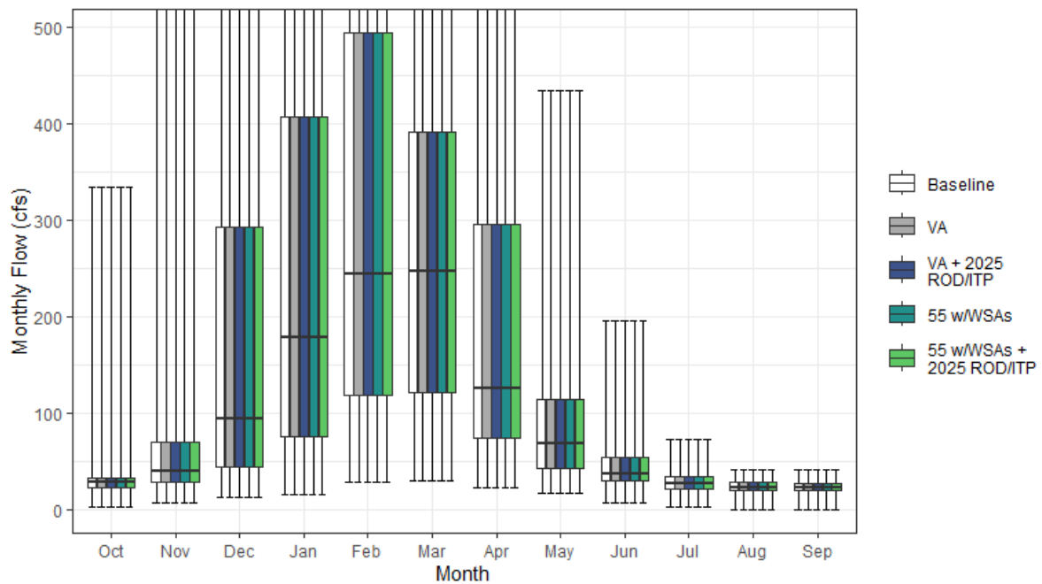
Figure H1a7-7. Big Chico Creek Streamflow above Confluence with Sacramento River Monthly Boxplot (cfs)
