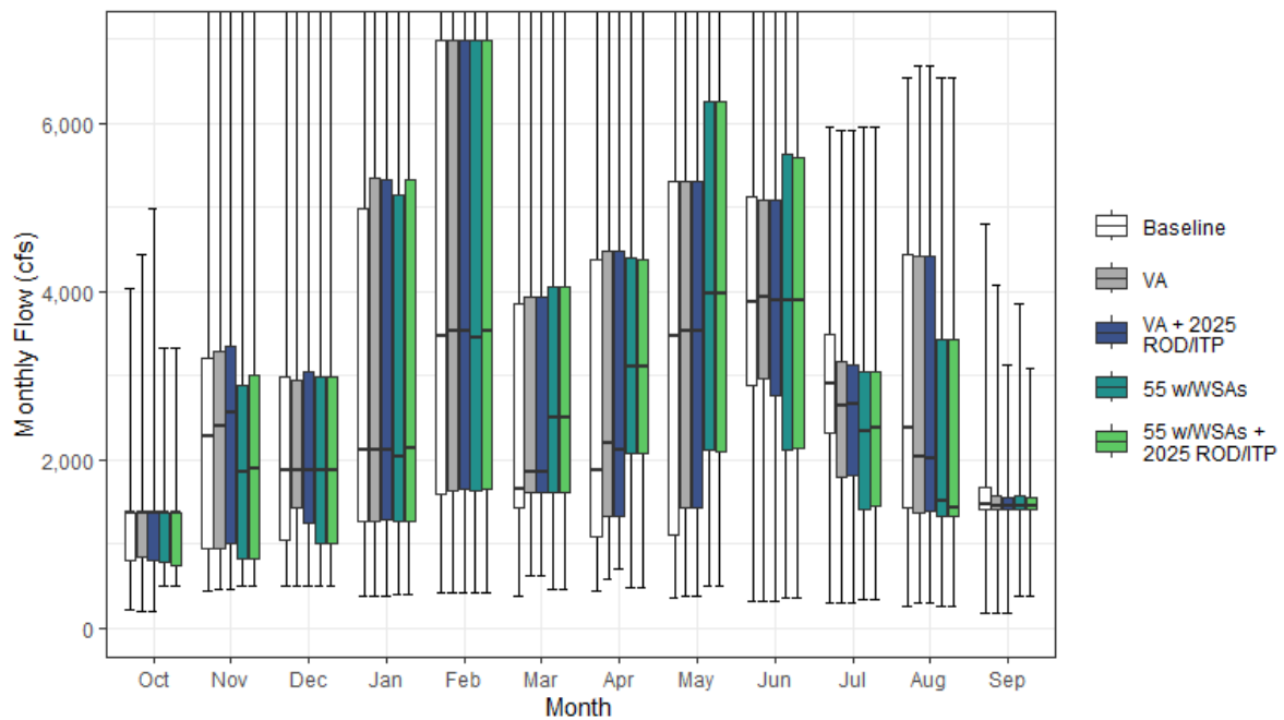
Figure H1a7-2. American River Streamflow above Confluence with Sacramento River Monthly Boxplot (cfs)
