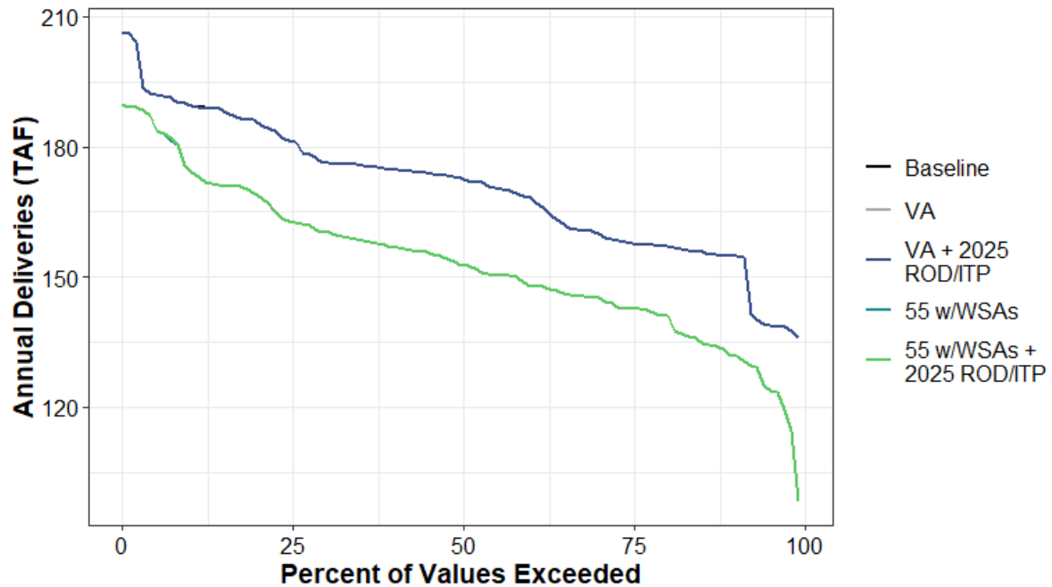
Figure H1a7-191. Total Water Supplied to Water Budget Area 24 (Agricultural) Annual Percent Exceedance Plot.
