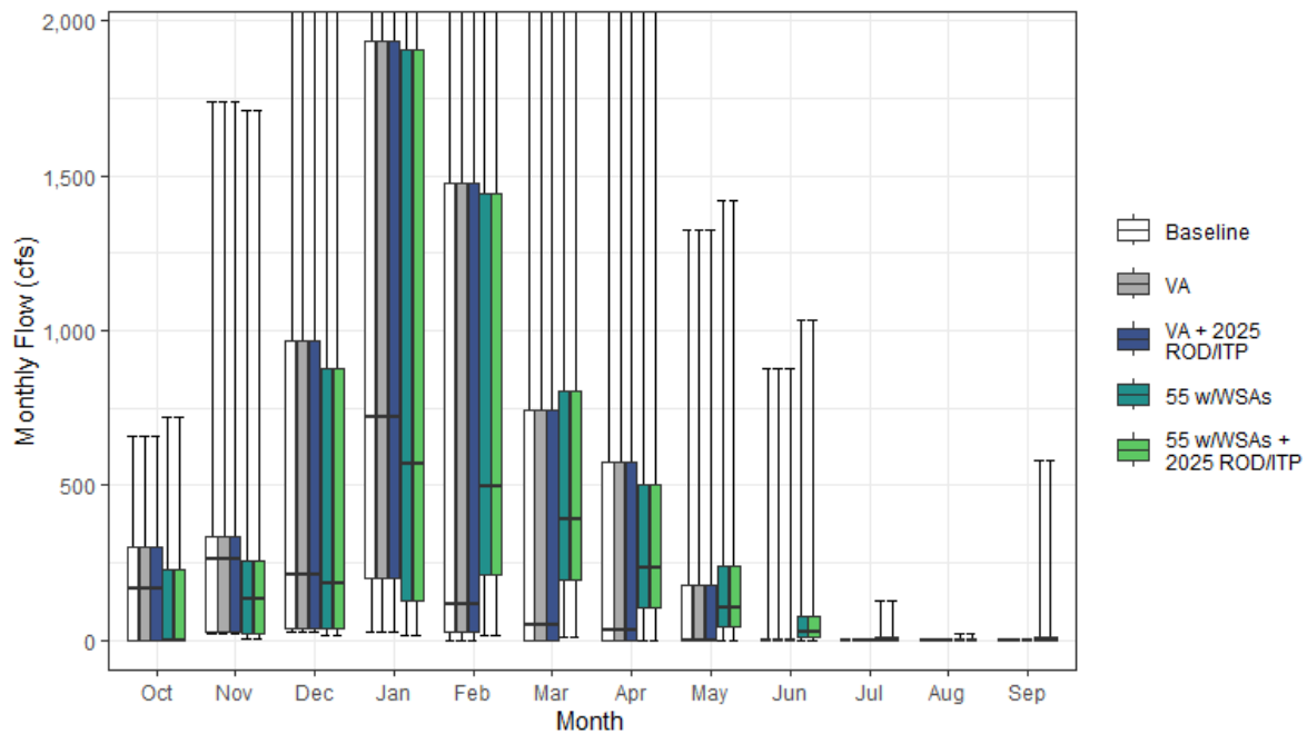
Figure H1a7-35. Stony Creek Streamflow above Confluence with Sacramento River Monthly Boxplot (cfs)
