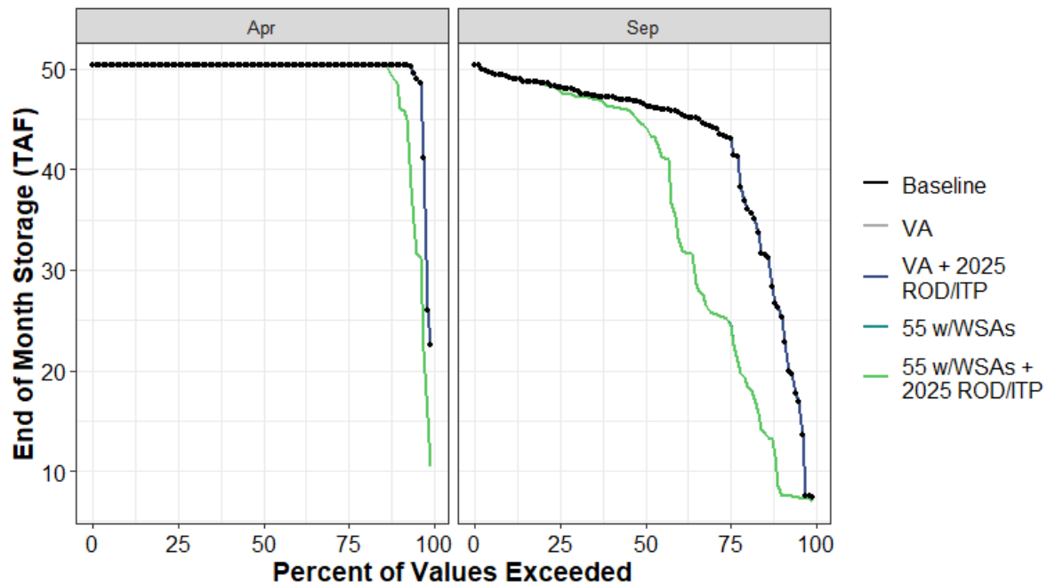
Figure H1a7-149. Stony Gorge Reservoir End of April and End of September Storage (TAF) Percent Exceedance Plot
