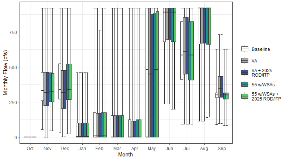
Figure H1a7-55. Hell Hole Tunnel Monthly Boxplot (cfs)
