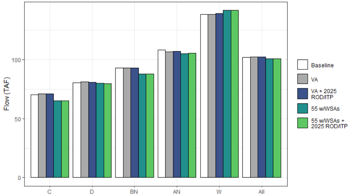
Figure H1a7-238. Total Average Annual Stream-Groundwater Flux (Net Groundwater Gain) for Delta Eastside Tributaries Region by WYT and Scenario (TAF/yr).
