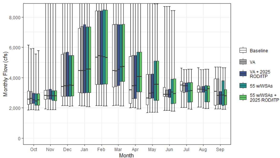
Figure H1a7-48. Georgiana Slough Monthly Boxplot (cfs)
