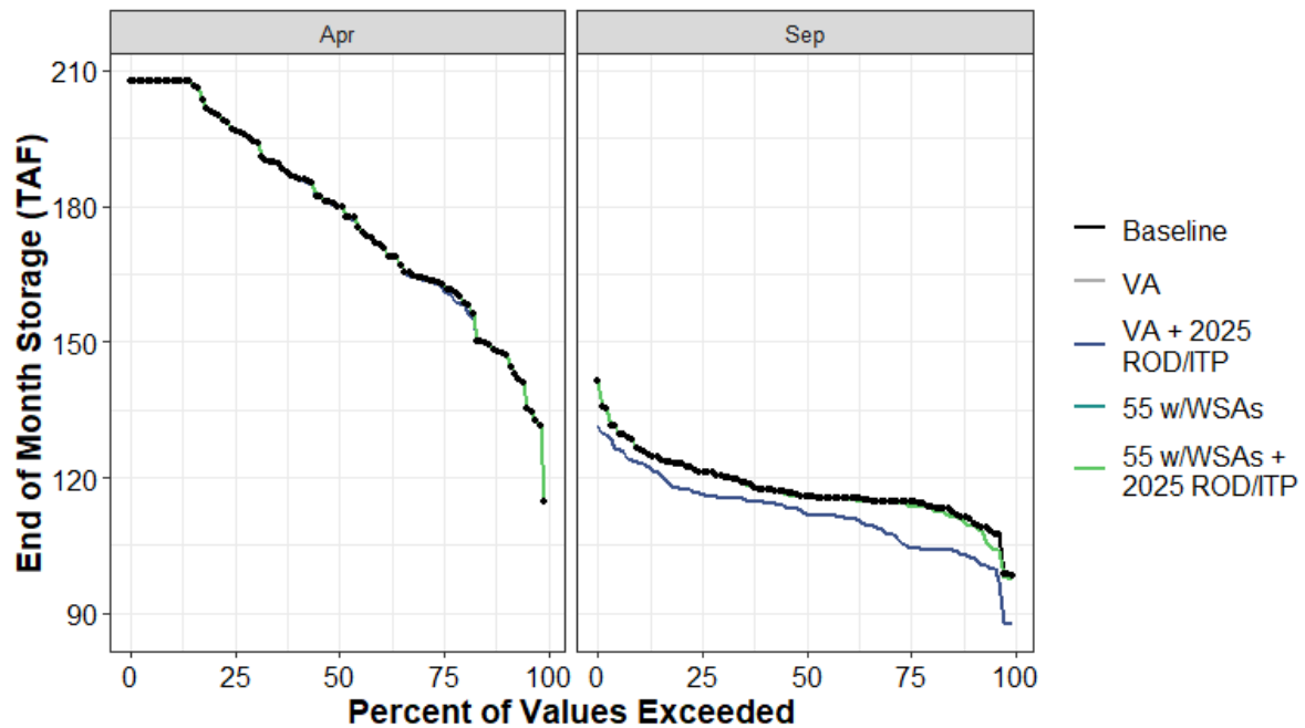
Figure H1a7-95. Hell Hole End of April and End of September Storage (TAF) Percent Exceedance Plot
