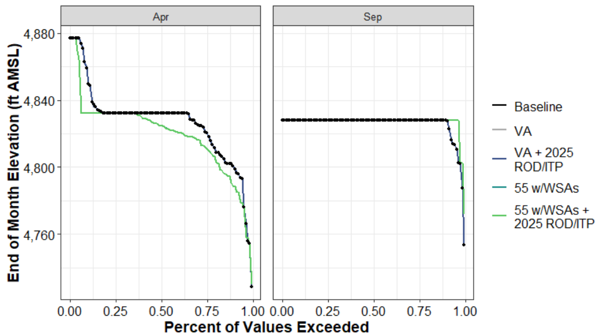
Figure H1a7-115. Lake Spaulding Reservoir End-of-April and End-of-September Elevation (ft AMSL) Percent Exceedance Plot
