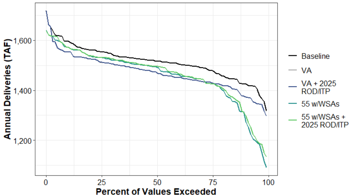
Figure H1a7-168. Total Water Supplied to Water Budget Area 8 (Agricultural) Annual Percent Exceedance Plot.
