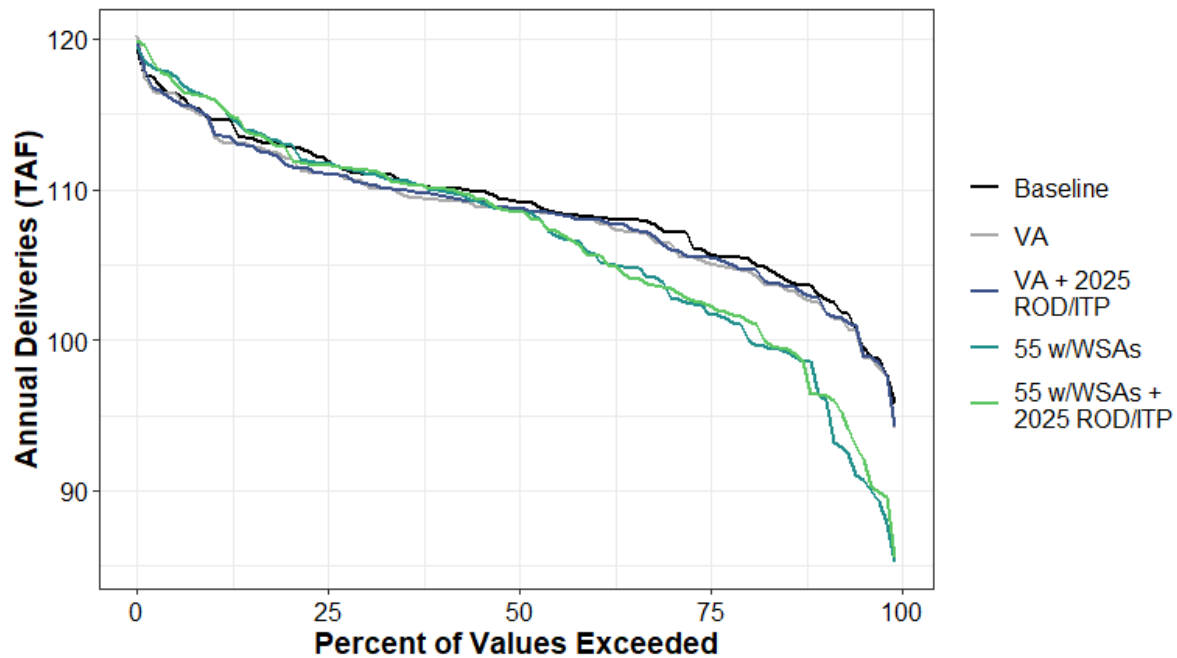
Figure H1a7-182. Total Water Supplied to Water Budget Area 17 (Agricultural) Annual Percent Exceedance Plot.
