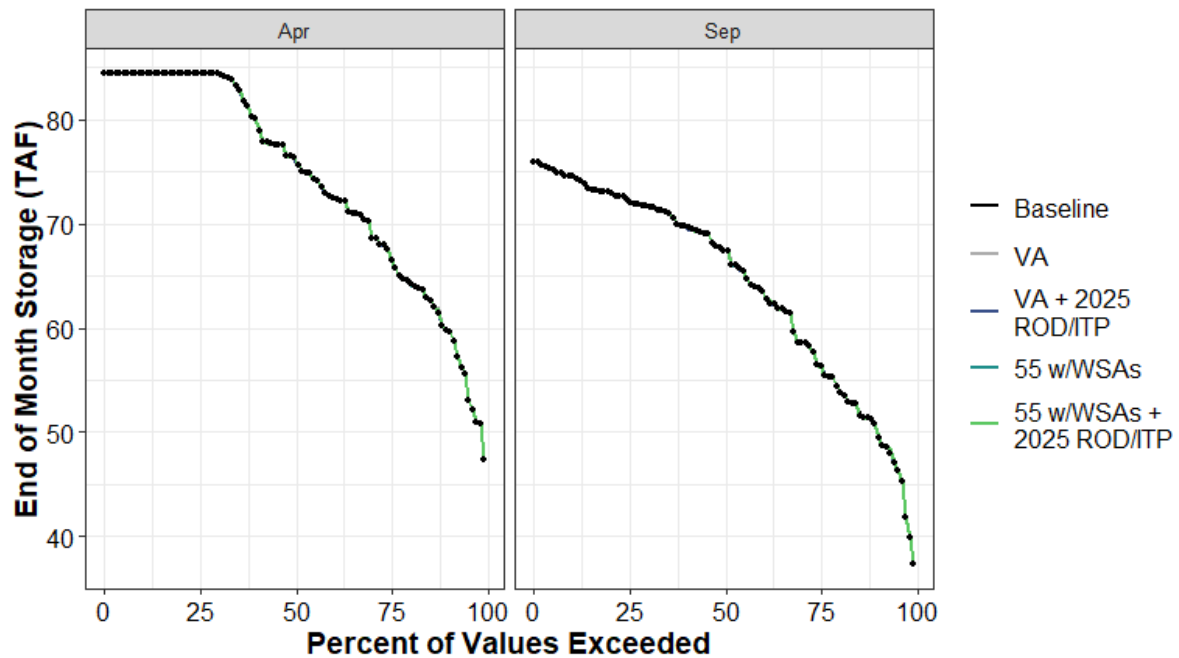
Figure H1a7-110. Lake Davis End of April and End of September Storage (TAF) Percent Exceedance Plot
