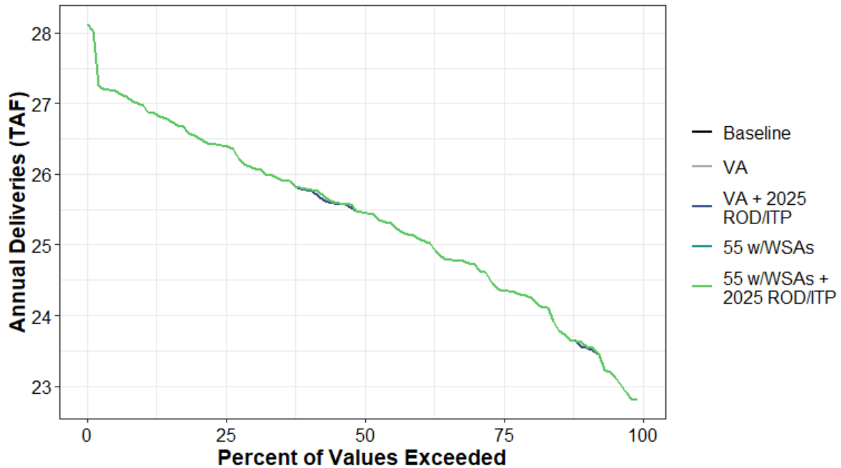
Figure H1a7-174. Total Water Supplied to Water Budget Area 11 (Refuge) Annual Percent Exceedance Plot.
