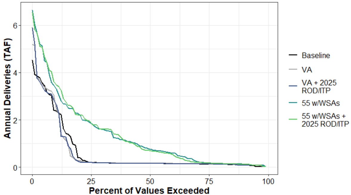
Figure H1a7-228. Surface Water Supplied to SWP Settlement (Urban) Annual Percent Exceedance Plot.
