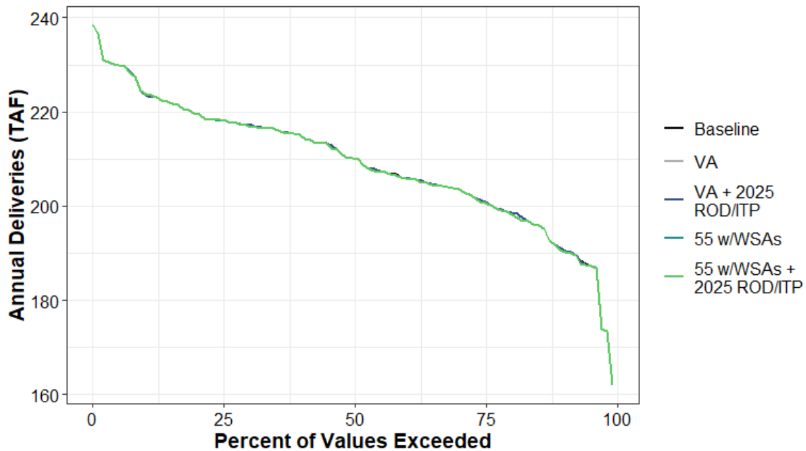
Figure H1a7-172. Total Water Supplied to Water Budget Area 10 (Agricultural) Annual Percent Exceedance Plot.
