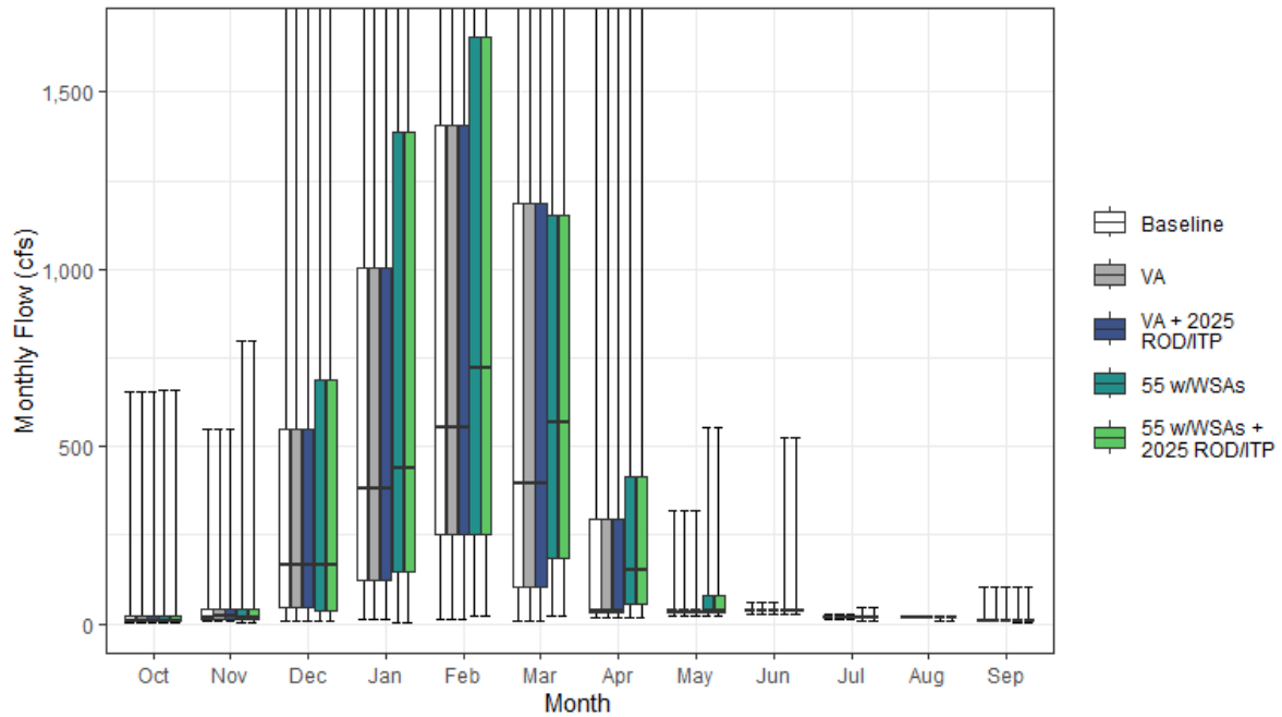
Figure H1a7-10. Cache Creek Streamflow above Yolo Bypass Monthly Boxplot (cfs)
