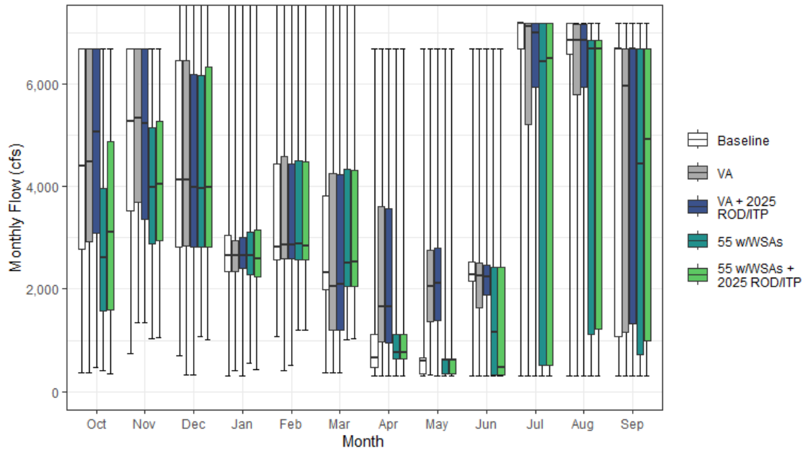
Figure H1a7-52. Banks Pumping Plant (SWP) Monthly Boxplot (cfs)
