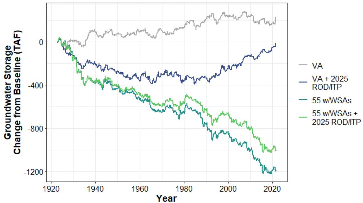
Figure H1a7-249. Sutter-Yuba Groundwater Basin End of Year Storage—Change from Baseline
