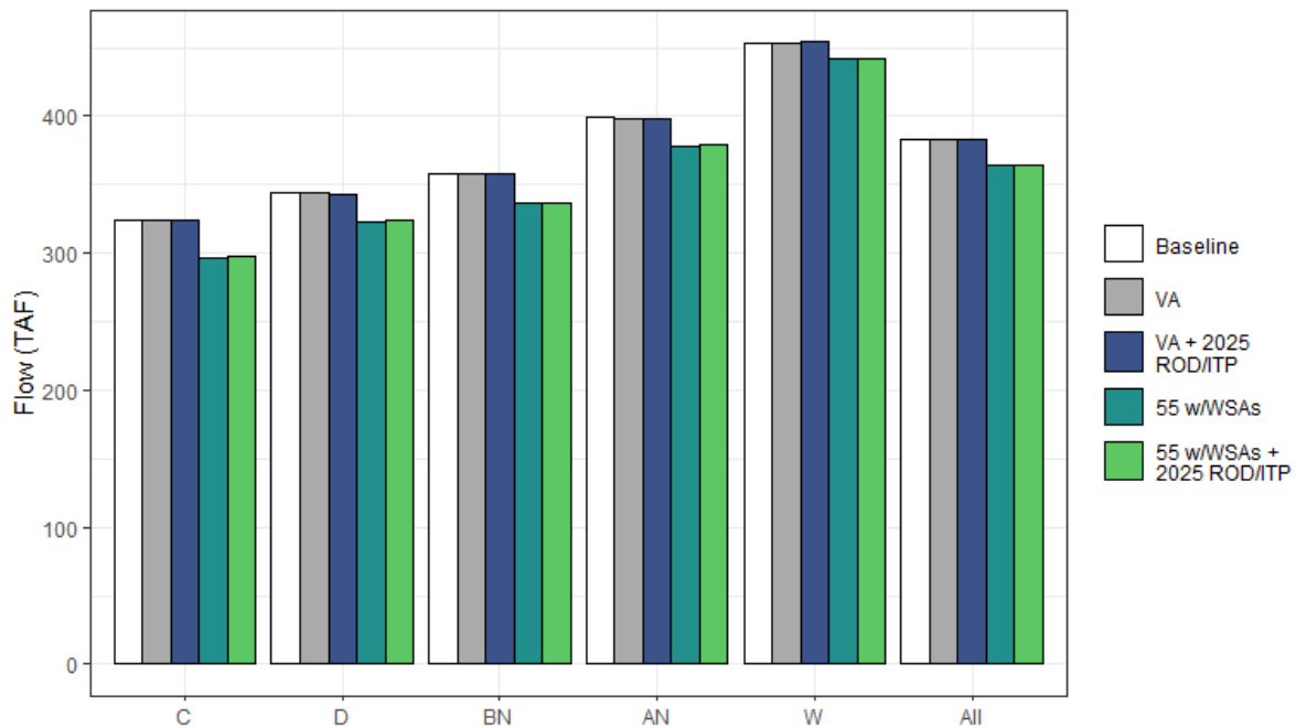
Figure H1a7-234. Total Average Annual Groundwater Recharge for the Delta Eastside Tributaries Region by WYT and Scenario (TAF/yr).
