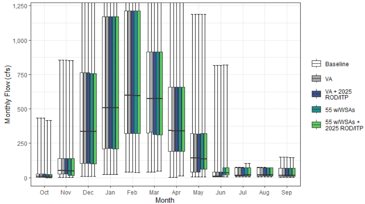
Figure H1a7-37. Thomes Creek Streamflow above Confluence with Sacramento River Monthly Boxplot (cfs)
