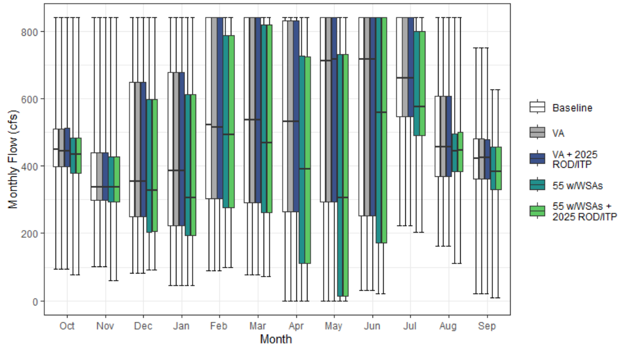
Figure H1a7-54. Drum Canal Monthly Boxplot (cfs)
