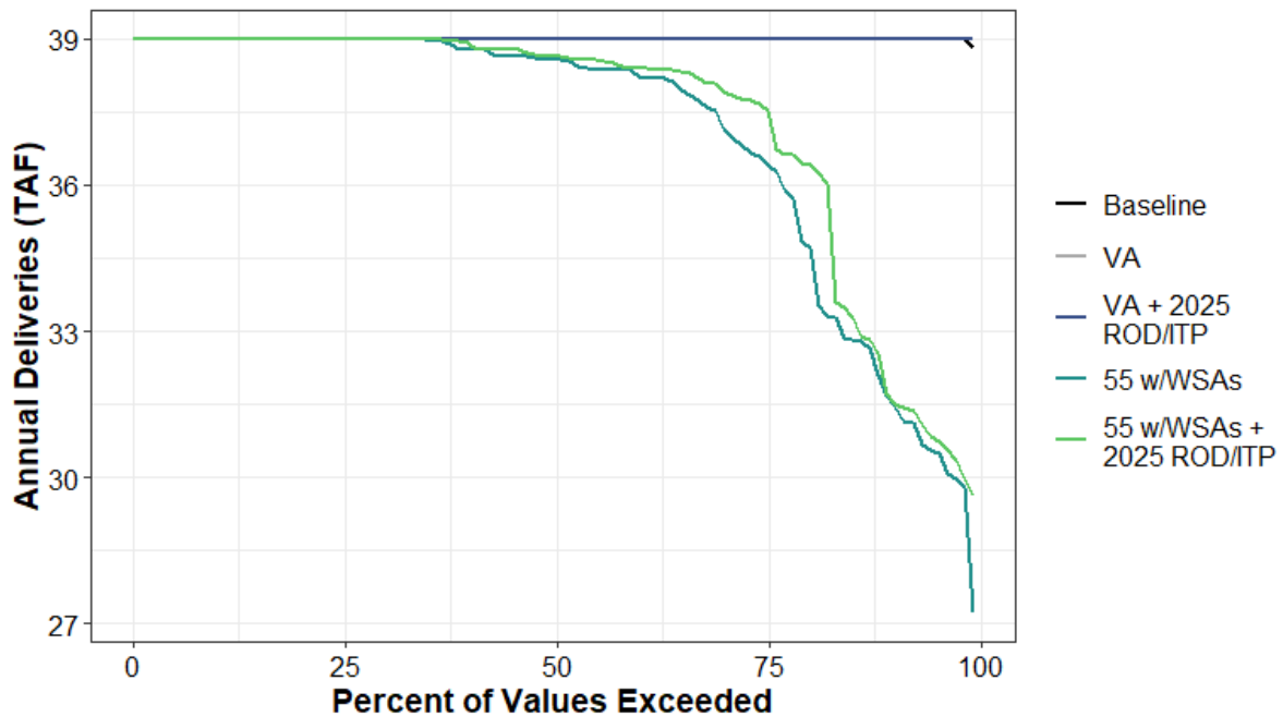
Figure H1a7-164. Total Water Supplied to Water Budget Area 3 (Urban) Annual Percent Exceedance Plot.
