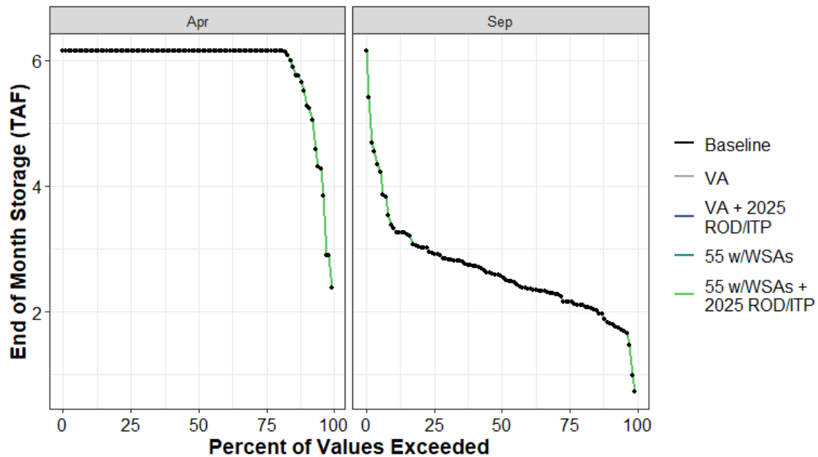
Figure H1a7-136. Philbrook Round Valley End of April and End of September Storage (TAF) Percent Exceedance Plot
