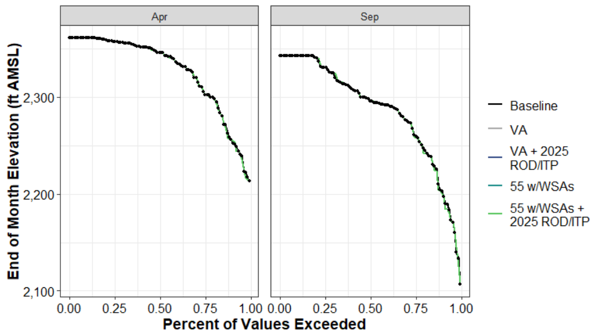
Figure H1a7-156. Trinity Reservoir End-of-April and End-of-September Elevation (ft AMSL) Percent Exceedance Plot
