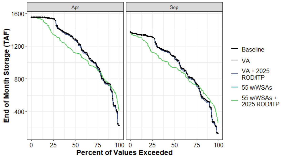
Figure H1a7-108. Lake Berryessa End of April and End of September Storage (TAF) Percent Exceedance Plot
