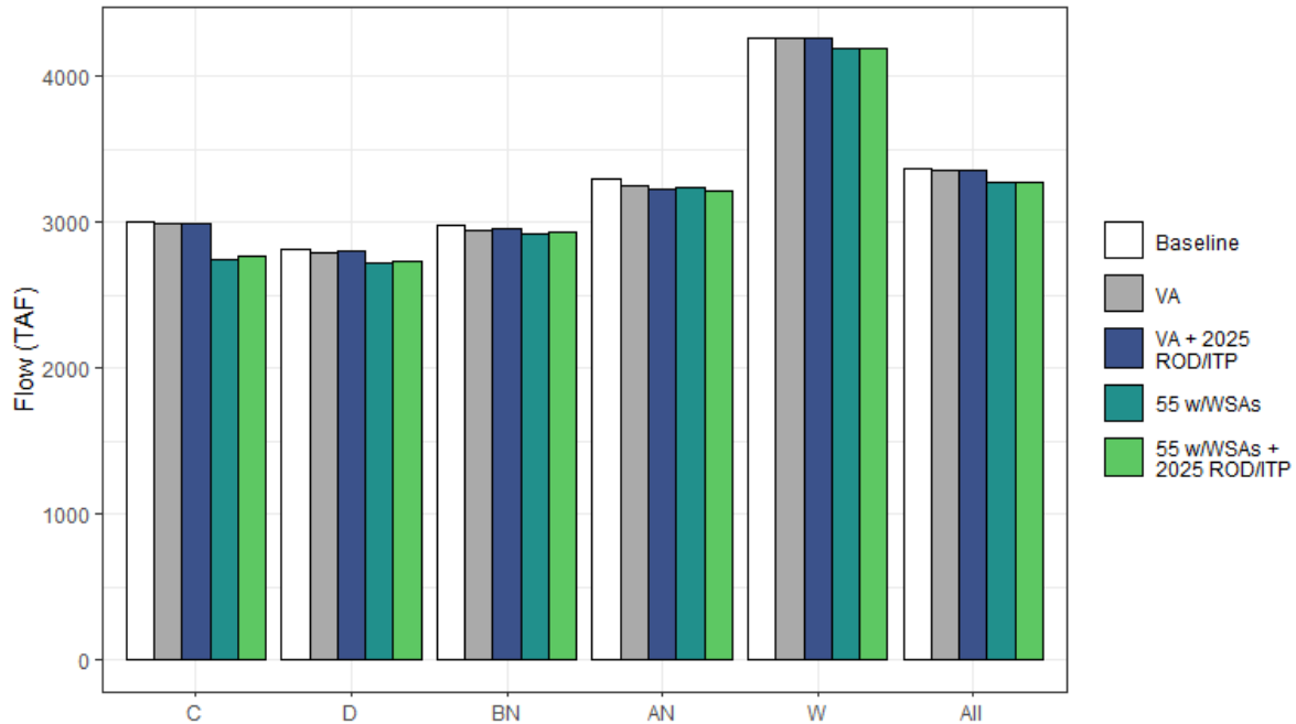
Figure H1a7-233. Total Average Annual Groundwater Recharge by WYT and Scenario (TAF/yr).
