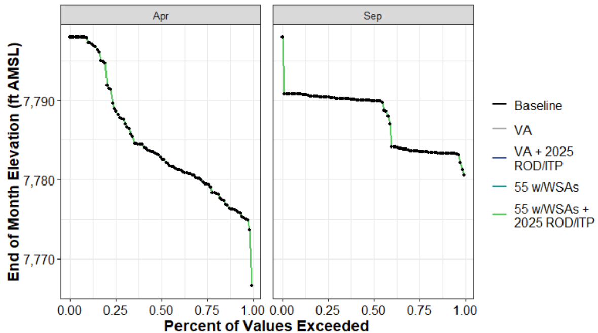
Figure H1a7-82. Caples Lake Reservoir End-of-April and End-of-September Elevation (ft AMSL) Percent Exceedance Plot
