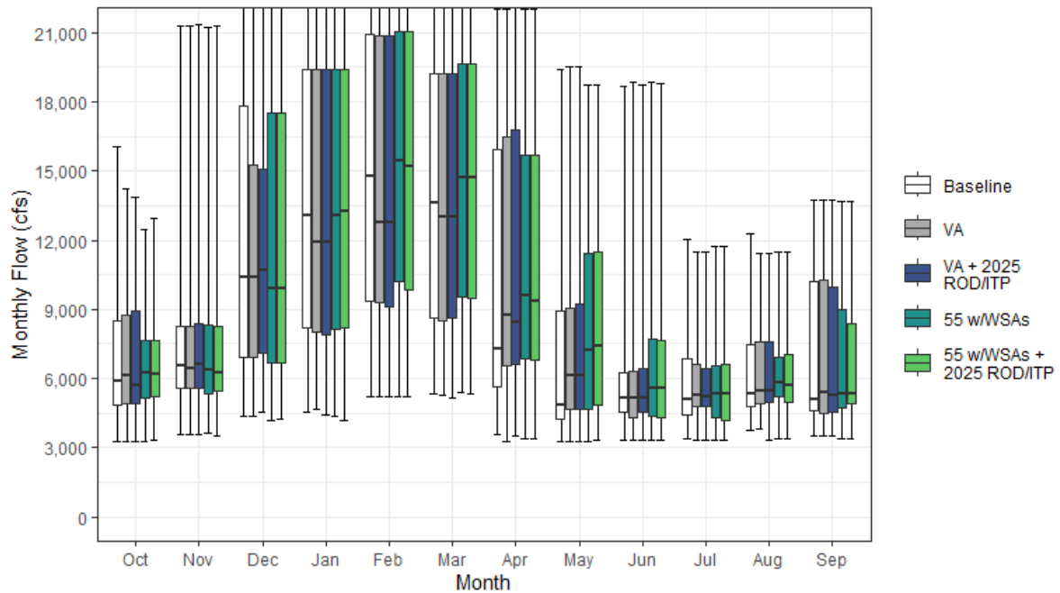
Figure H1a7-31. Sacramento River Streamflow at Knights Landing Monthly Boxplot (cfs)
