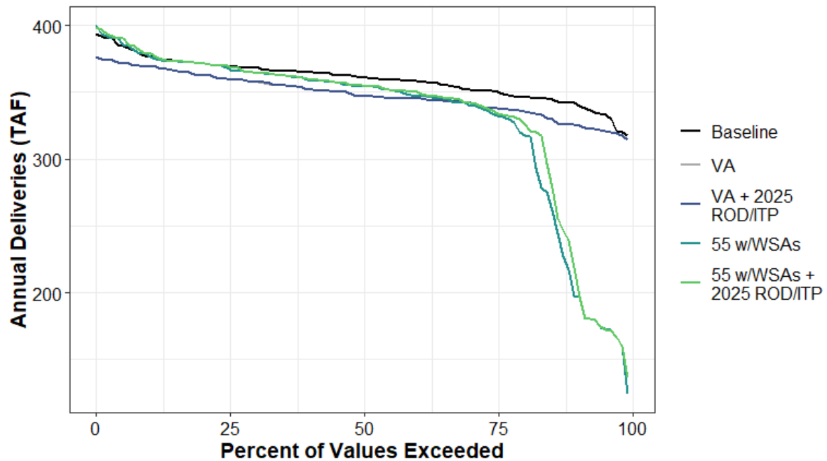
Figure H1a7-184. Total Water Supplied to Water Budget Areas 18 and 19 (Agricultural) Annual Percent Exceedance Plot.
