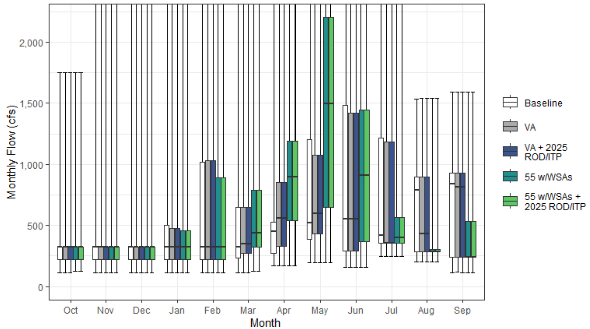
Figure H1a7-23. Mokelumne River Streamflow below Camanche Reservoir Monthly Boxplot (cfs)
