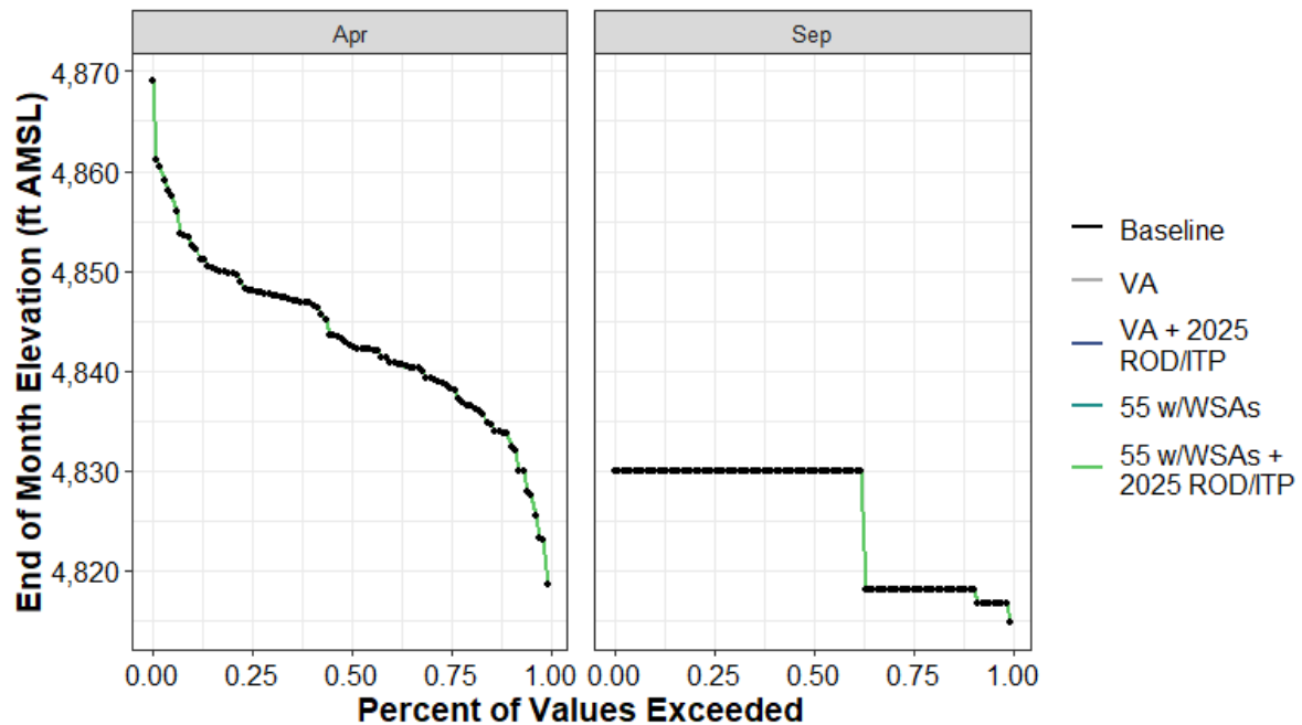
Figure H1a7-158. Union Valley Reservoir End-of-April and End-of-September Elevation (ft AMSL) Percent Exceedance Plot
