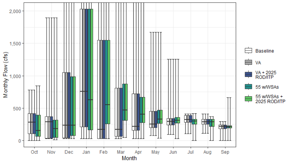
Figure H1a7-34. Stony Creek Streamflow below Black Butte Reservoir Monthly Boxplot (cfs)
