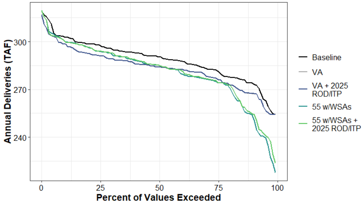
Figure H1a7-170. Total Water Supplied to Water Budget Area 9 (Agricultural) Annual Percent Exceedance Plot.
