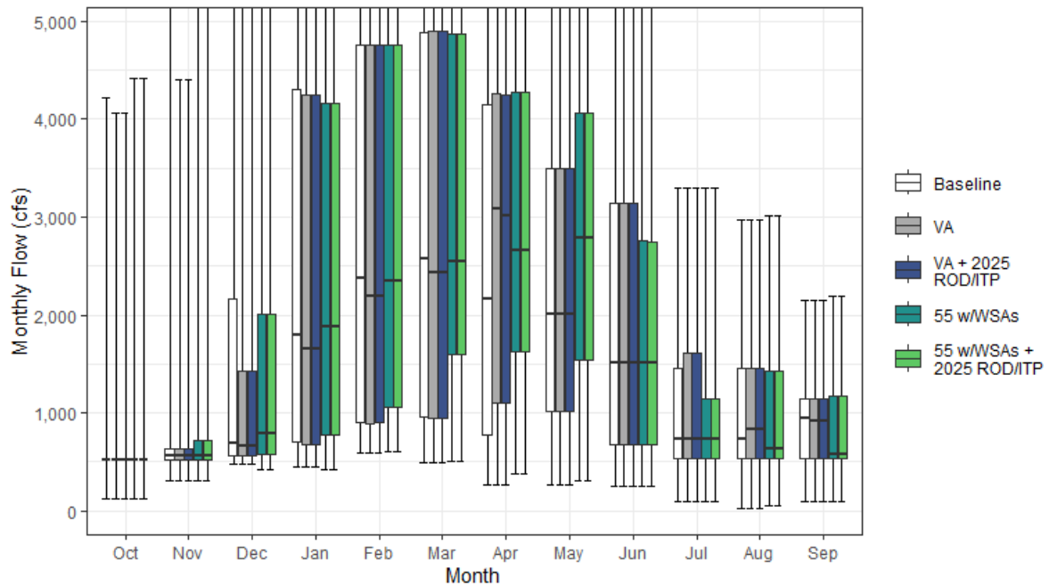
Figure H1a7-44. Yuba River Streamflow above Confluence with Feather River Monthly Boxplot (cfs)
