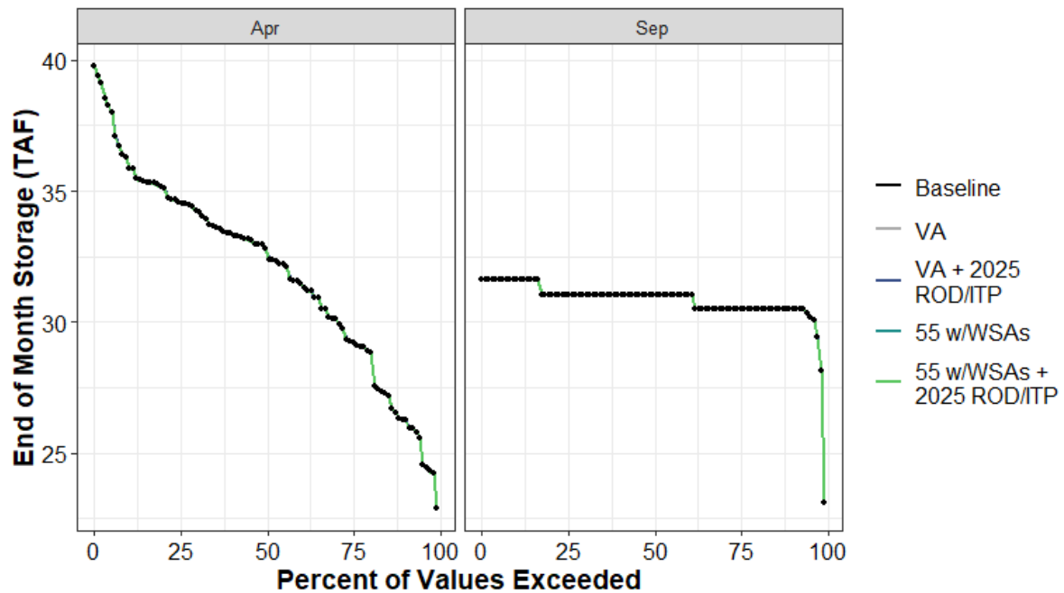
Figure H1a7-97. Ice House End of April and End of September Storage (TAF) Percent Exceedance Plot
