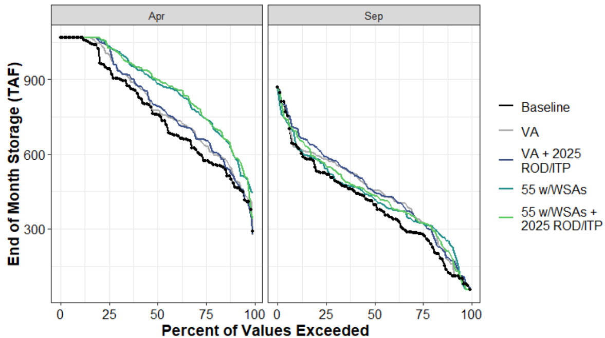
Figure H1a7-152. SWP San Luis Reservoir End of April and End of September Storage (TAF) Percent Exceedance Plot
