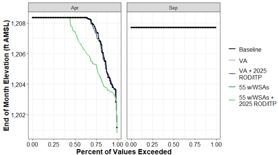
Figure H1a7-160. Whiskeytown Reservoir End-of-April and End-of-September Elevation (ft AMSL) Percent Exceedance Plot
