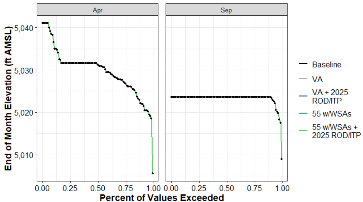
Figure H1a7-118. Little Grass Valley Reservoir End-of-April and End-of-September Elevation (ft AMSL) Percent Exceedance Plot
