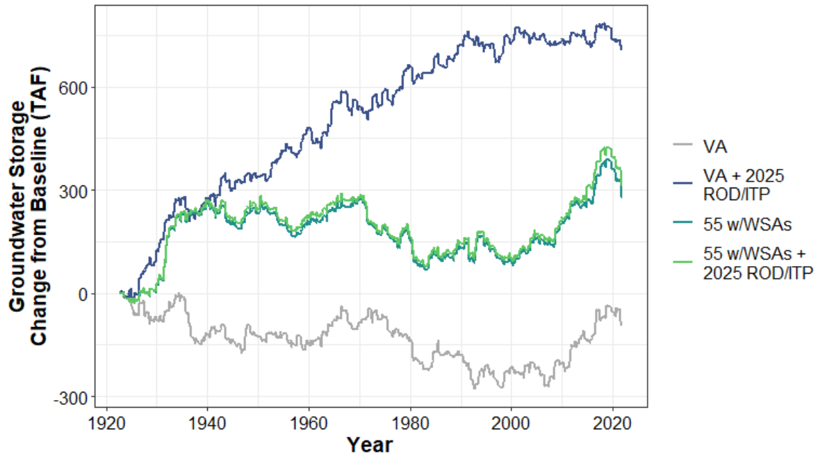
Figure H1a7-242. Butte Groundwater Basin End of Year Storage—Change from Baseline (TAF)
