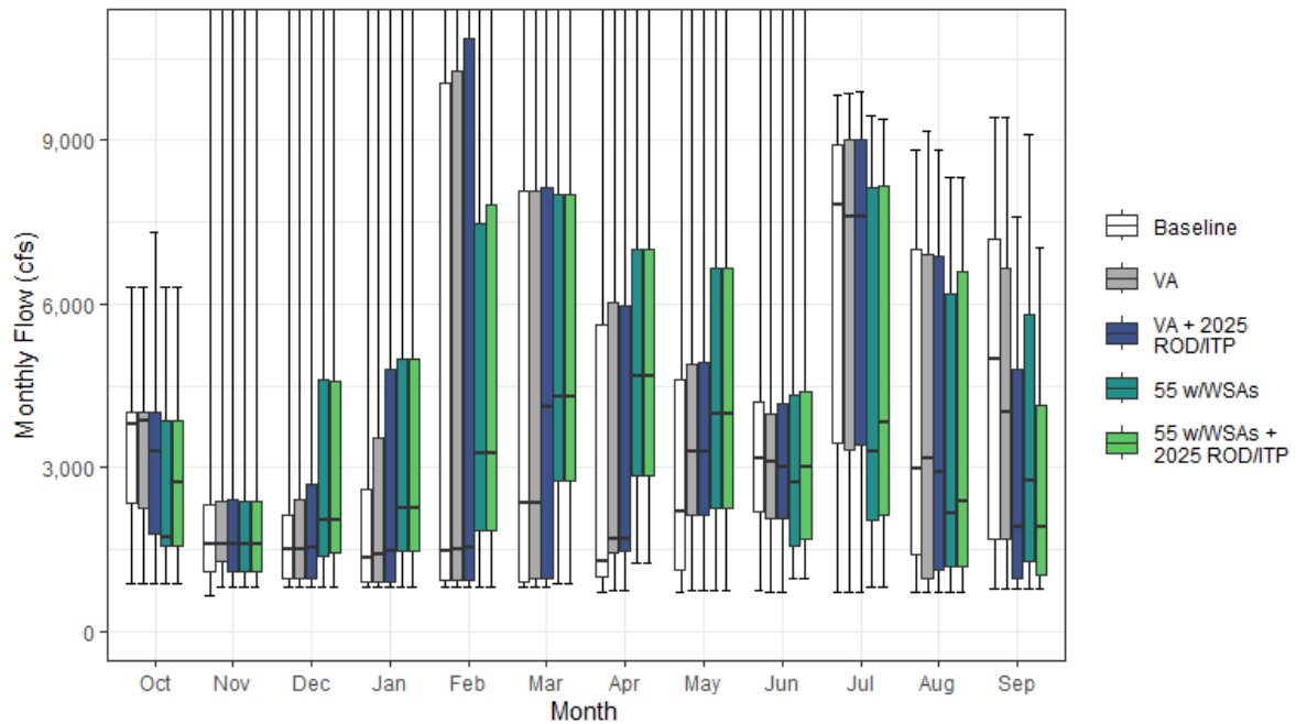
Figure H1a7-19. Feather River Streamflow below Oroville Reservoir Monthly Boxplot (cfs)
