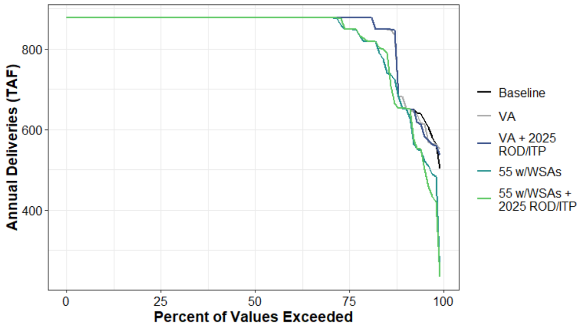
Figure H1a7-216. Surface Water Supplied to CVP SOD Exchange Annual Percent Exceedance Plot.
