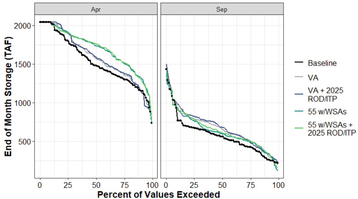
Figure H1a7-153. Total San Luis Reservoir End of April and End of September Storage (TAF) Percent Exceedance Plot
