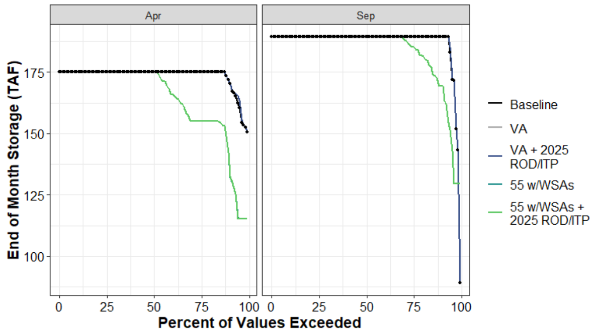
Figure H1a7-134. Pardee Reservoir End of April and End of September Storage (TAF) Percent Exceedance Plot
