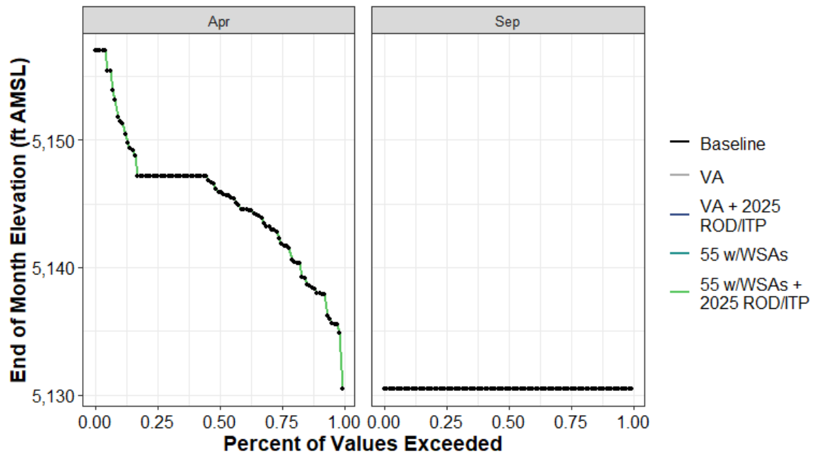
Figure H1a7-74. Bucks Lake Reservoir End-of-April and End-of-September Elevation (ft AMSL) Percent Exceedance Plot
