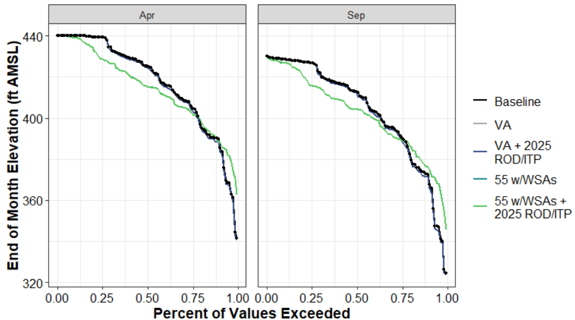
Figure H1a7-109. Lake Berryessa Reservoir End-of-April and End-of-September Elevation (ft AMSL) Percent Exceedance Plot
