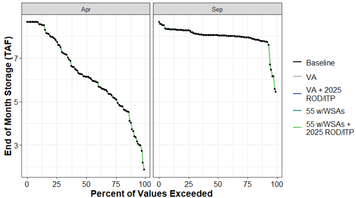
Figure H1a7-145. Silver Lake End of April and End of September Storage (TAF) Percent Exceedance Plot
