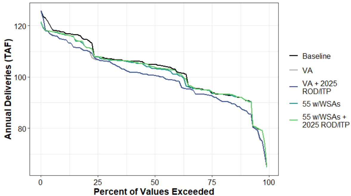
Figure H1a7-161. Total Water Supplied to Water Budget Area 2 (Agricultural) Annual Percent Exceedance Plot.
