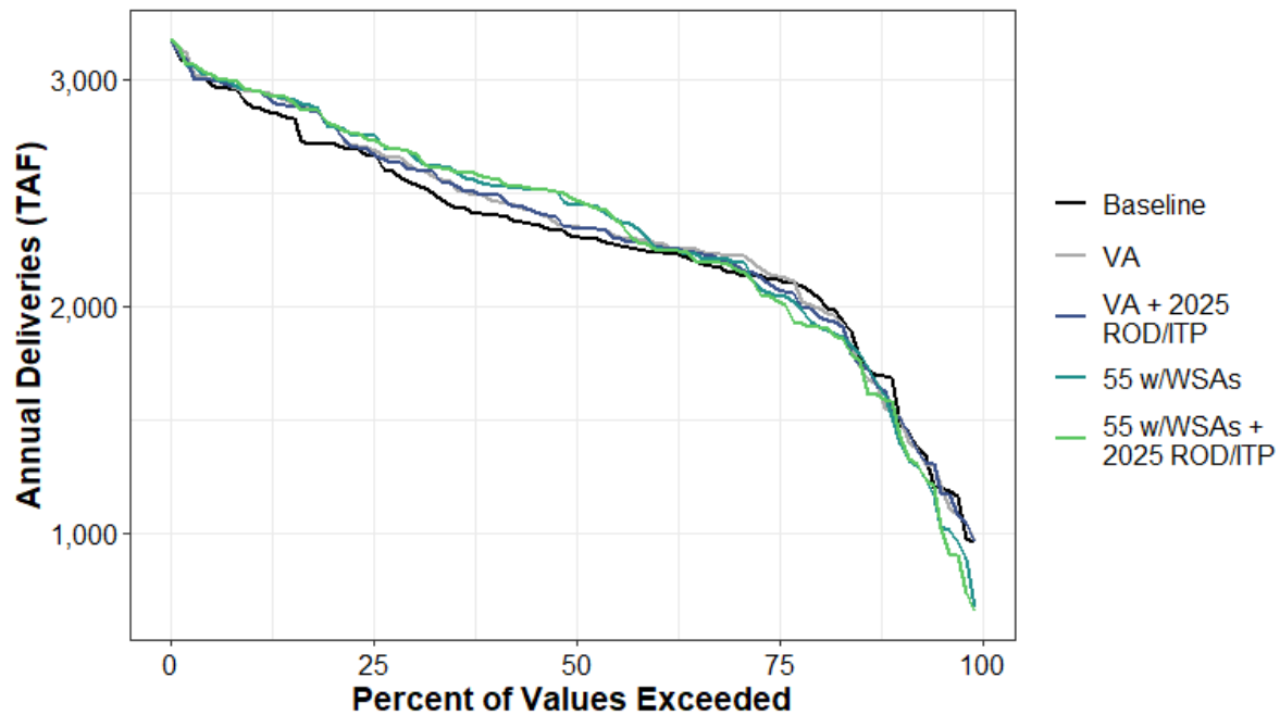
Figure H1a7-213. Surface Water Supplied to Total CVP South of Delta Annual Percent Exceedance Plot.
