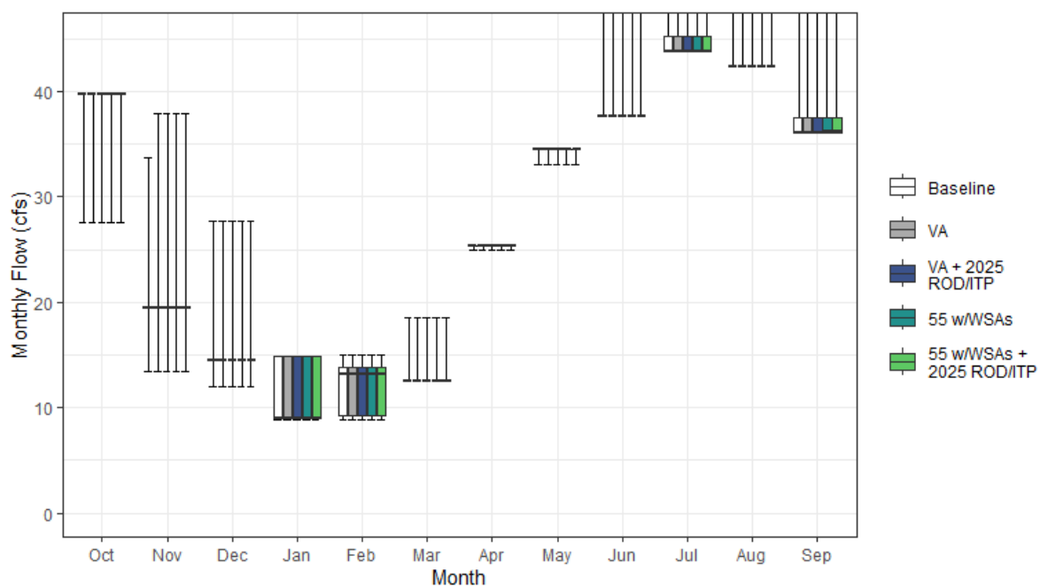
Figure H1a7-56. Jenkinson Lake Camino Conduit Monthly Boxplot (cfs)
