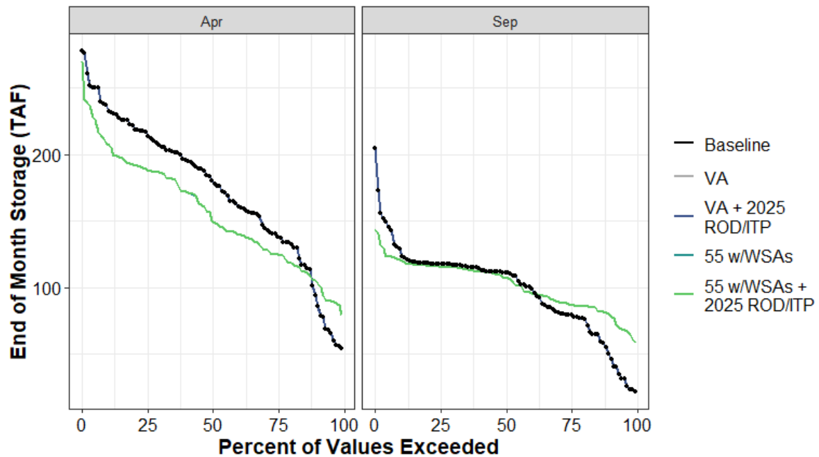
Figure H1a7-130. New Hogan Reservoir End of April and End of September Storage (TAF) Percent Exceedance Plot
