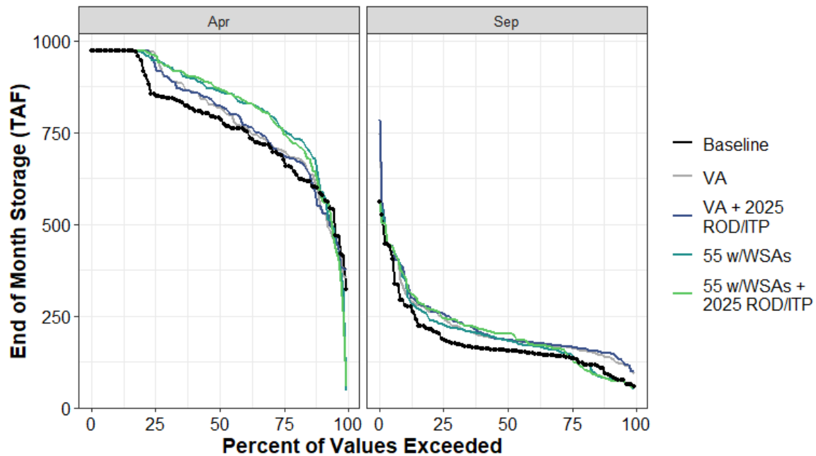
Figure H1a7-85. CVP San Luis Reservoir End of April and End of September Storage (TAF) Percent Exceedance Plot
