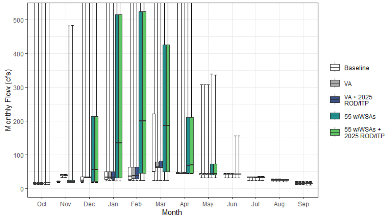
Figure H1a7-27. Putah Creek Streamflow above Yolo Bypass Monthly Boxplot (cfs)
