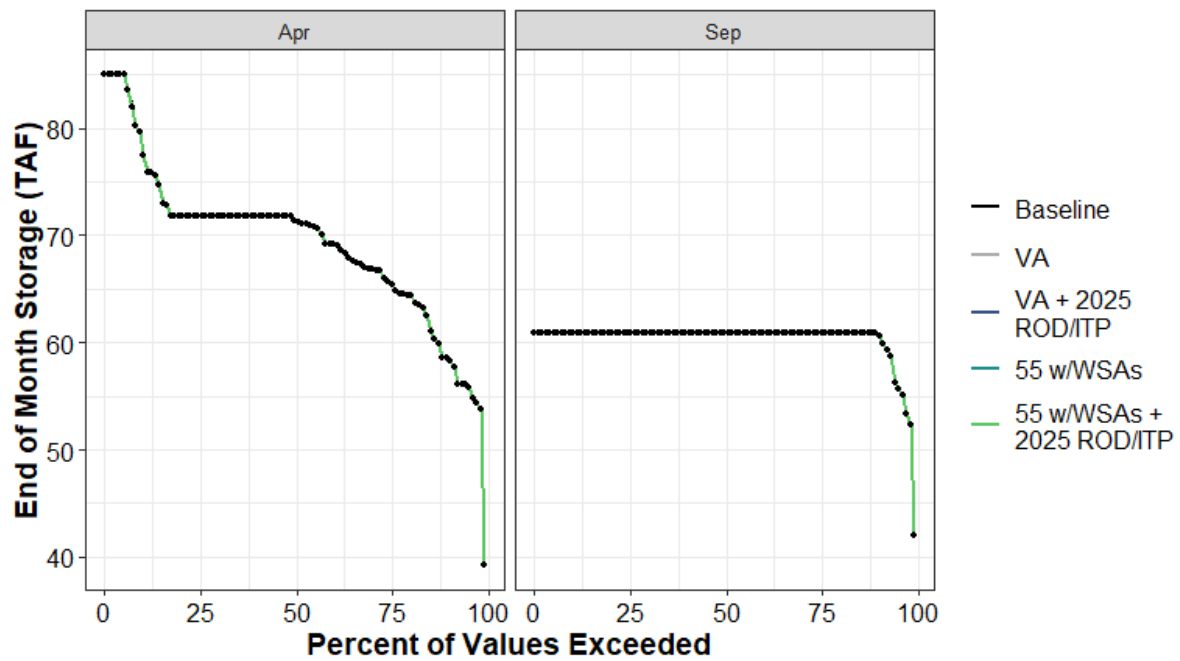
Figure H1a7-117. Little Grass Valley Reservoir End of April and End of September Storage (TAF) Percent Exceedance Plot
