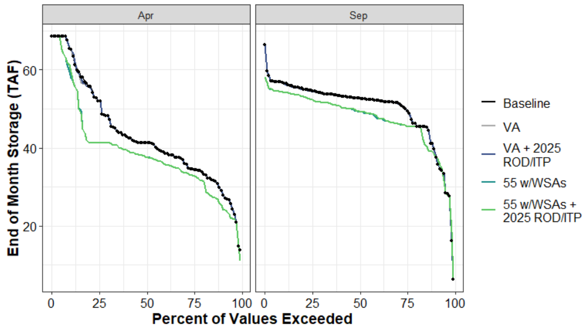
Figure H1a7-71. Bowman Lake End of April and End of September Storage (TAF) Percent Exceedance Plot
