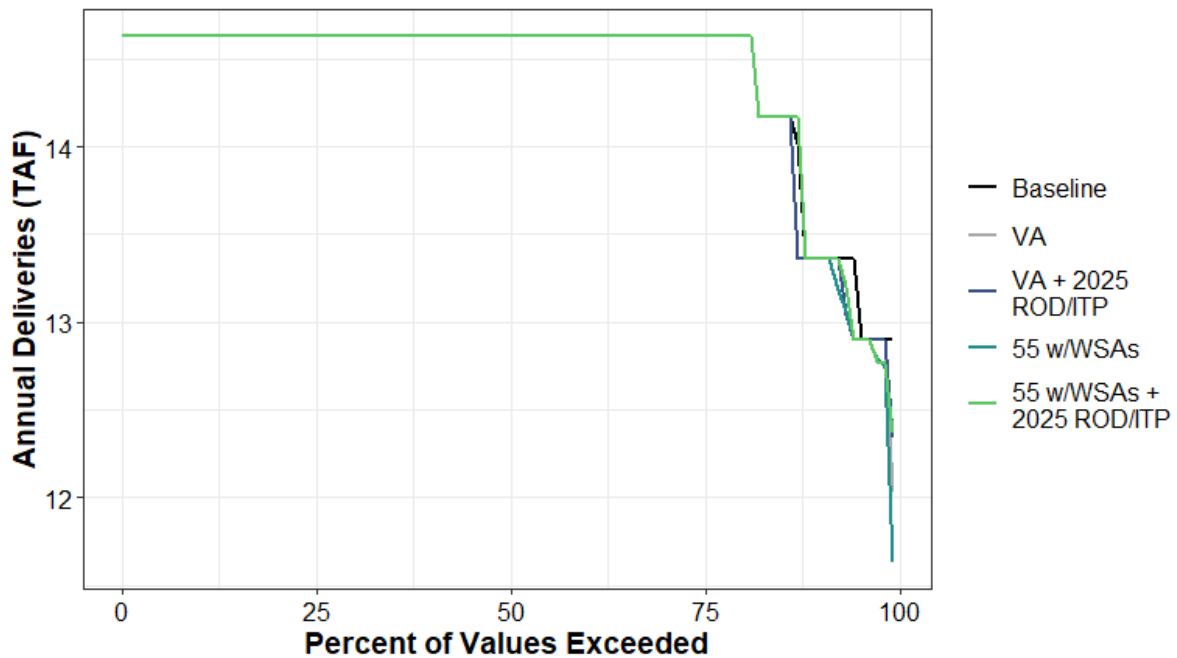
Figure H1a7-211. Surface Water Supplied to CVP Settlement (M&I) Annual Percent Exceedance Plot.
