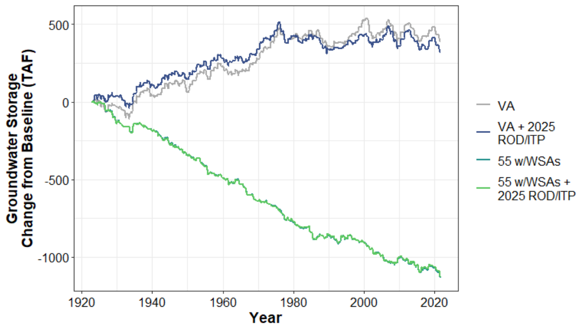
Figure H1a7-241. American River Groundwater Basin End of Year Storage—Change from Baseline (TAF)
