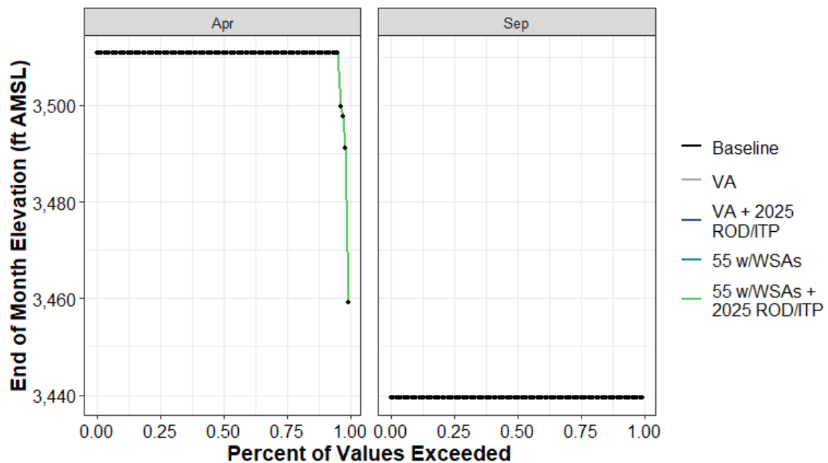
Figure H1a7-148. Sly Creek Reservoir End-of-April and End-of-September Elevation (ft AMSL) Percent Exceedance Plot
