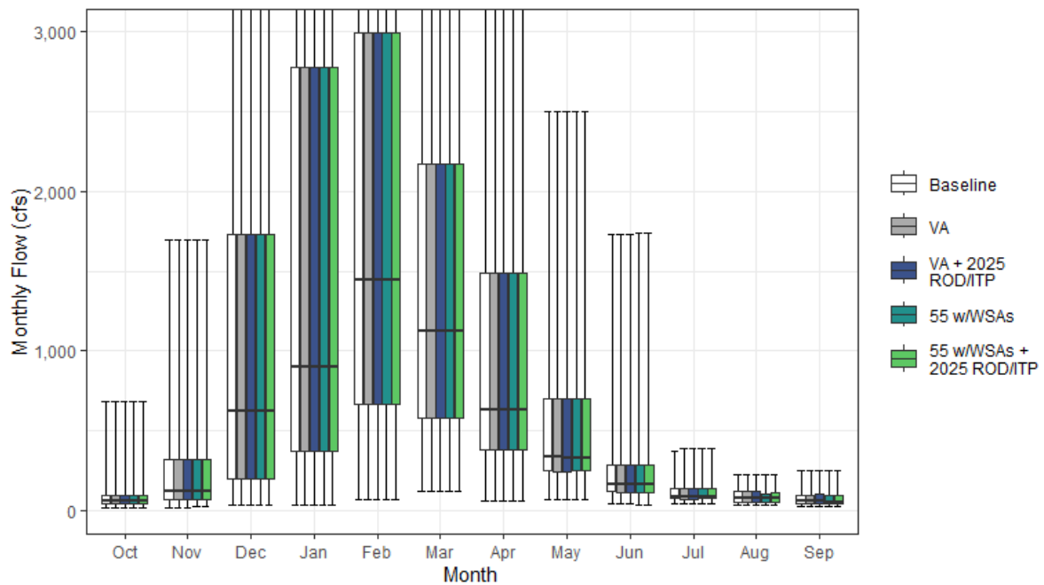
Figure H1a7-15. Cottonwood Creek Streamflow above Confluence with Sacramento River Monthly Boxplot (cfs)
