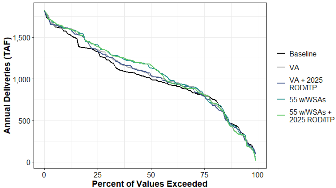
Figure H1a7-214. Surface Water Supplied to CVP South of Delta Water Service (Agricultural) Annual Percent Exceedance Plot.
