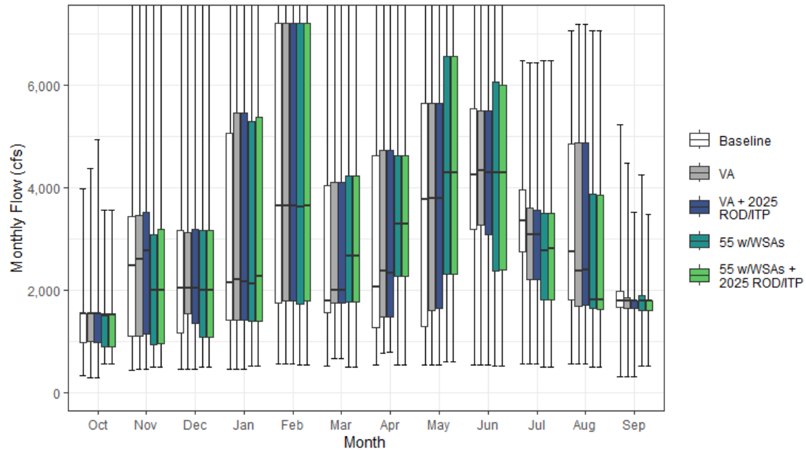
Figure H1a7-1. American River Streamflow below Folsom Reservoir Monthly Boxplot (cfs)
