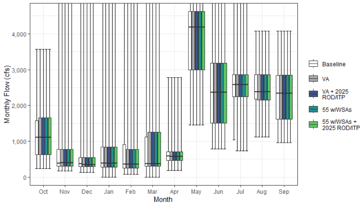
Figure H1a7-38. Trinity River Streamflow below Lewiston Reservoir Monthly Boxplot (cfs)
