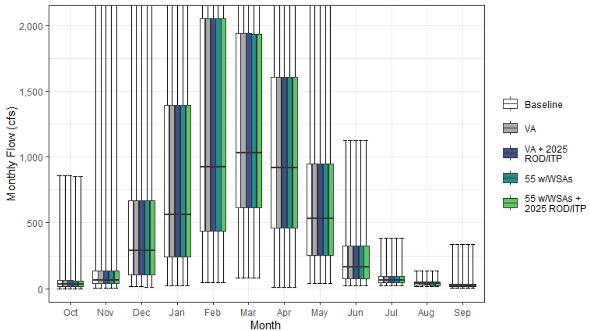
Figure H1a7-14. Cosumnes River Streamflow above Confluence with Delta Monthly Boxplot (cfs)
