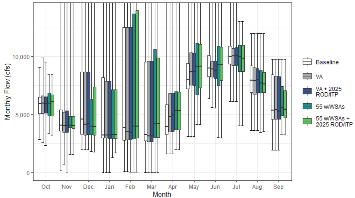
Figure H1a7-28. Sacramento River Streamflow below Shasta Reservoir Monthly Boxplot (cfs)
