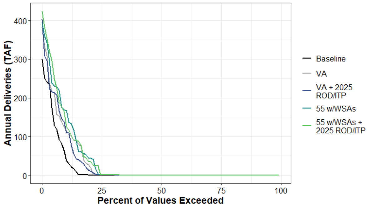
Figure H1a7-223. Surface Water Supplied to SWP Article 21 Central Coast and Tulare Annual Percent Exceedance Plot.
