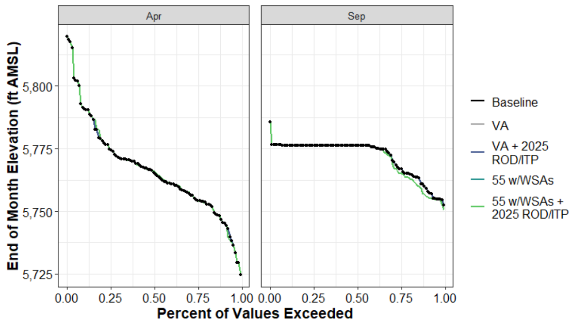
Figure H1a7-124. Lower Bear Reservoir End-of-April and End-of-September Elevation (ft AMSL) Percent Exceedance Plot
