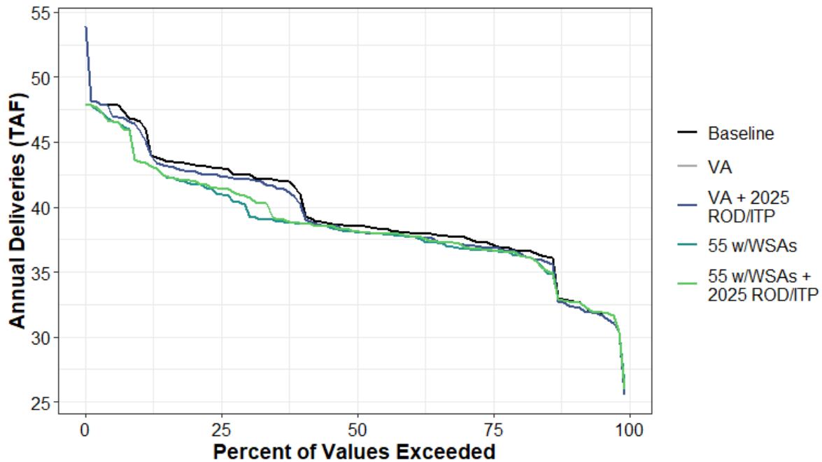
Figure H1a7-163. Total Water Supplied to Water Budget Area 3 (Agricultural) Annual Percent Exceedance Plot.
