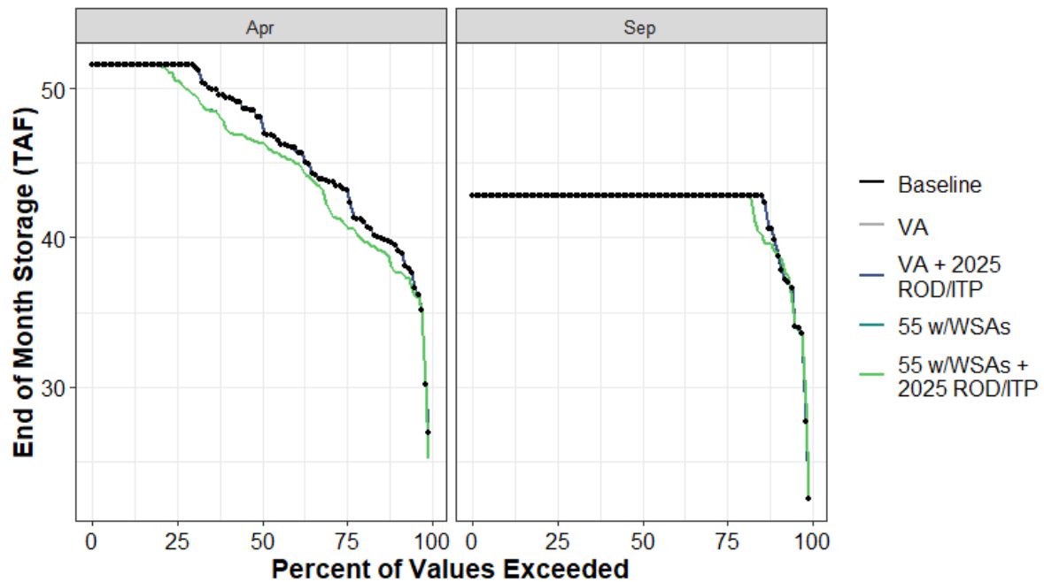
Figure H1a7-101. Jackson Meadows Reservoir End of April and End of September Storage (TAF) Percent Exceedance Plot
