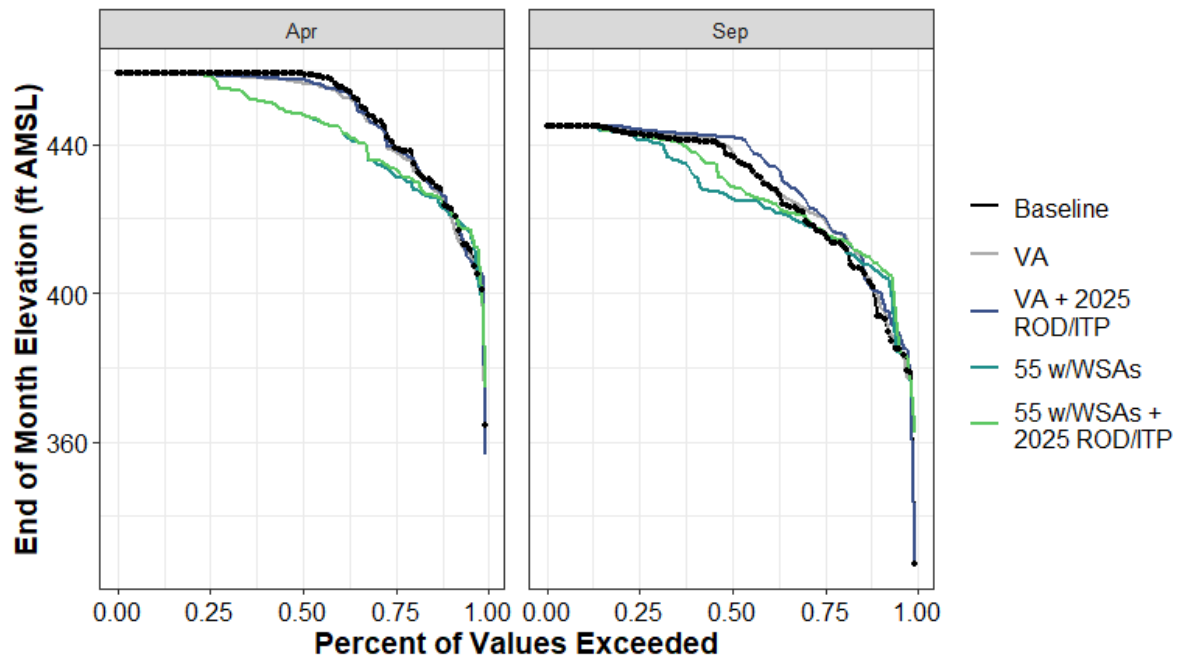
Figure H1a7-89. Folsom Lake Reservoir End-of-April and End-of-September Elevation (ft AMSL) Percent Exceedance Plot
