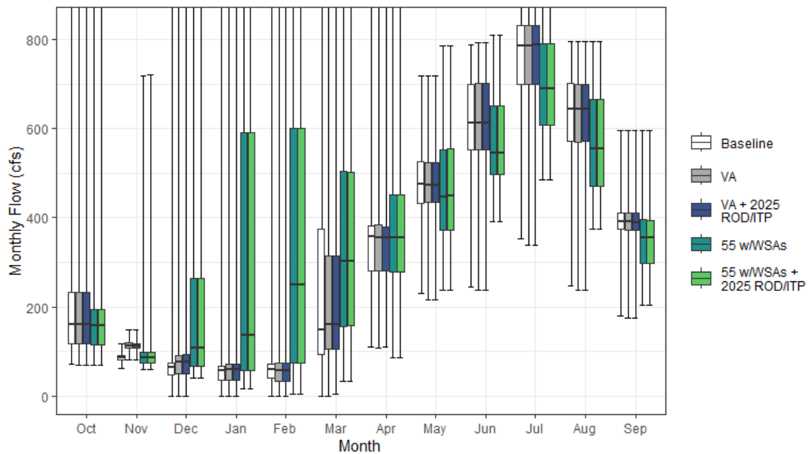
Figure H1a7-26. Putah Creek Streamflow below Lake Berryessa Monthly Boxplot (cfs)
