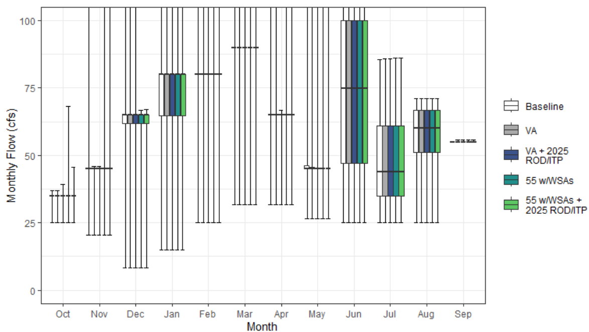
Figure H1a7-58. Toadtown Canal Monthly Boxplot (cfs)
