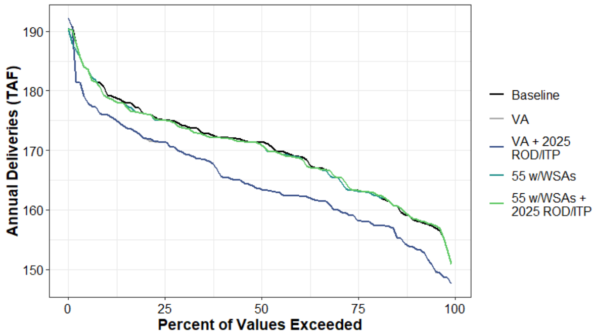
Figure H1a7-189. Total Water Supplied to Water Budget Area 22 (Agricultural) Annual Percent Exceedance Plot.
