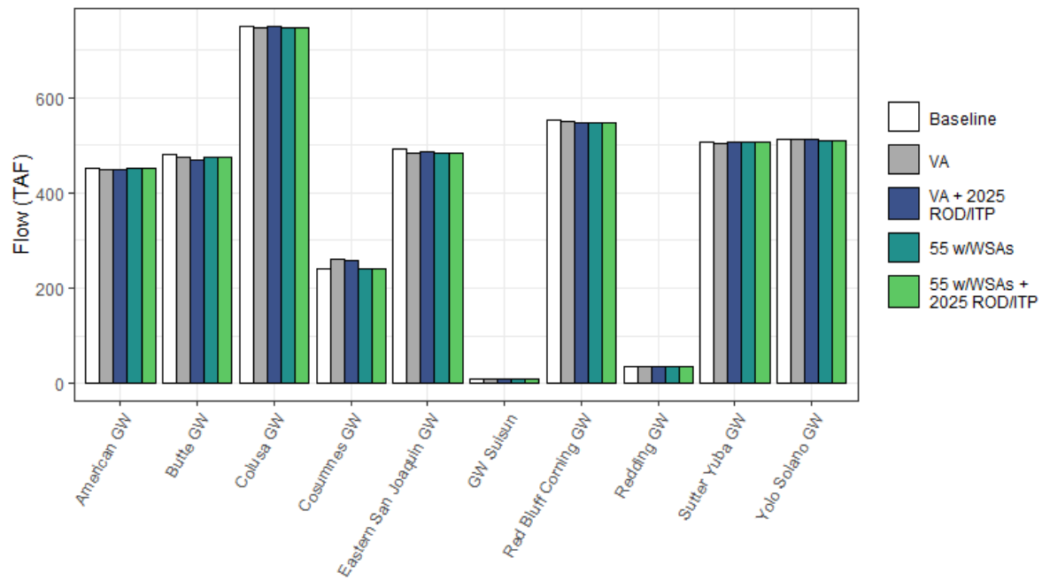
Figure H1a7-232. Annual Average Groundwater Pumping by Basin (TAF/yr).
