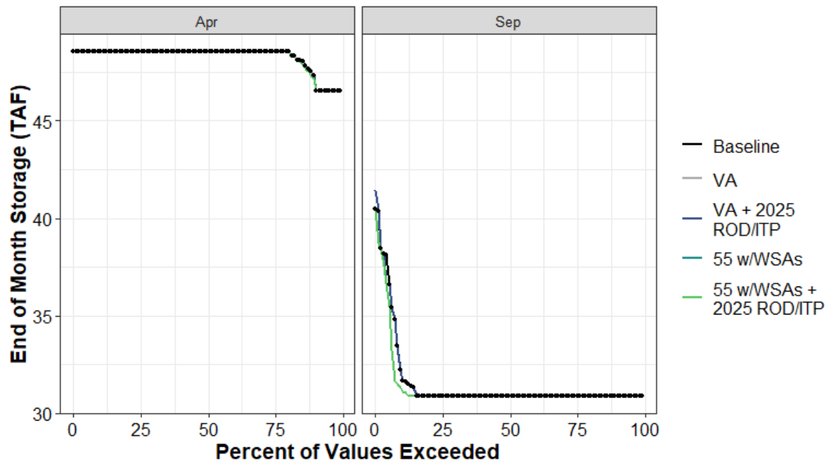
Figure H1a7-141. Scotts Flat Reservoir End of April and End of September Storage (TAF) Percent Exceedance Plot
