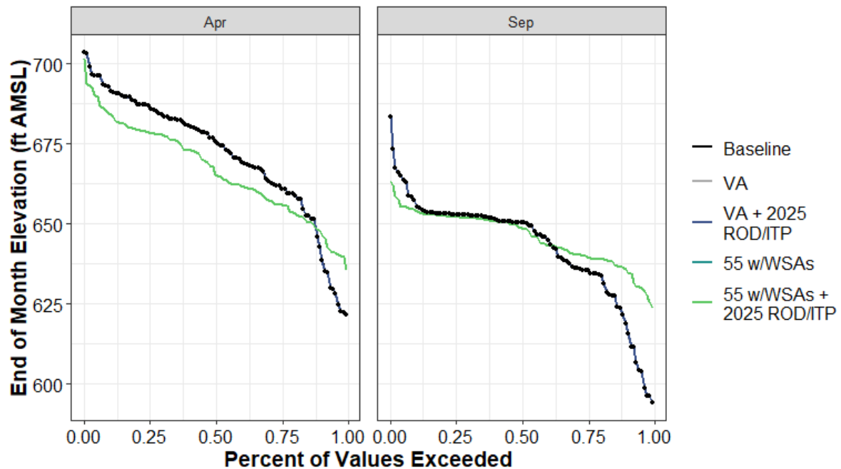
Figure H1a7-131. New Hogan Reservoir End-of-April and End-of-September Elevation (ft AMSL) Percent Exceedance Plot
