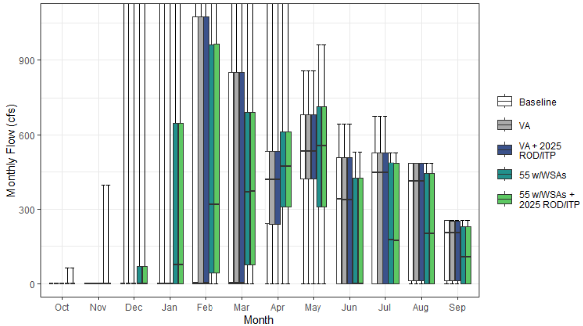
Figure H1a7-9. Cache Creek Streamflow below Clear Lake Monthly Boxplot (cfs)
