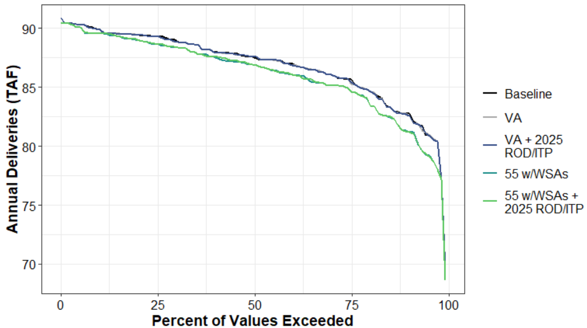
Figure H1a7-203. Surface Water Supplied to Upper Watershed and Foothill (Urban) Annual Percent Exceedance Plot.
