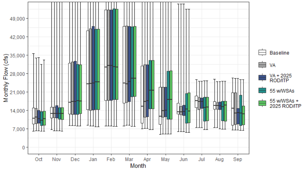
Figure H1a7-32. Sacramento River Streamflow at Freeport Monthly Boxplot (cfs)
