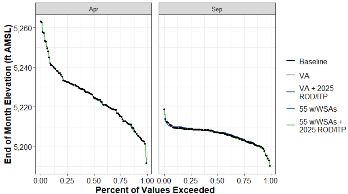
Figure H1a7-92. French Meadows Reservoir End-of-April and End-of-September Elevation (ft AMSL) Percent Exceedance Plot
