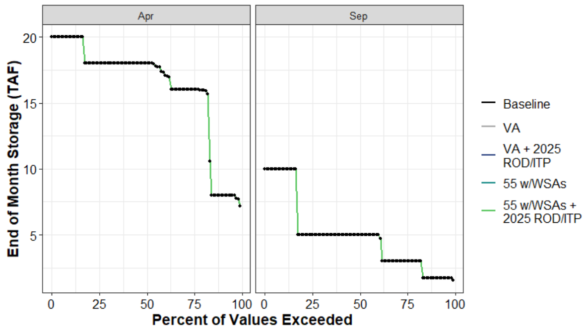
Figure H1a7-127. Mountain Meadows Reservoir End of April and End of September Storage (TAF) Percent Exceedance Plot
