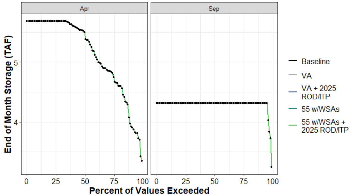
Figure H1a7-116. Lake Valley End of April and End of September Storage (TAF) Percent Exceedance Plot
