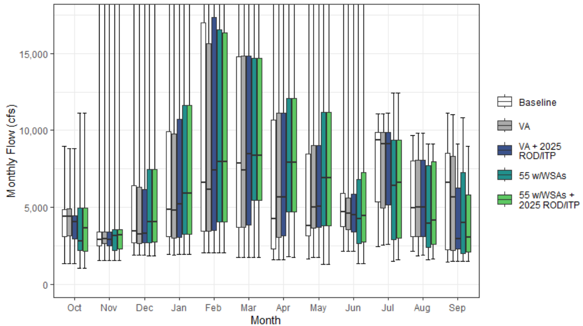
Figure H1a7-20. Feather River Streamflow above Confluence with Sacramento River Monthly Boxplot (cfs)
