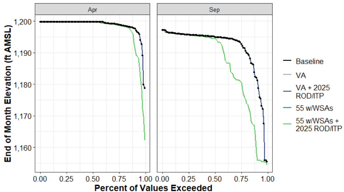
Figure H1a7-87. East Park Reservoir End-of-April and End-of-September Elevation (ft AMSL) Percent Exceedance Plot
