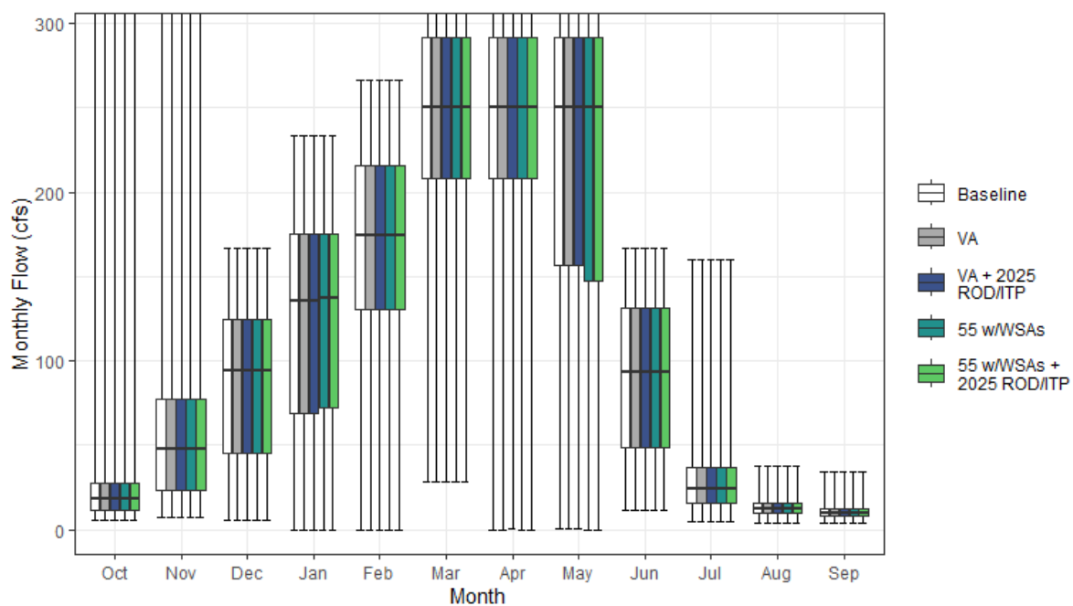
Figure H1a7-59. Slate Creek Tunnel Monthly Boxplot (cfs)
