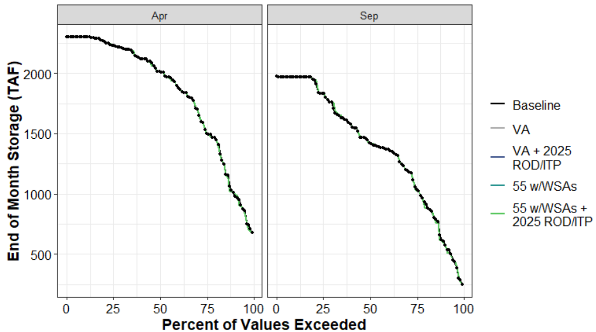
Figure H1a7-155. Trinity Reservoir End of April and End of September Storage (TAF) Percent Exceedance Plot
