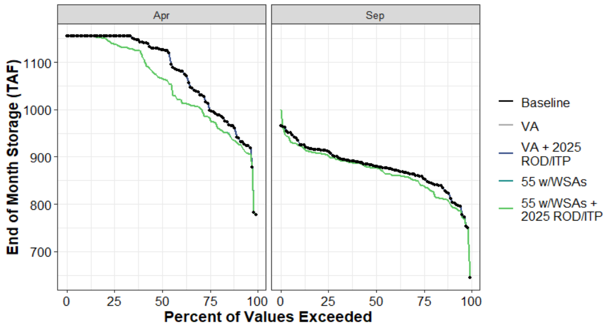
Figure H1a7-83. Clear Lake End of April and End of September Storage (TAF) Percent Exceedance Plot
