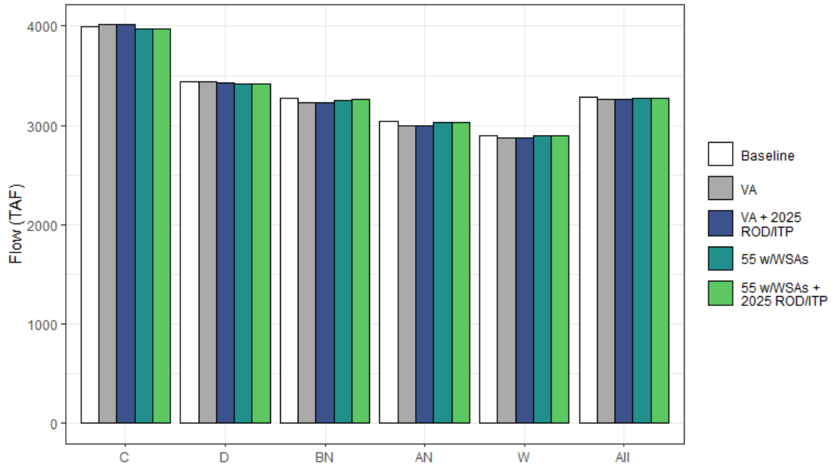
Figure H1a7-231. Average Total Annual Groundwater Pumping for the Sacramento Watershed Region by WYT and Scenario (TAF/yr).
