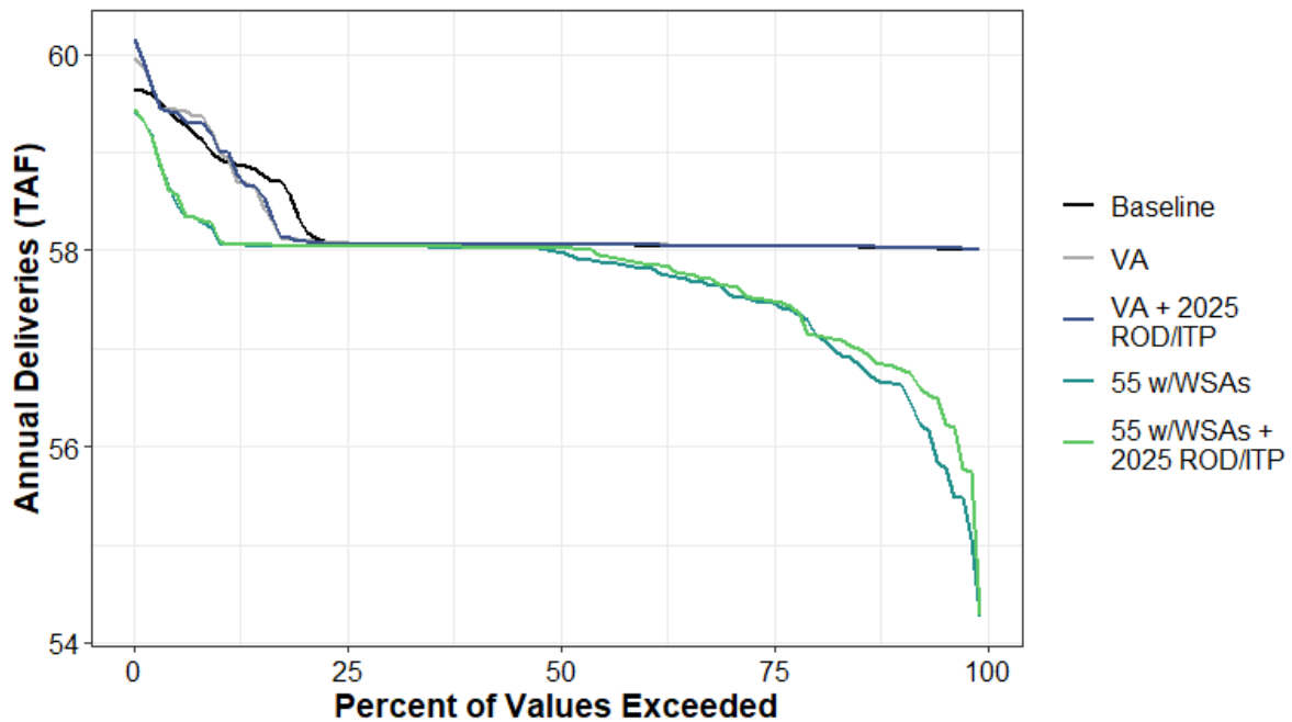
Figure H1a7-186. Total Water Supplied to Water Budget Areas 20 and 25 (Urban) Annual Percent Exceedance Plot.
