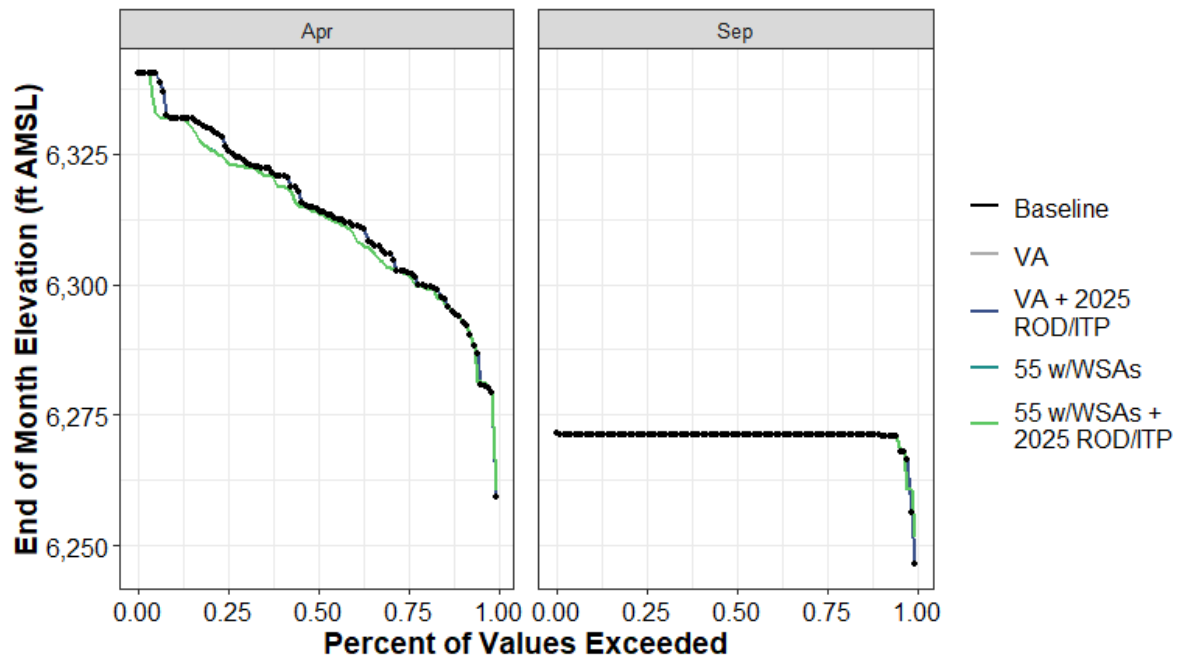
Figure H1a7-113. Lake Fordyce Reservoir End-of-April and End-of-September Elevation (ft AMSL) Percent Exceedance Plot
