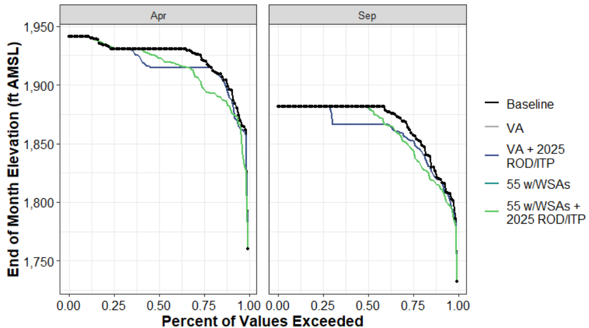
Figure H1a7-129. New Bullards Bar Reservoir End-of-April and End-of-September Elevation (ft AMSL) Percent Exceedance Plot
