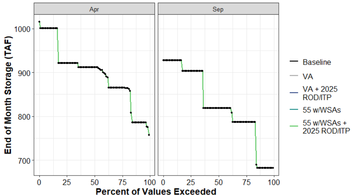
Figure H1a7-104. Lake Almanor End of April and End of September Storage (TAF) Percent Exceedance Plot
