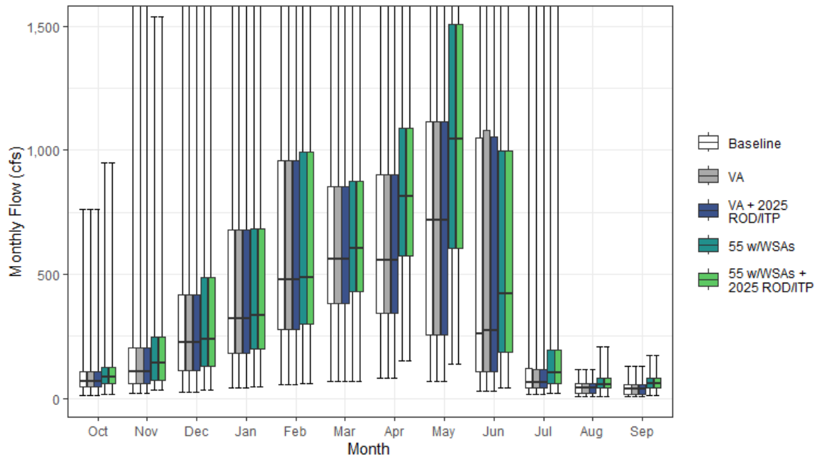
Figure H1a7-42. Yuba River, South Fork Streamflow above Confluence with Yuba River Monthly Boxplot (cfs)
