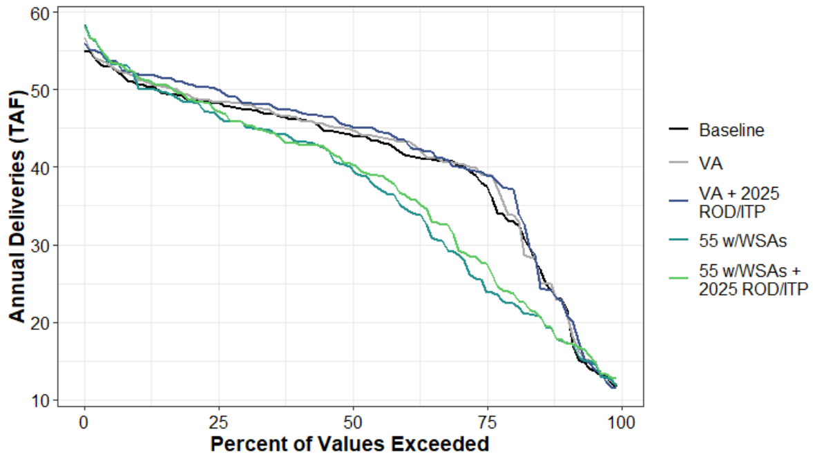
Figure H1a7-220. Surface Water Supplied to SWP Table A North of Delta Annual Percent Exceedance Plot.
