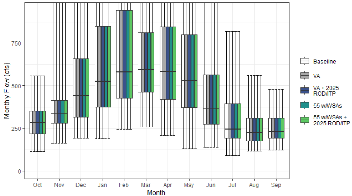
Figure H1a7-4. Battle Creek Streamflow above Confluence with Sacramento River Monthly Boxplot (cfs)
