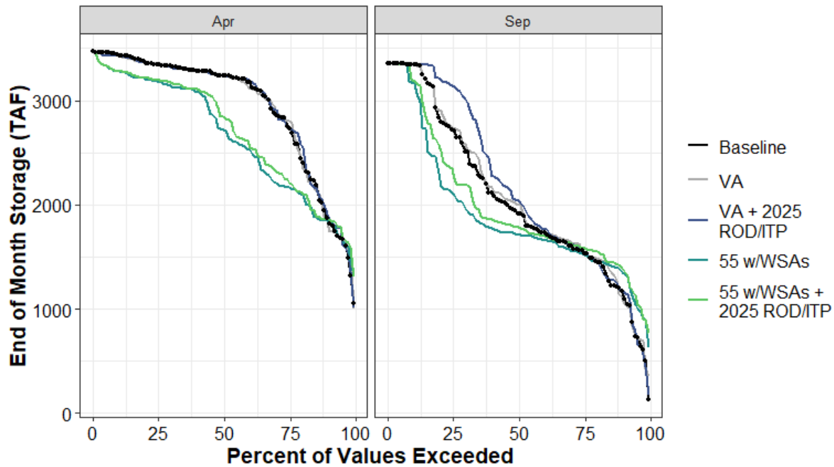
Figure H1a7-132. Oroville Reservoir End of April and End of September Storage (TAF) Percent Exceedance Plot
