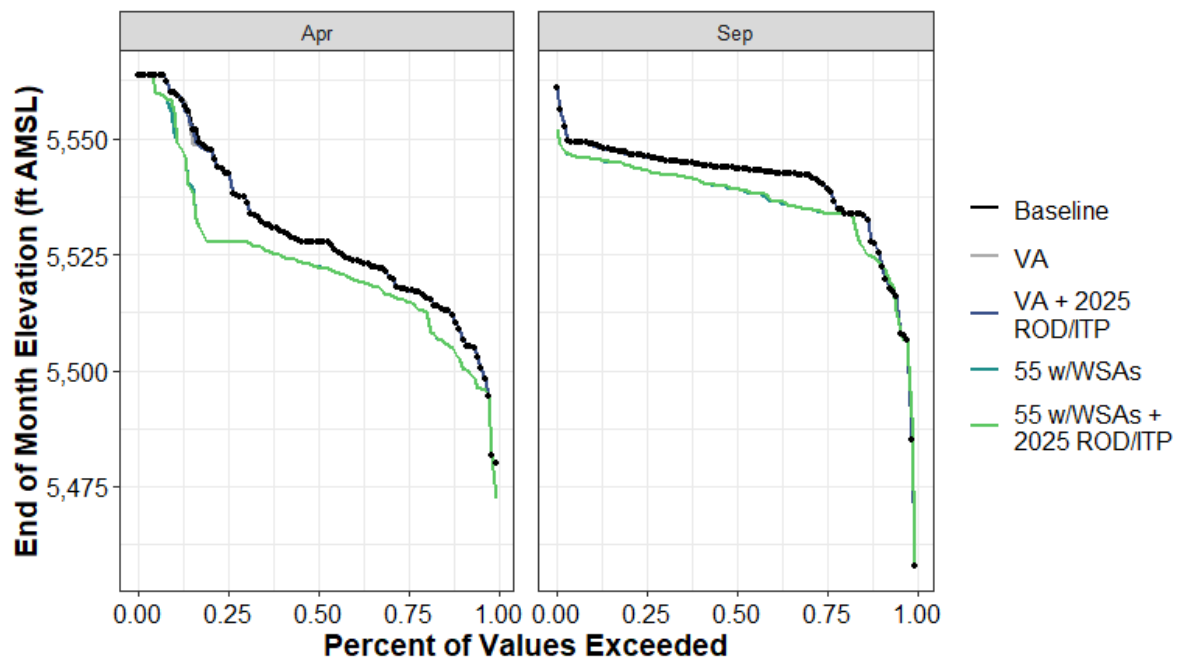
Figure H1a7-72. Bowman Lake Reservoir End-of-April and End-of-September Elevation (ft AMSL) Percent Exceedance Plot
