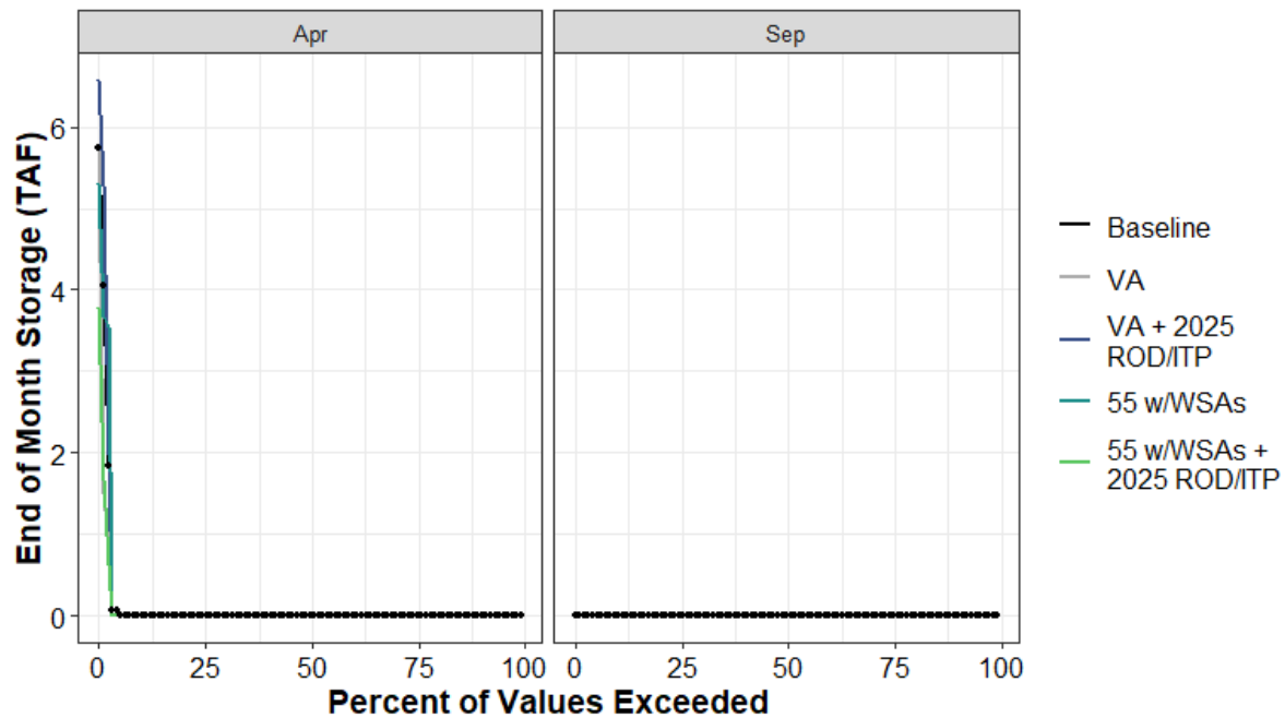
Figure H1a7-90. French Lake End of April and End of September Storage (TAF) Percent Exceedance Plot
