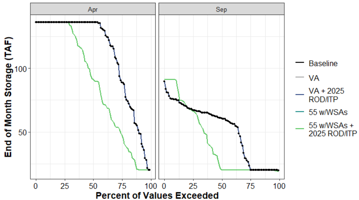
Figure H1a7-69. Black Butte Reservoir End of April and End of September Storage (TAF) Percent Exceedance Plot
