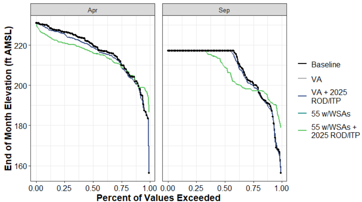
Figure H1a7-78. Camanche Reservoir End-of-April and End-of-September Elevation (ft AMSL) Percent Exceedance Plot
