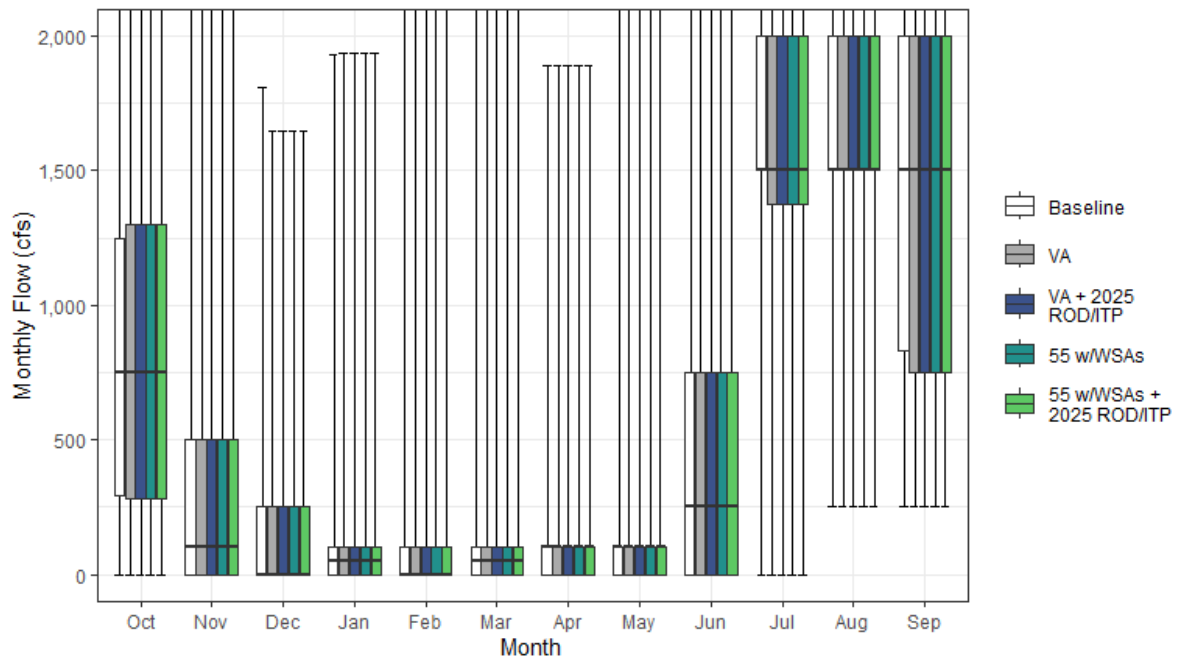
Figure H1a7-63. Clear Creek Tunnel Monthly Boxplot (cfs)
