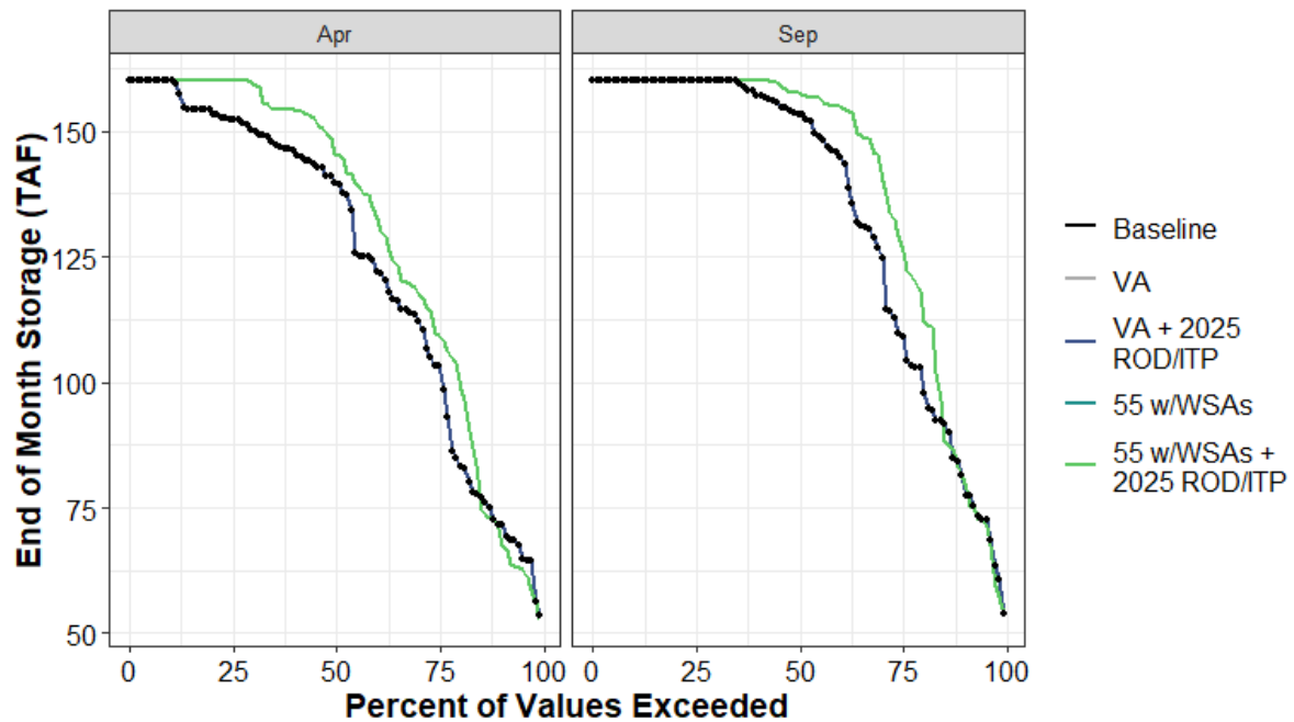
Figure H1a7-121. Los Vaqueros Reservoir End of April and End of September Storage (TAF) Percent Exceedance Plot
