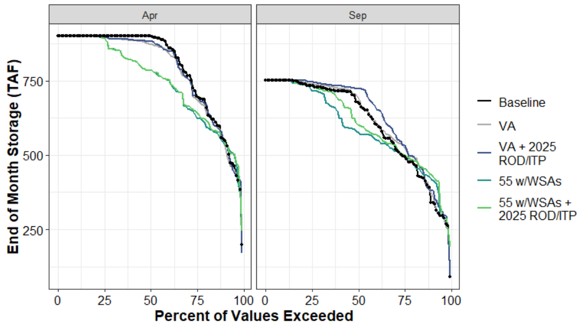
Figure H1a7-88. Folsom Lake End of April and End of September Storage (TAF) Percent Exceedance Plot
