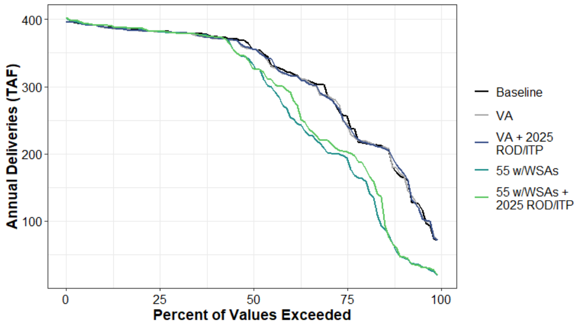
Figure H1a7-208. Surface Water Supplied to CVP North of Delta Water Service (Agricultural) Annual Percent Exceedance Plot.
