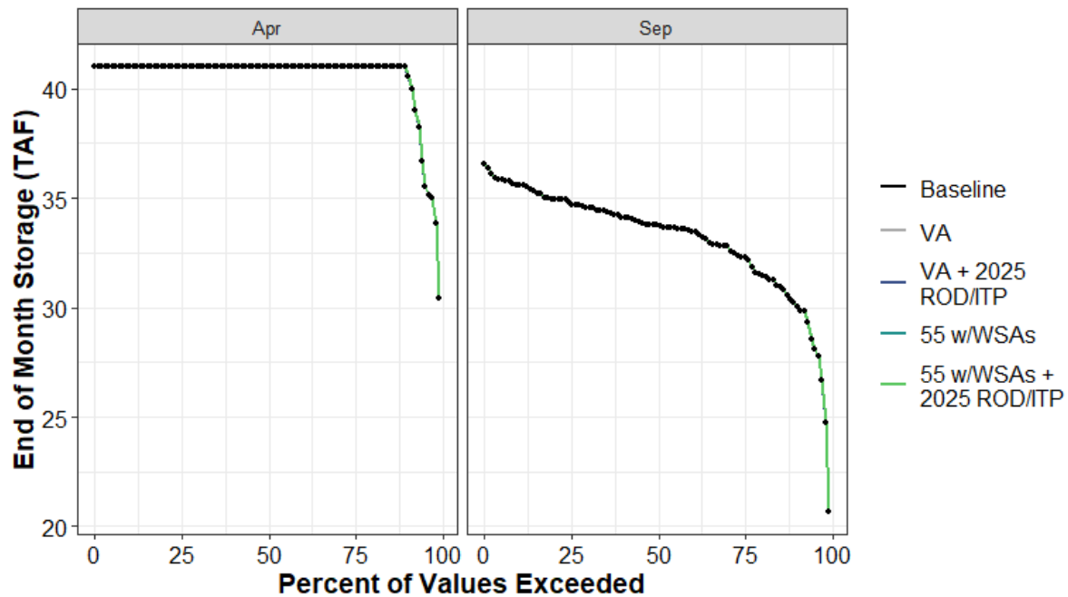
Figure H1a7-103. Jenkinson Lake End of April and End of September Storage (TAF) Percent Exceedance Plot
