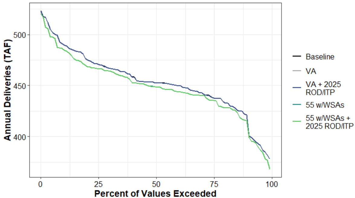
Figure H1a7-197. Total Water Supplied to Water Budget Area 60N (Agricultural) Annual Percent Exceedance Plot.
