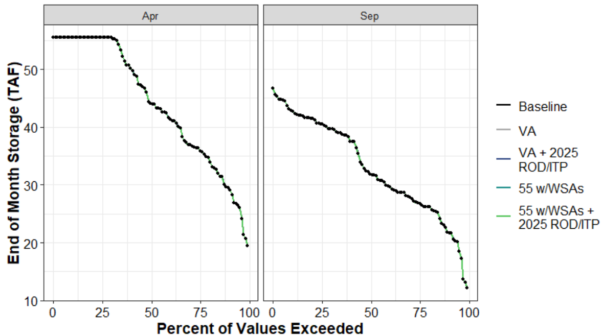
Figure H1a7-93. Frenchman Lake End of April and End of September Storage (TAF) Percent Exceedance Plot
