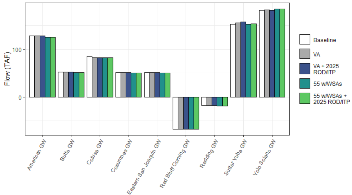
Figure H1a7-240. Stream-Groundwater Flux (Net Groundwater Gain) by Basin (TAF/yr).
