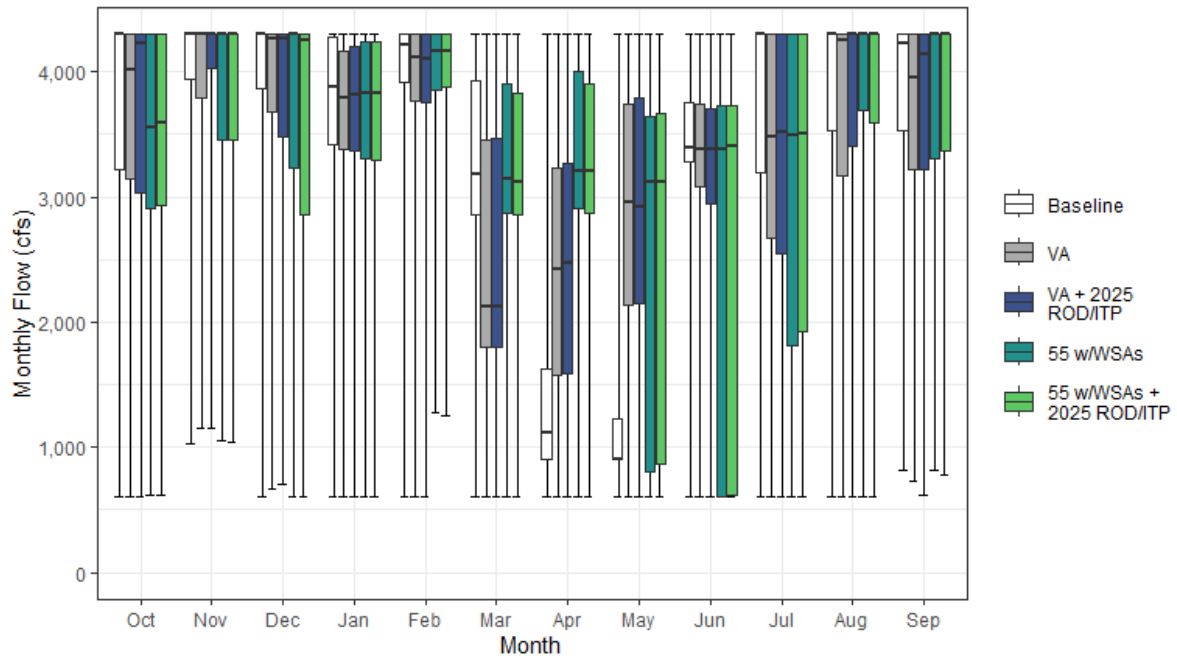
Figure H1a7-51. Jones Pumping Plant (CVP) Monthly Boxplot (cfs)
