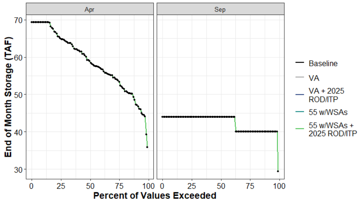
Figure H1a7-119. Loon Lake End of April and End of September Storage (TAF) Percent Exceedance Plot
