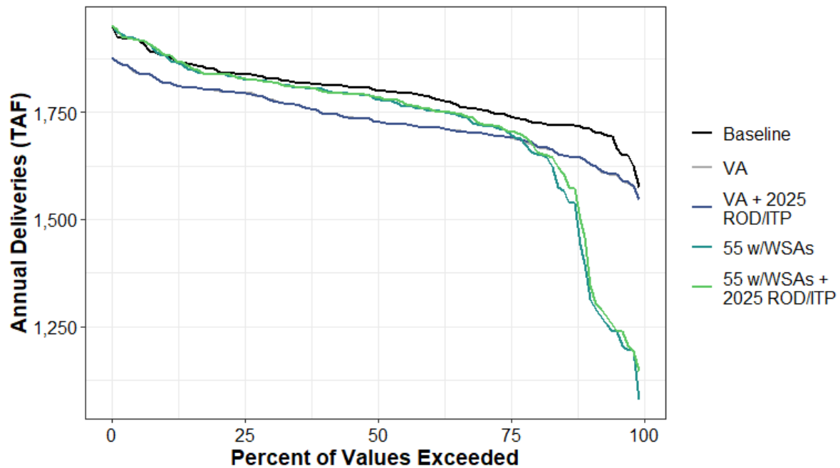
Figure H1a7-210. Surface Water Supplied to CVP Settlement (Agricultural) Annual Percent Exceedance Plot.
