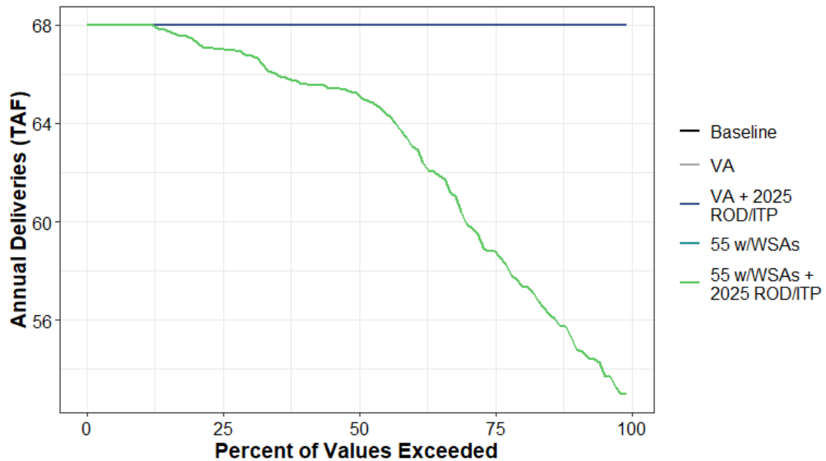
Figure H1a7-200. Total Water Supplied to Water Budget Area 60S (Urban) Annual Percent Exceedance Plot.
