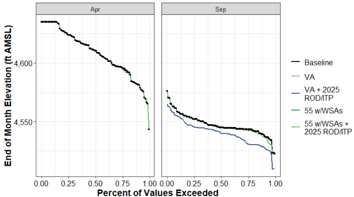
Figure H1a7-96. Hell Hole Reservoir End-of-April and End-of-September Elevation (ft AMSL) Percent Exceedance Plot
