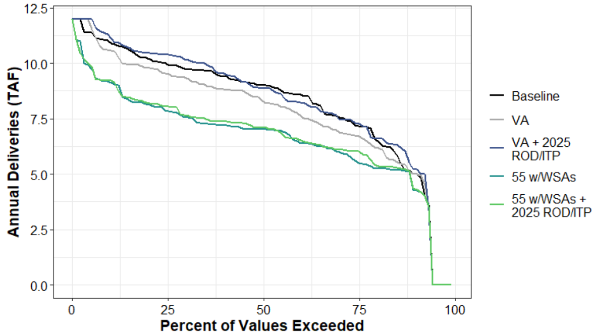
Figure H1a7-226. Surface Water Supplied to SWP Article 21 Napa Annual Percent Exceedance Plot.
