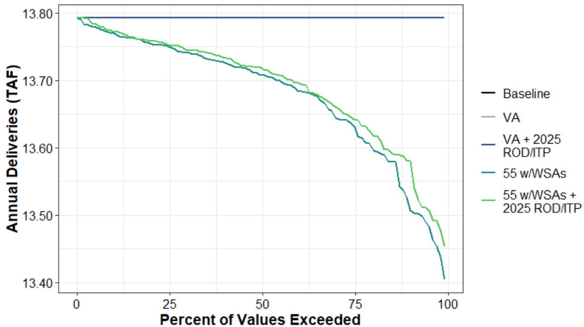
Figure H1a7-176. Total Water Supplied to Water Budget Areas 12 and 13 (Urban) Annual Percent Exceedance Plot.
