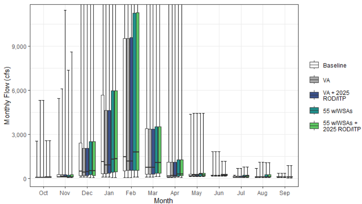
Figure H1a7-39. Yolo Bypass Streamflow below Putah Creek Inflow Monthly Boxplot (cfs)
