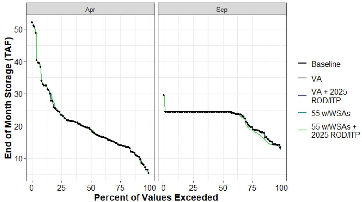
Figure H1a7-123. Lower Bear End of April and End of September Storage (TAF) Percent Exceedance Plot
