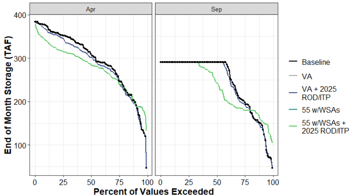
Figure H1a7-77. Camanche Reservoir End of April and End of September Storage (TAF) Percent Exceedance Plot
