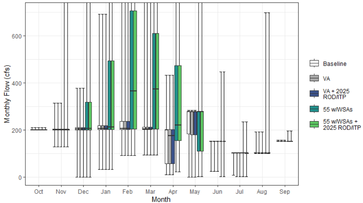
Figure H1a7-13. Clear Creek Streamflow above Confluence with Sacramento River Monthly Boxplot (cfs)
