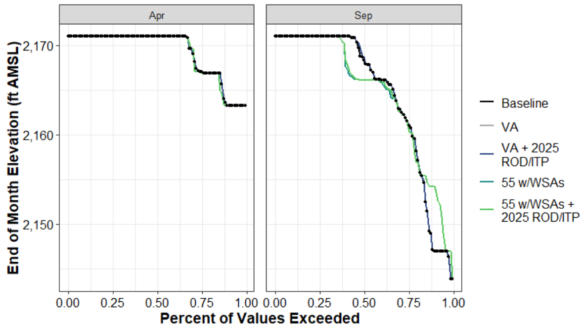
Figure H1a7-138. Rollins Reservoir End-of-April and End-of-September Elevation (ft AMSL) Percent Exceedance Plot
