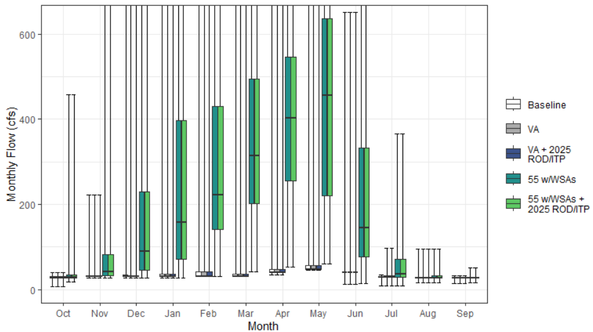
Figure H1a7-41. Yuba River, Middle Fork Streamflow above Confluence with North Fork Yuba Monthly Boxplot (cfs)
