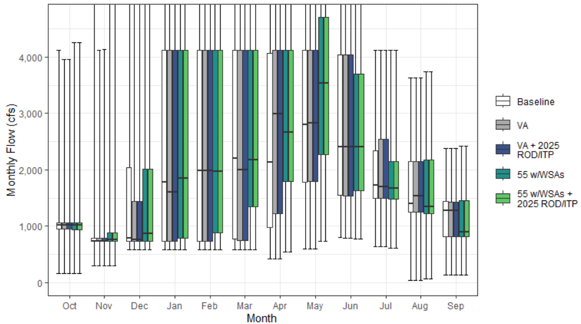
Figure H1a7-43. Yuba River Streamflow below Englebright Reservoir Monthly Boxplot (cfs)
