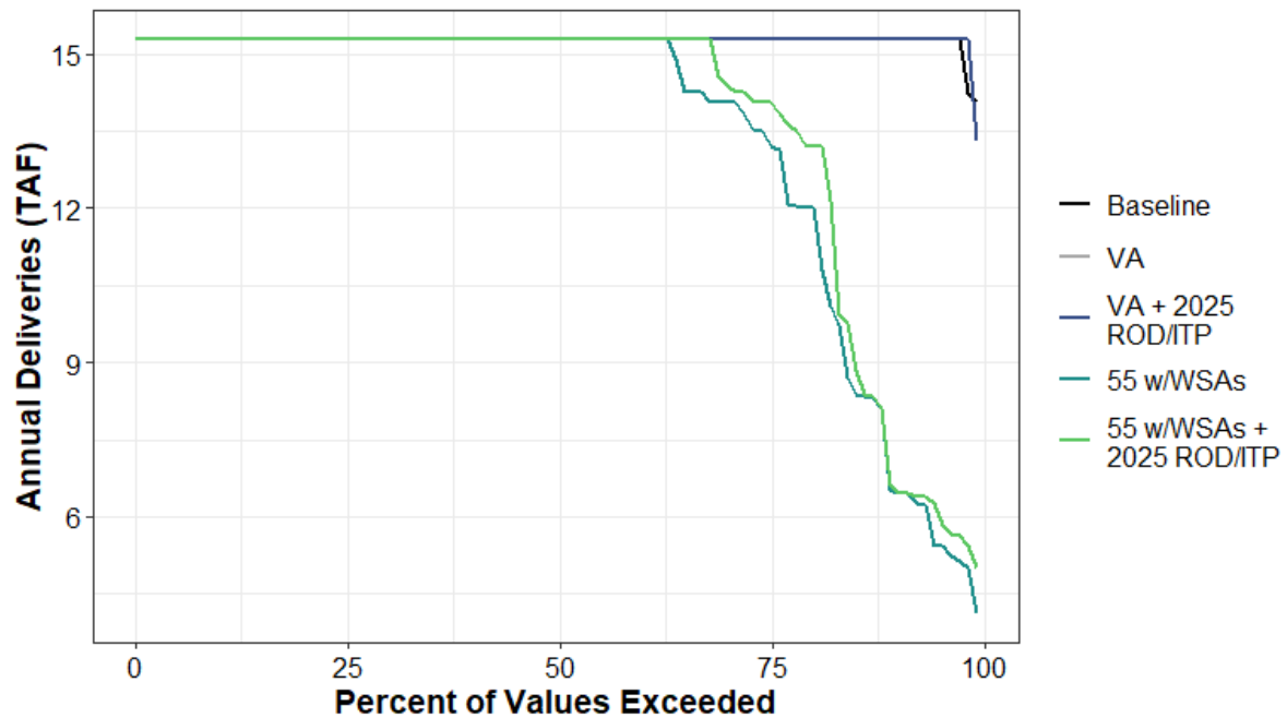
Figure H1a7-188. Total Water Supplied to Water Budget Area 21 (Urban) Annual Percent Exceedance Plot.
