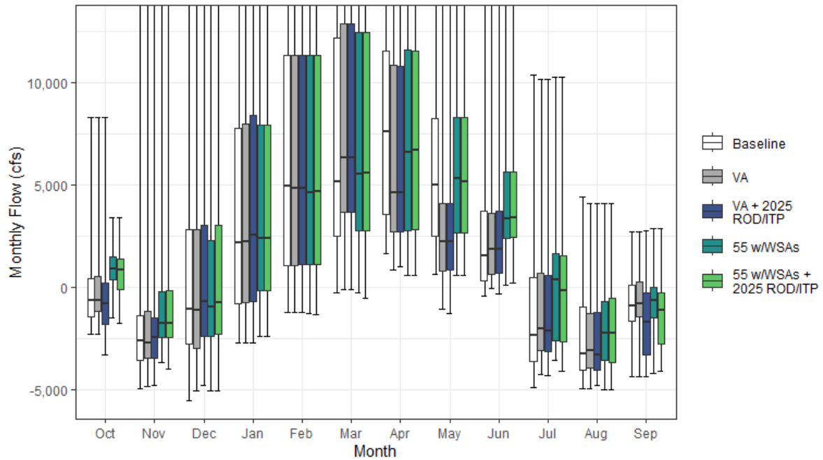
Figure H1a7-49. San Joaquin River at Jersey Point (QWEST) Monthly Boxplot (cfs)
