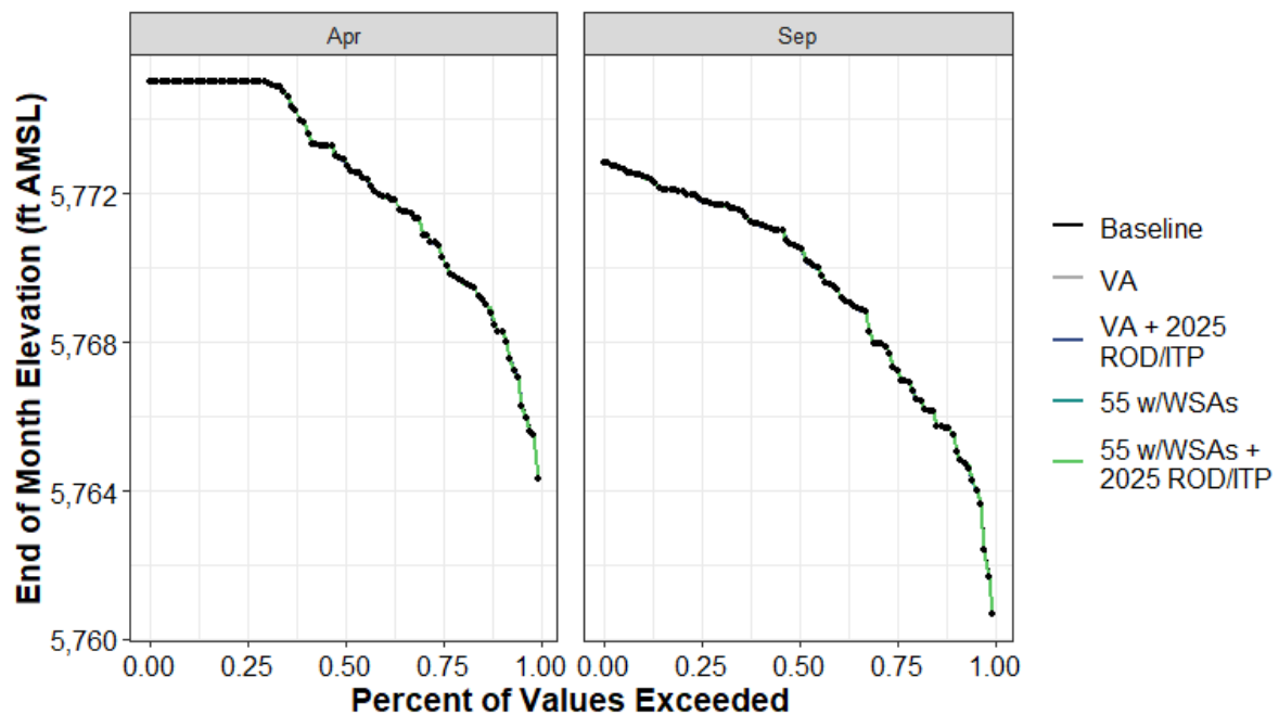
Figure H1a7-111. Lake Davis Reservoir End-of-April and End-of-September Elevation (ft AMSL) Percent Exceedance Plot
