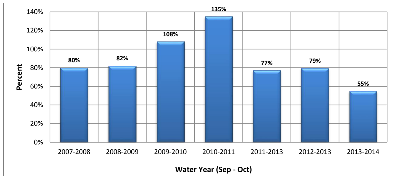
Figure 12 - Percent of Normal Precipitation in California by Water Year
