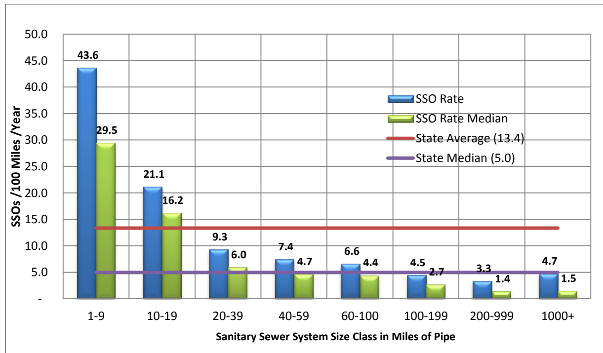
Figure 19 – SSO Rates for Municipal Sanitary Sewer Systems by System Size for Fiscal Year 2013-2014
