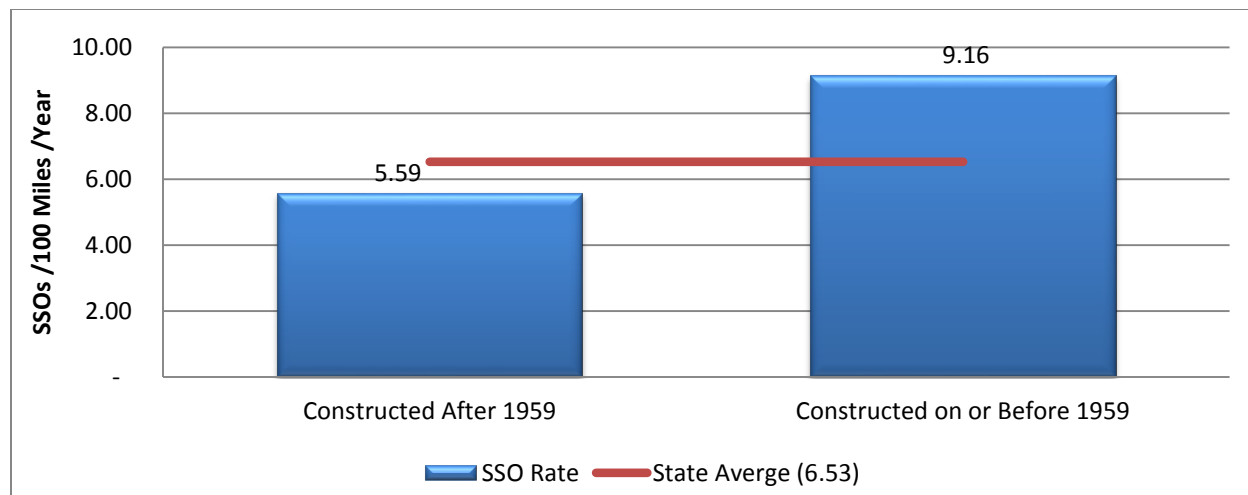
Figure 20 – SSO Rates Correlated to Pipe Age (Data from 1/2/2007 to 6/30/2013)
