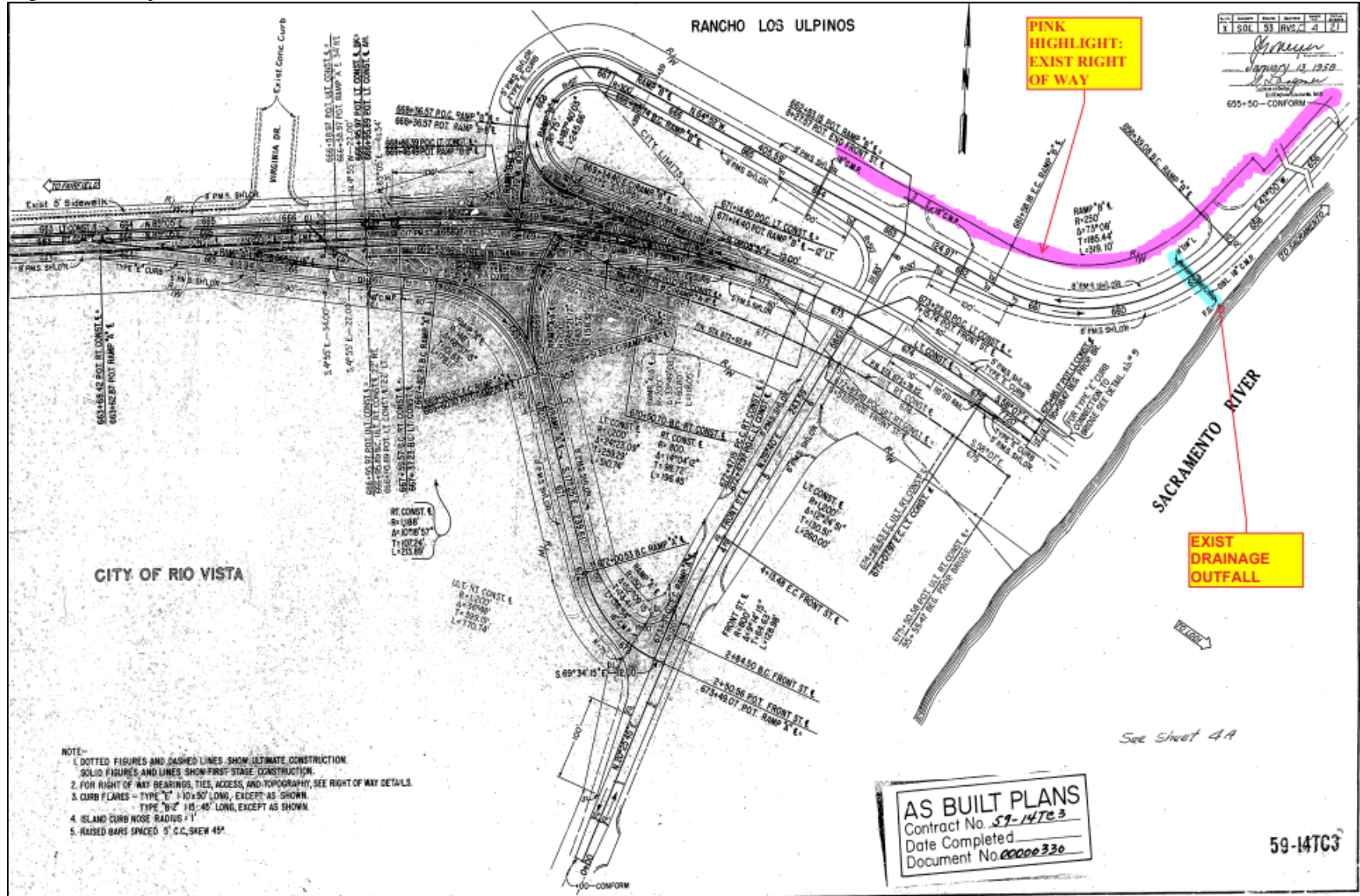
Figure 3: Project Construction Plan
