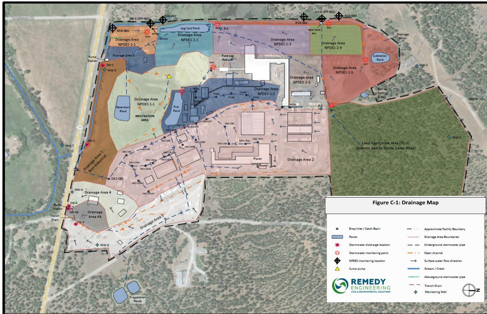
Figure C-1. Facility Storm Water Drainage Map
