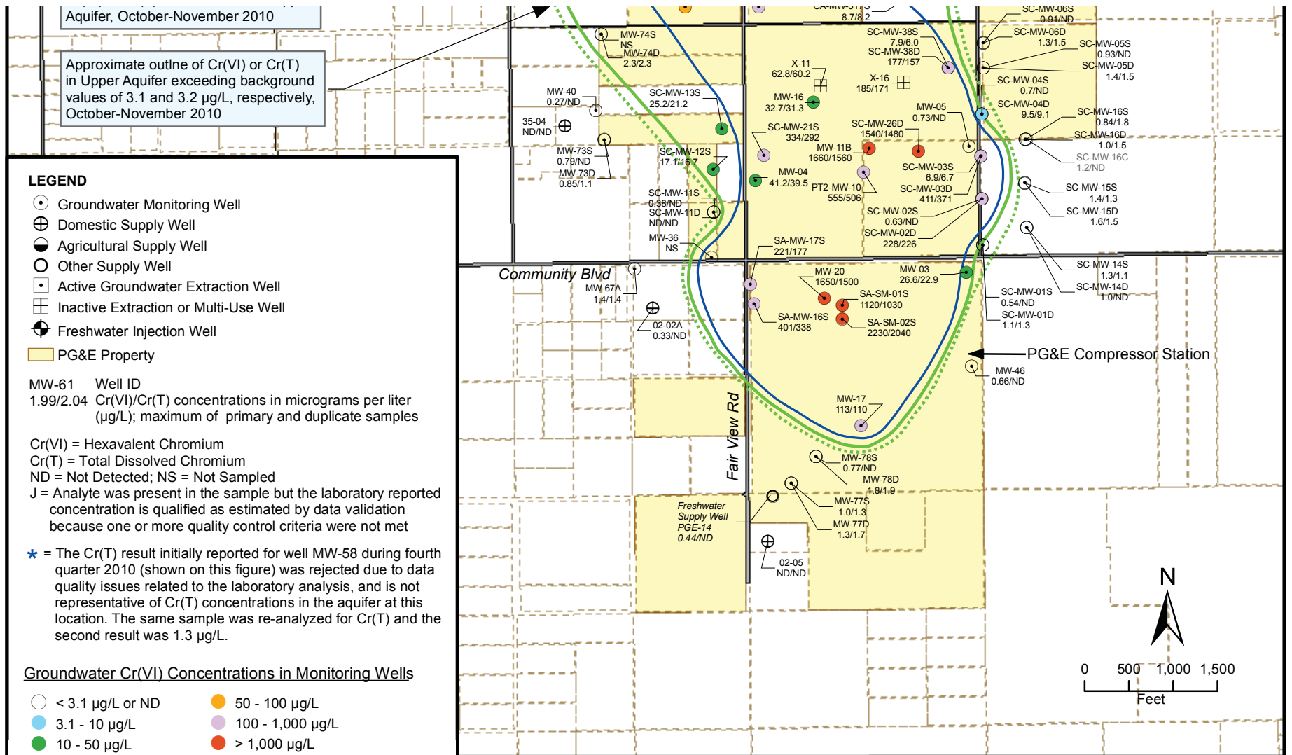
FIGURE 4 REVISED 2/10/2011 HEXAVALENT AND TOTAL CHROMIUM CONCENTRATIONS OCTOBER-NOVEMBER 2010 AND INTERPRETED MAXIMUM PLUME OUTLINE IN UPPER AQUIFER
