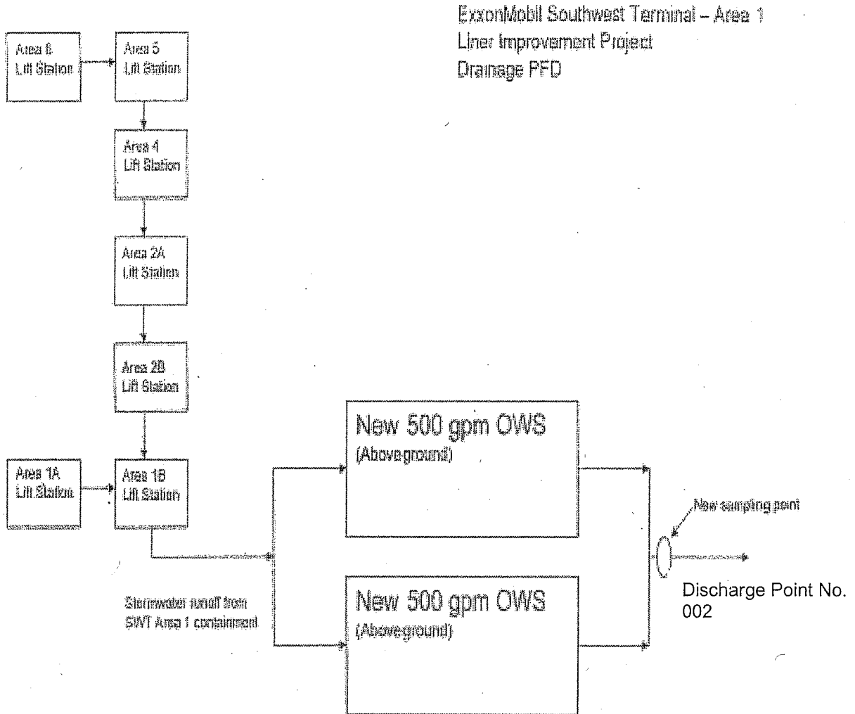
Form 2-F, Attachment IV.B, Outfall 002 Flow Diagram
