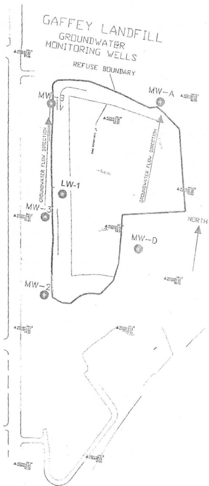
Figure 3. Groundwater Gradient
