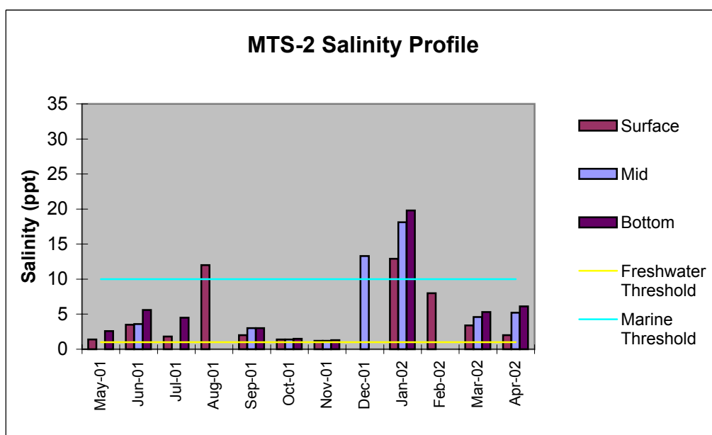
Figure 3-1a: Salinity Profiles at Different Depths at Metals Translator Stations MTS-1 and MTS-2
