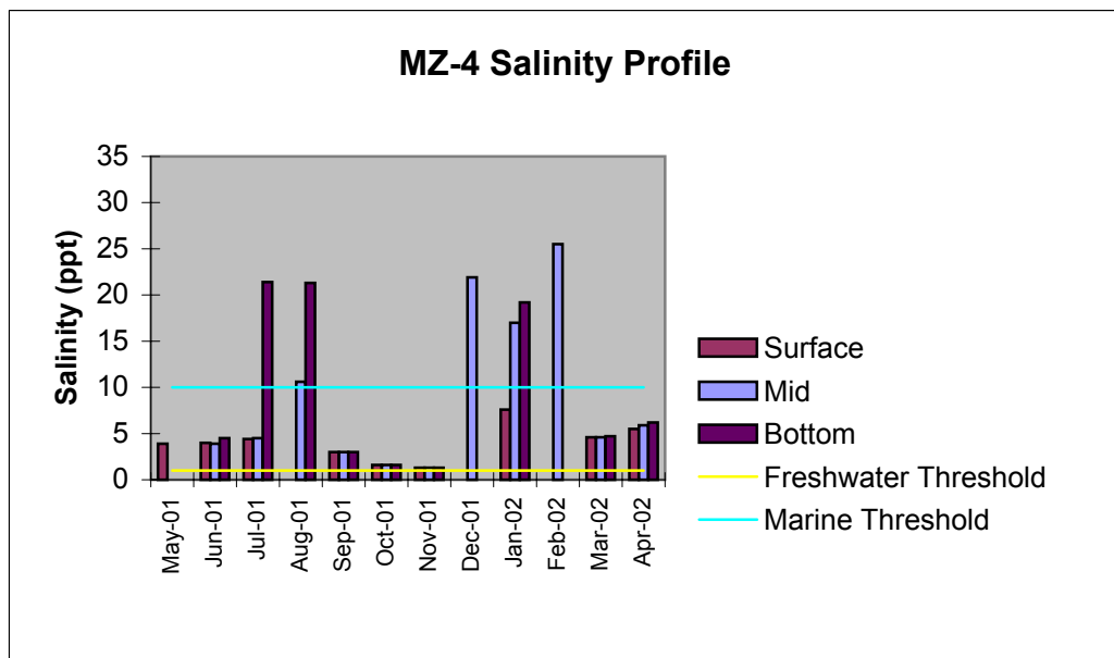
Figure 3-2b: Salinity Profiles at Different Depths at Mixing Zone Stations MZ-3 and MZ-4
