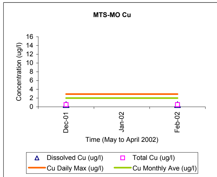
Figure 3-3c: Summary of Copper Concentrations at Metals Translator Station MTS-M and MTS-MO
