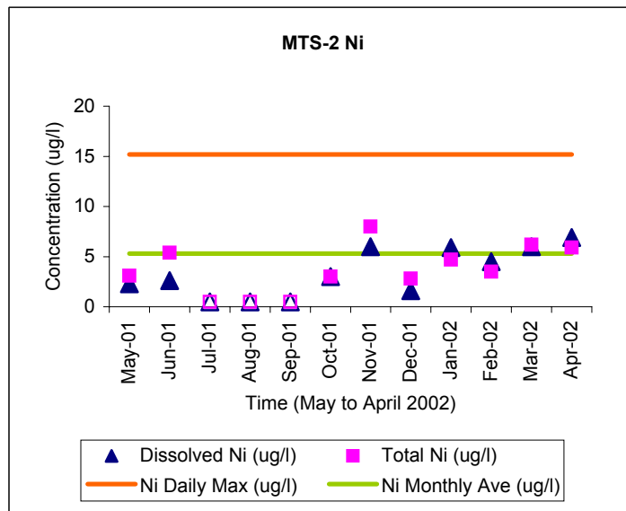
Figure 3-5a: Summary of Nickel Concentrations at Metals Translator Station MTS-1 and MTS-2
