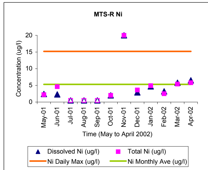
Figure 3-5b: Summary of Nickel Concentrations at Metals Translator Station MTS-3 and MTS-R
