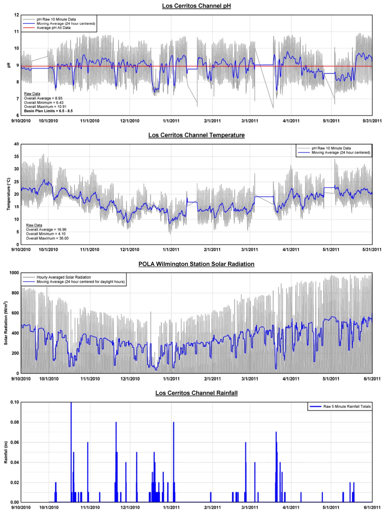
Figure D-6. Time Series Records of pH, Temperature, Solar Radiation and Rainfall in Los Cerritos Channel at Stearns Street. September 10, 2010 to June 1, 2011.
