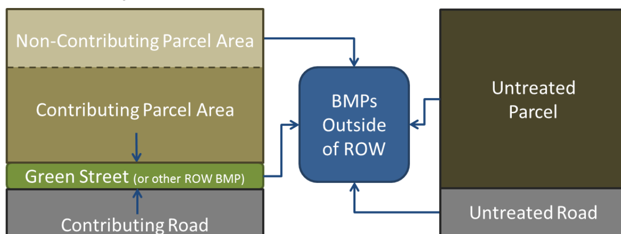
Figure 1-5. Green streets model schematic (arrows denote direction of runoff routing; figure not to scale).
