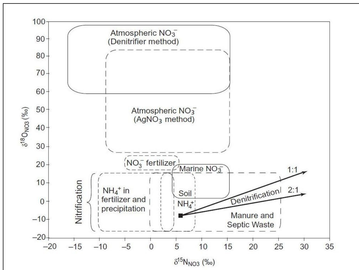
Figure 19. Typical values of \delta^{18}\text{O} and \delta^{15}\text{N} of nitrate derived from various sources (diagram from Michener and Lajtha, 2007).
