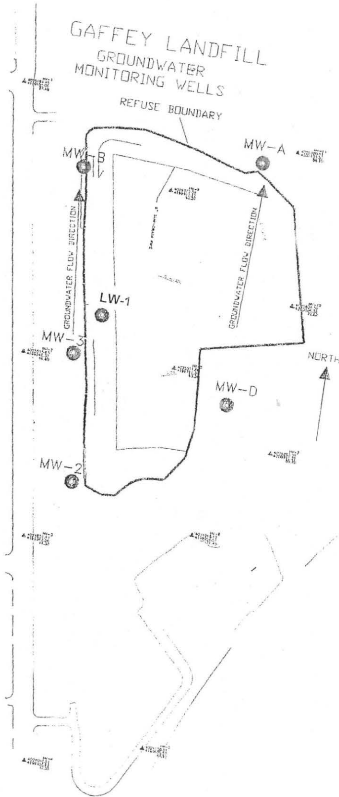
Figure 3. Groundwater Gradient
